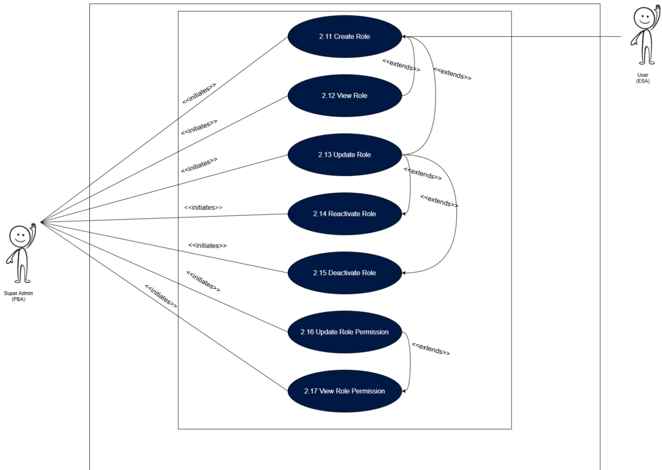
Figure 3: Admin Subsystem Use Case Diagram (Continued)
