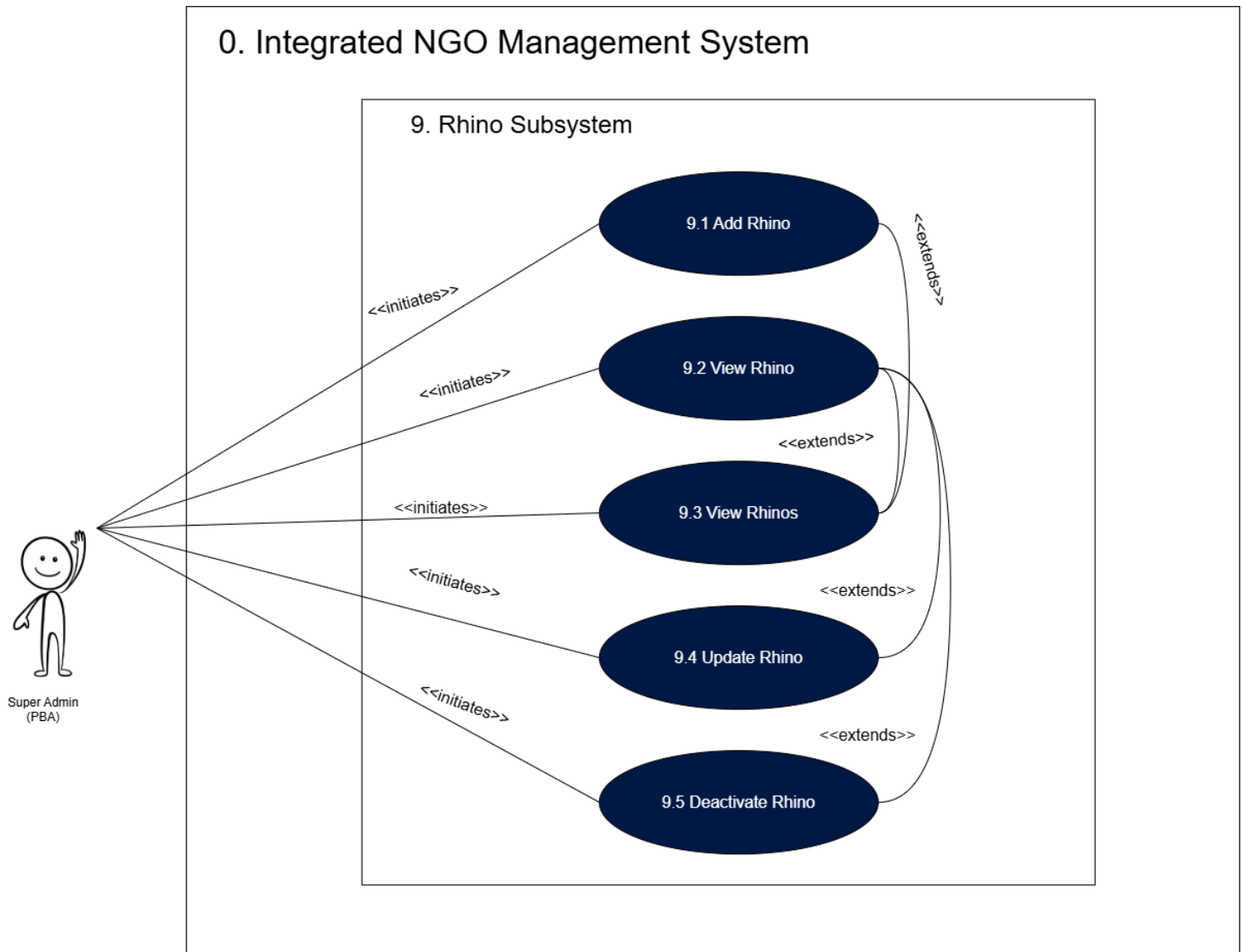
Figure 13: Rhino Subsystem Use Case Diagram
