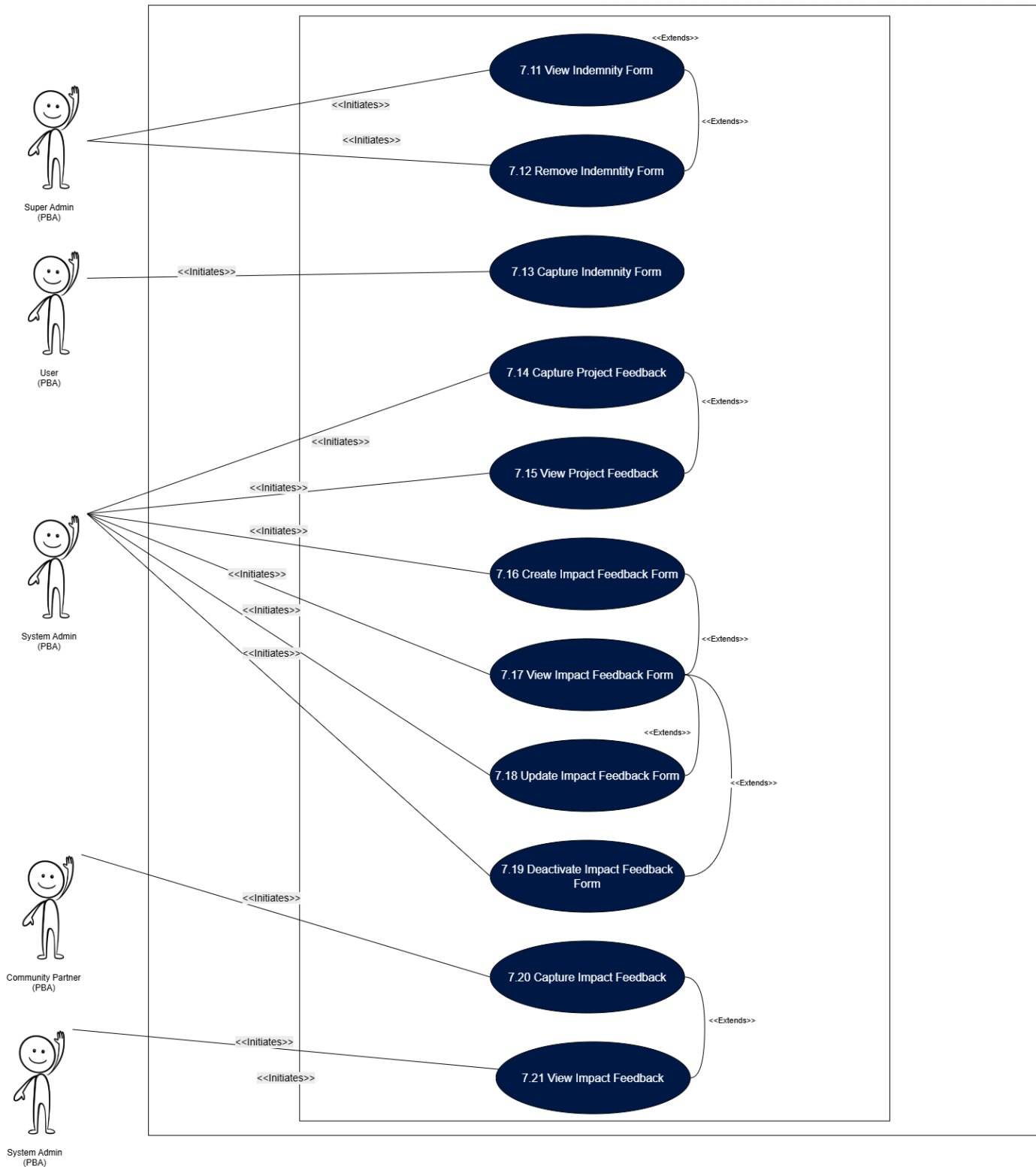
Figure 9: Project Management Subsystem Use Case Diagram (Continued)
