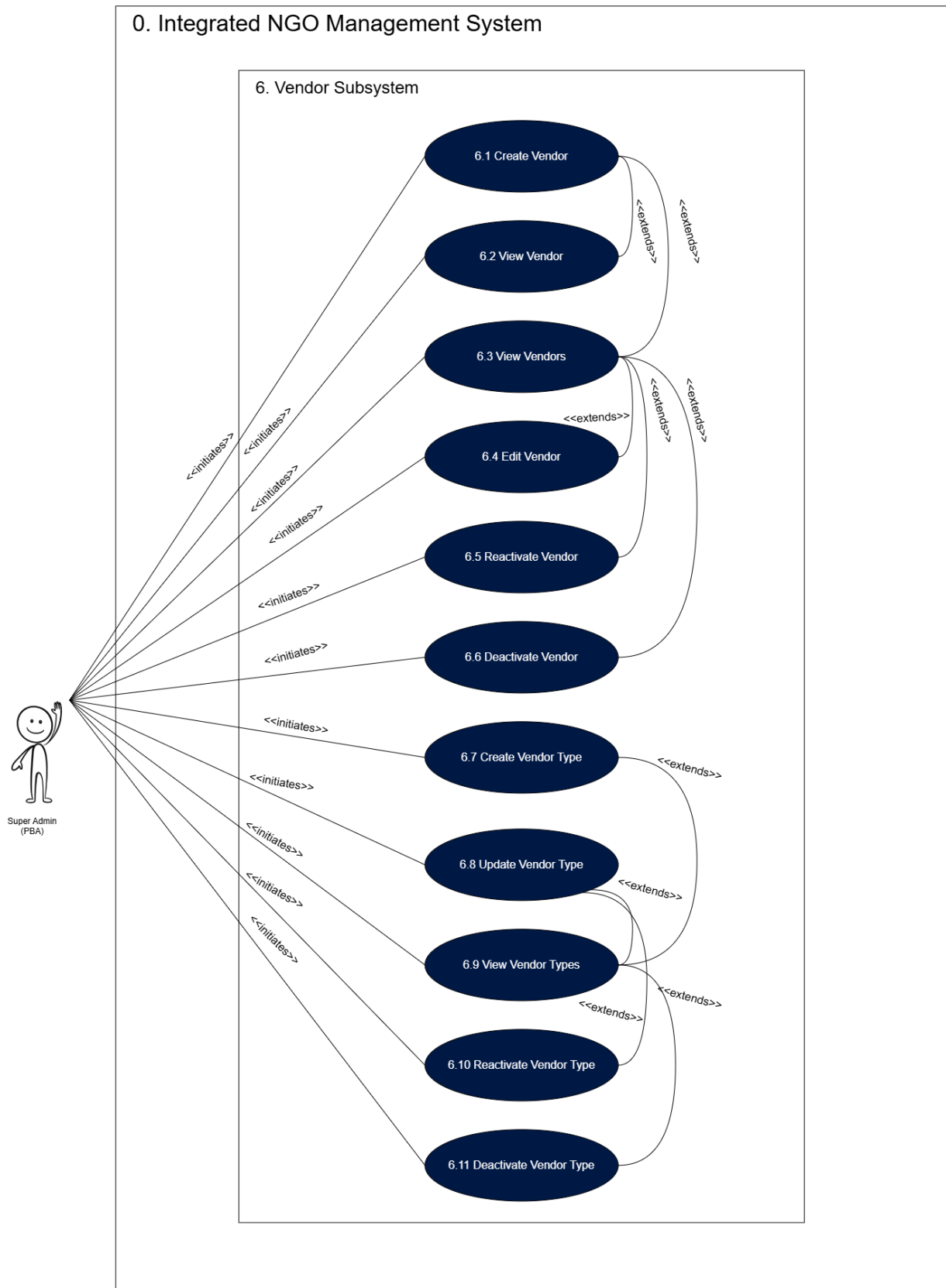
Figure 7: Vendor Subsystem Use Case Diagram
