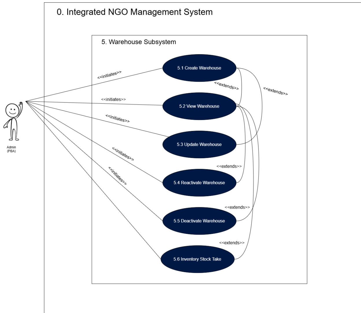
Figure 6: Warehouse Subsystem Use Case Diagram
