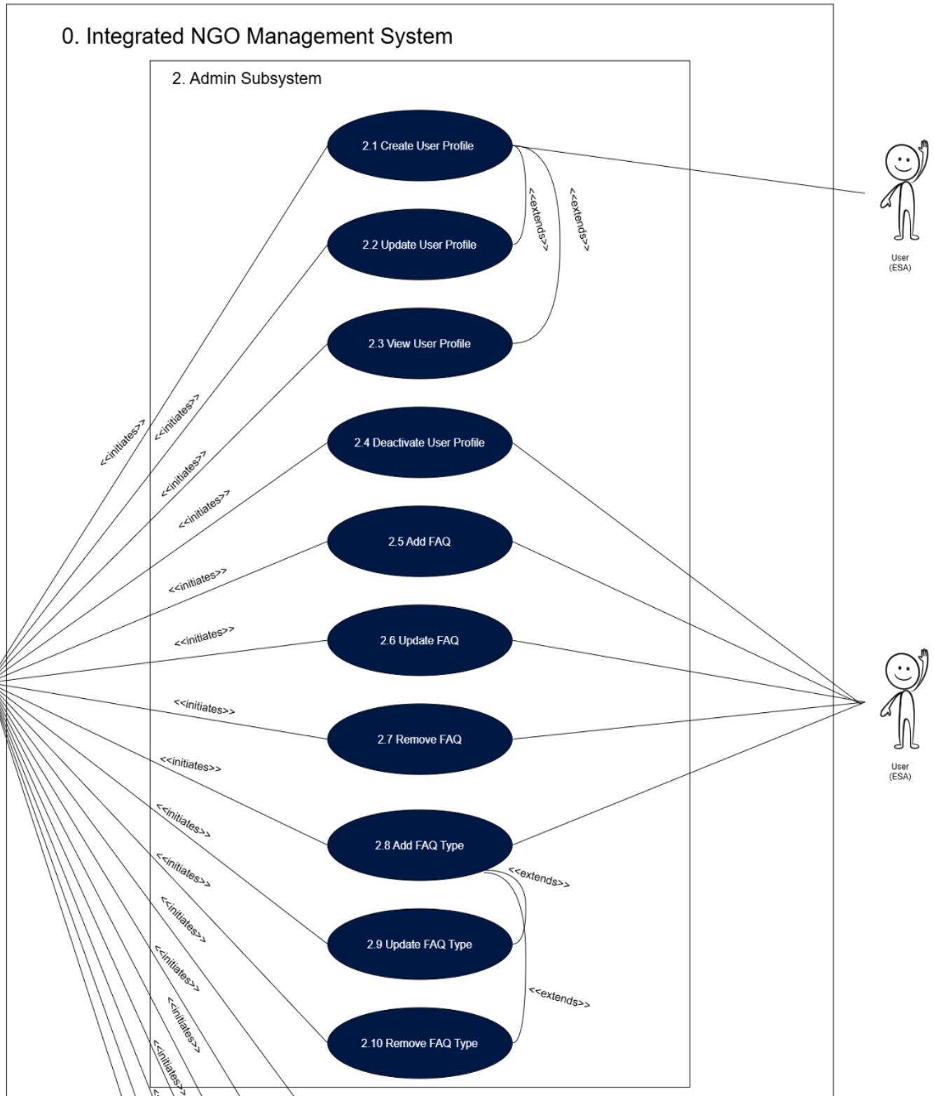
Figure 2: Admin Subsystem Use Case Diagram
