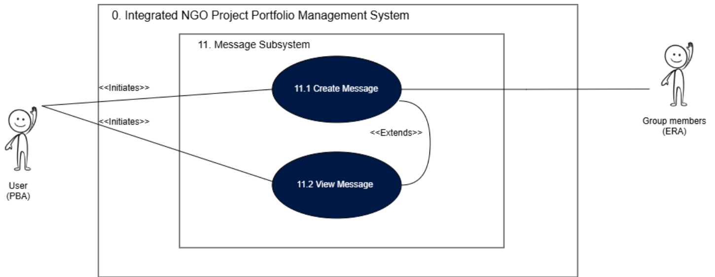
Figure 15: Message Subsystem Use Case Diagram
