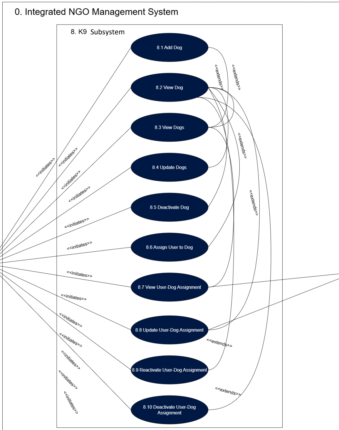
Figure 11: K9 Subsystem Use Case Diagram
