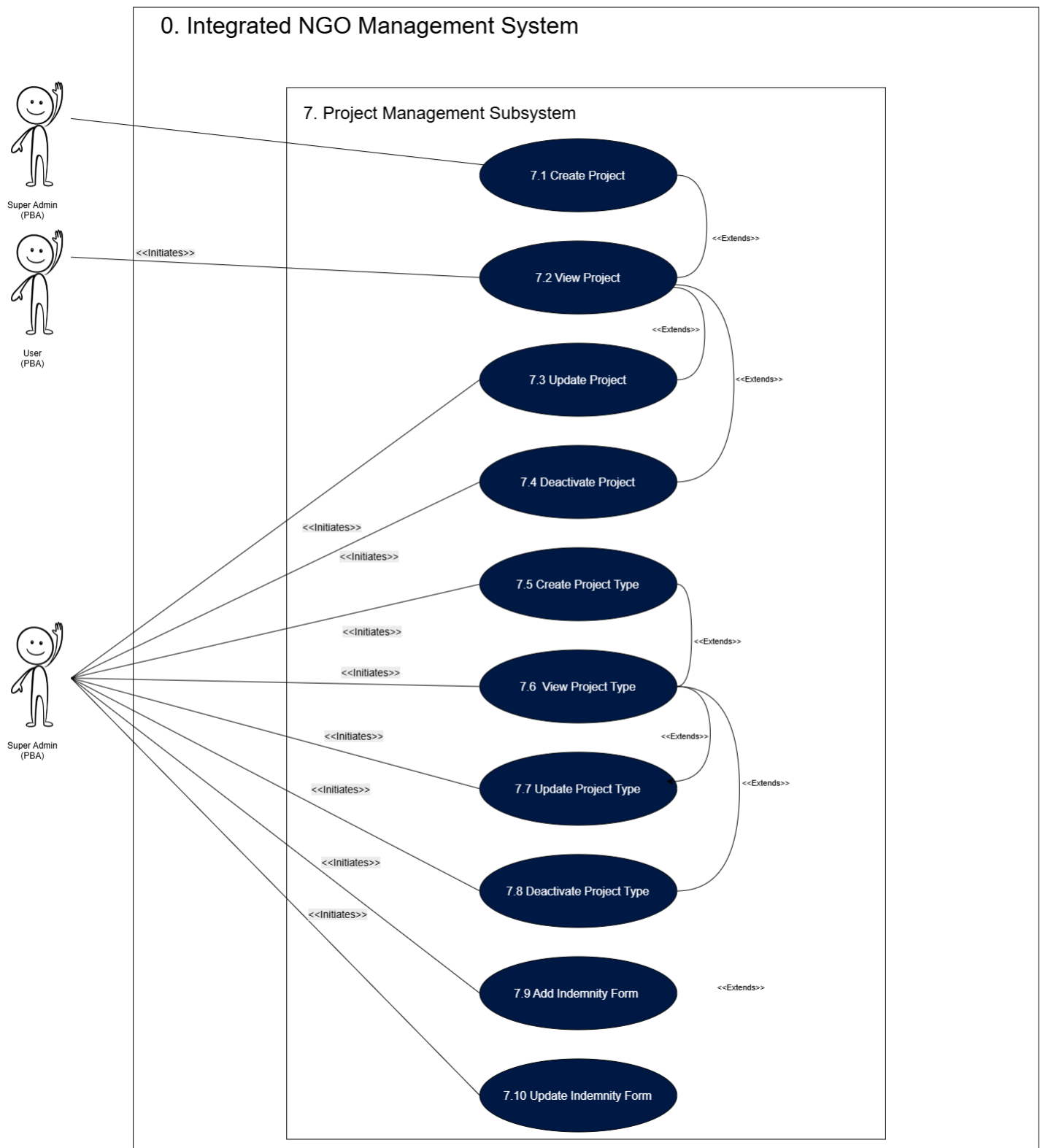
Figure 8: Project Management Subsystem Use Case Diagram
