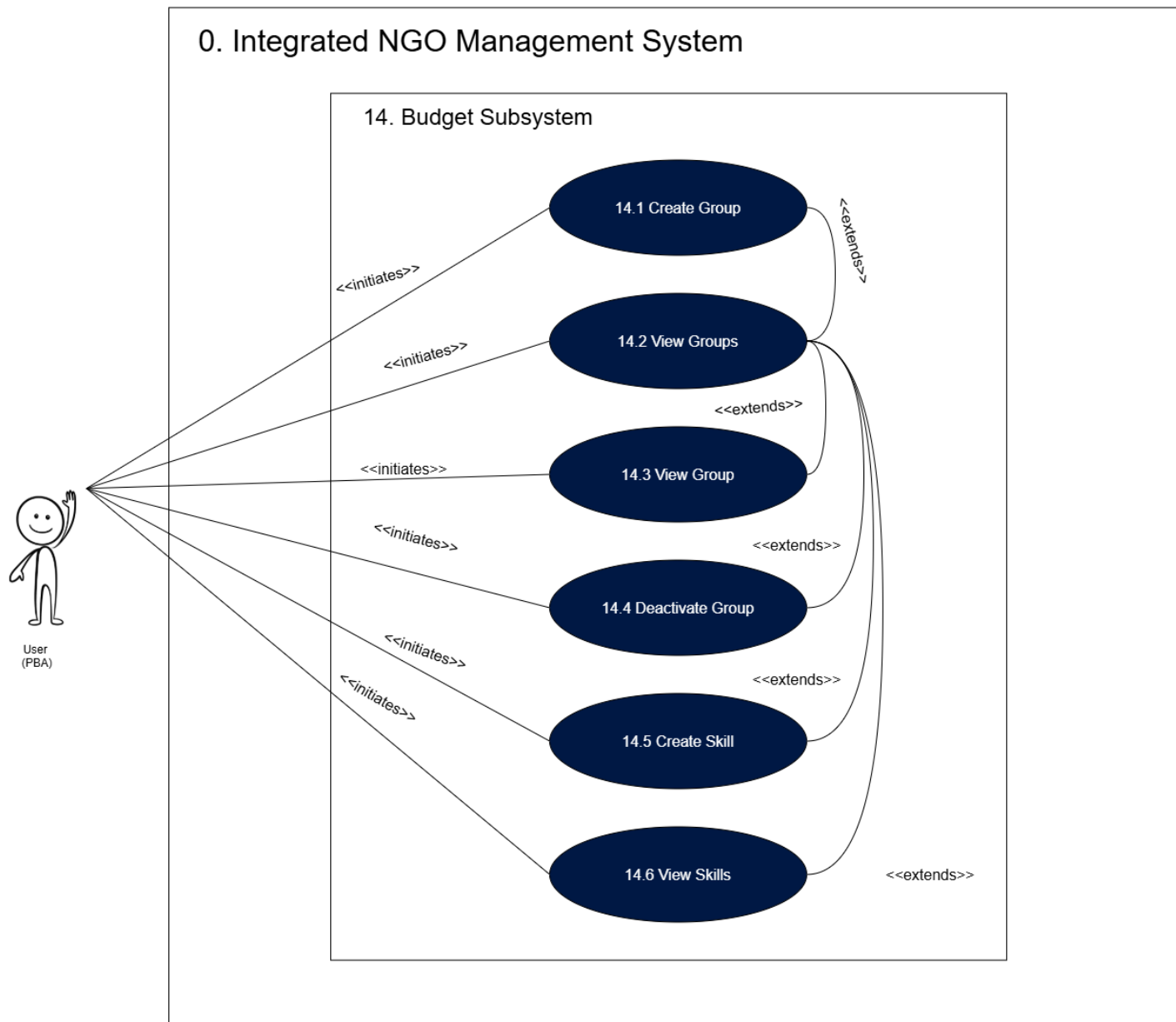
Figure 18: Budget Subsystem Use Case Diagram
