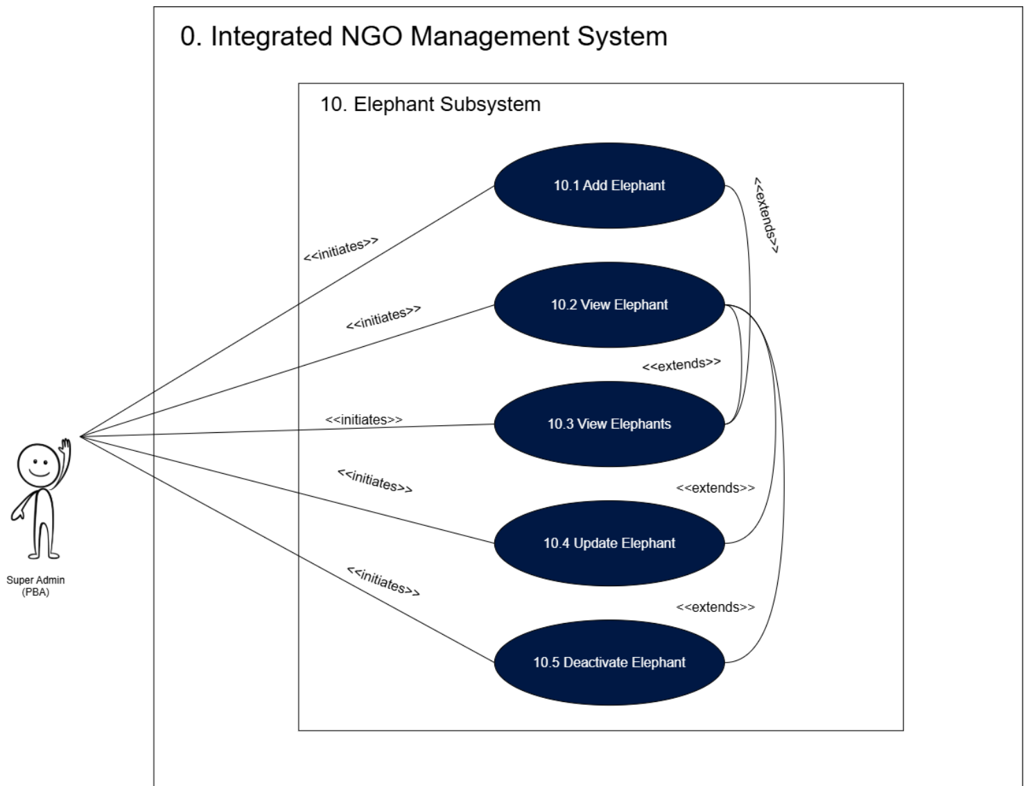
Figure 14: Elephant Subsystem Use Case Diagram
