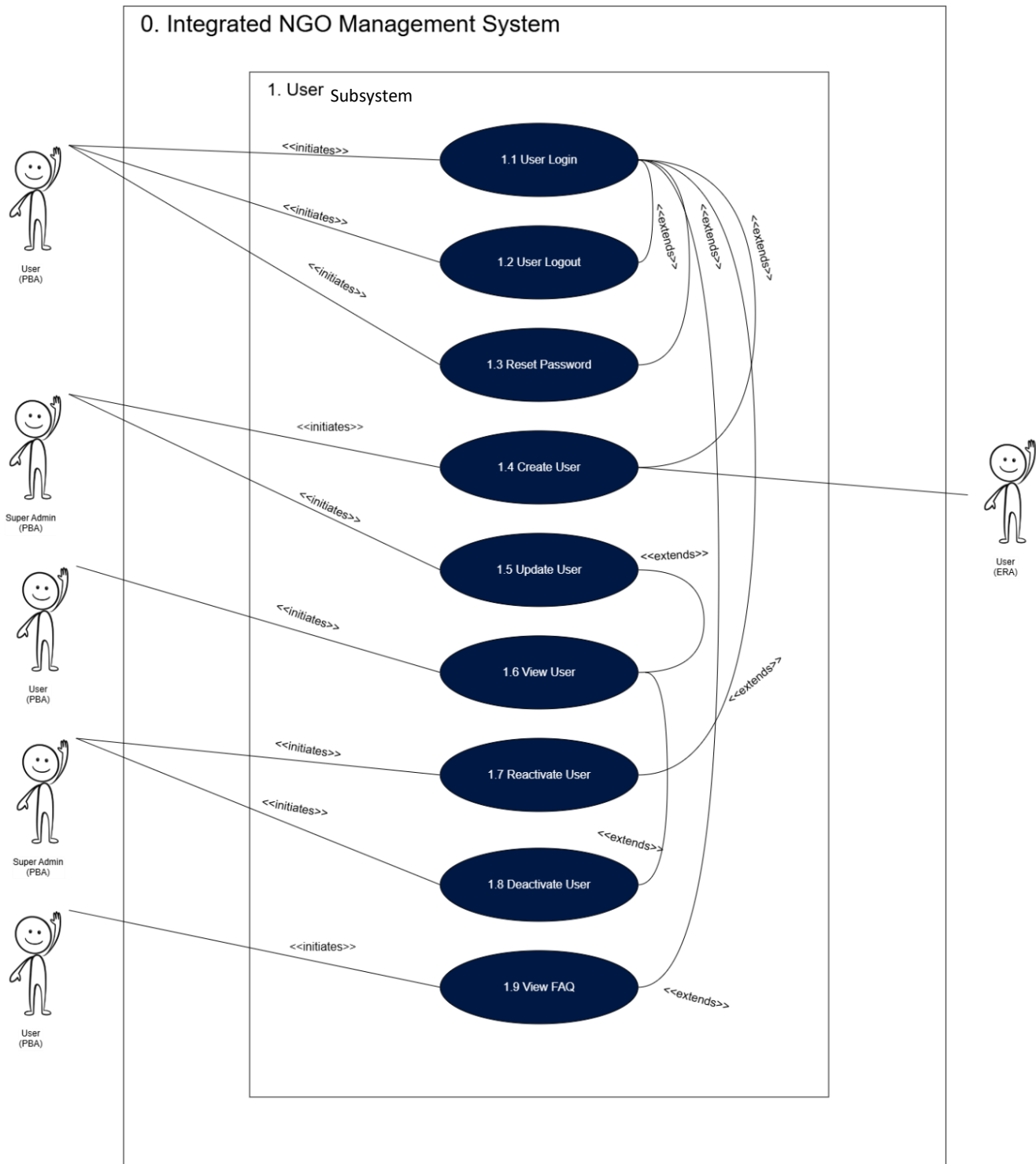
Figure 1: User Subsystem Use Case Diagram
