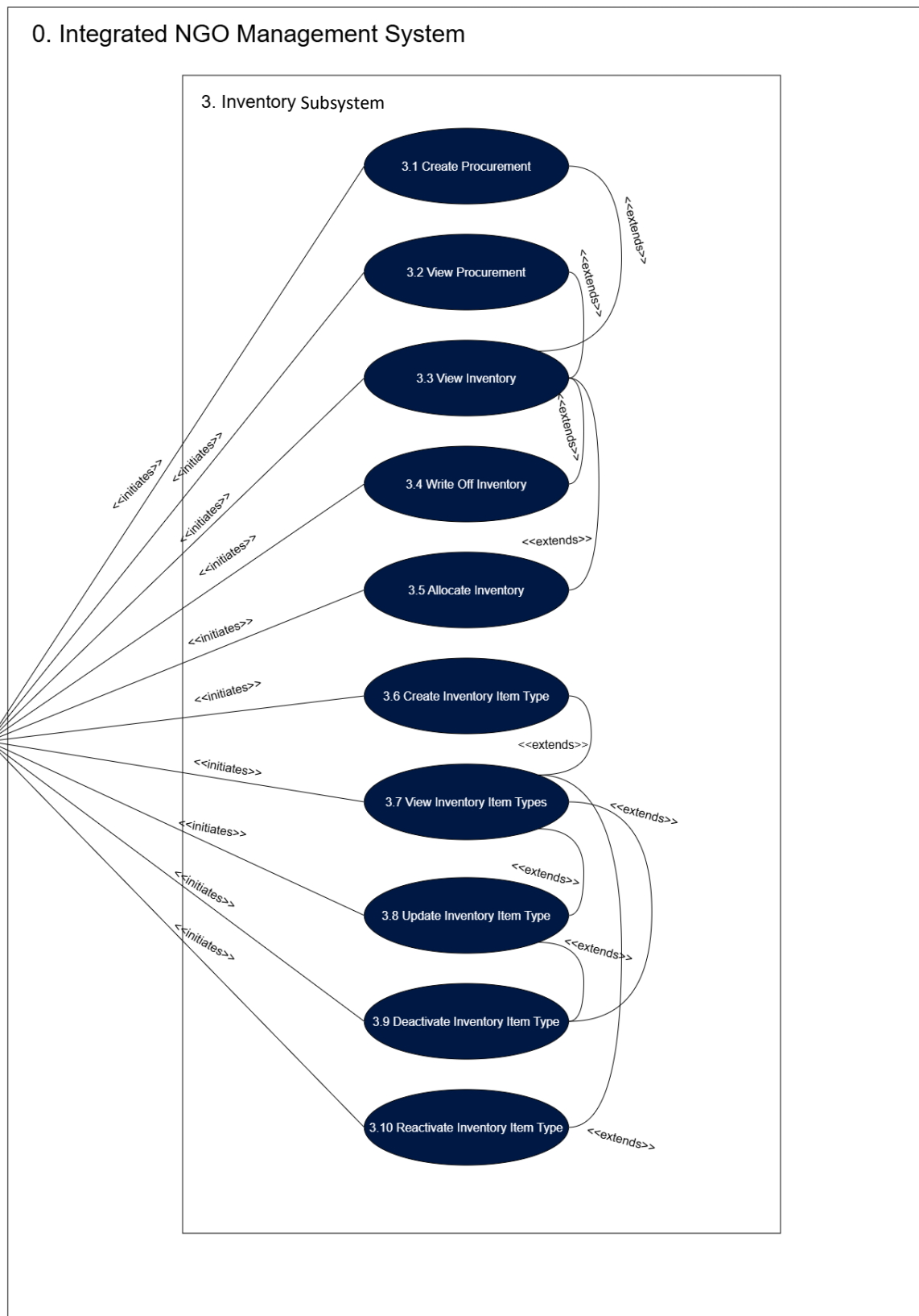
Figure 4: Inventory Subsystem Use Case Diagram
