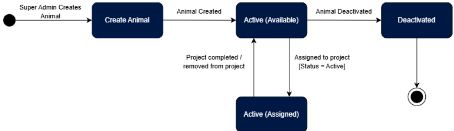
Figure 3: Animal State Diagram
