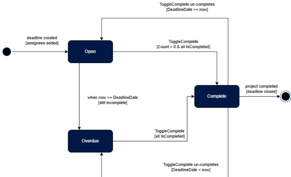
Figure 2: Deadline State Diagram
