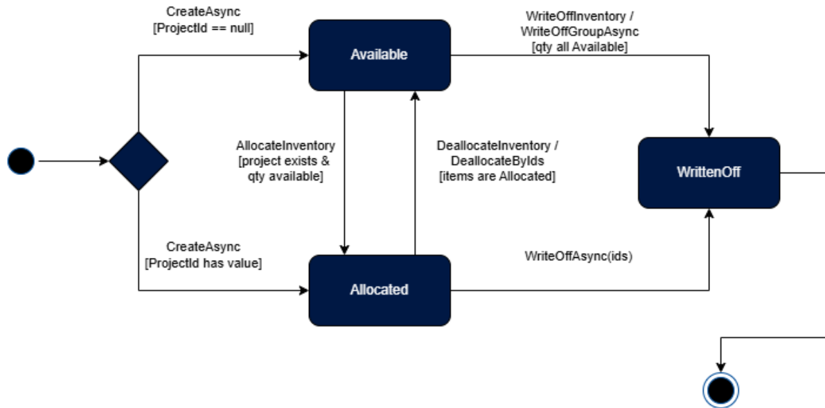
Figure 1: Inventory State Diagram
