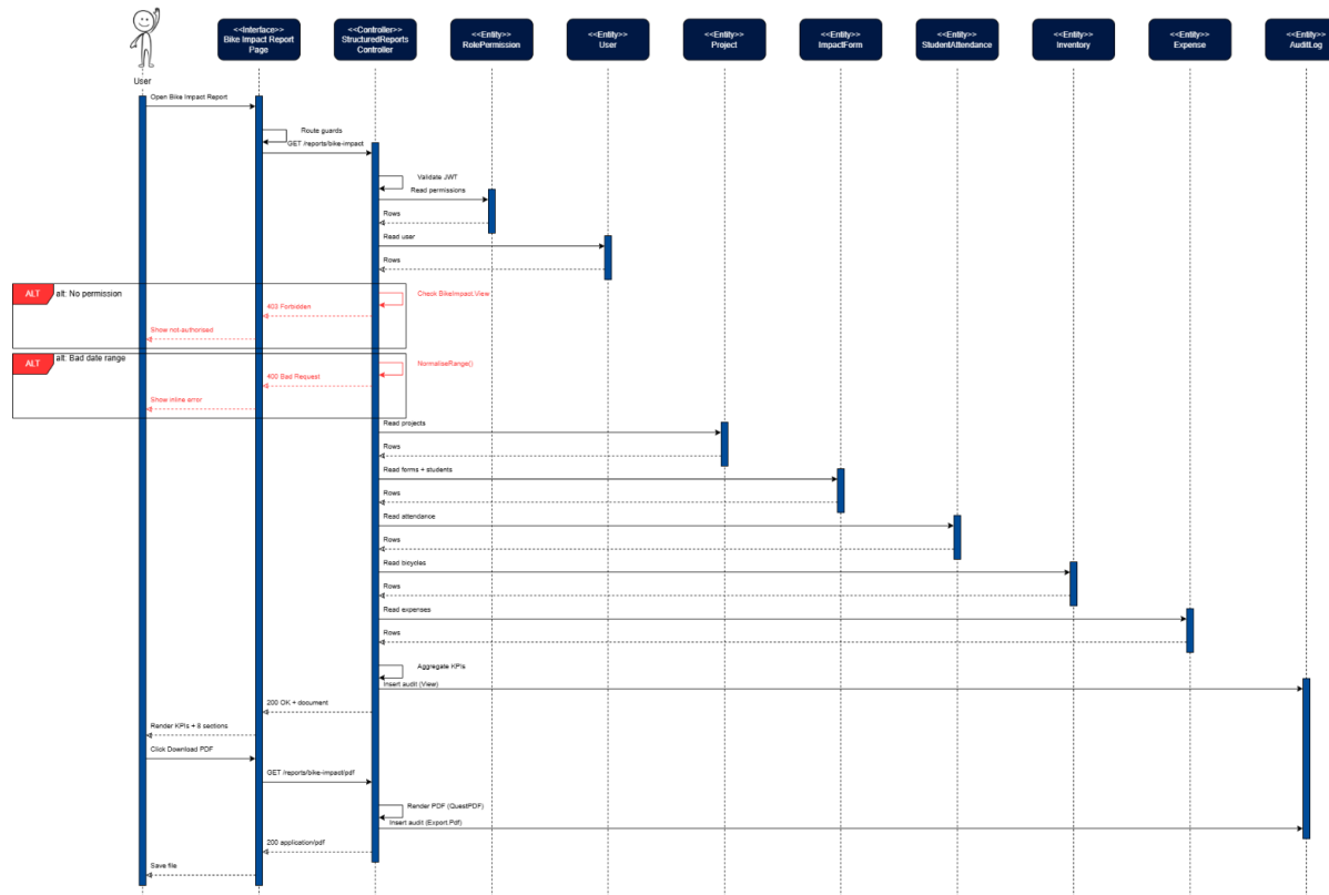
Figure 116: View Bike Impact Report Sequence Diagram
