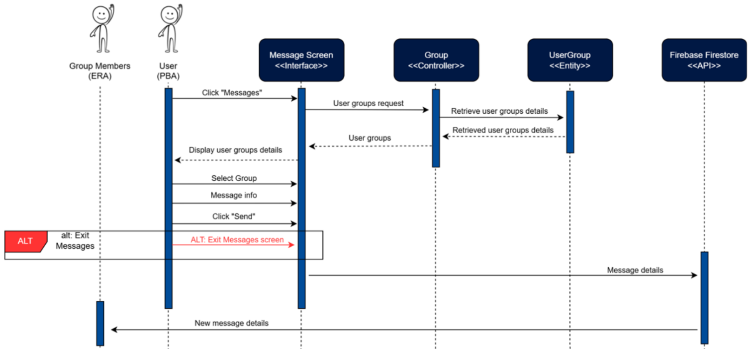
Figure 110: Create Message Sequence Diagram
