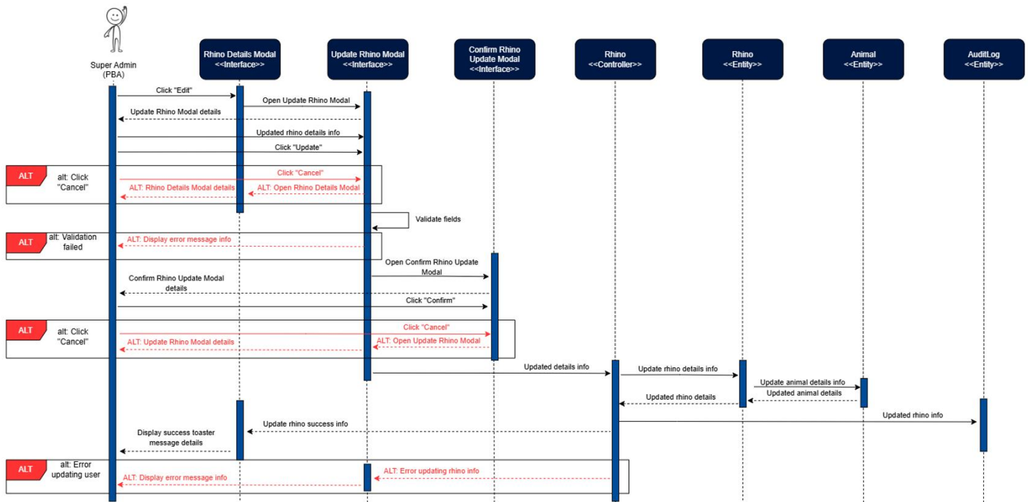
Figure 103: Update Rhino Sequence Diagram
