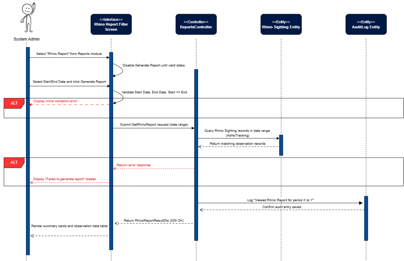
Figure 118: View Rhino Report Sequence Diagram
