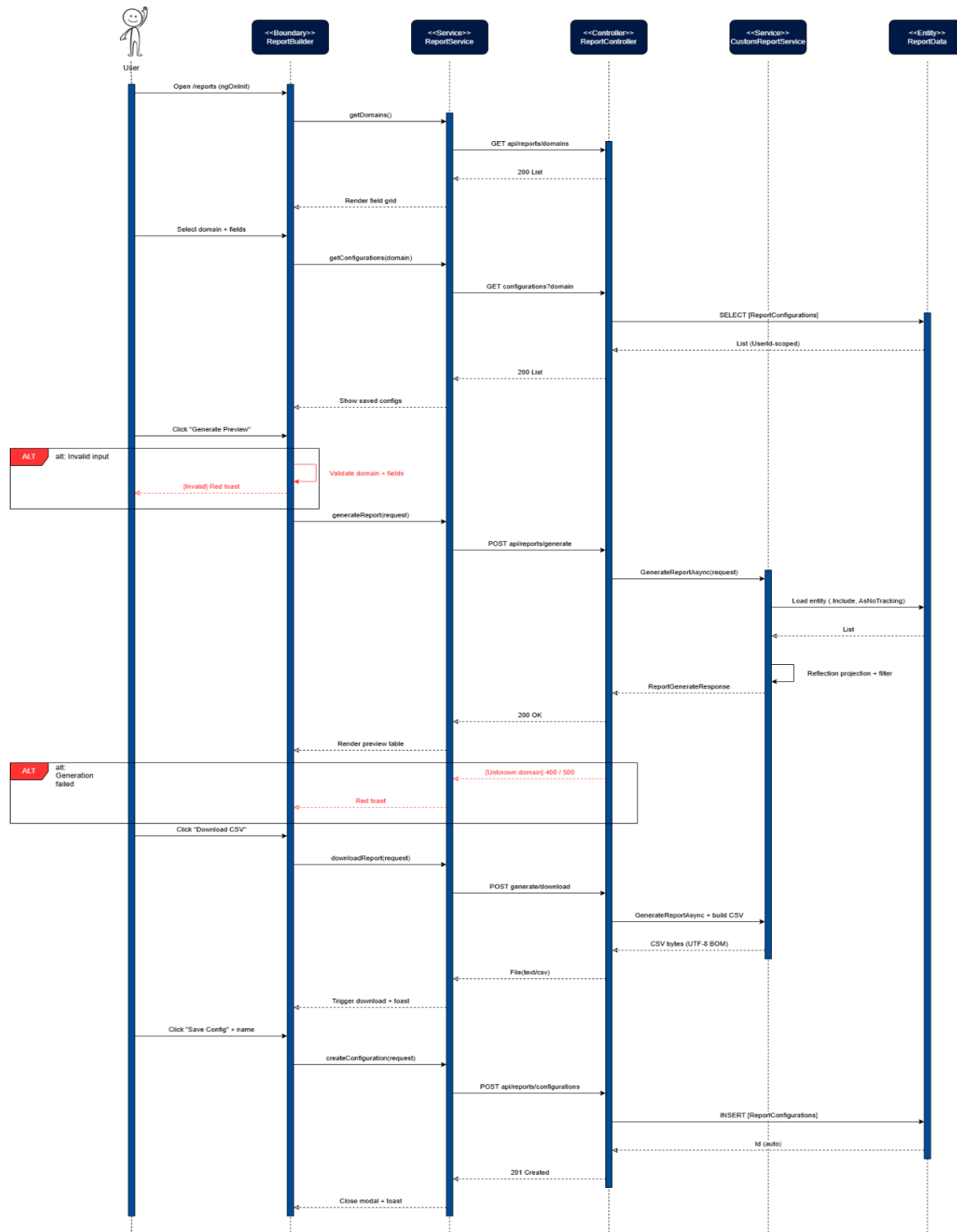
Figure 112: Generate Custom Report Sequence Diagram
