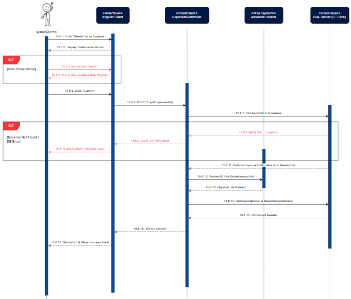
Figure 130: Remove Expense Sequence Diagram
