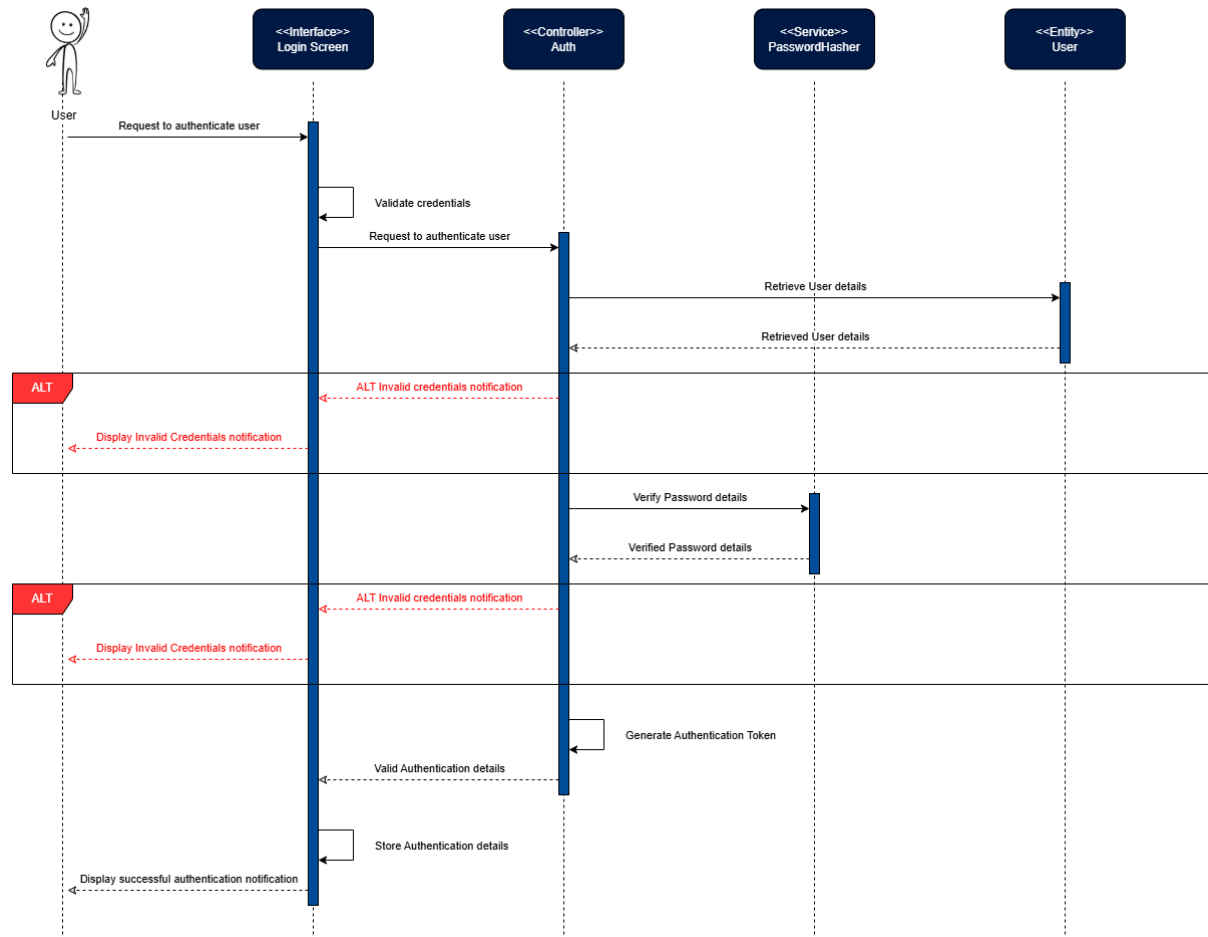
Figure 1: User Login Sequence Diagram
