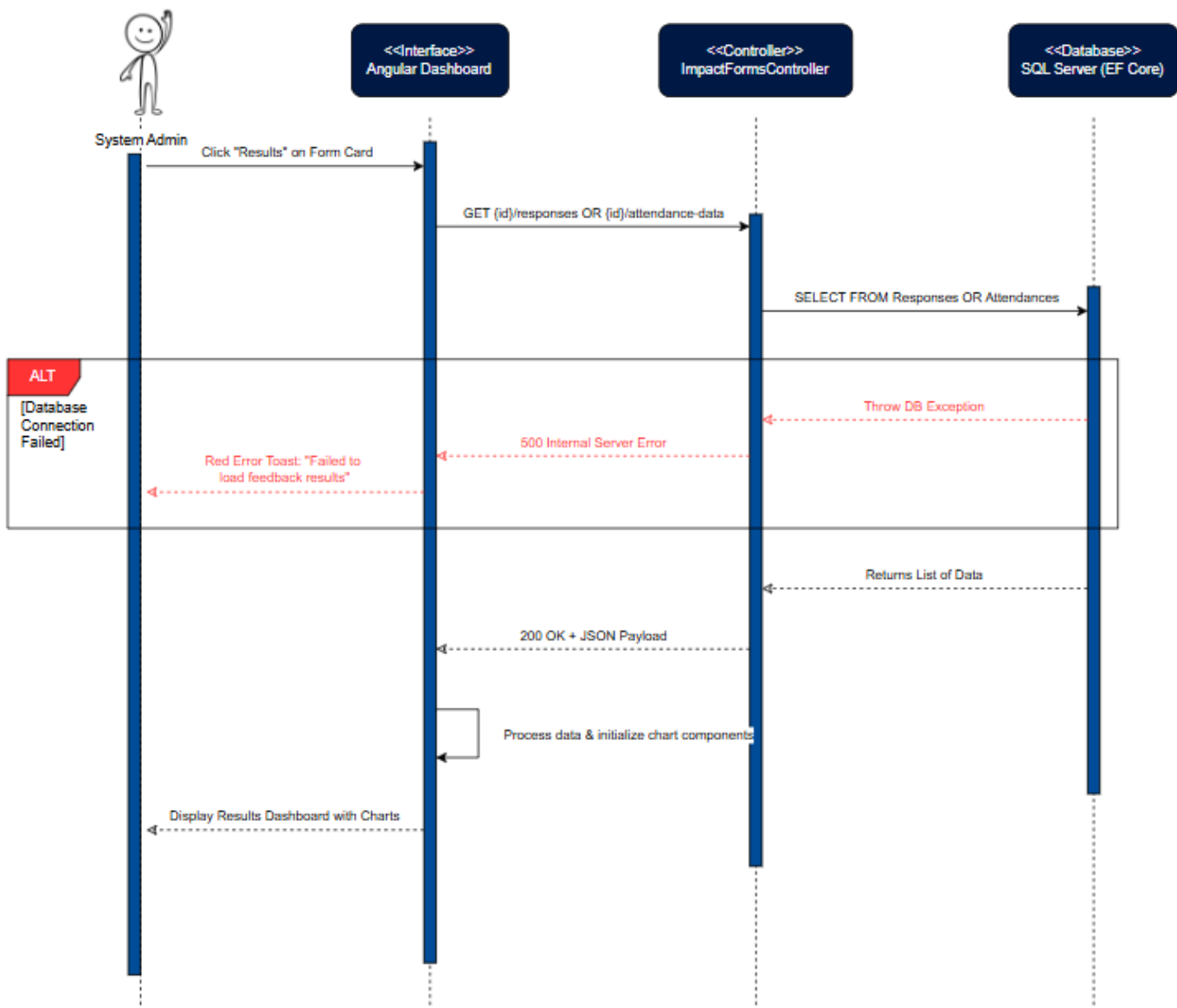
Figure 76: View Impact Feedback Sequence Diagram
