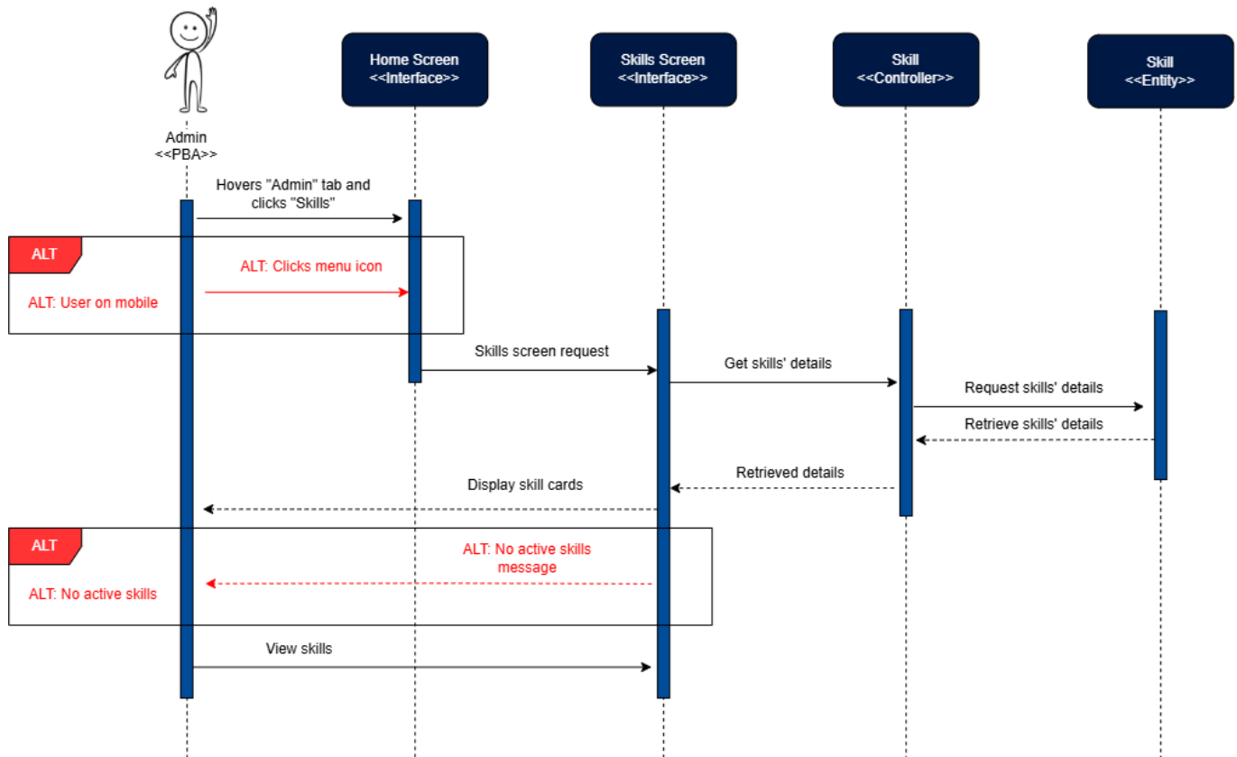
Figure 35: View Skills Sequence Diagram
