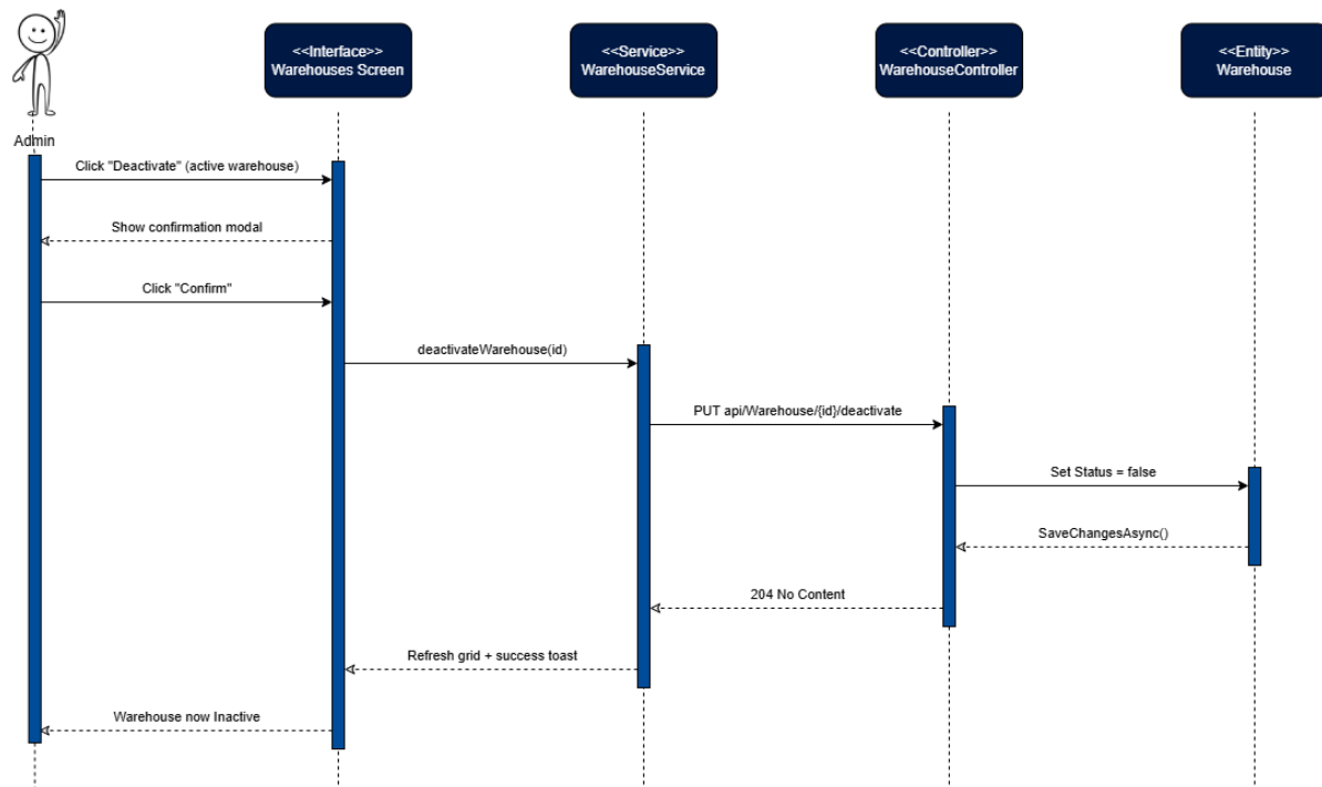
Figure 43: Deactivate Warehouse Sequence Diagram
