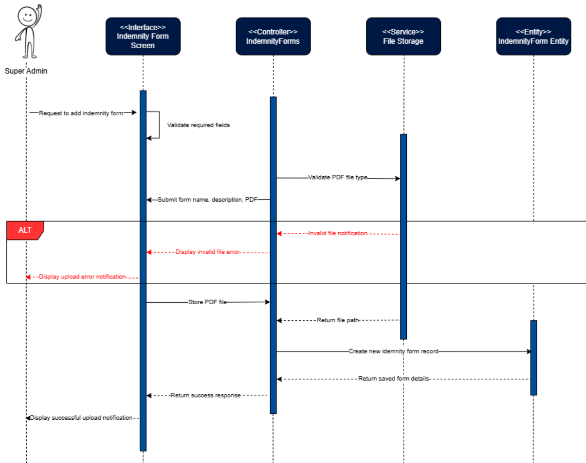
Figure 64: Add Indemnity Form Sequence Diagram
