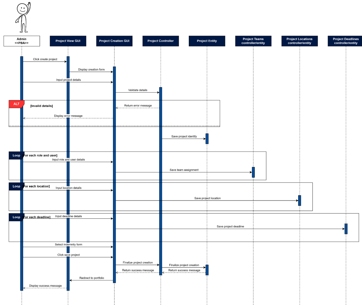
Figure 56: Create Project Sequence Diagram
