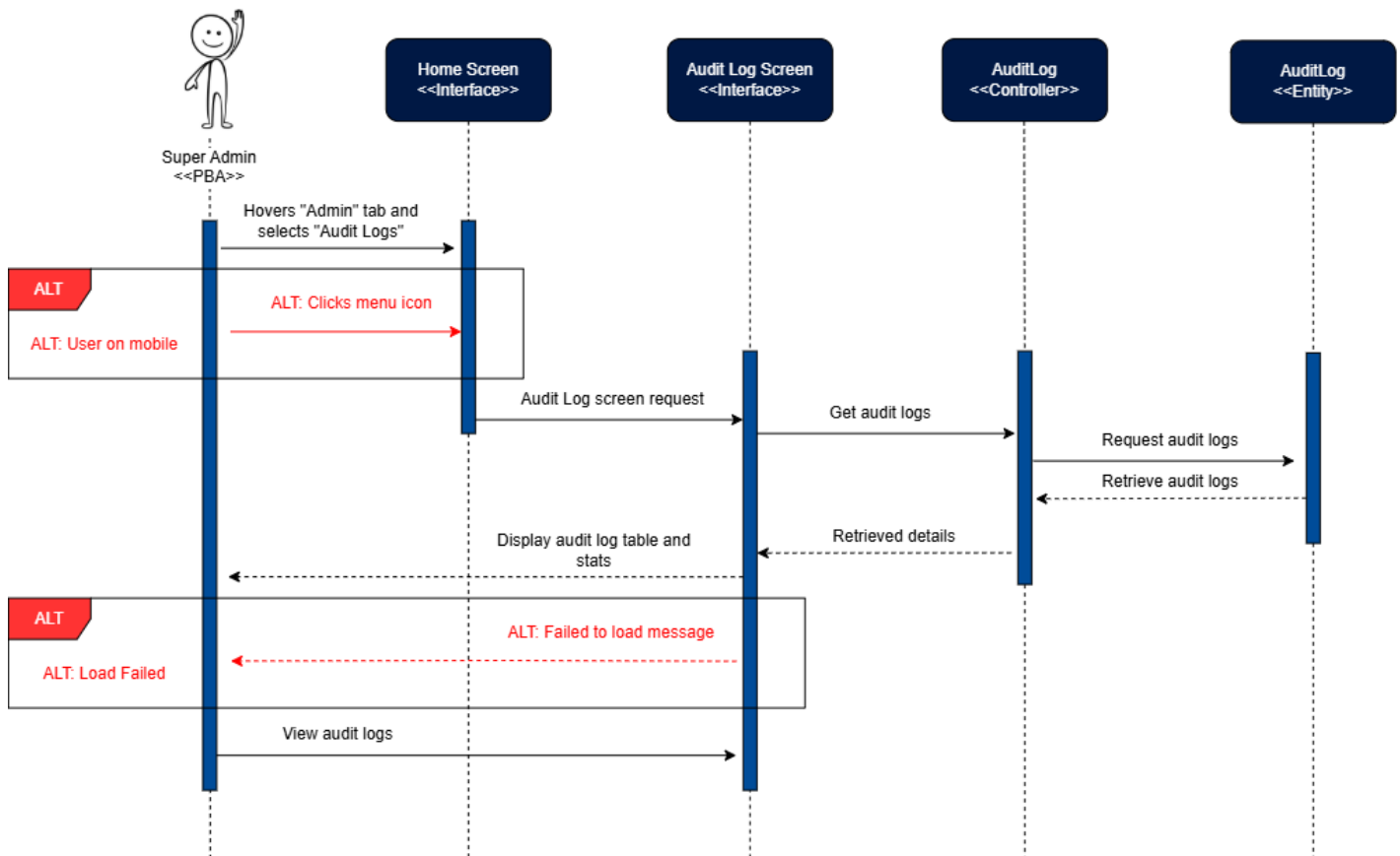
Figure 124: View Audit Log Sequence Diagram
