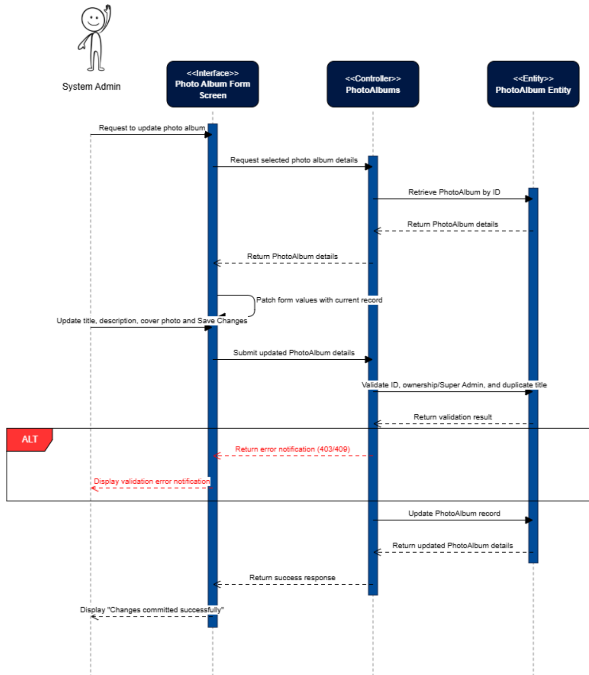
Figure 82: Update Photo Album Sequence Diagram
