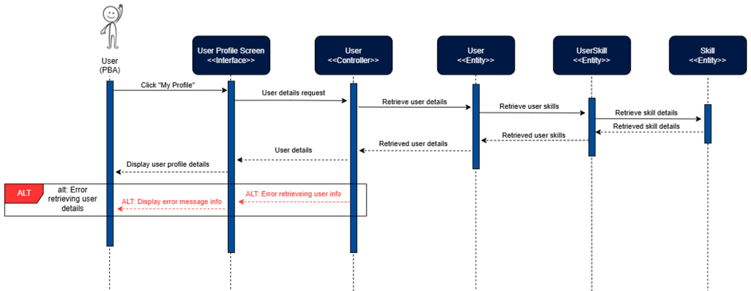
Figure 6: View User Sequence Diagram
