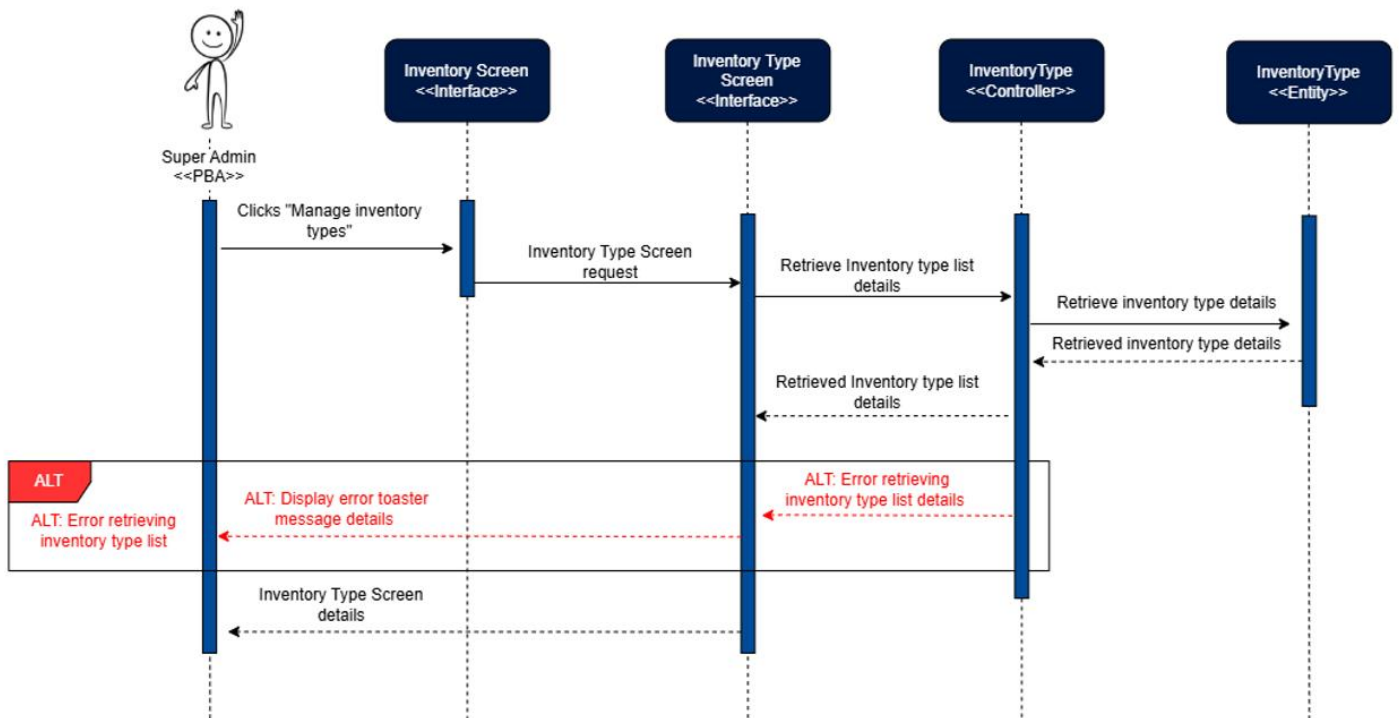
Figure 26: View Inventory Item Types Sequence Diagram
