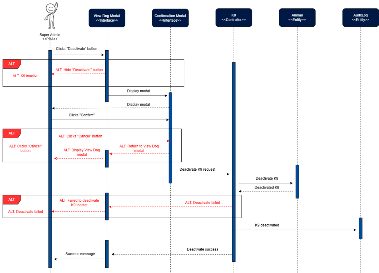
Figure 88: Deactivate Dog Sequence Diagram
