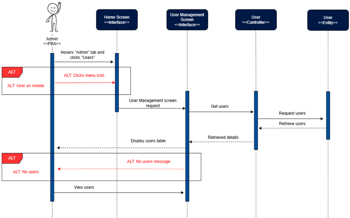
Figure 12: View User Profile Sequence Diagram
