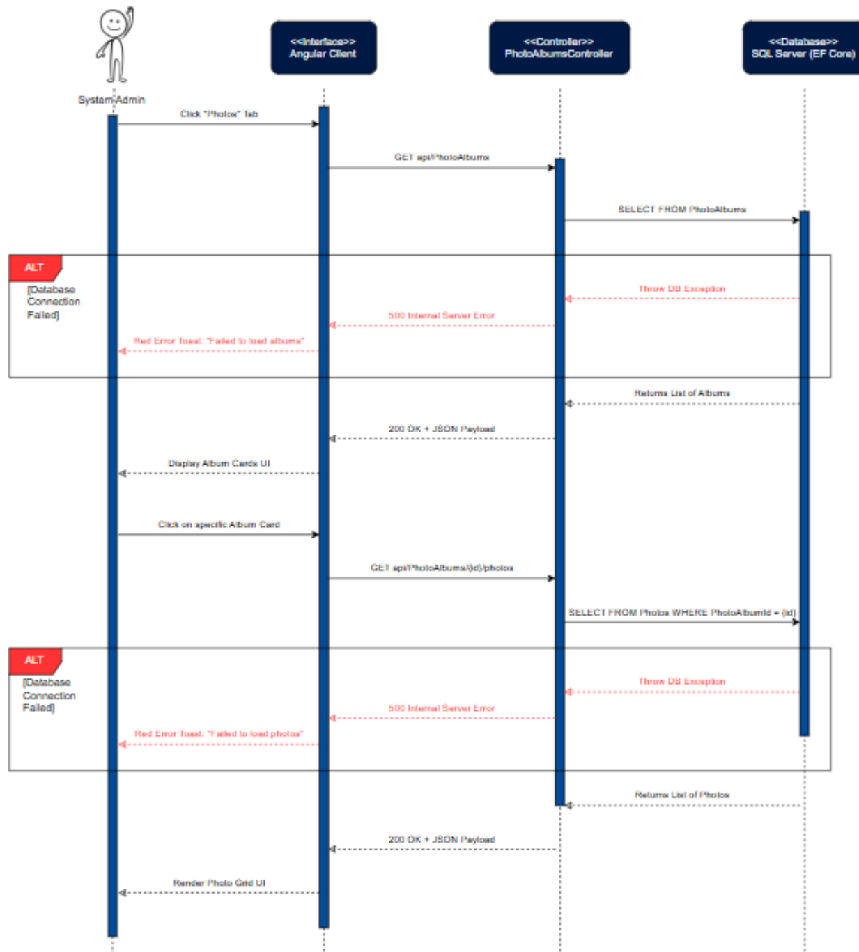
Figure 78: View Photo Sequence Diagram
