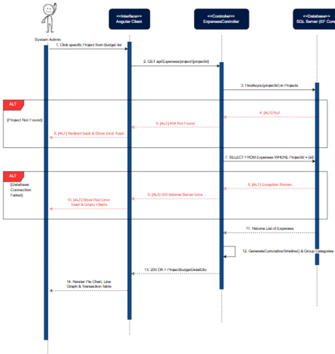
Figure 125: View Project Budget Sequence Diagram
