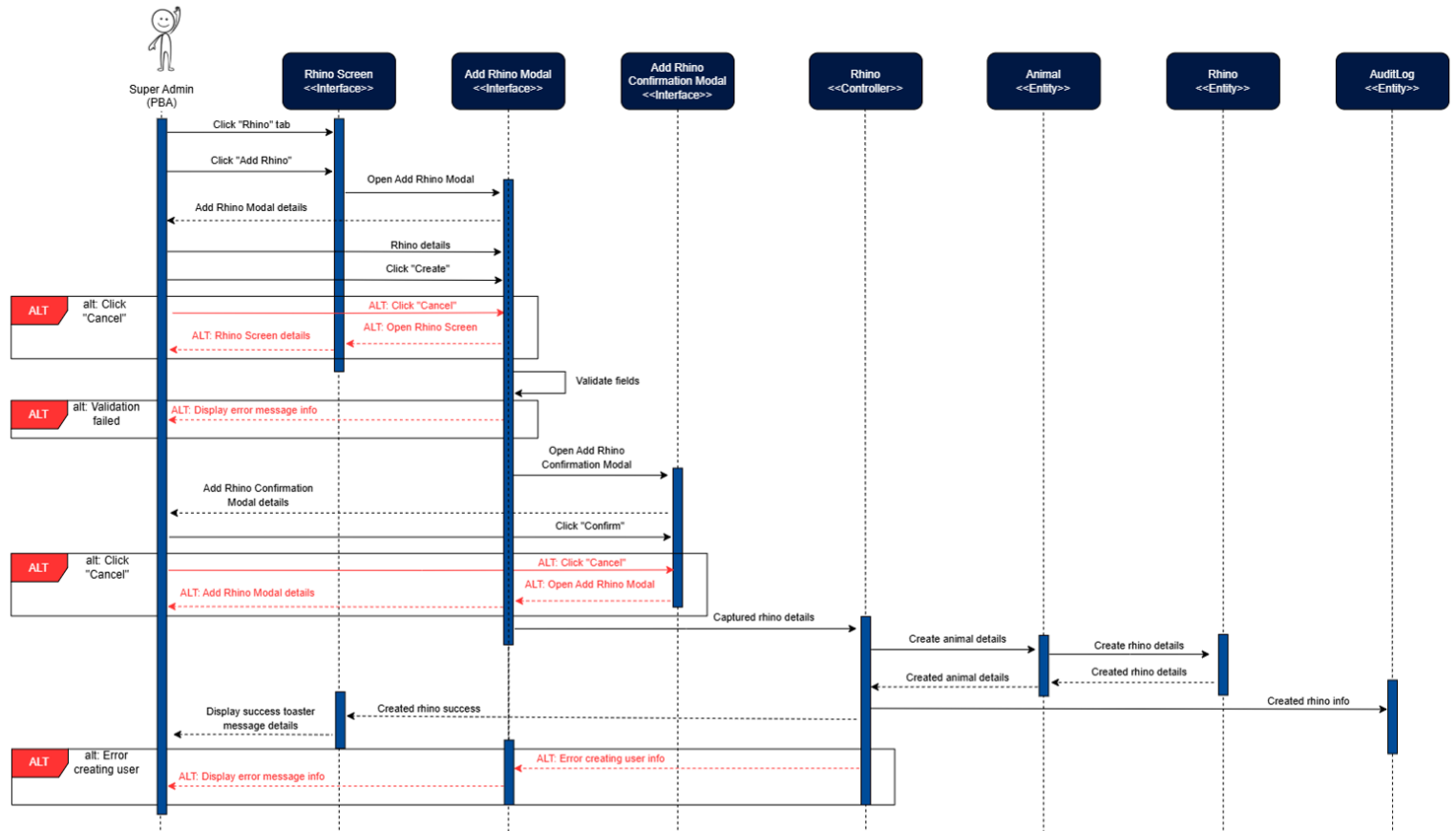
Figure 100: Add Rhino Sequence Diagram
