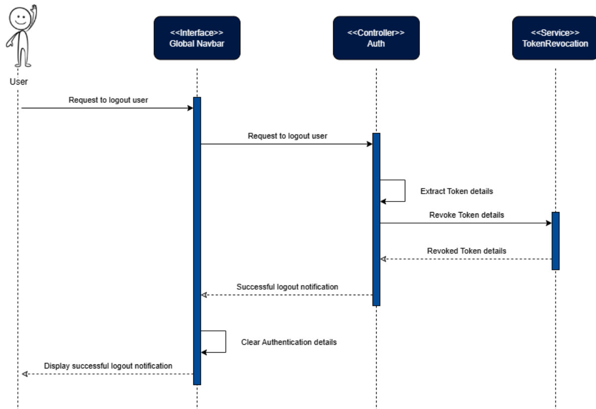
Figure 2: User Logout Sequence Diagram
