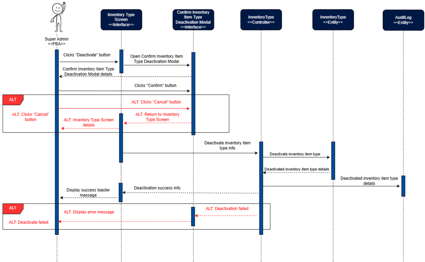
Figure 28: Deactivate Inventory Item Type Sequence Diagram
