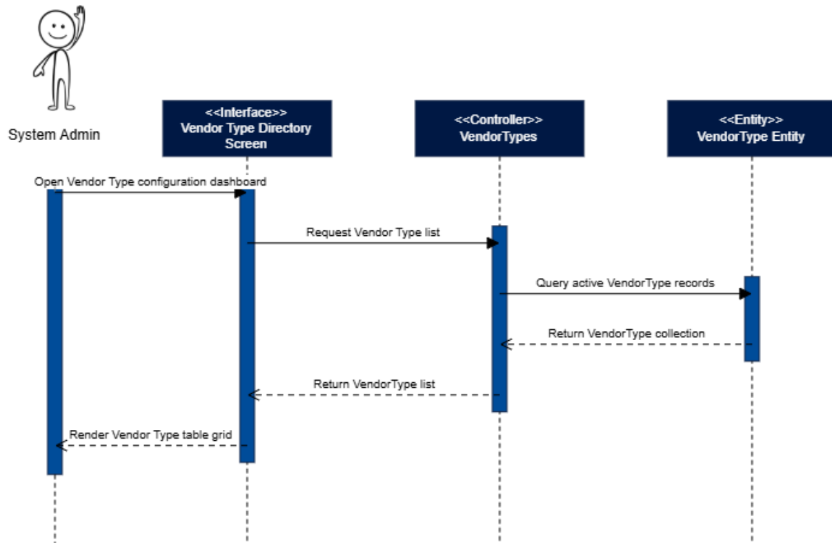
Figure 53: View Vendor Types Sequence Diagram
