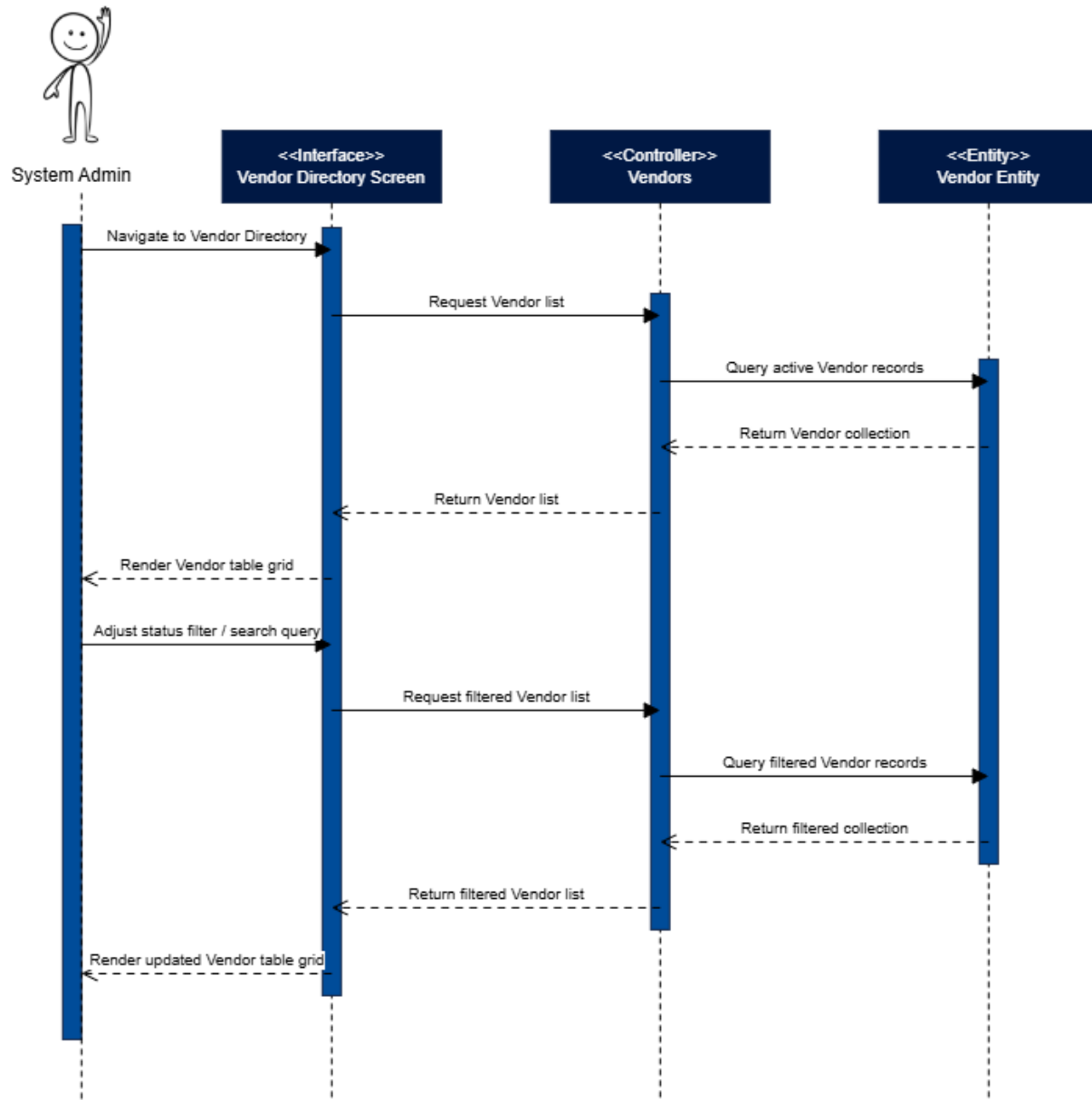
Figure 47: View Vendors Sequence Diagram
