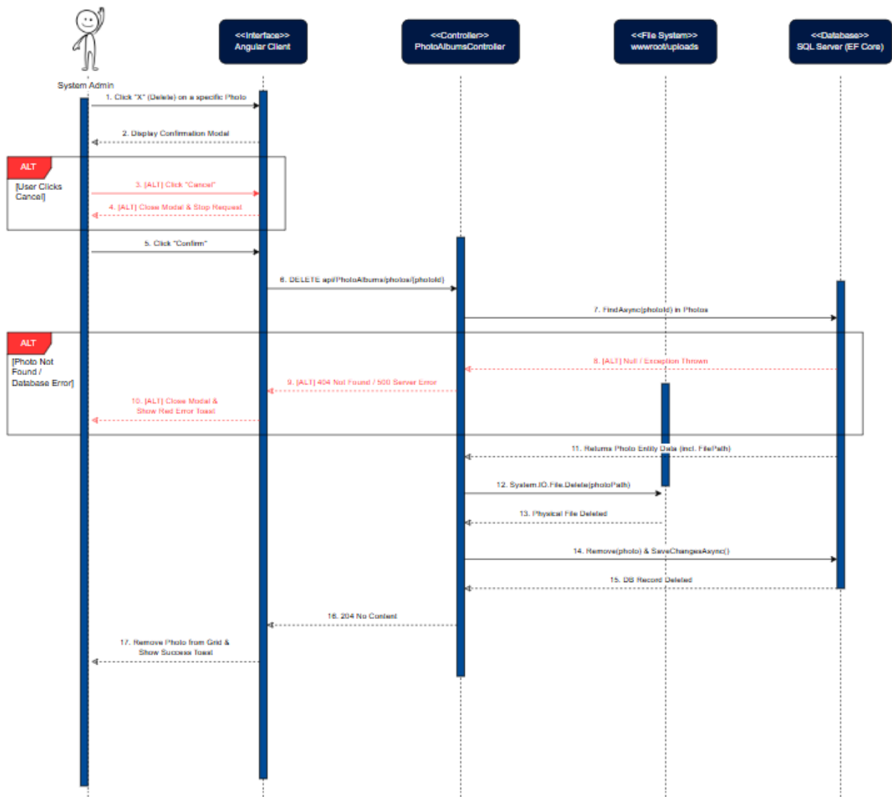
Figure 79: Remove Photo Sequence Diagram
