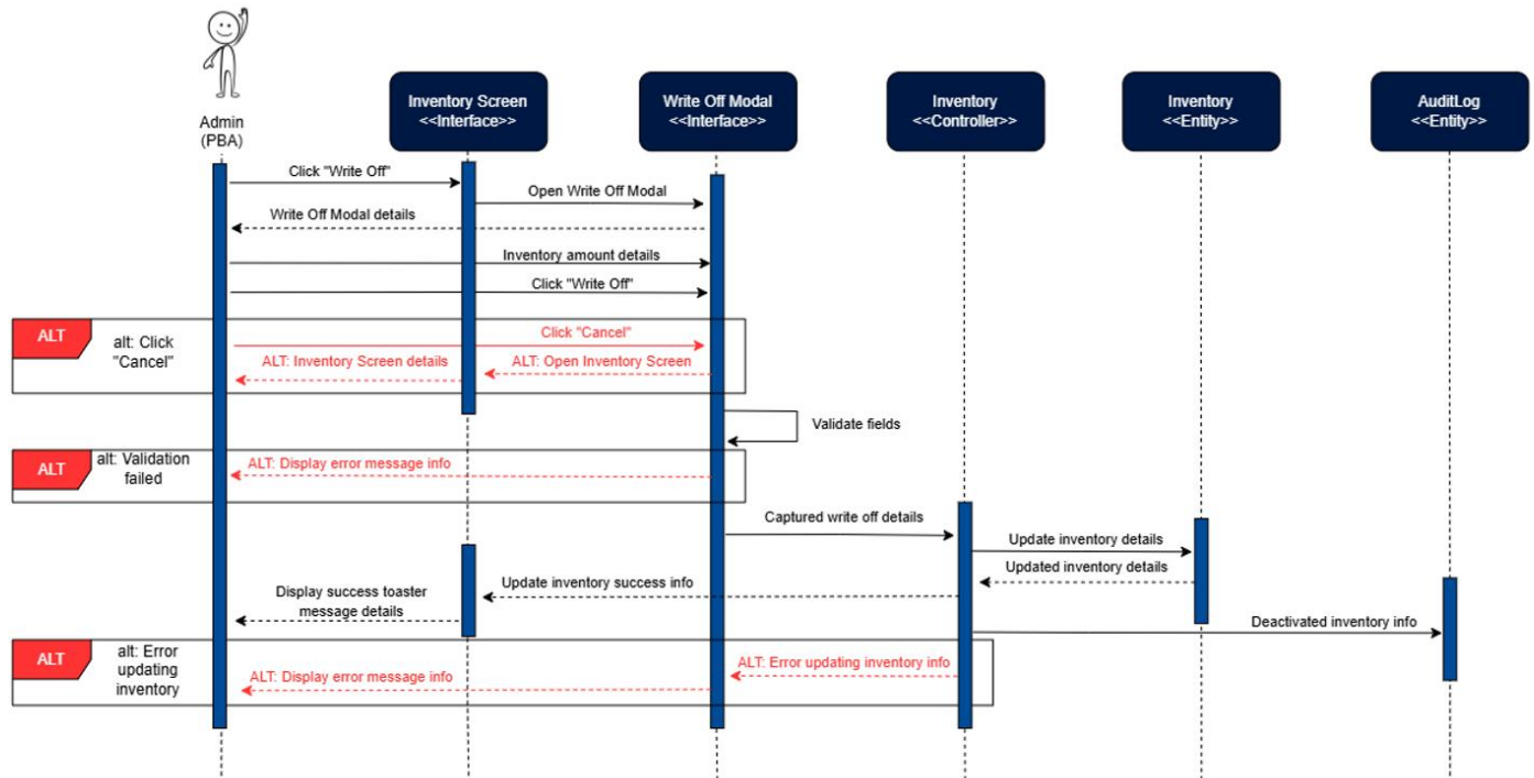
Figure 22: Write Off Inventory Sequence Diagram
