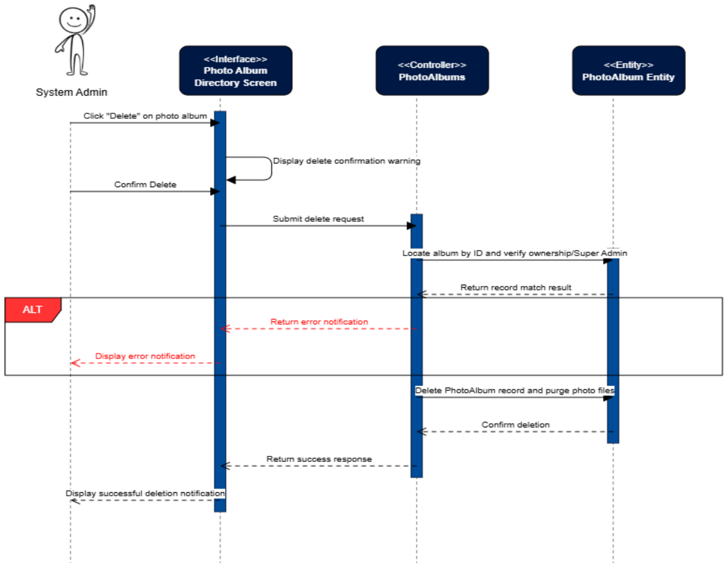
Figure 83: Remove Photo Album Sequence Diagram
