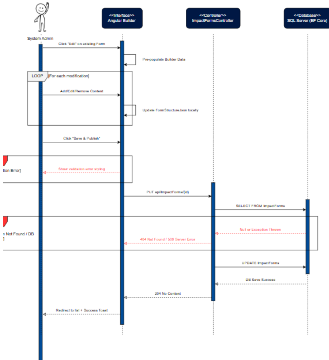
Figure 73: Update Impact Feedback Form Sequence Diagram
