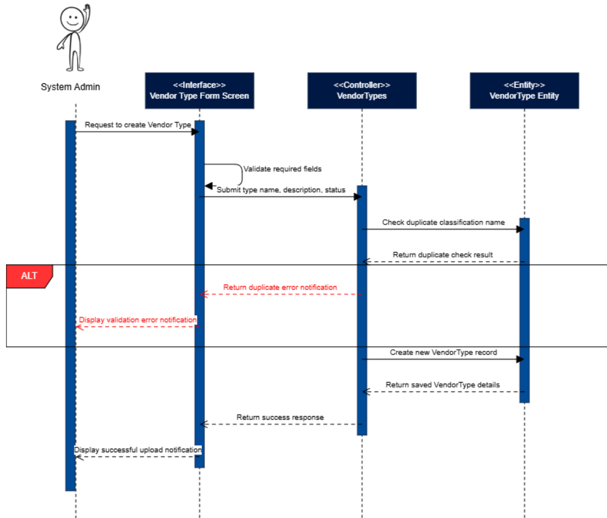
Figure 51: Create Vendor Type Sequence Diagram
