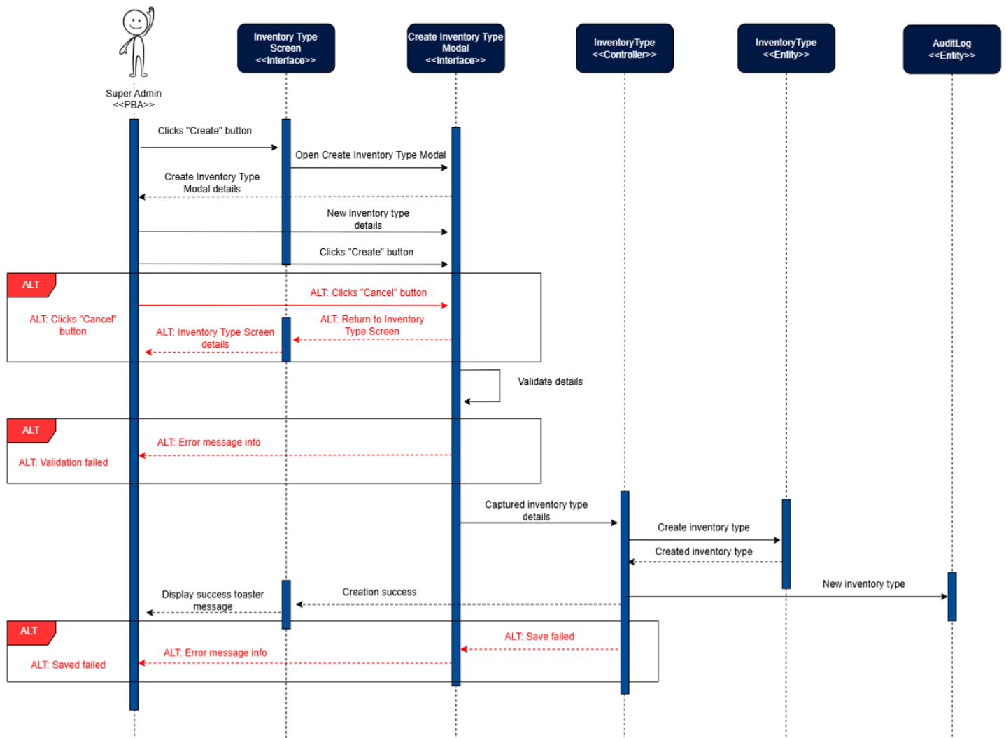
Figure 24: Create Inventory Item Type Sequence Diagram
