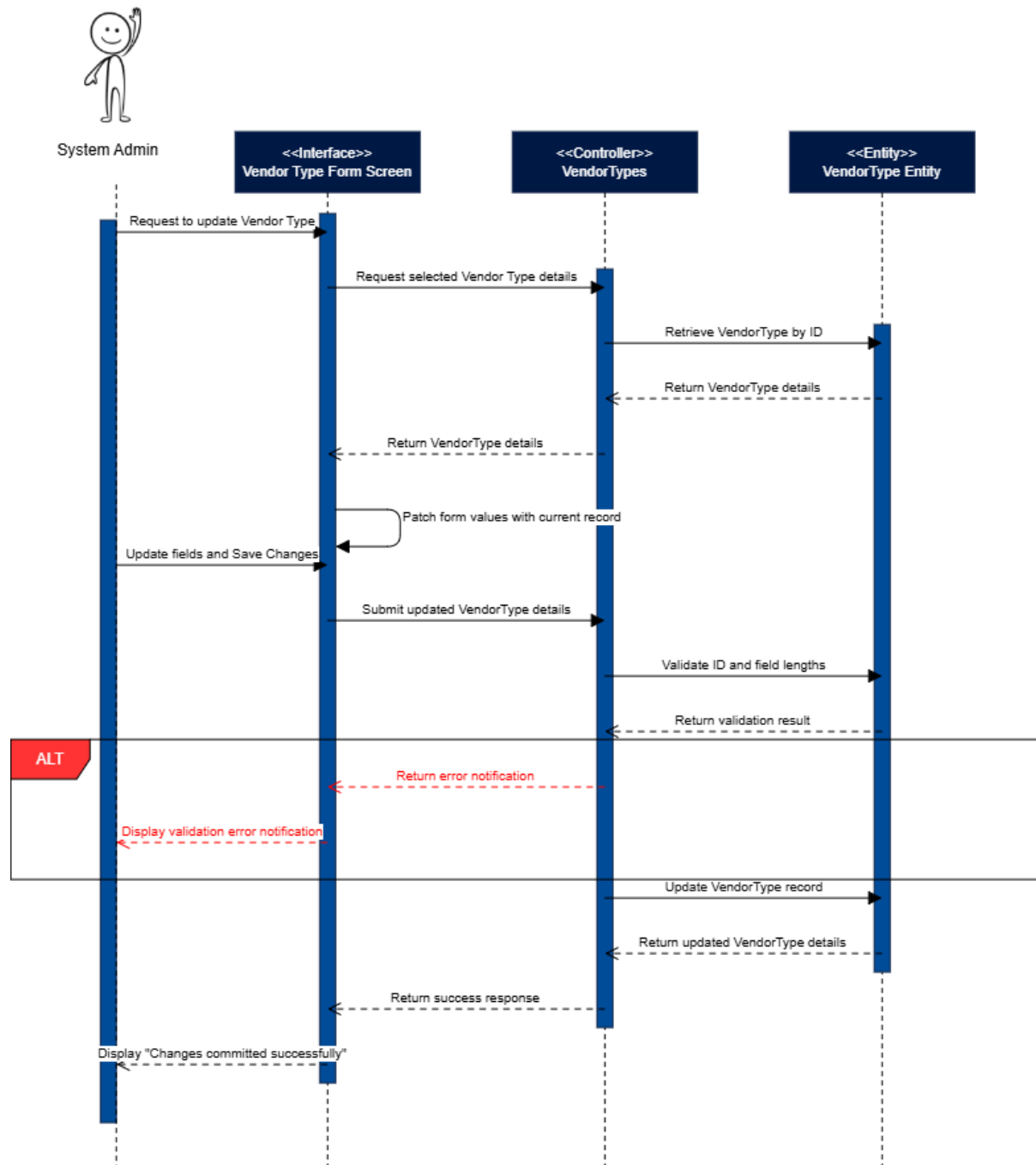
Figure 52: Update Vendor Type Sequence Diagram
