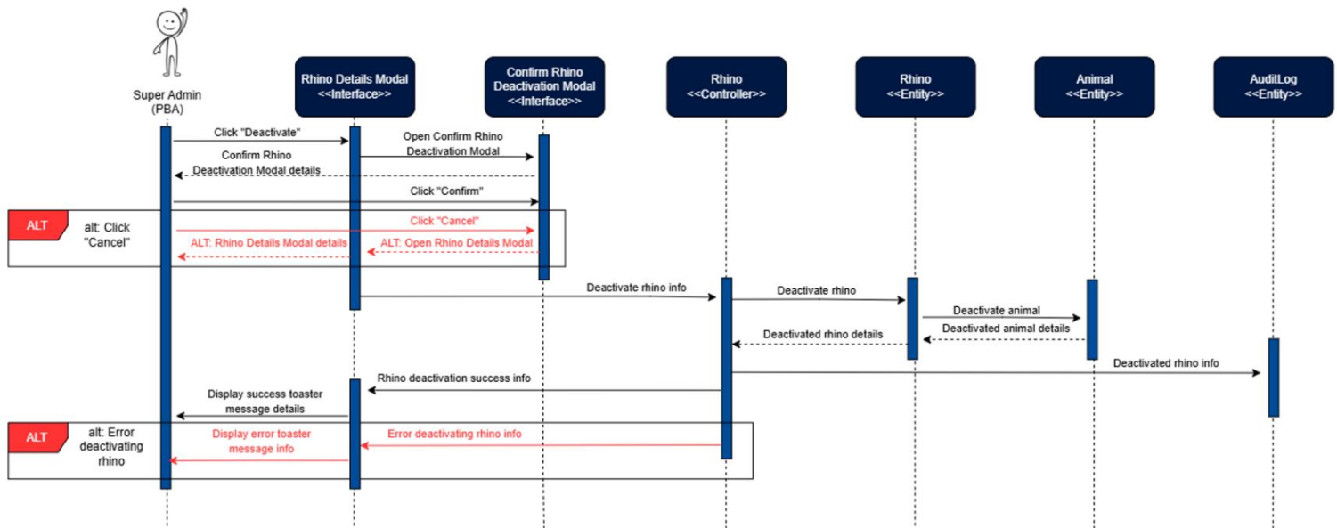
Figure 104: Deactivate Rhino Sequence Diagram
