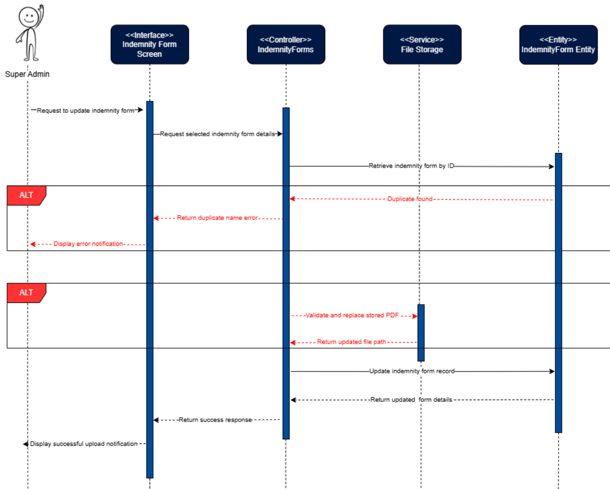
Figure 65: Update Indemnity Form Sequence Diagram
