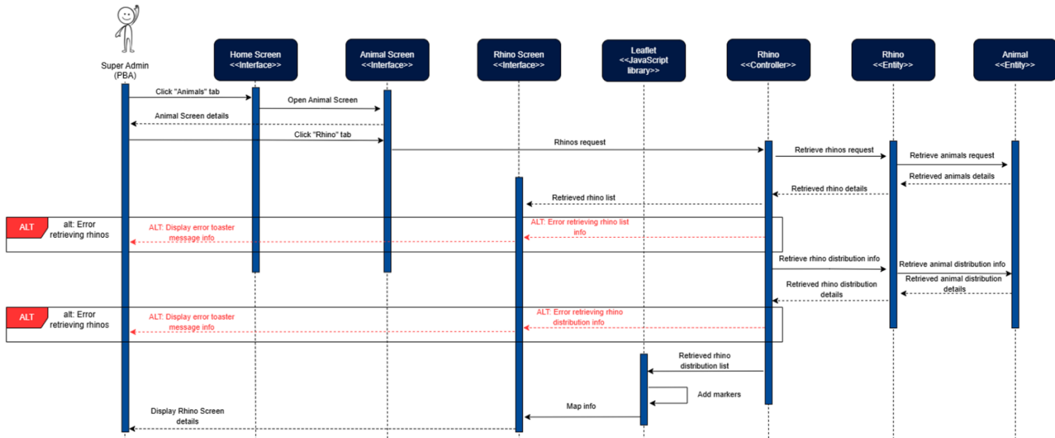
Figure 102: View Rhinos Sequence Diagram
