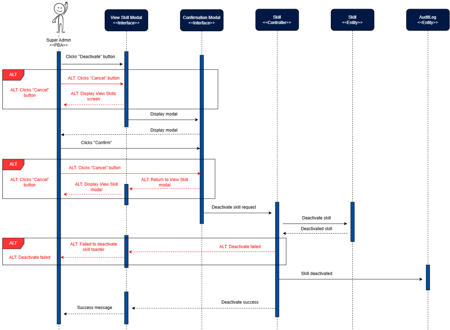
Figure 38: Deactivate Skill Sequence Diagram
