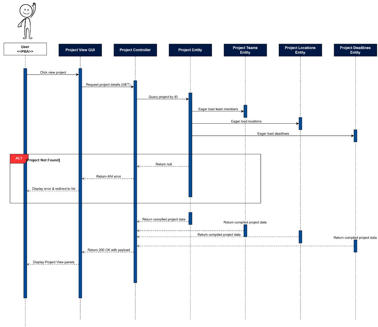
Figure 57: View Project Sequence Diagram
