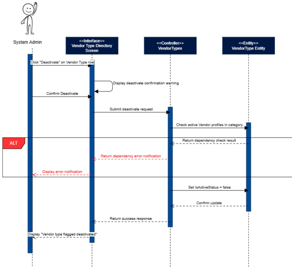
Figure 55: Deactivate Vendor Type Sequence Diagram
