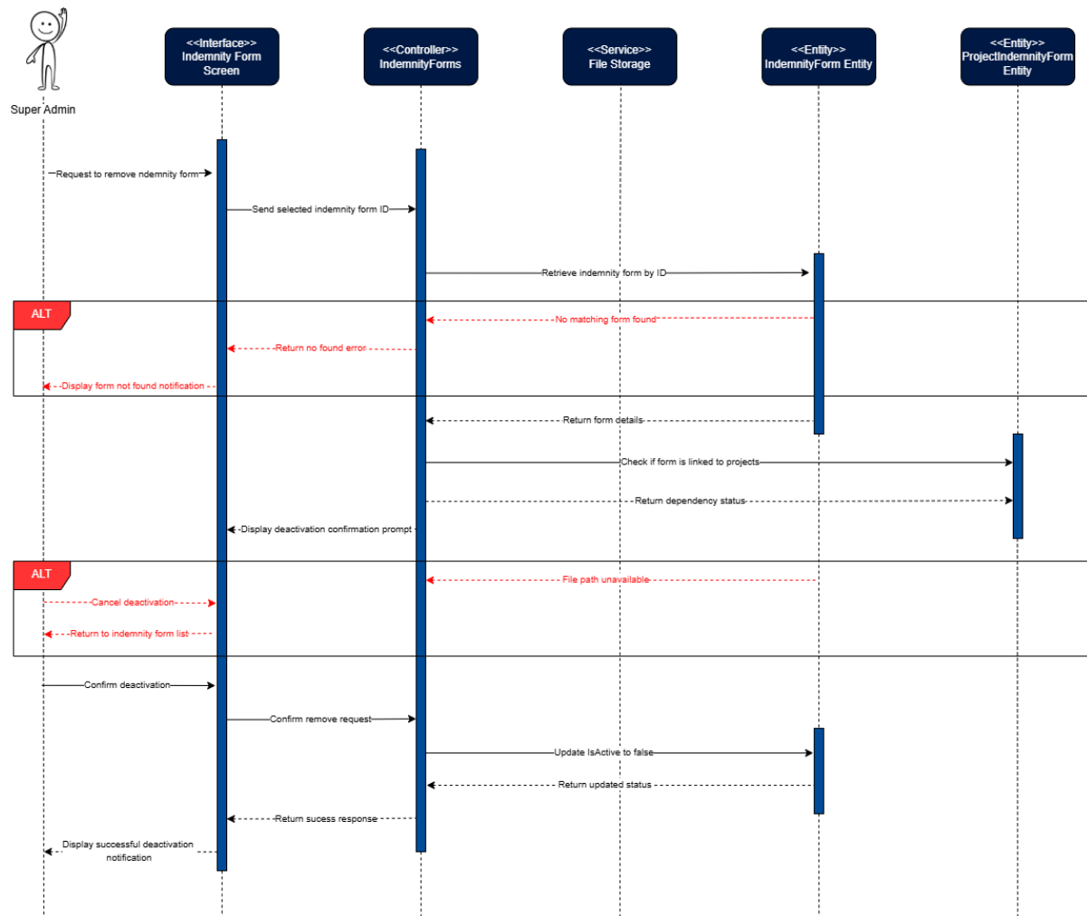
Figure 67: Remove Indemnity Form Sequence Diagram
