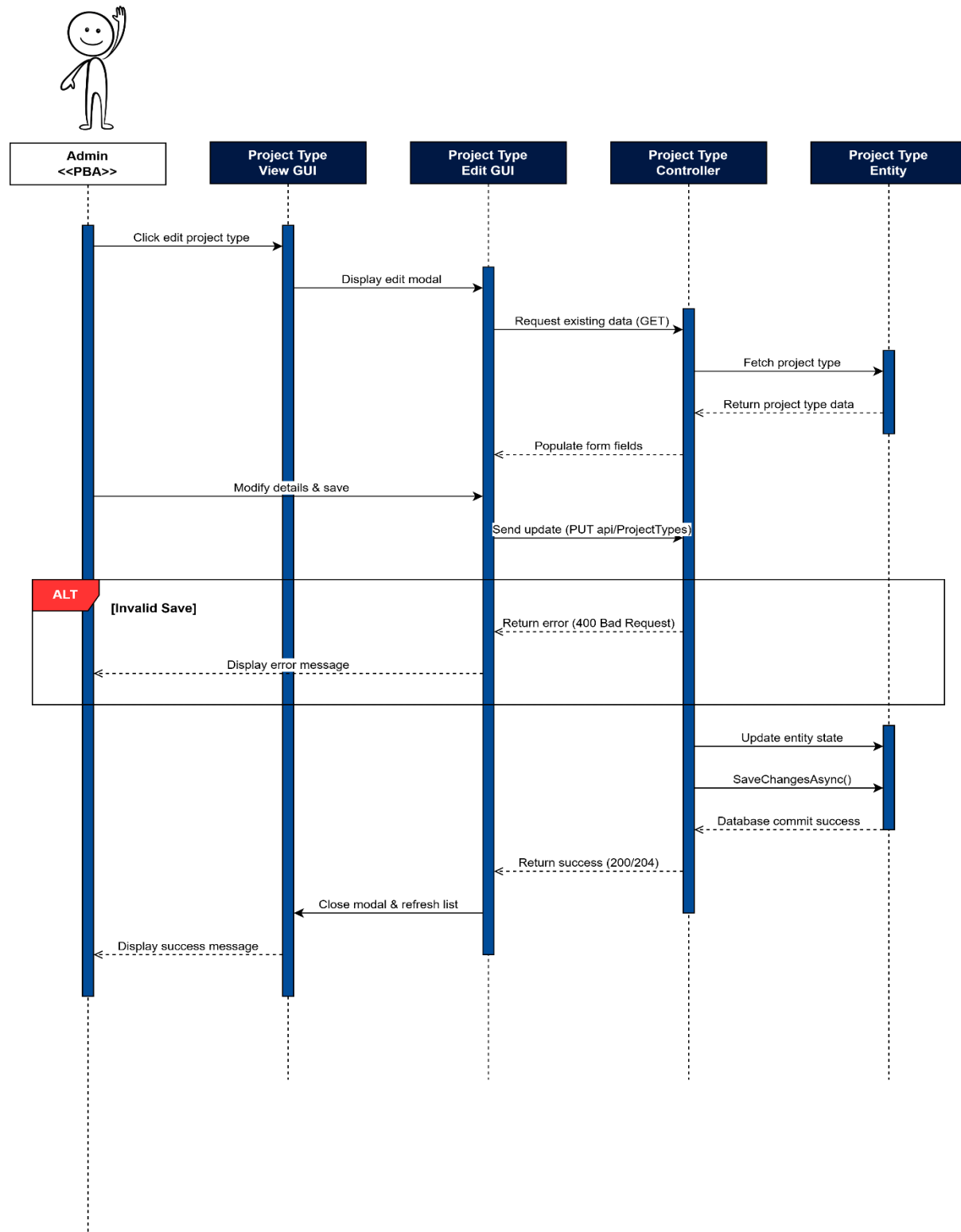
Figure 62: Update Project Type Sequence Diagram
