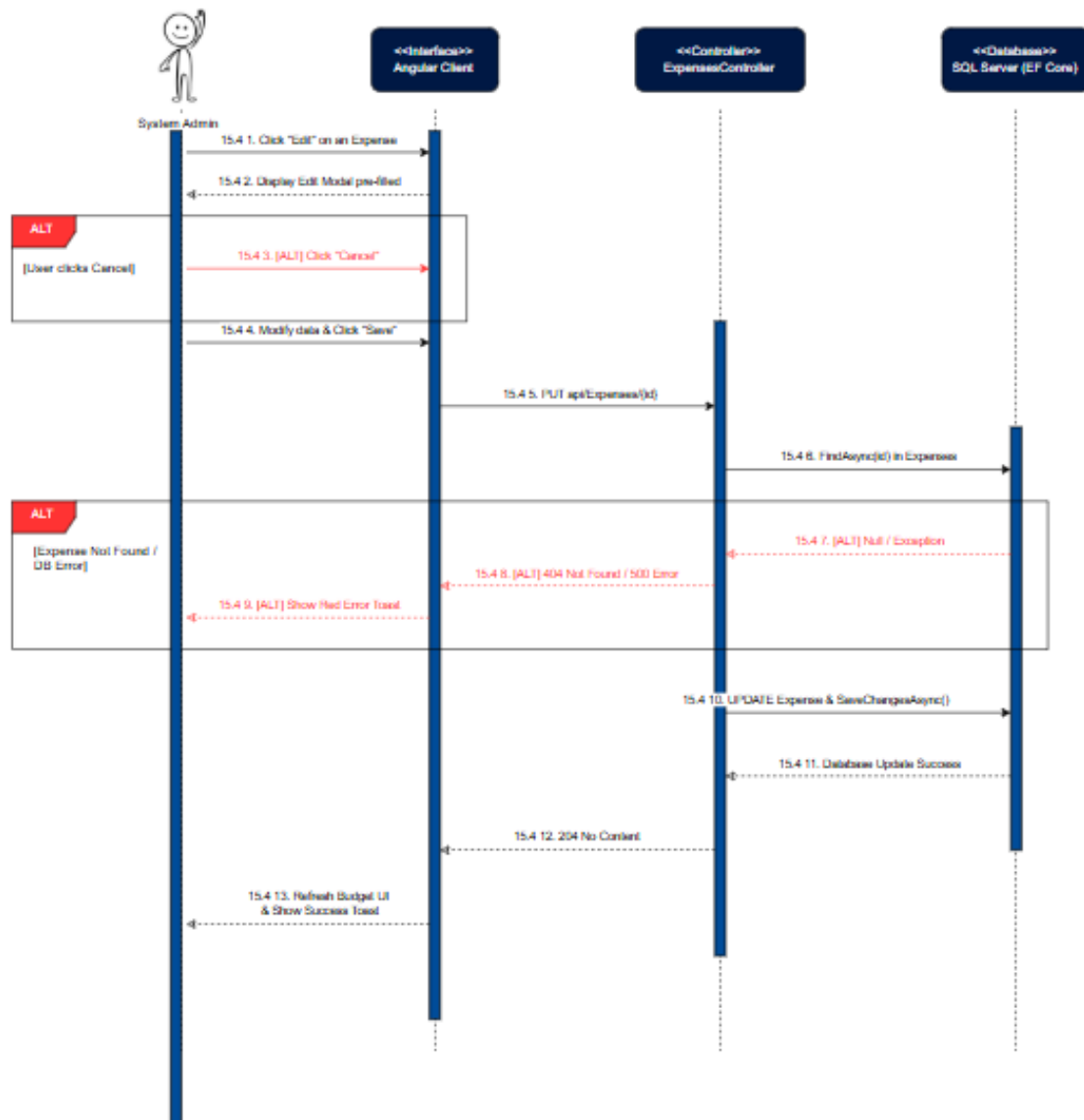
Figure 128: Update An Expense Sequence Diagram
