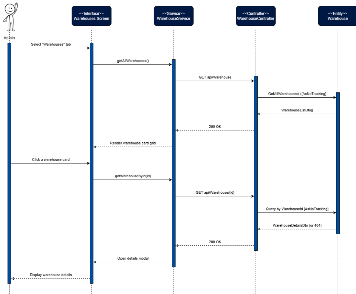
Figure 40: View Warehouse Sequence Diagram
