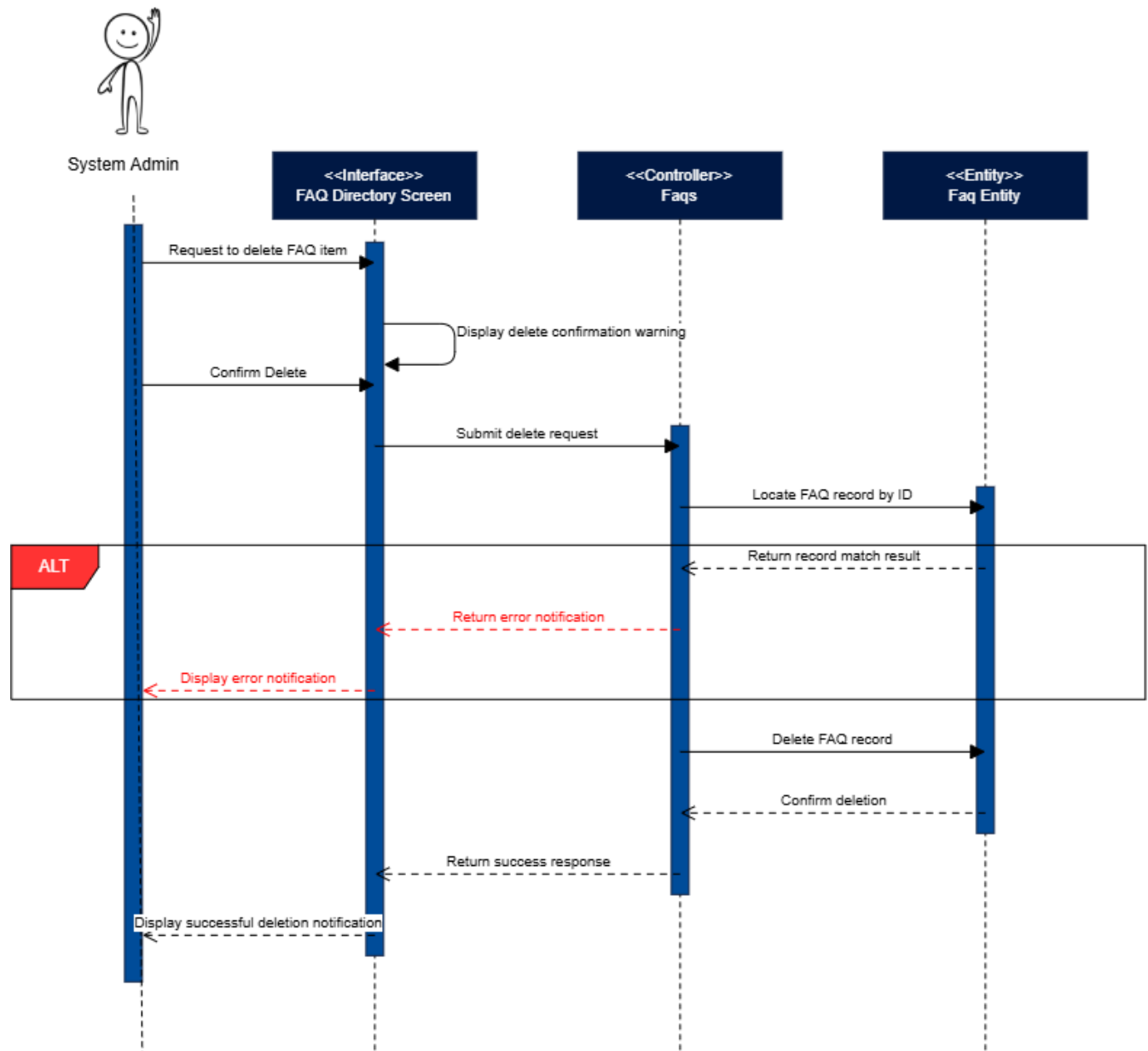
Figure 16: Remove FAQ Sequence Diagram
