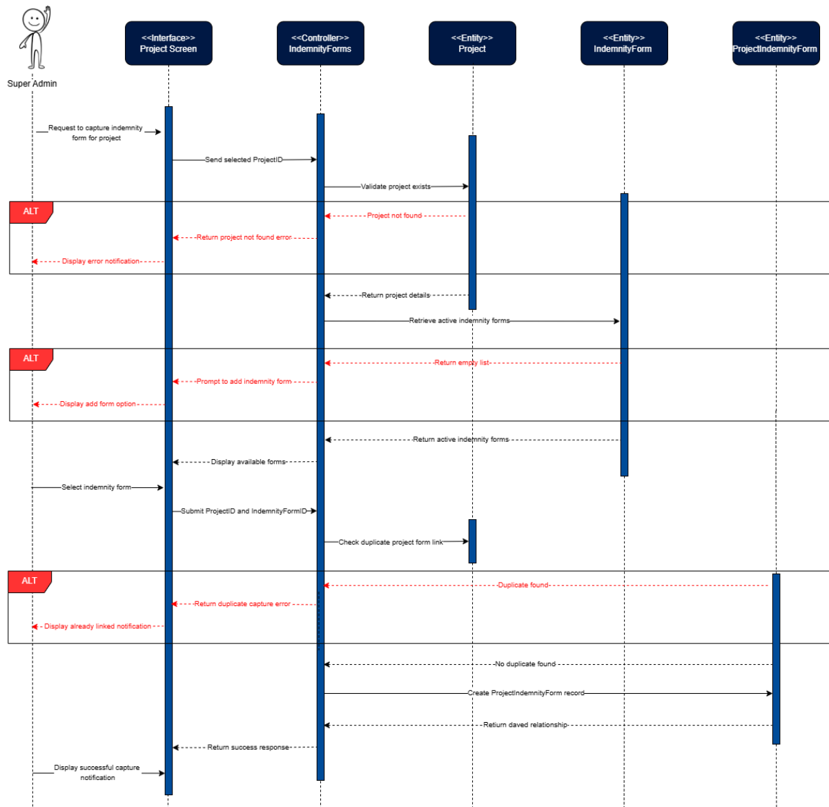
Figure 68: Capture Indemnity Form Sequence Diagram
