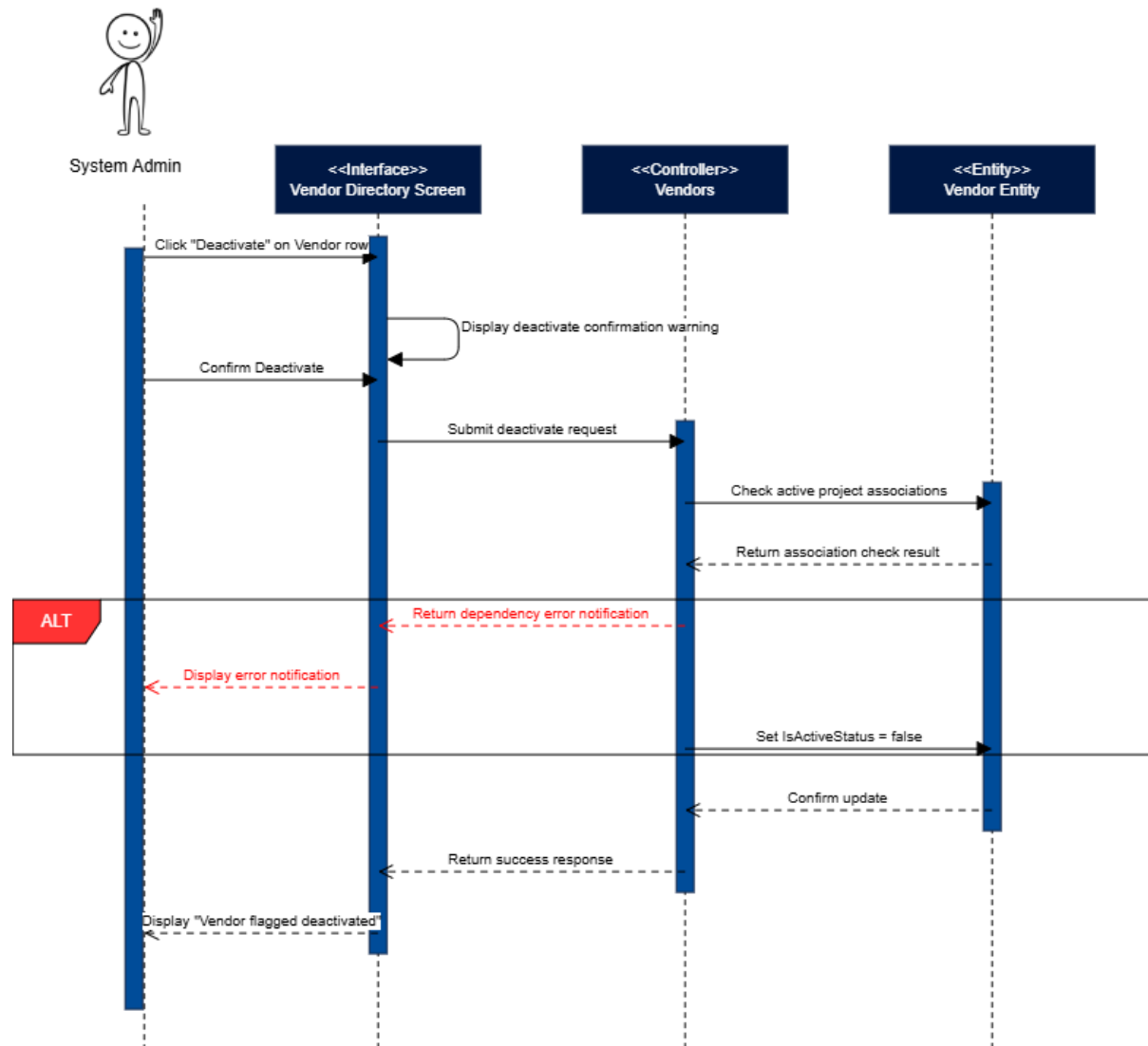
Figure 50: Deactivate Vendor Sequence Diagram
