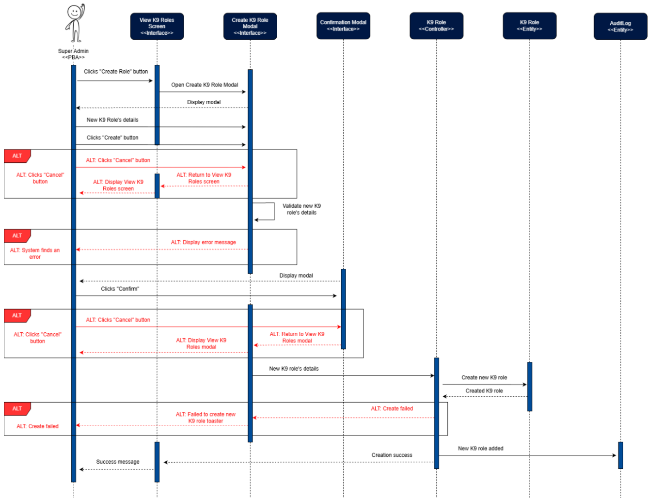
Figure 94: Add K9 Role Sequence Diagram
