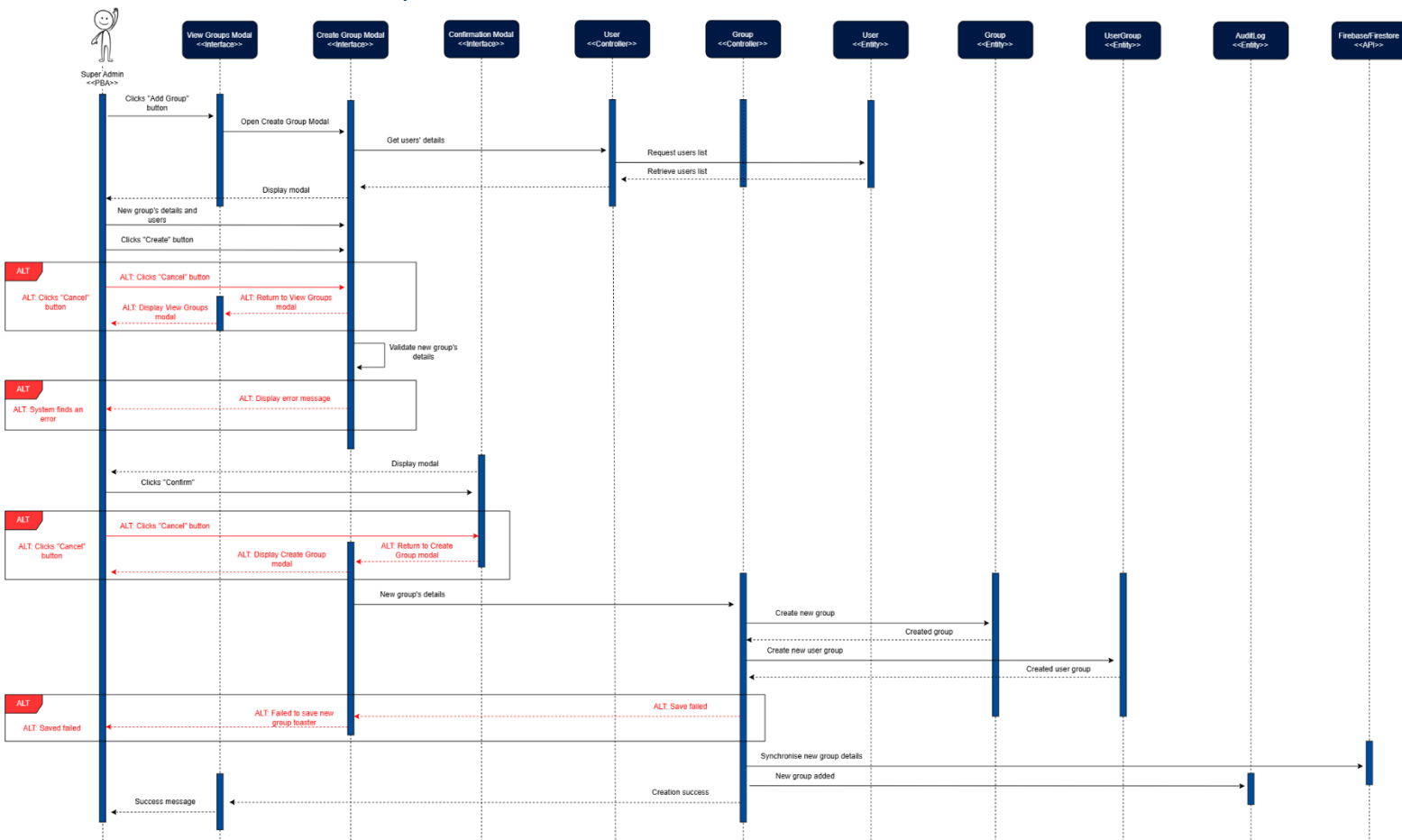
Figure 30: Create Group Sequence Diagram
