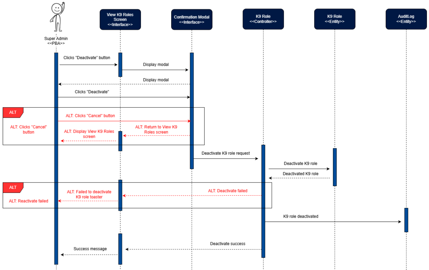
Figure 98: Deactivate K9 Role Sequence Diagram
