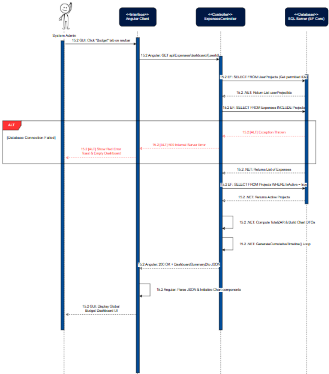
Figure 126: View Project Budgets Sequence Diagram
