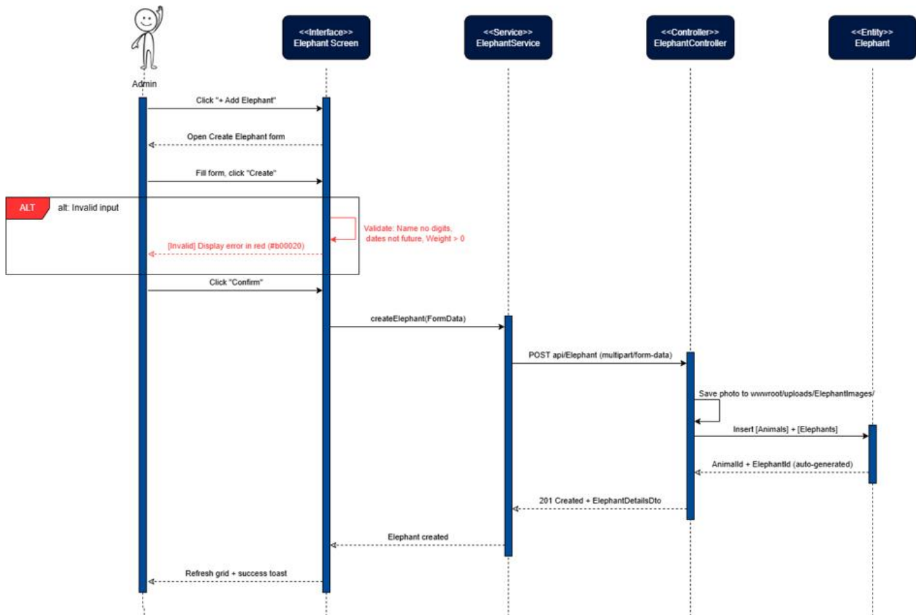
Figure 105: Add Elephant Sequence Diagram
