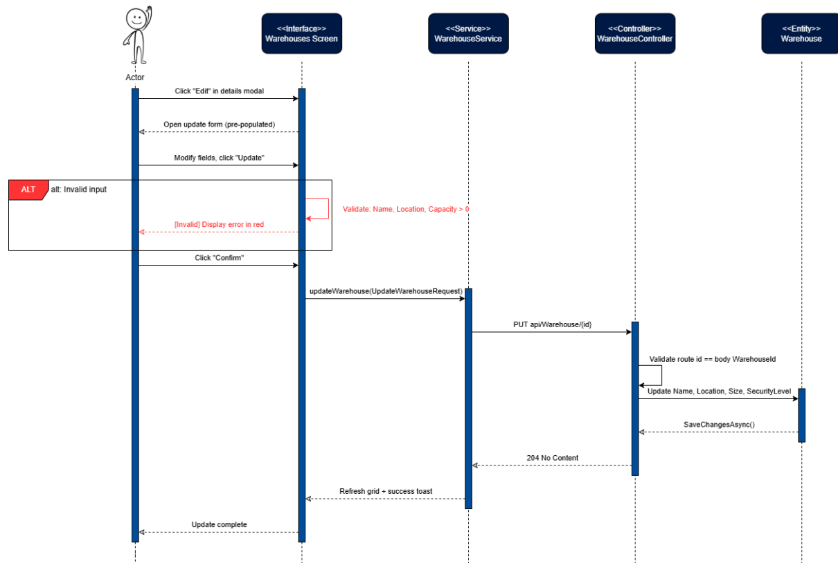
Figure 41: Update Warehouse Sequence Diagram
