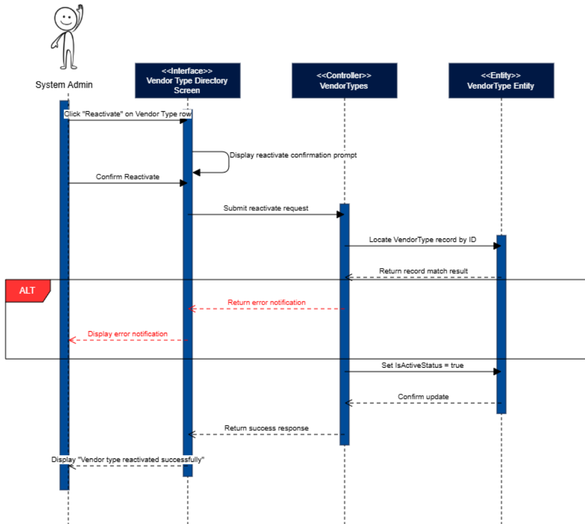
Figure 54: Reactivate Vendor Type Sequence Diagram
