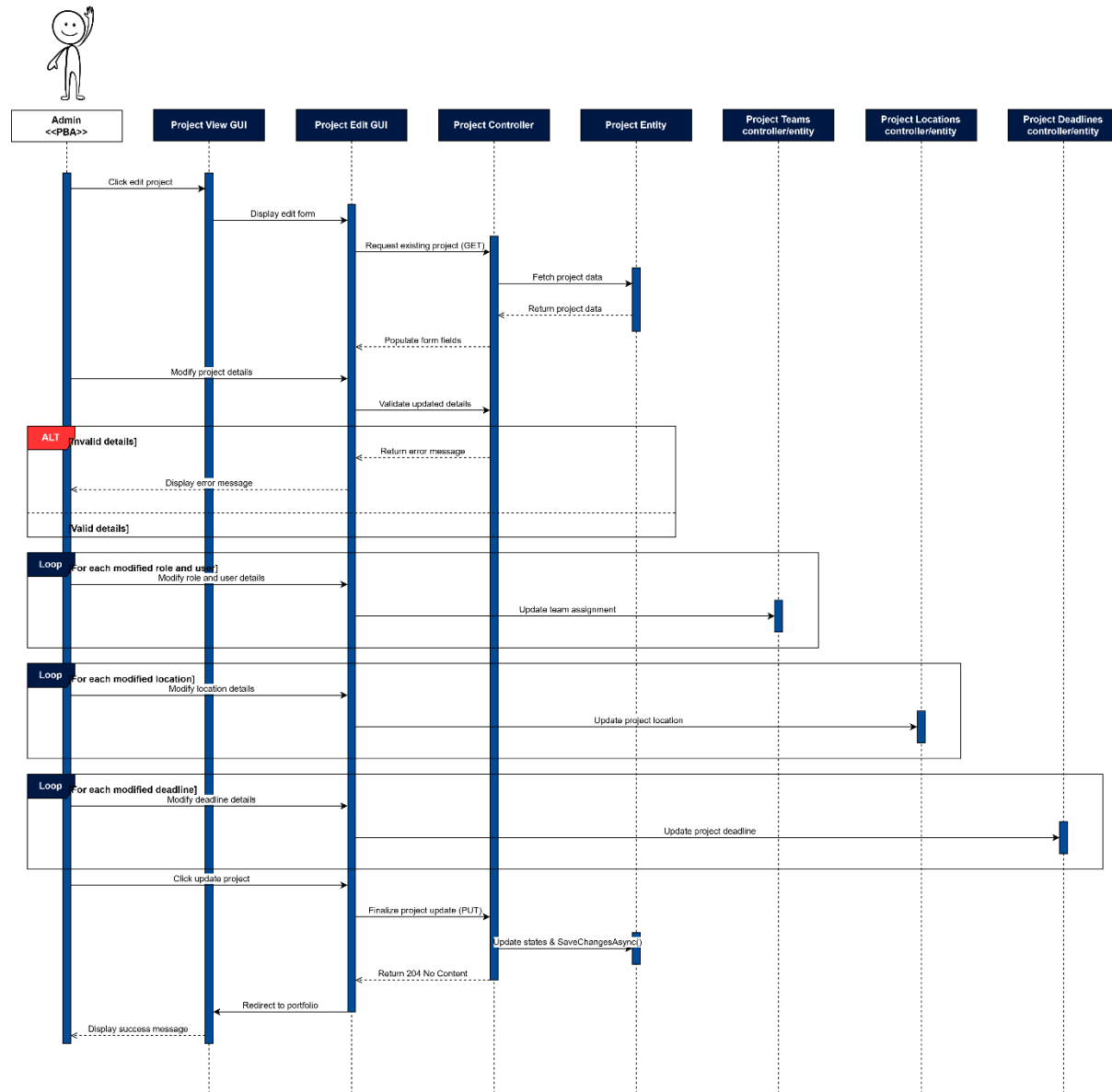
Figure 58: Update Project Sequence Diagram
