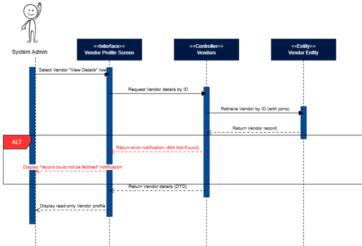
Figure 46: View Vendor Sequence Diagram
