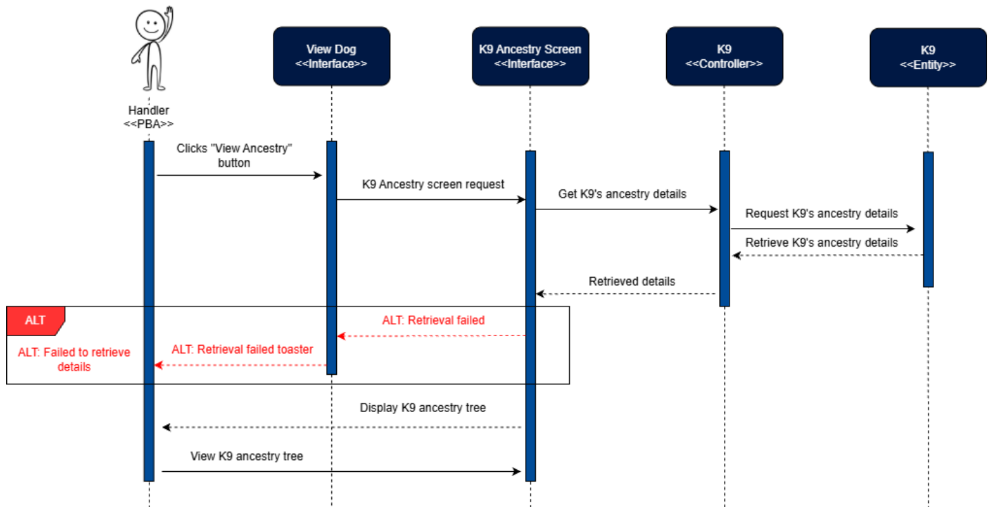
Figure 99: View K9 Ancestry Sequence Diagram
