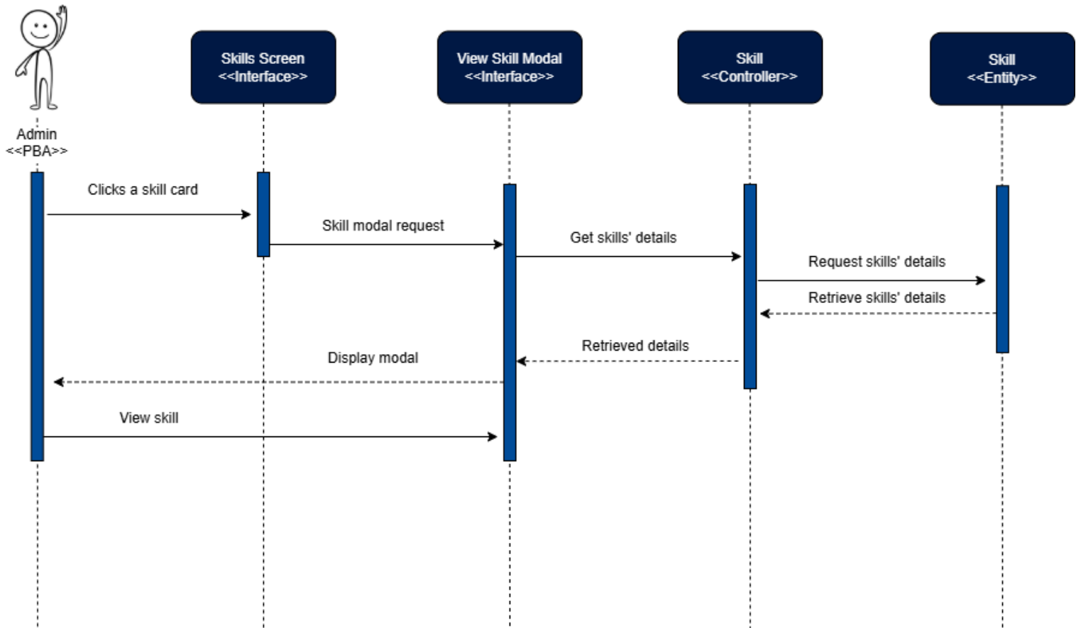
Figure 36: View Skill Sequence Diagram
