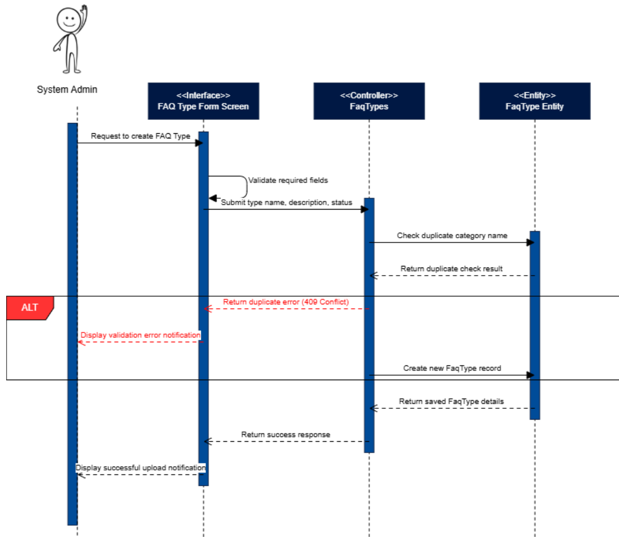
Figure 17: Add FAQ Type Sequence Diagram
