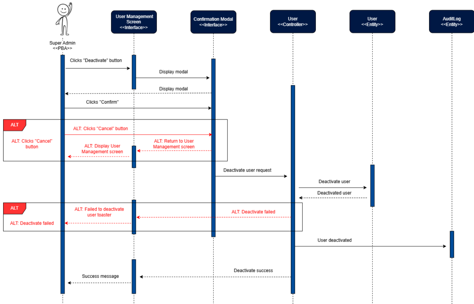
Figure 13: Deactivate User Sequence Diagram
