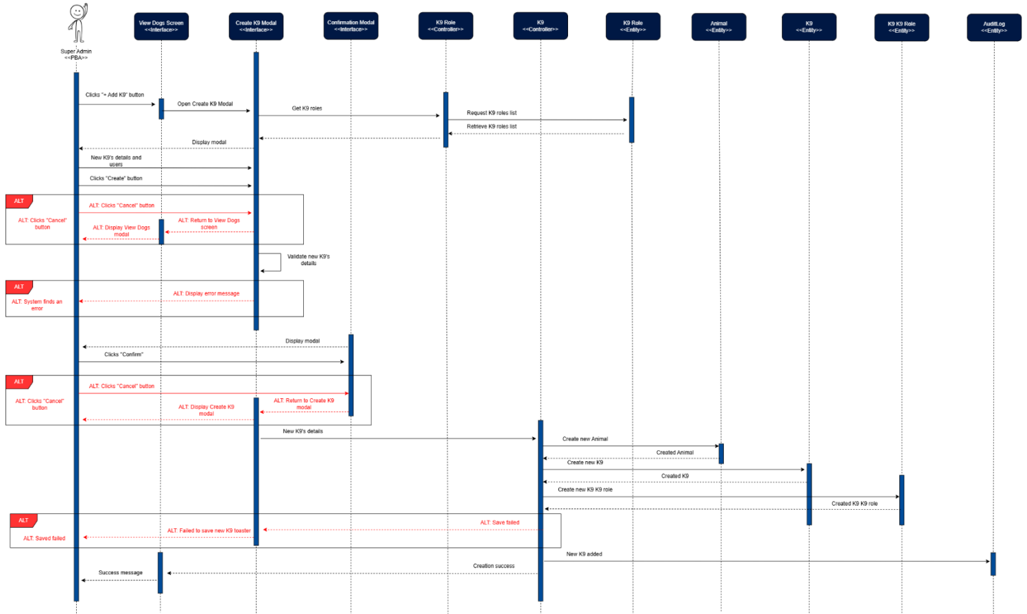
Figure 84: Add Dog Sequence Diagram
