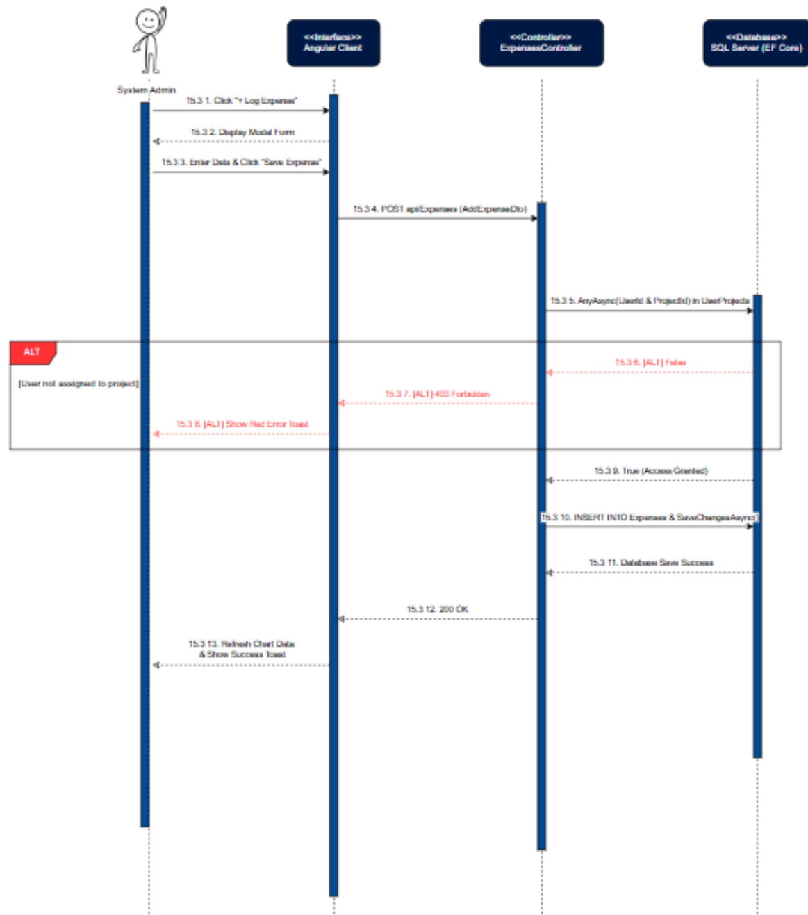
Figure 127: Log An Expense Sequence Diagram
