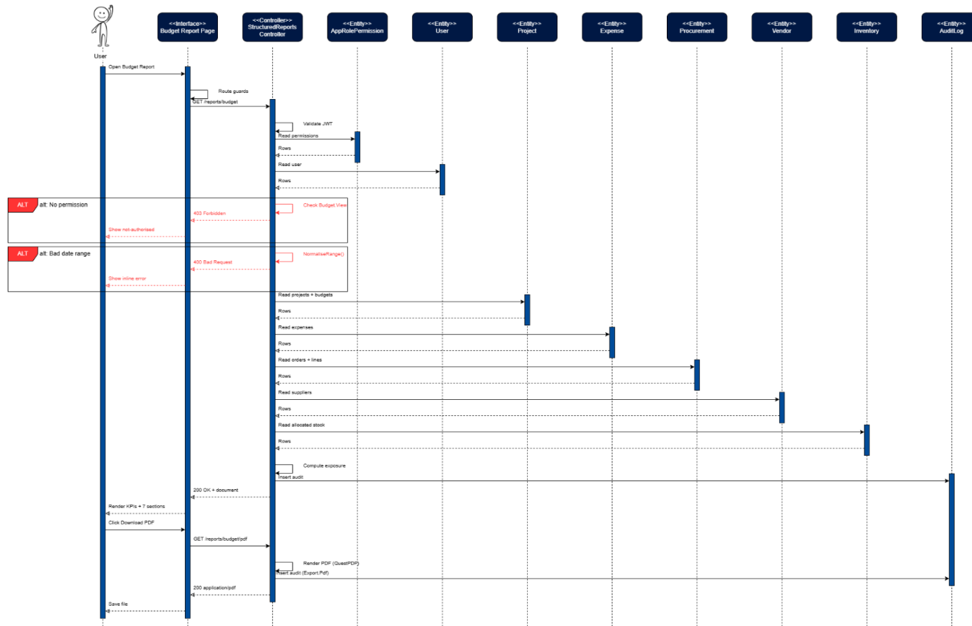
Figure 117: View Budget Report Sequence Diagram
