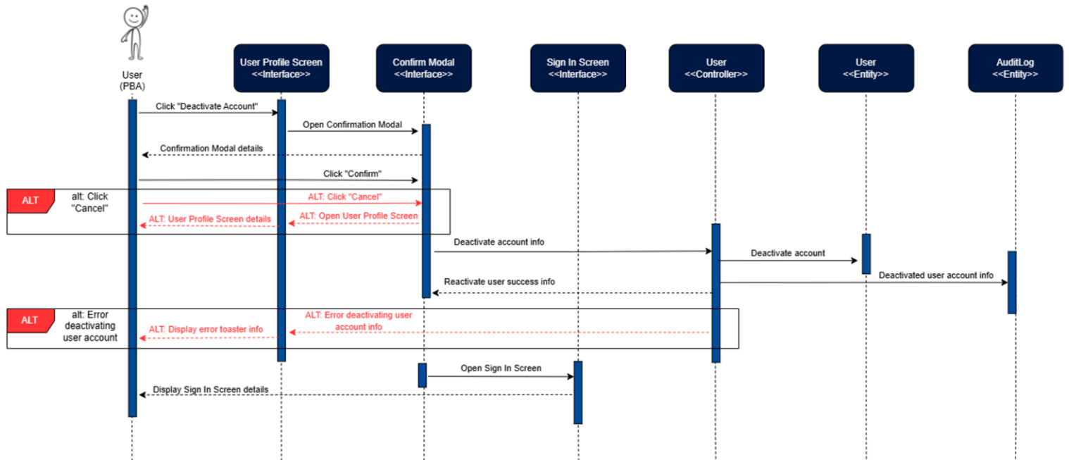
Figure 8: Deactivate User Sequence Diagram
