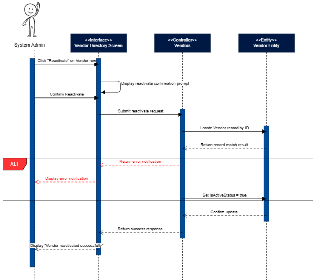
Figure 49: Reactivate Vendor Sequence Diagram
