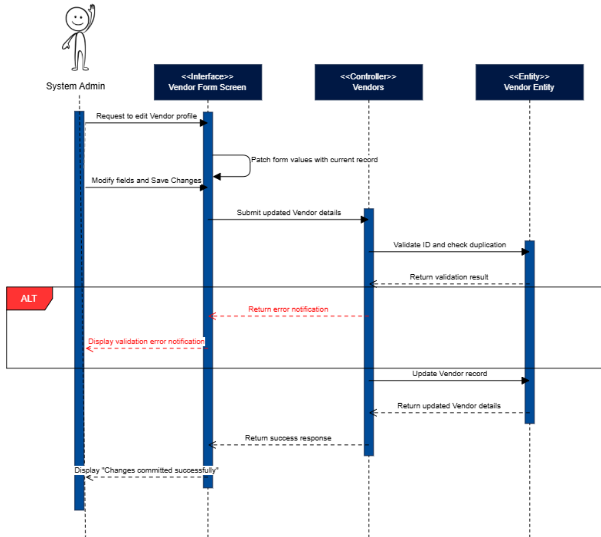
Figure 48: Edit Vendor Sequence Diagram
