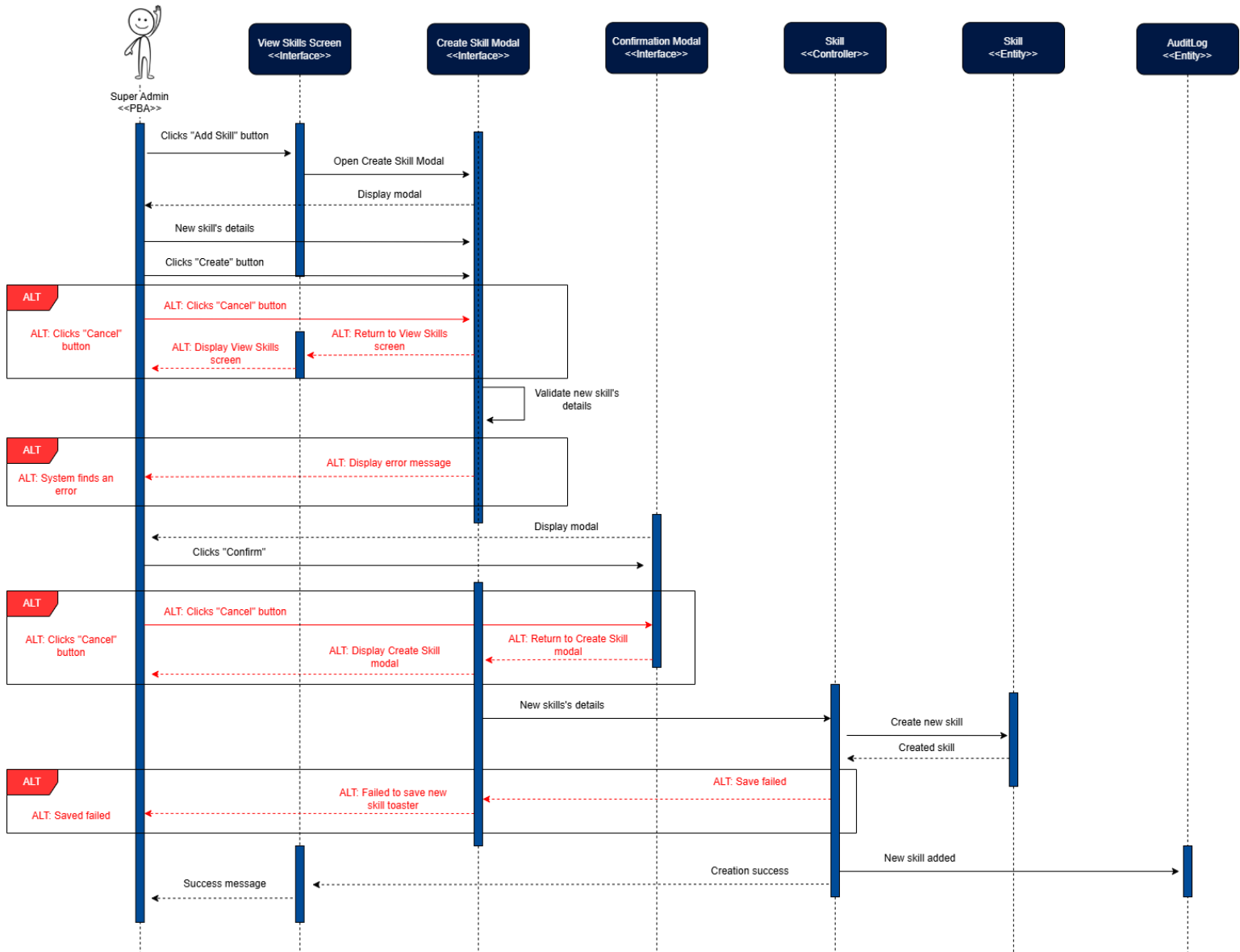
Figure 34: Create Skill Sequence Diagram
