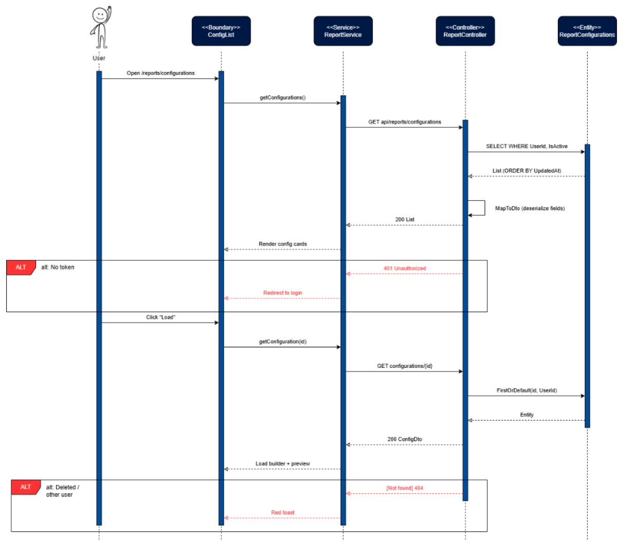
Figure 113: View Custom Report Sequence Diagram
