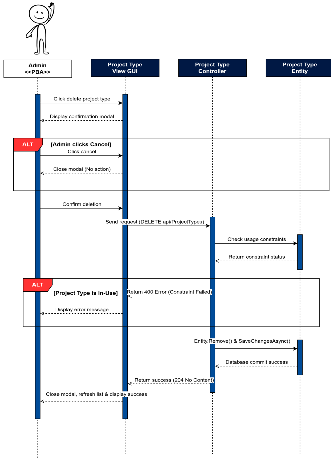
Figure 63: Deactivate Project Type Sequence Diagram
