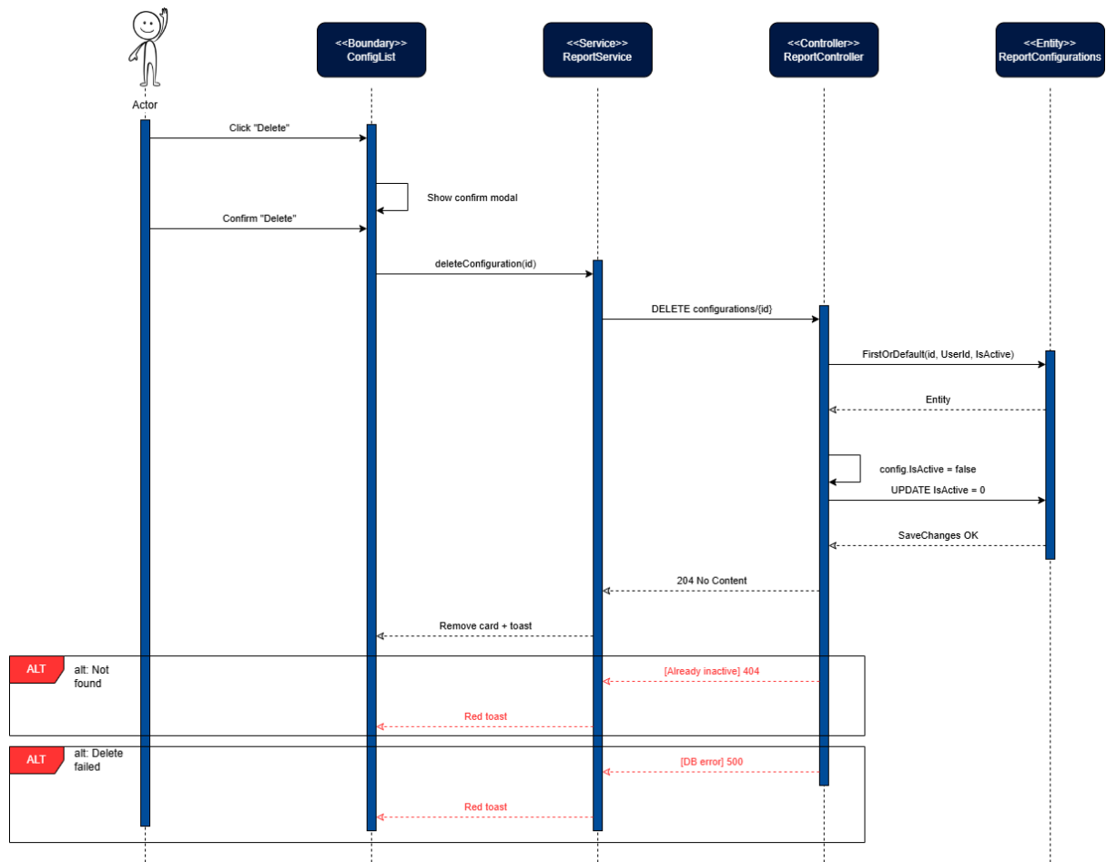
Figure 115: Remove Custom Report Sequence Diagram
