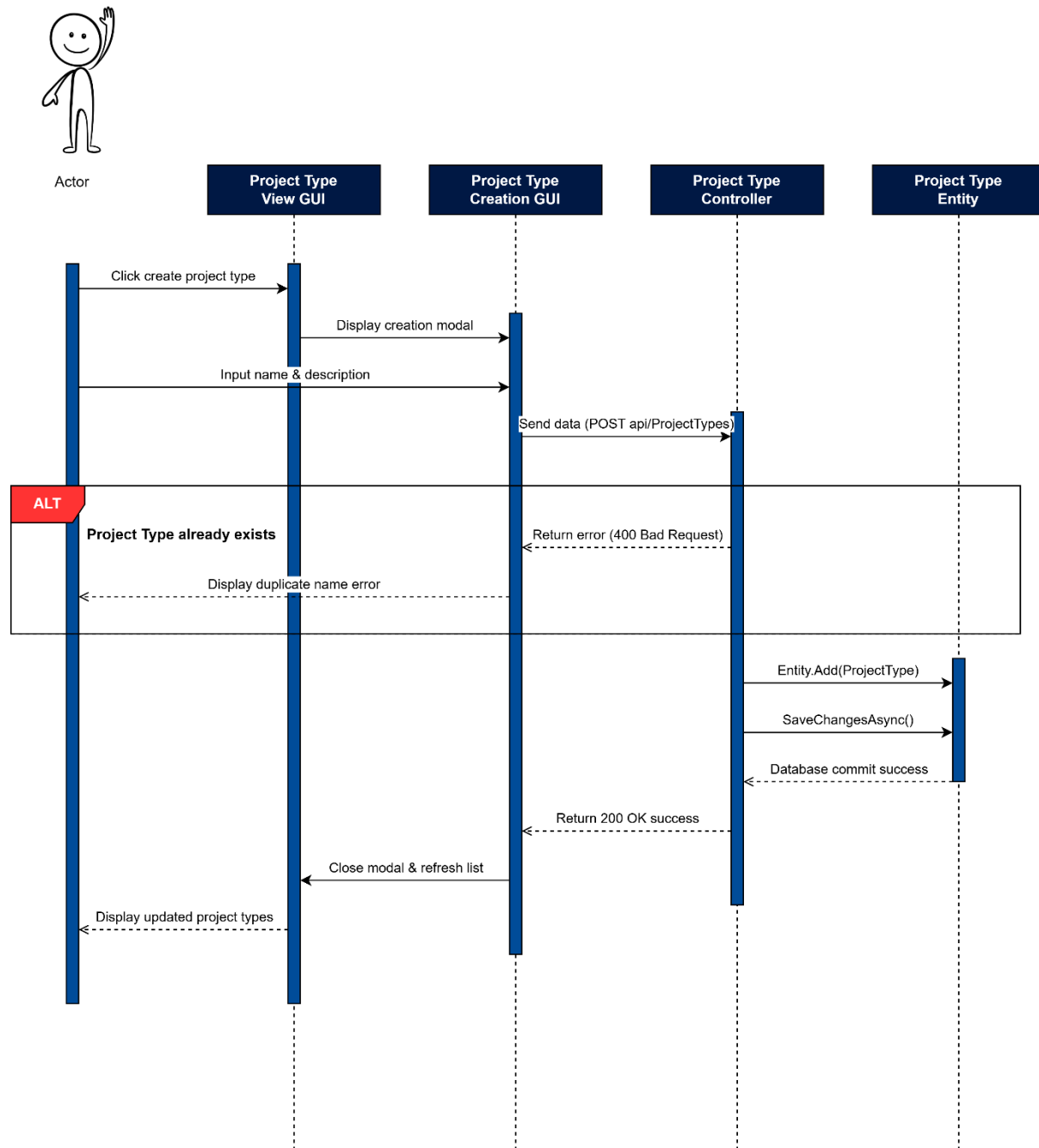
Figure 60: Create Project Type Sequence Diagram
