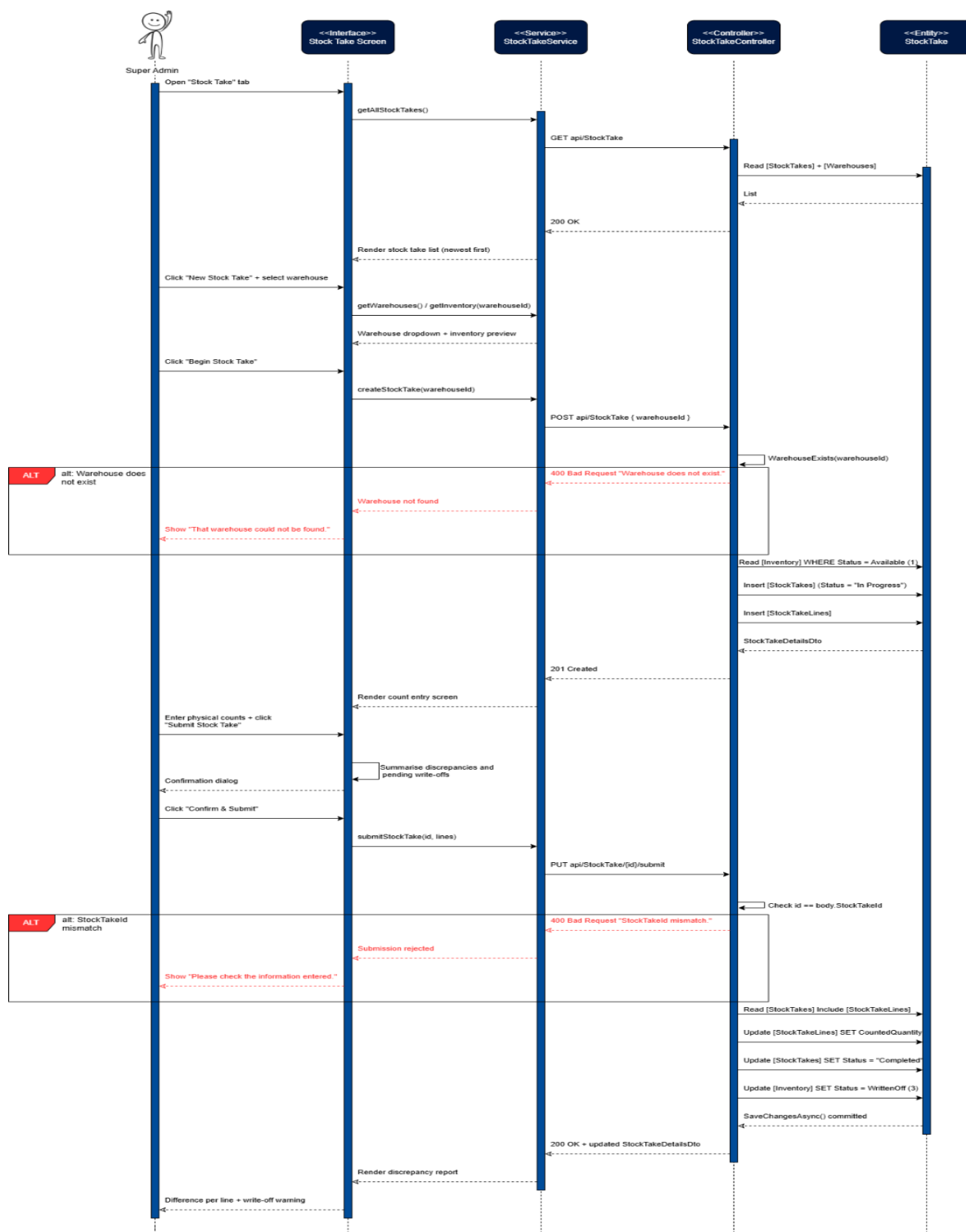
Figure 44: Inventory Stock Take Sequence Diagram
