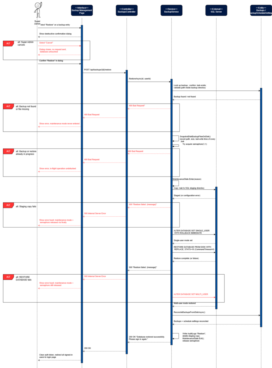
Figure 123: Restore System Sequence Diagram
