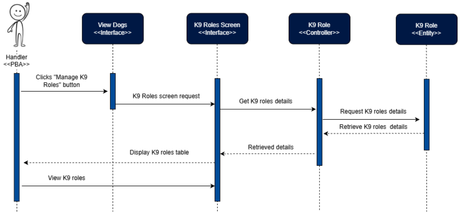
Figure 95: View K9 Role Sequence Diagram
