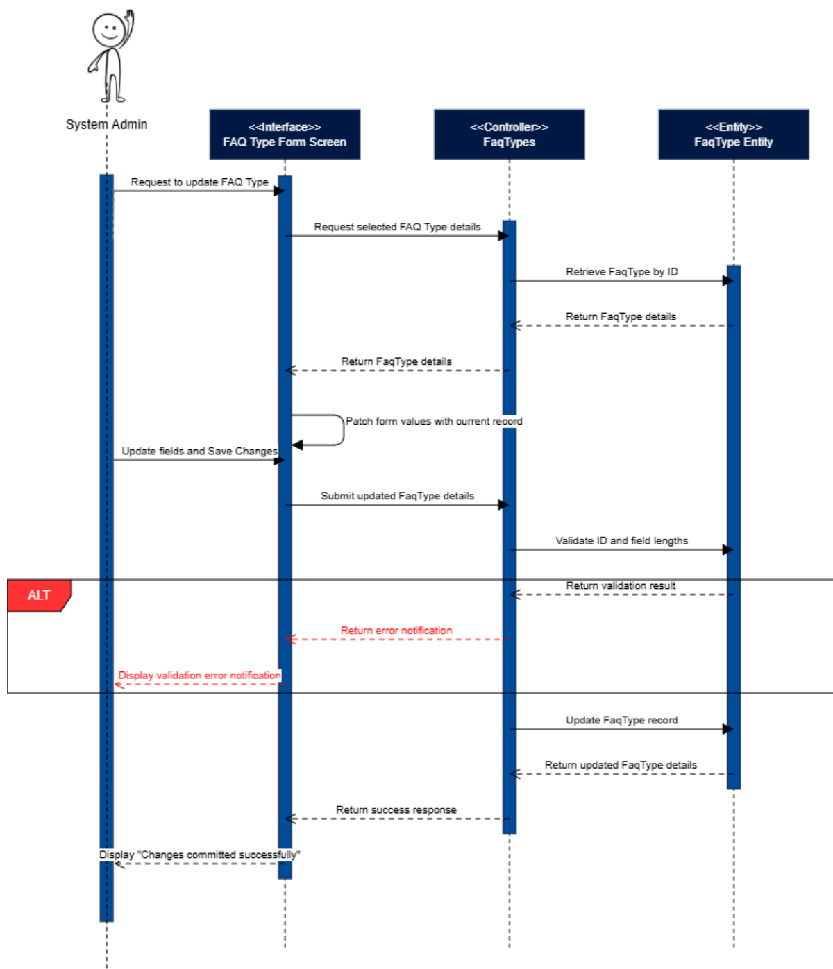
Figure 18: Update FAQ Type Sequence Diagram
