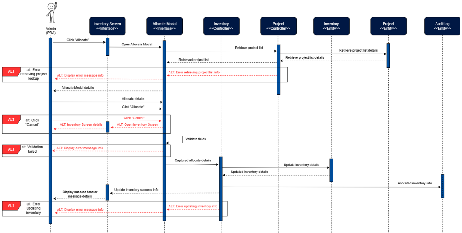
Figure 23: Allocate Inventory Sequence Diagram
