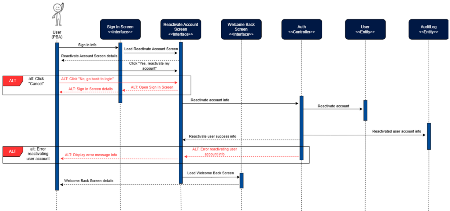
Figure 7: Reactivate User Sequence Diagram
