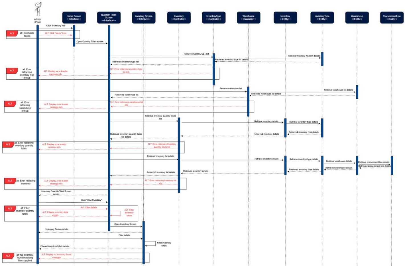
Figure 21: View Inventory Sequence Diagram
