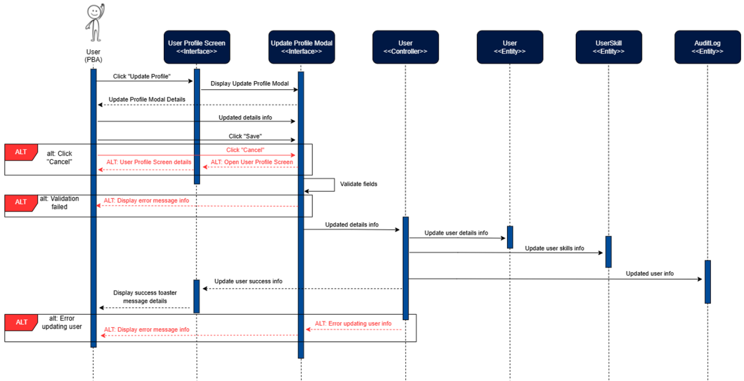
Figure 5: Update User Sequence Diagram
