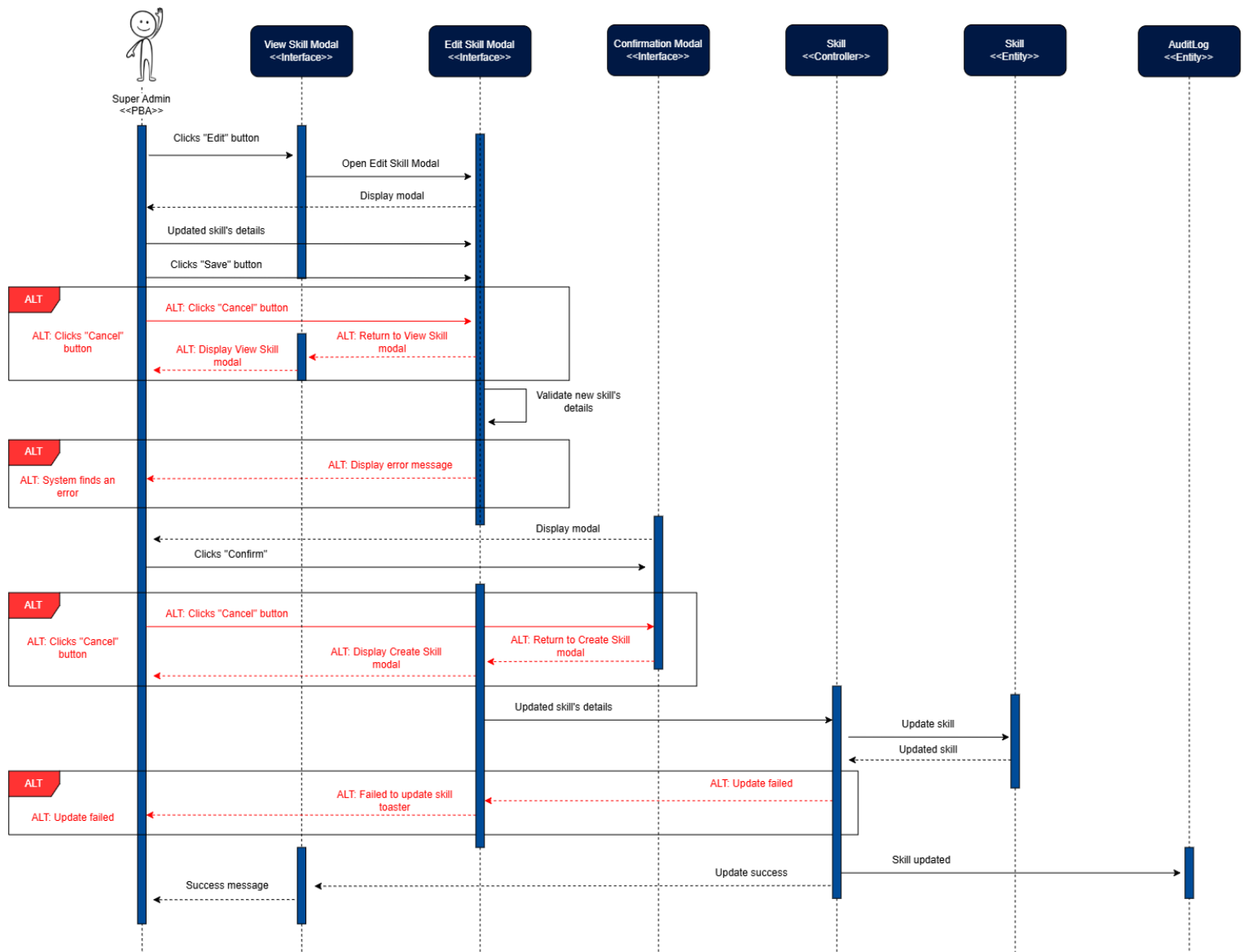
Figure 37: Update Skill Sequence Diagram
