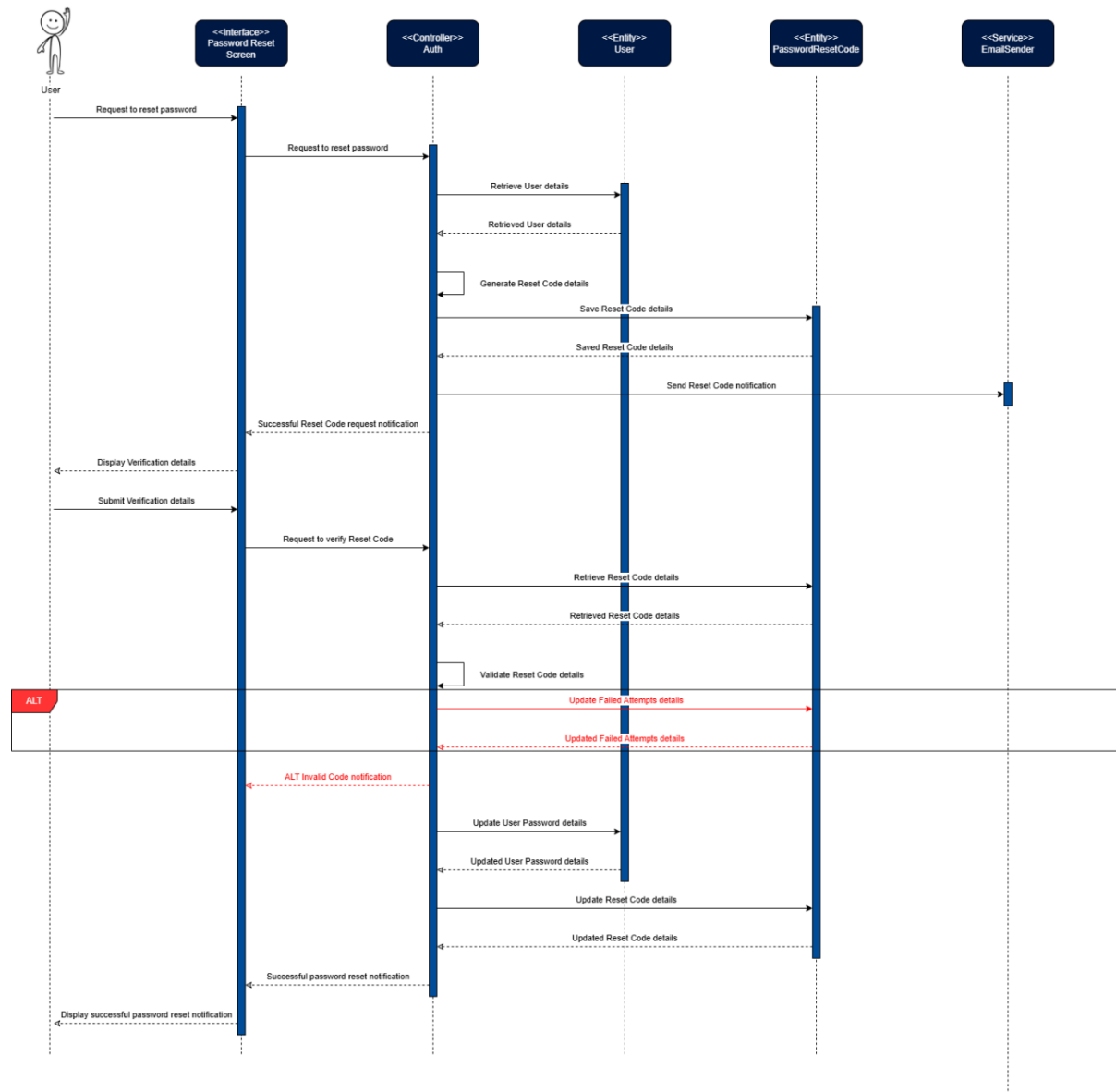
Figure 3: Password Reset Sequence Diagram
