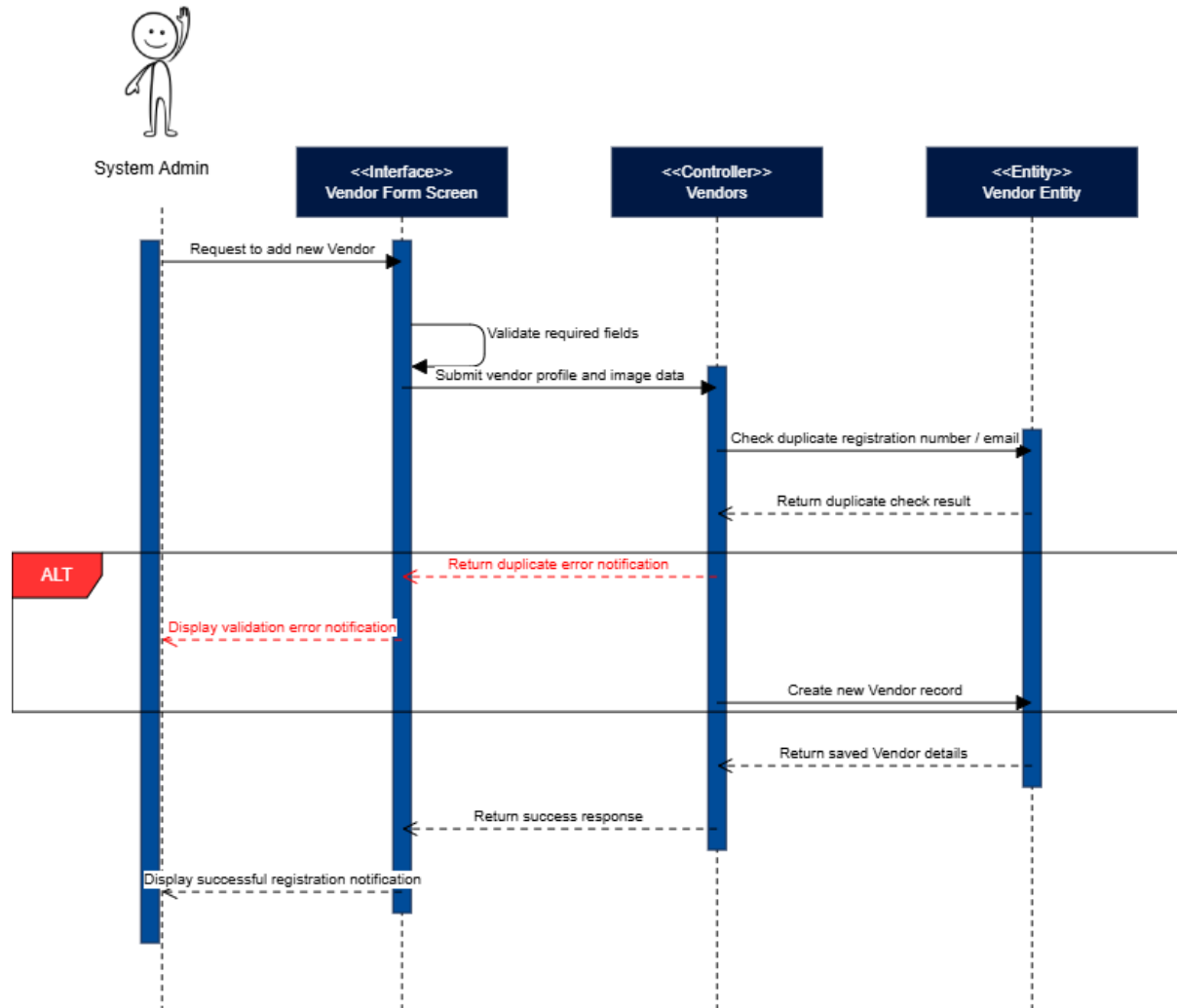
Figure 45: Create Vendor Sequence Diagram
