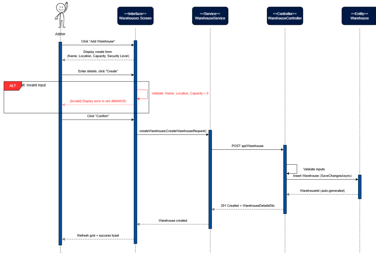
Figure 39: Create Warehouse Sequence Diagram
