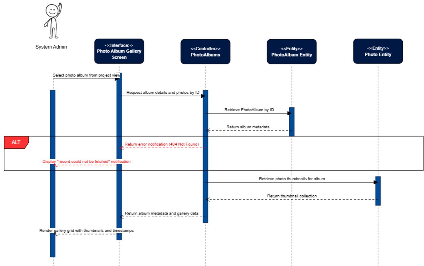
Figure 81: View Photo Album Sequence Diagram
