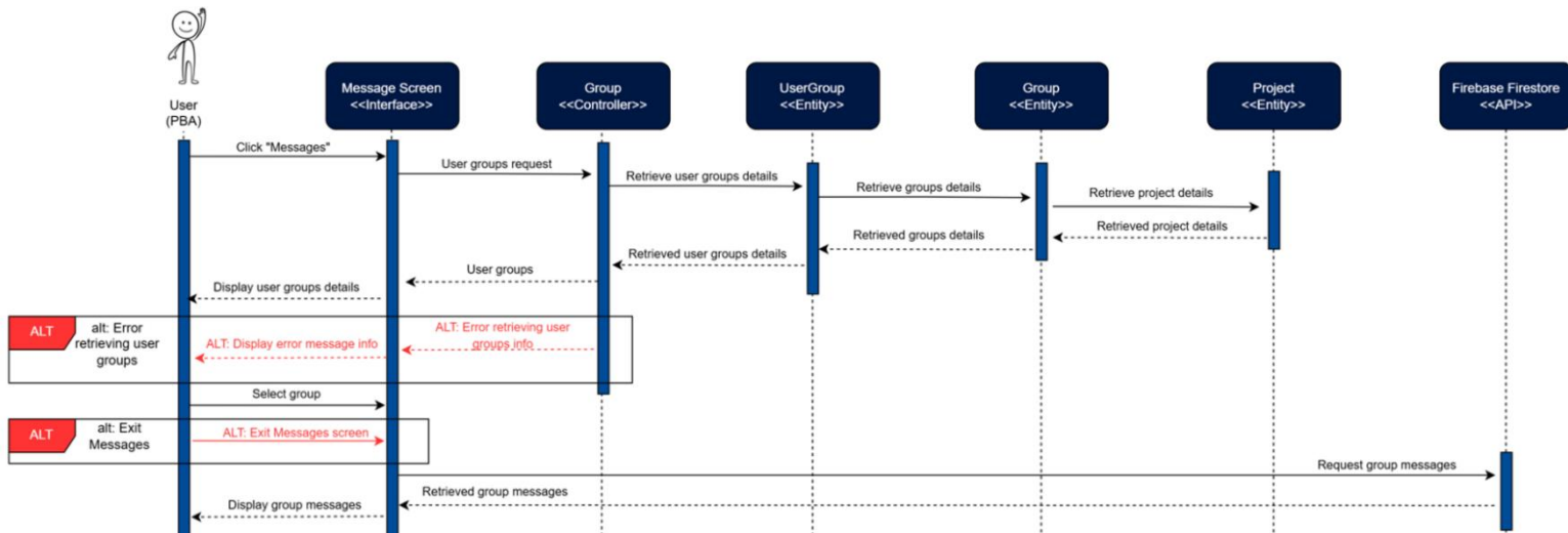
Figure 111: View Message Sequence Diagram
