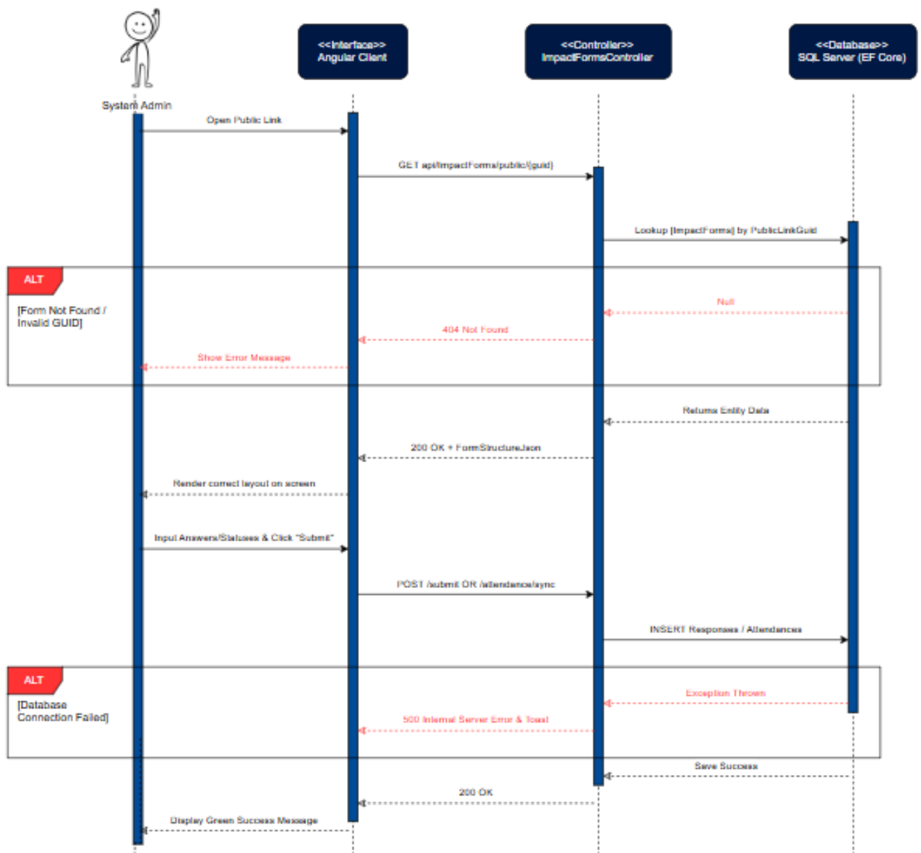
Figure 75: Capture Impact Feedback Sequence Diagram
