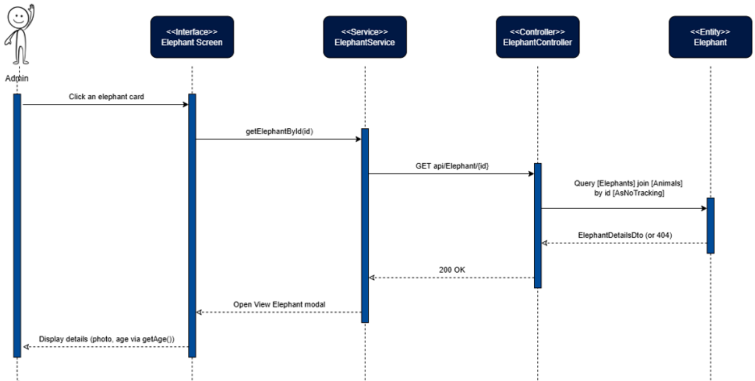
Figure 106: View Elephant Sequence Diagram
