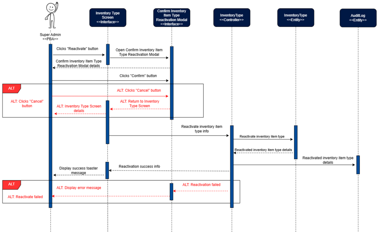
Figure 29: Reactivate Inventory Item Type Sequence Diagram
