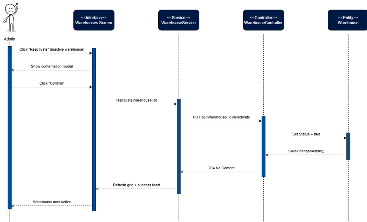
Figure 42: Reactivate Warehouse Sequence Diagram
