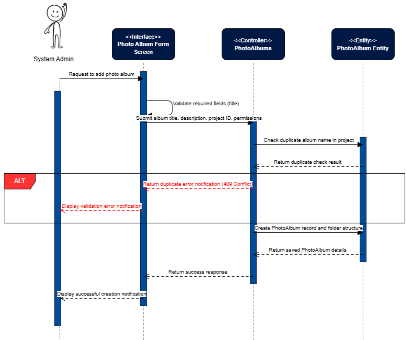
Figure 80: Add Photo Album Sequence Diagram
