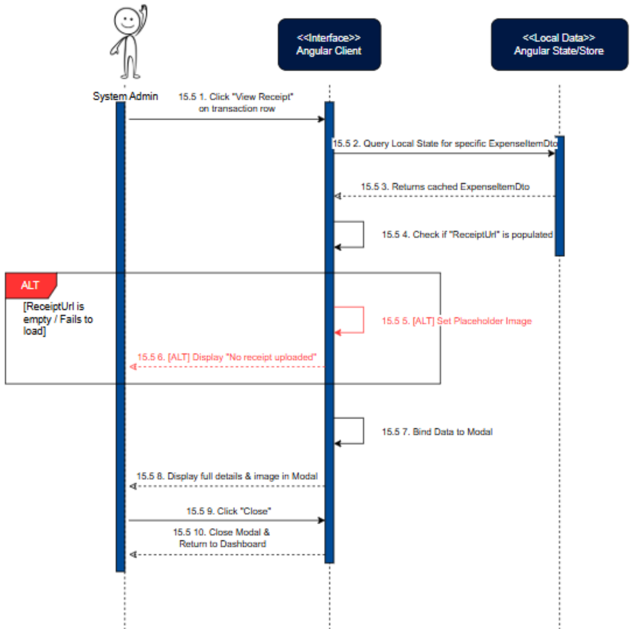
Figure 129: View Expense Sequence Diagram
