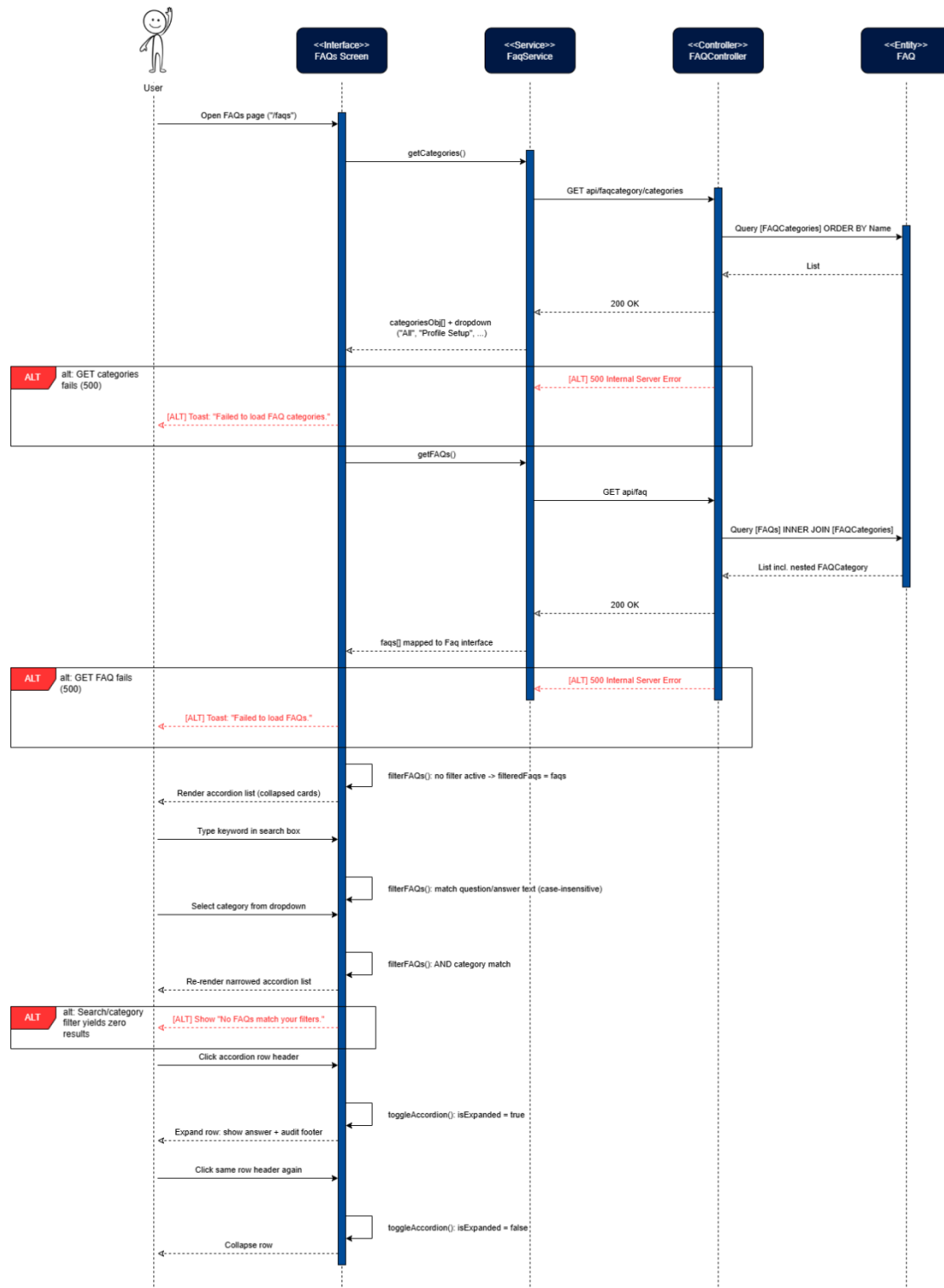
Figure 9: View FAQ Sequence Diagram
