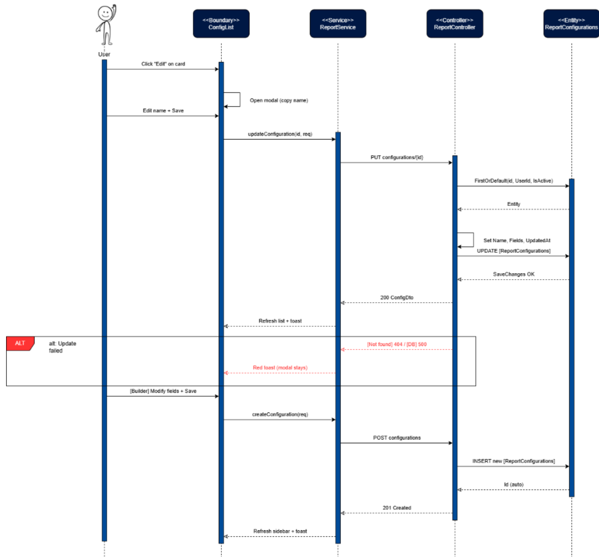
Figure 114: Update Custom Report Sequence Diagram
