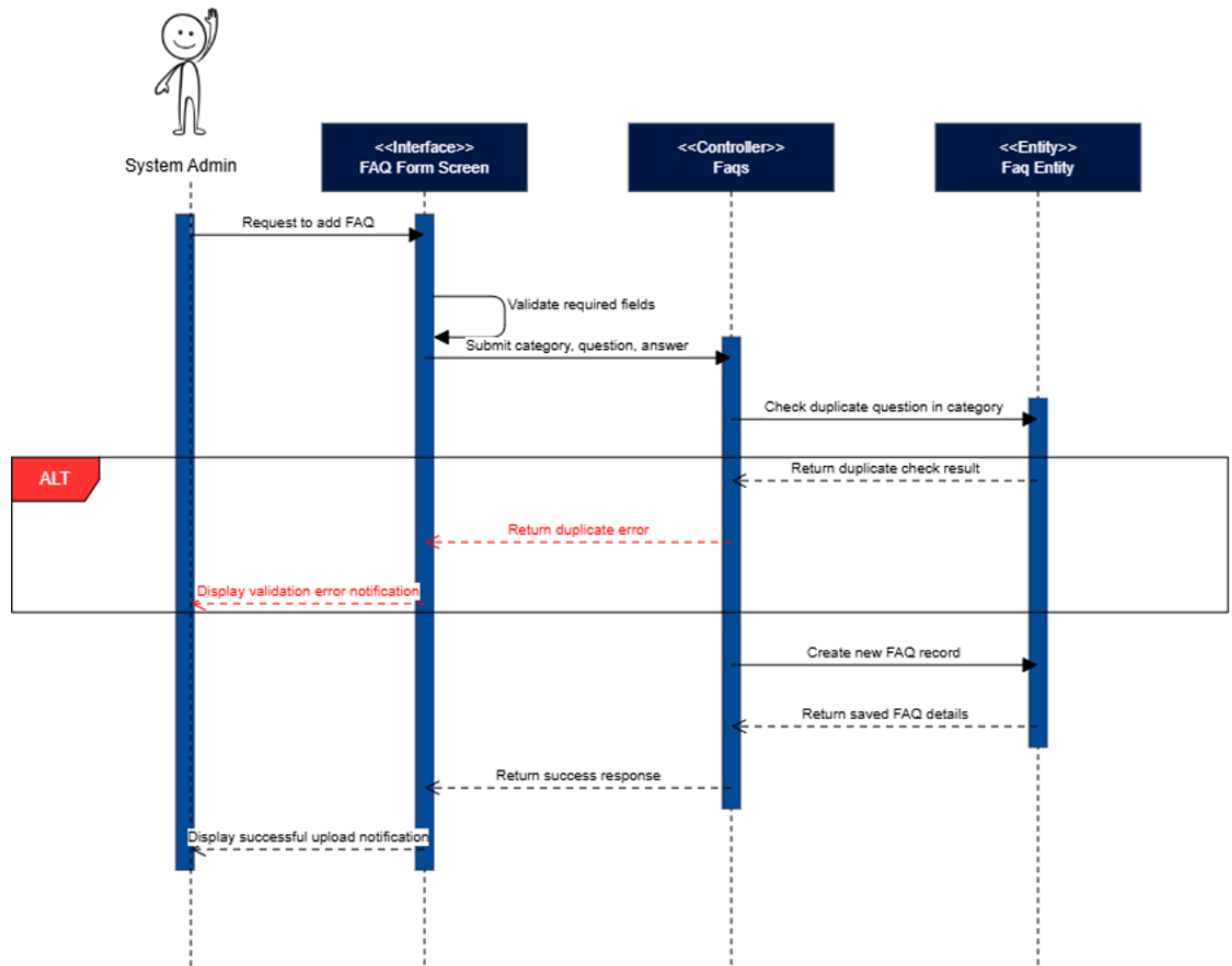
Figure 14: Add FAQ Sequence Diagram
