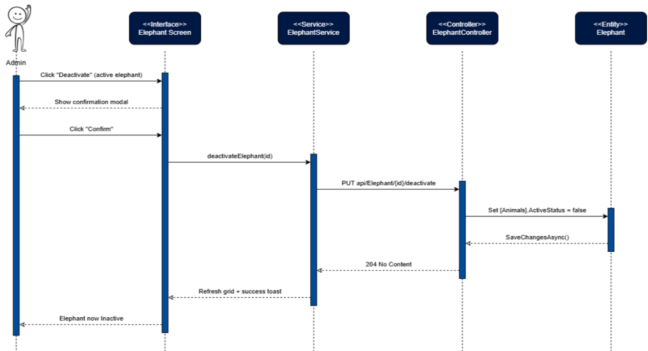
Figure 109: Deactivate Elephant Sequence Diagram
