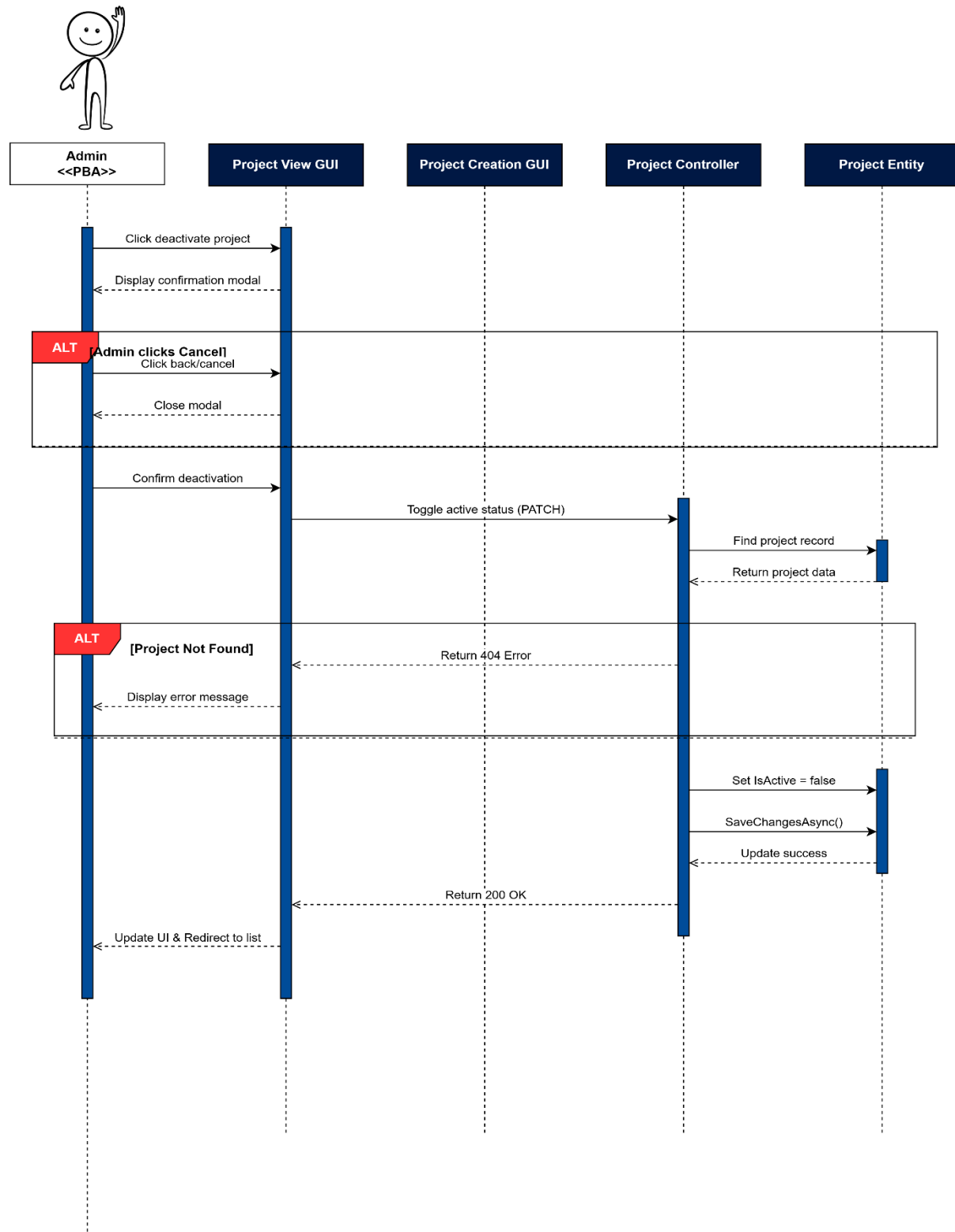
Figure 59: Deactivate Project Sequence Diagram
