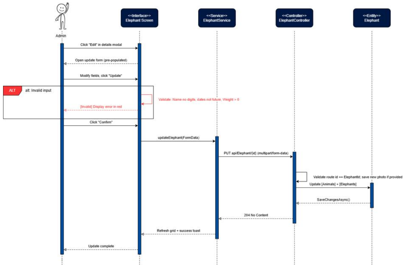
Figure 108: Update Elephant Sequence Diagram
