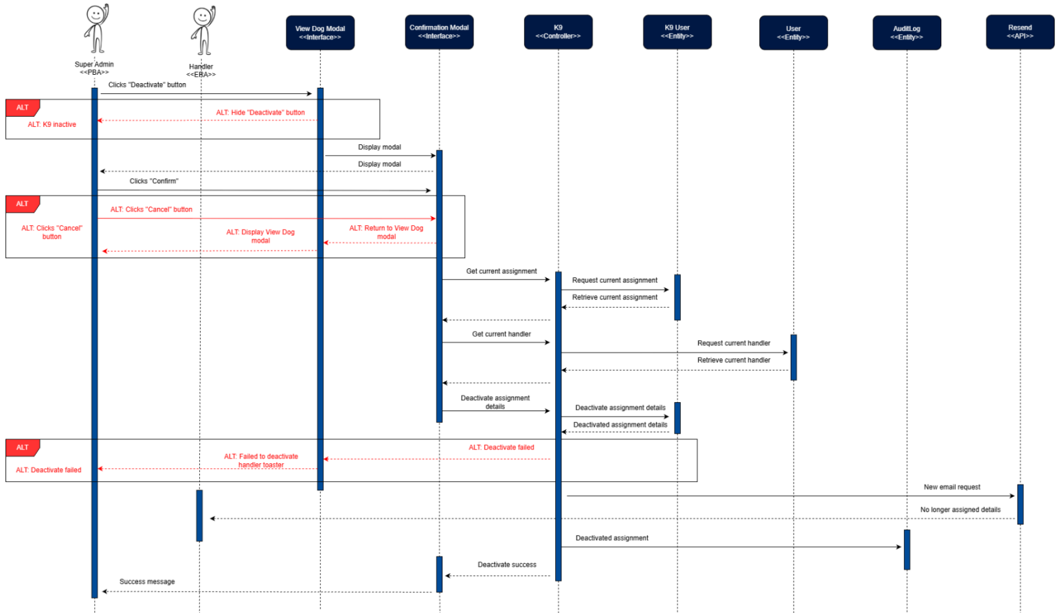
Figure 93: Deactivate User-Dog Assignment Sequence Diagram
