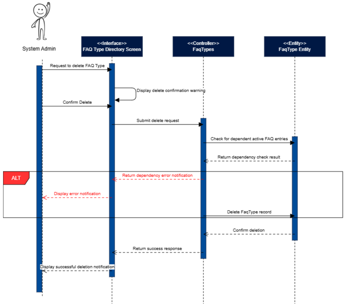
Figure 19: Remove FAQ Type Sequence Diagram
