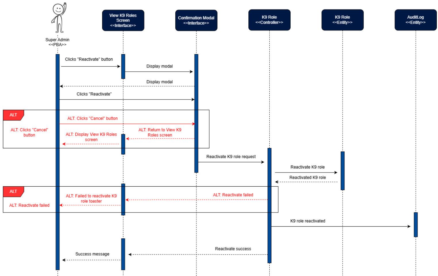
Figure 97: Reactivate K9 Role Sequence Diagram
