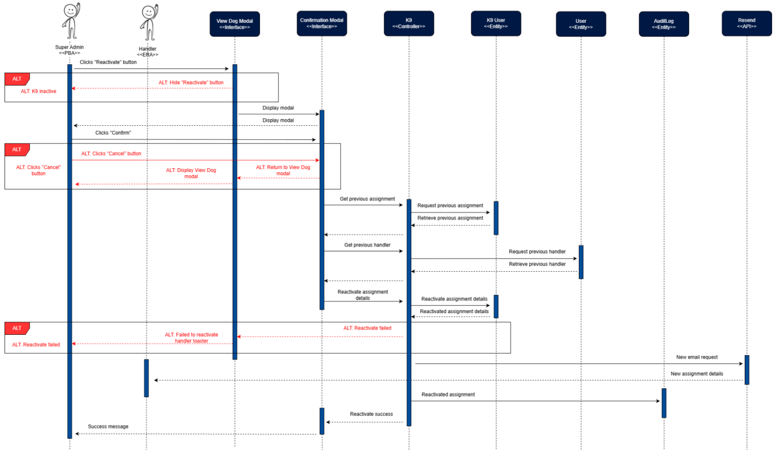
Figure 92: Reactivate User-Dog Assignment Sequence Diagram
