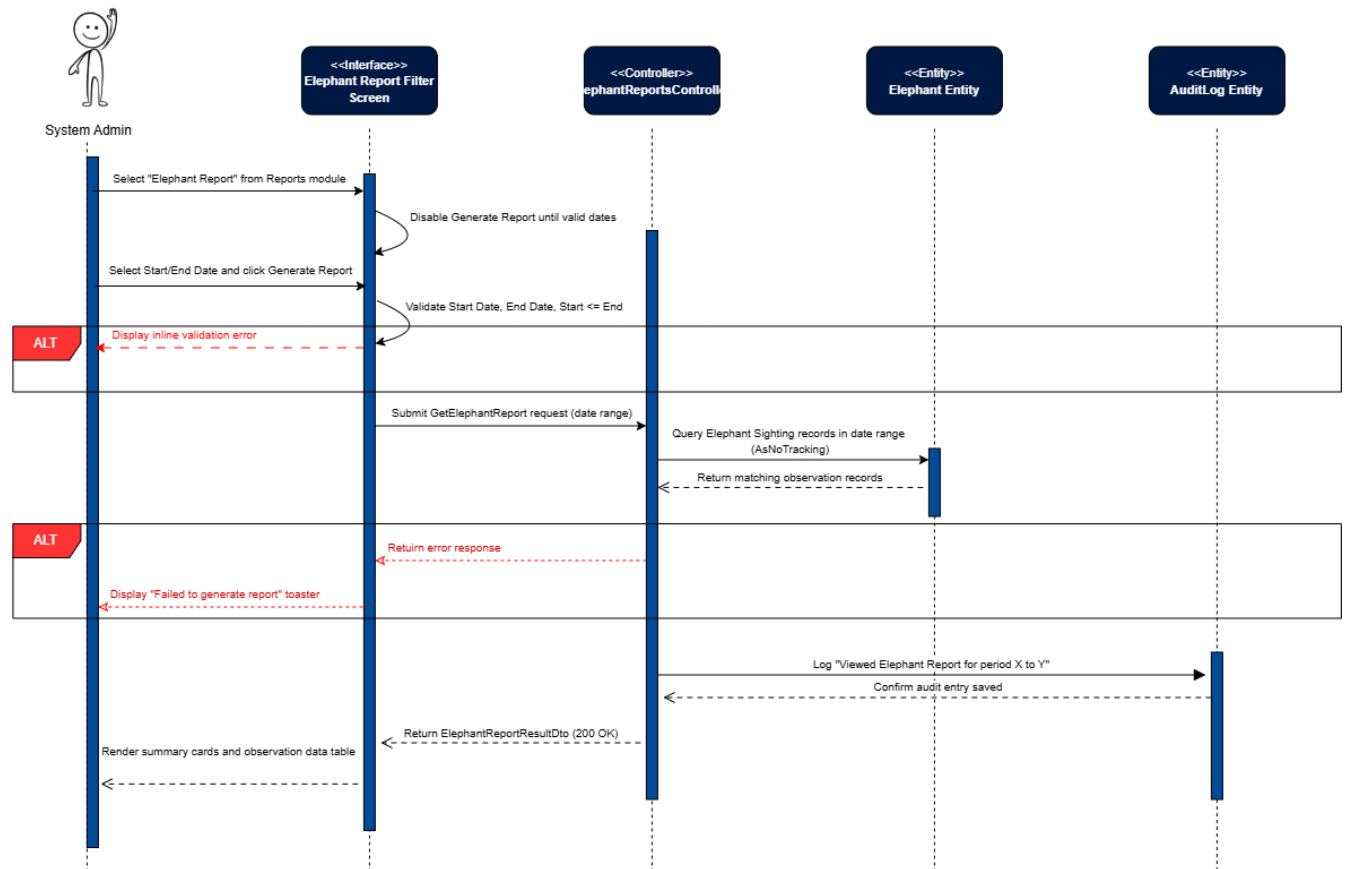
Figure 119: View Elephant Report Sequence Diagram
