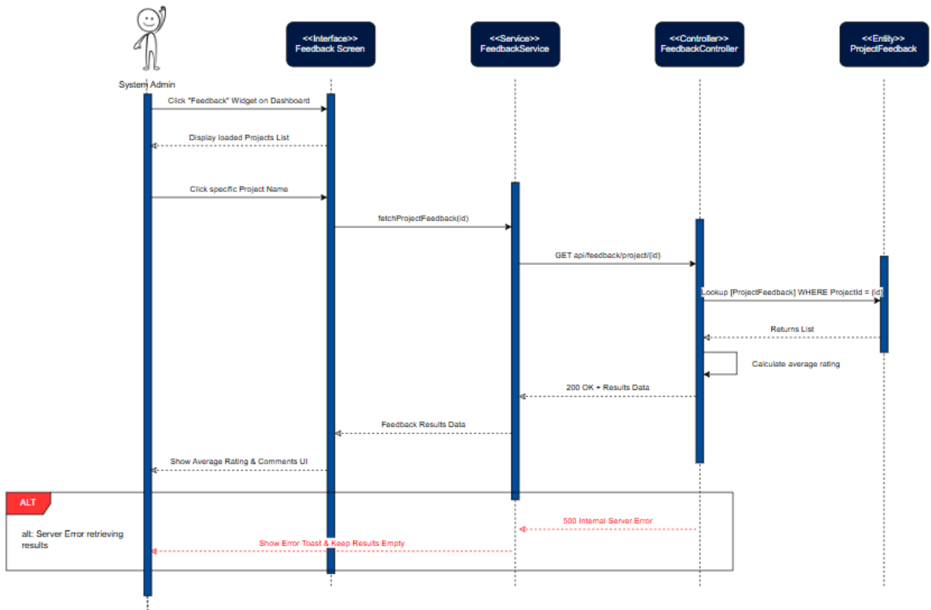
Figure 70: View Project Feedback Sequence Diagram
