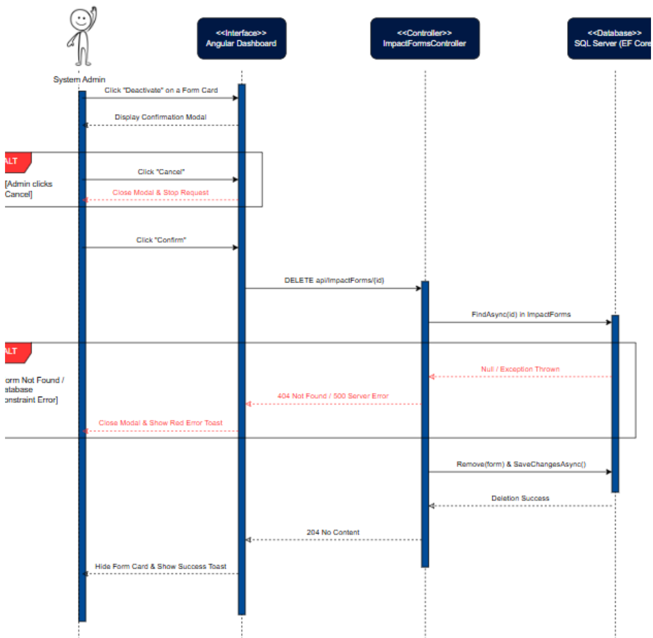
Figure 74: Deactivate Impact Feedback Form Sequence Diagram
