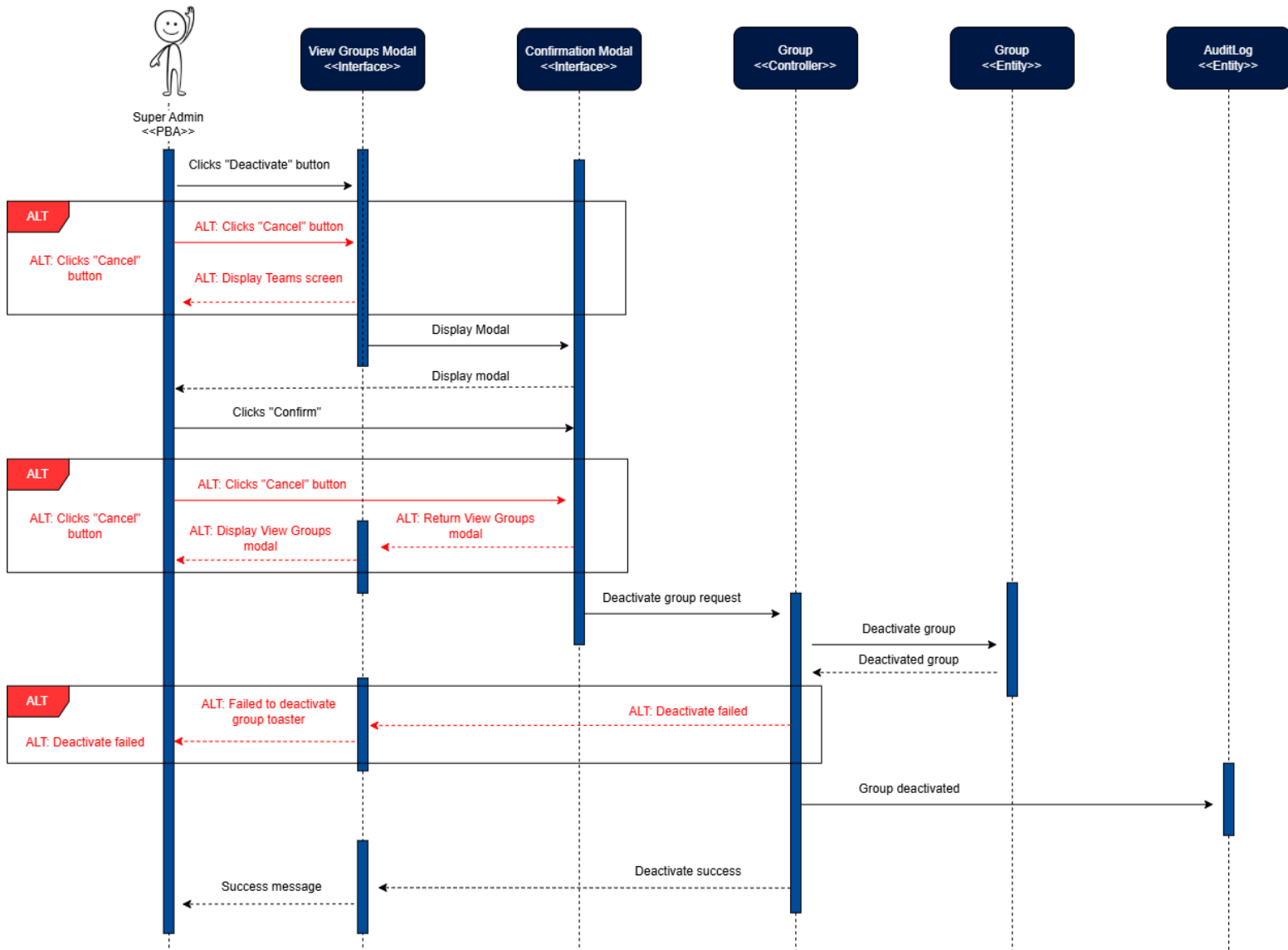
Figure 33: Deactivate Group Sequence Diagram
