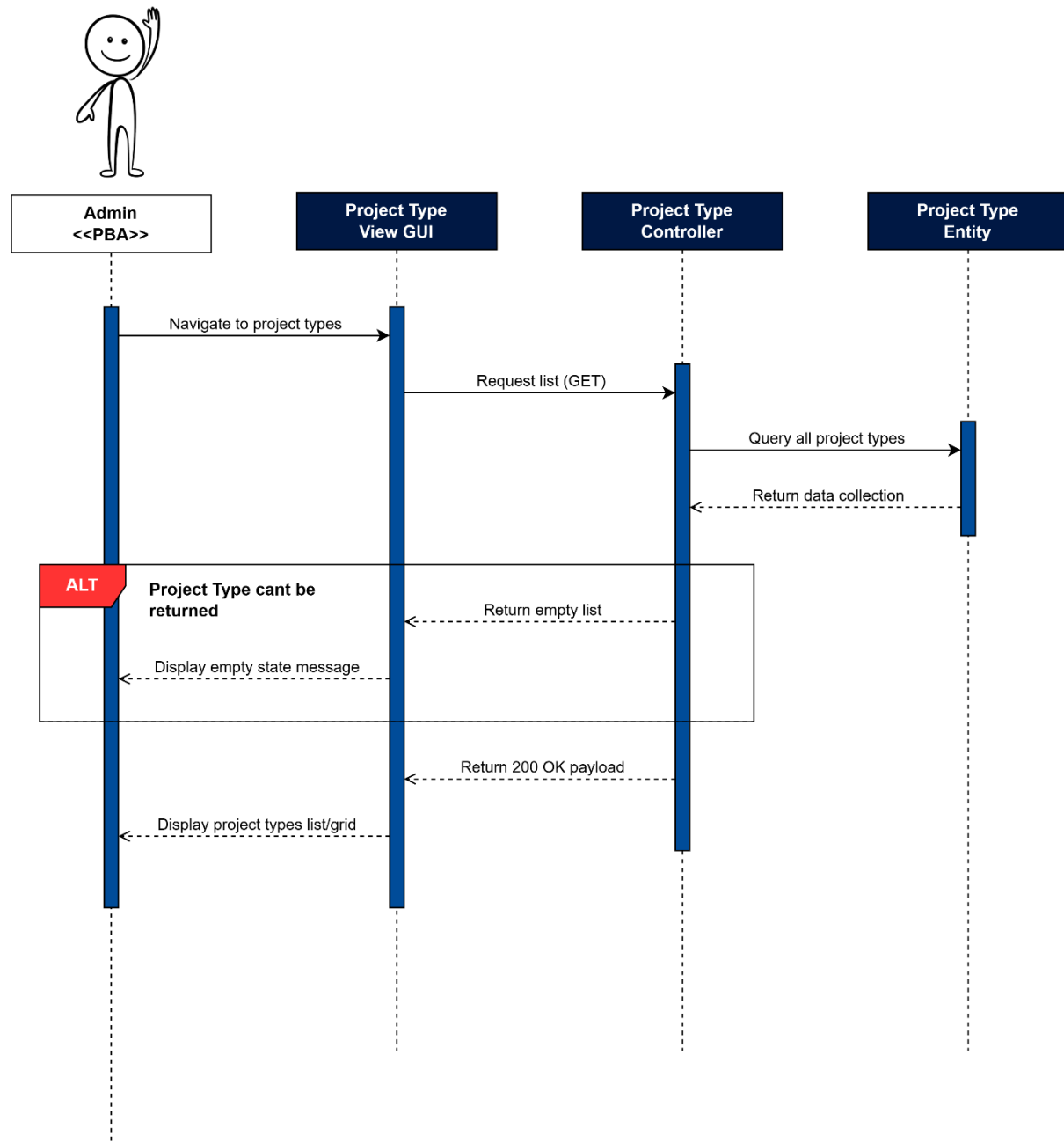
Figure 61: View Project Type Sequence Diagram
