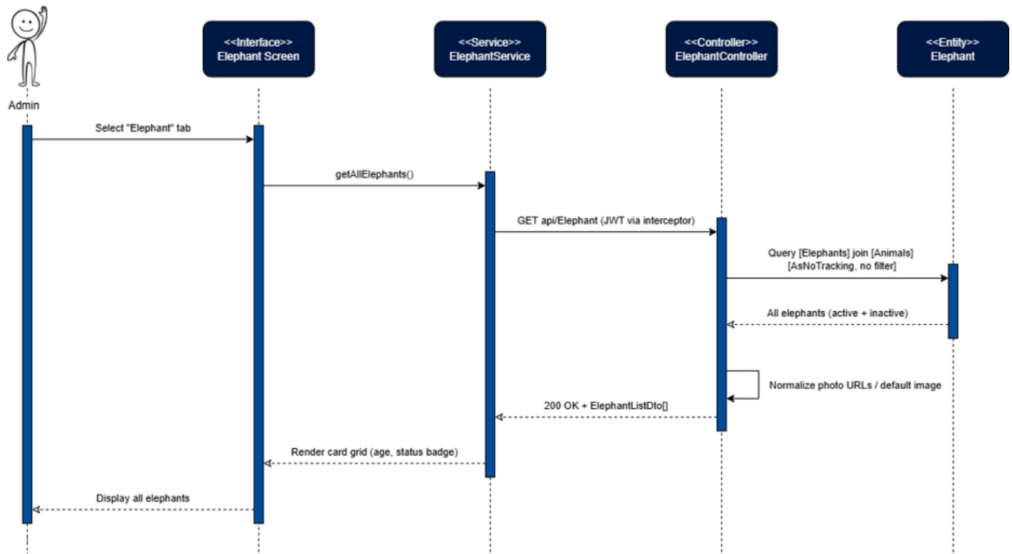
Figure 107: View Elephants Sequence Diagram
