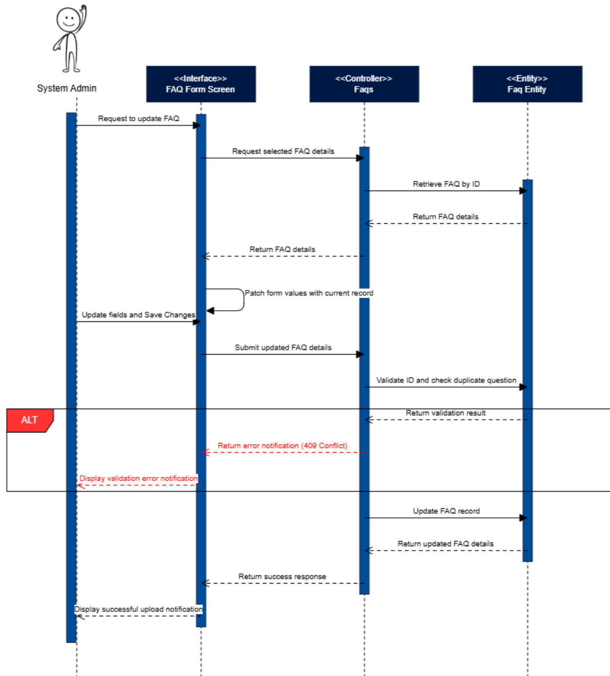
Figure 15: Update FAQ Sequence Diagram
