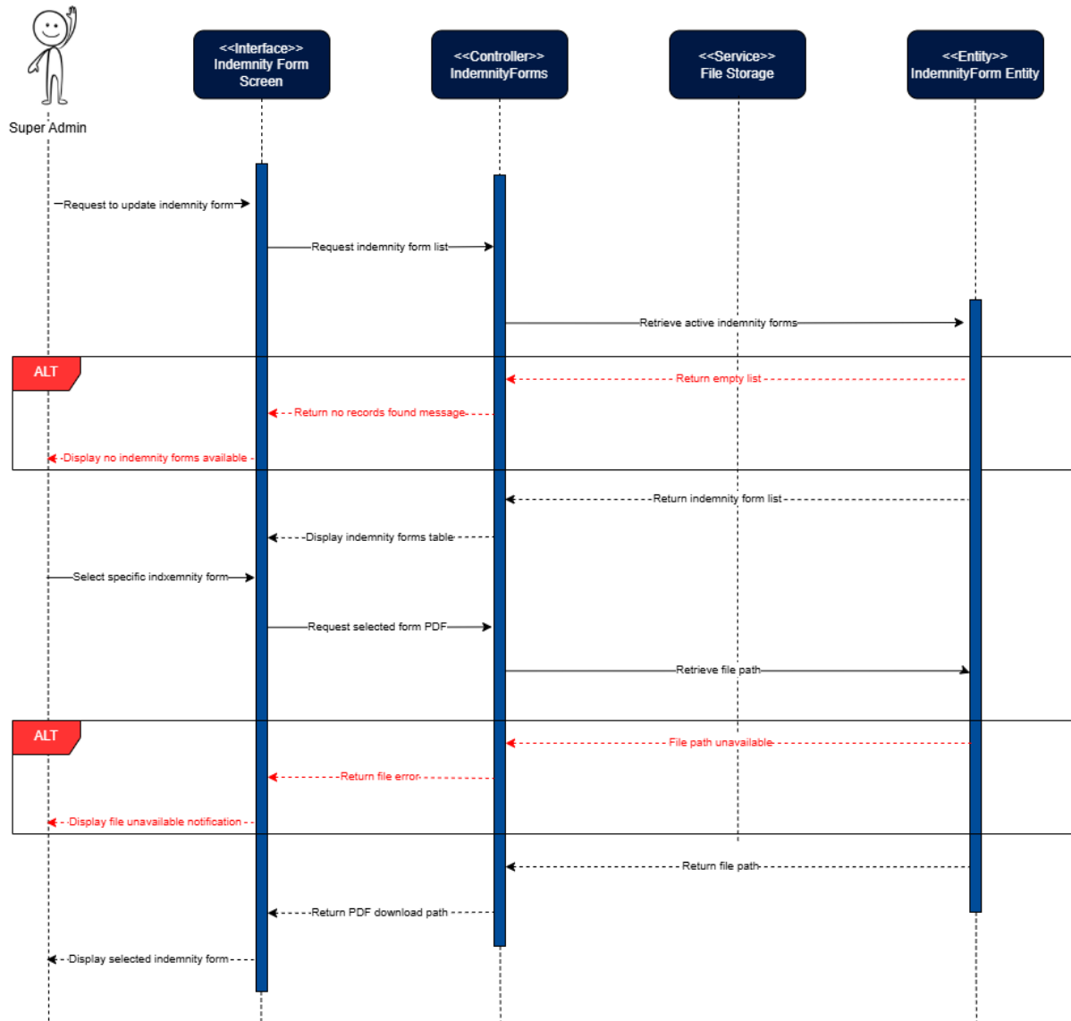
Figure 66: View Indemnity Form Sequence Diagram
