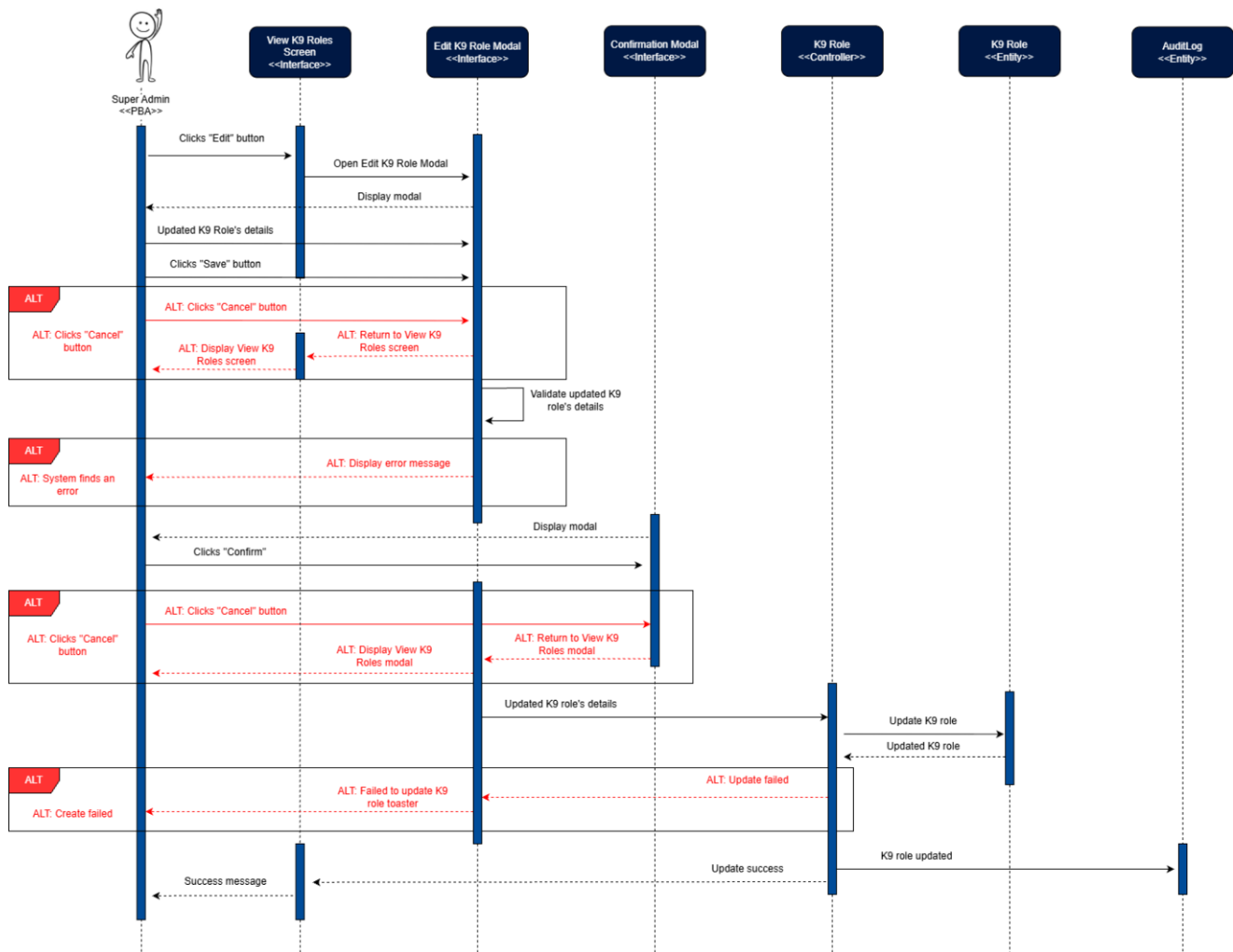
Figure 96: Update K9 Role Sequence Diagram
