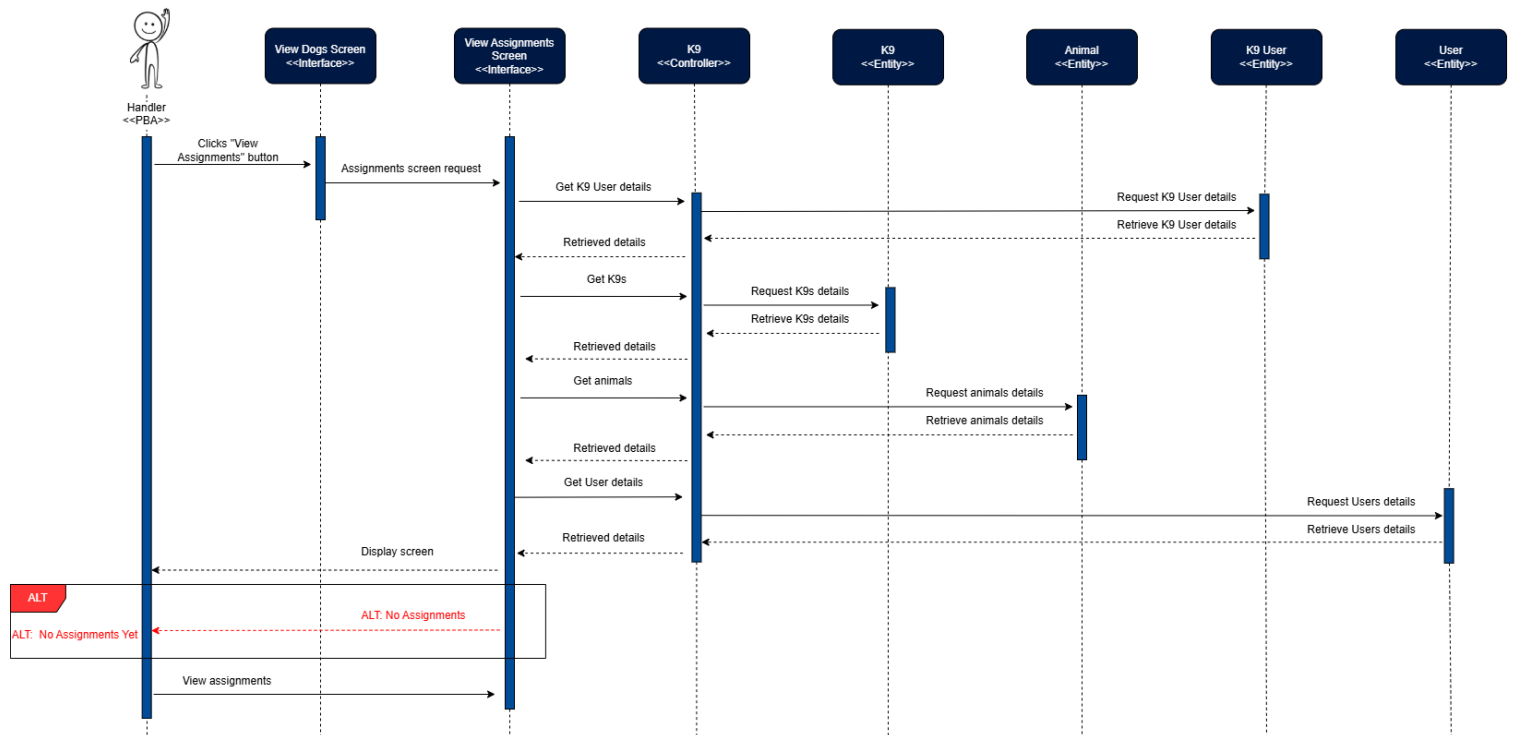
Figure 90: View User-Dog Assignment Sequence Diagram
