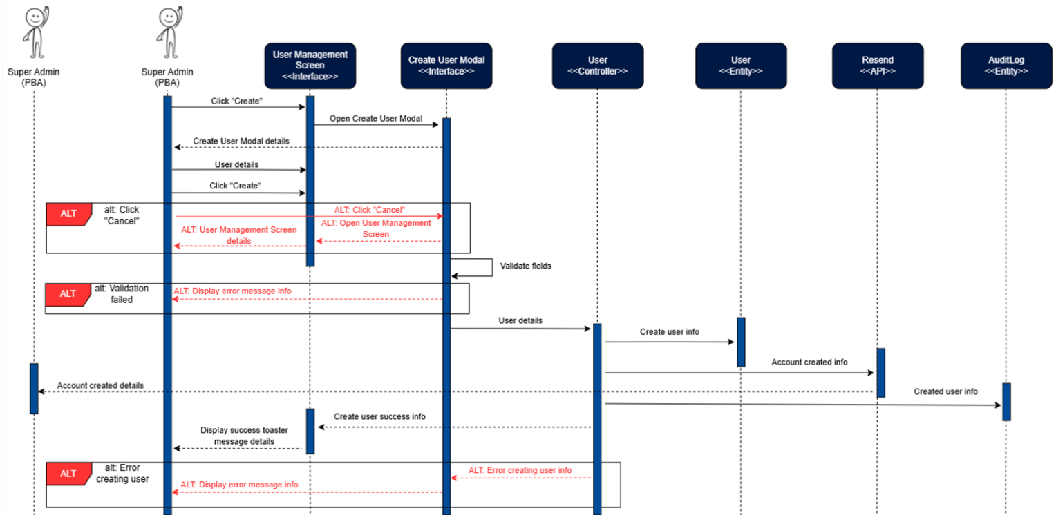
Figure 10: Create User Profile Sequence Diagram
