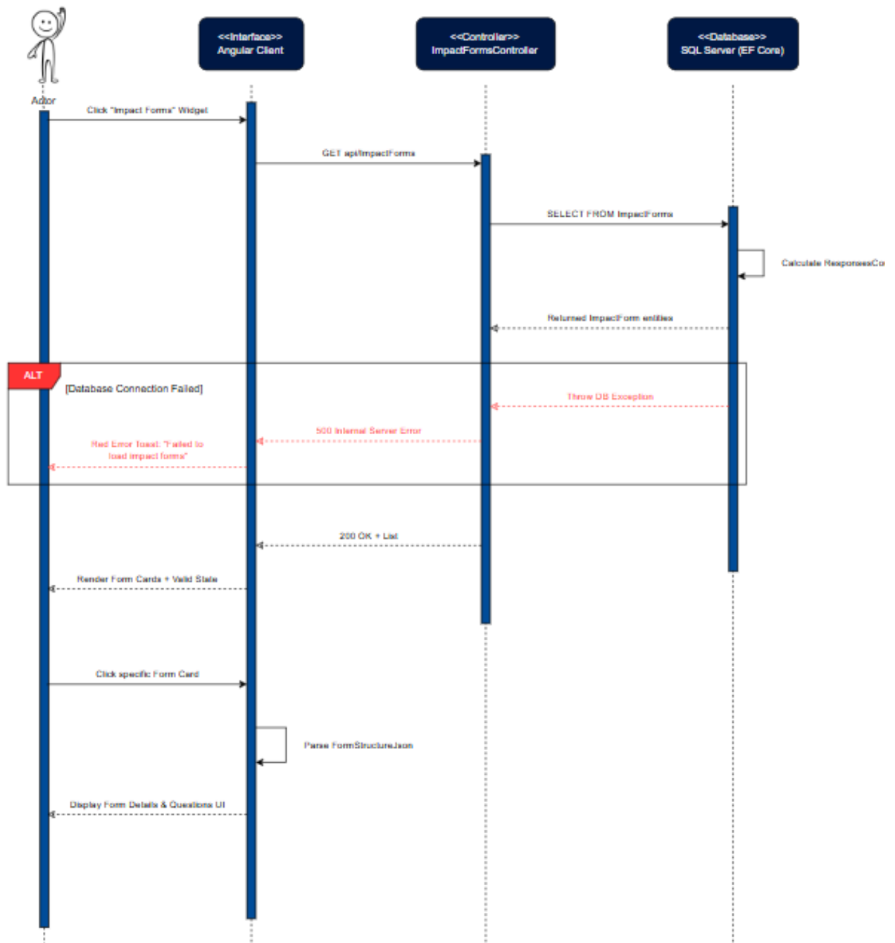
Figure 72: View Impact Feedback Form Sequence Diagram
