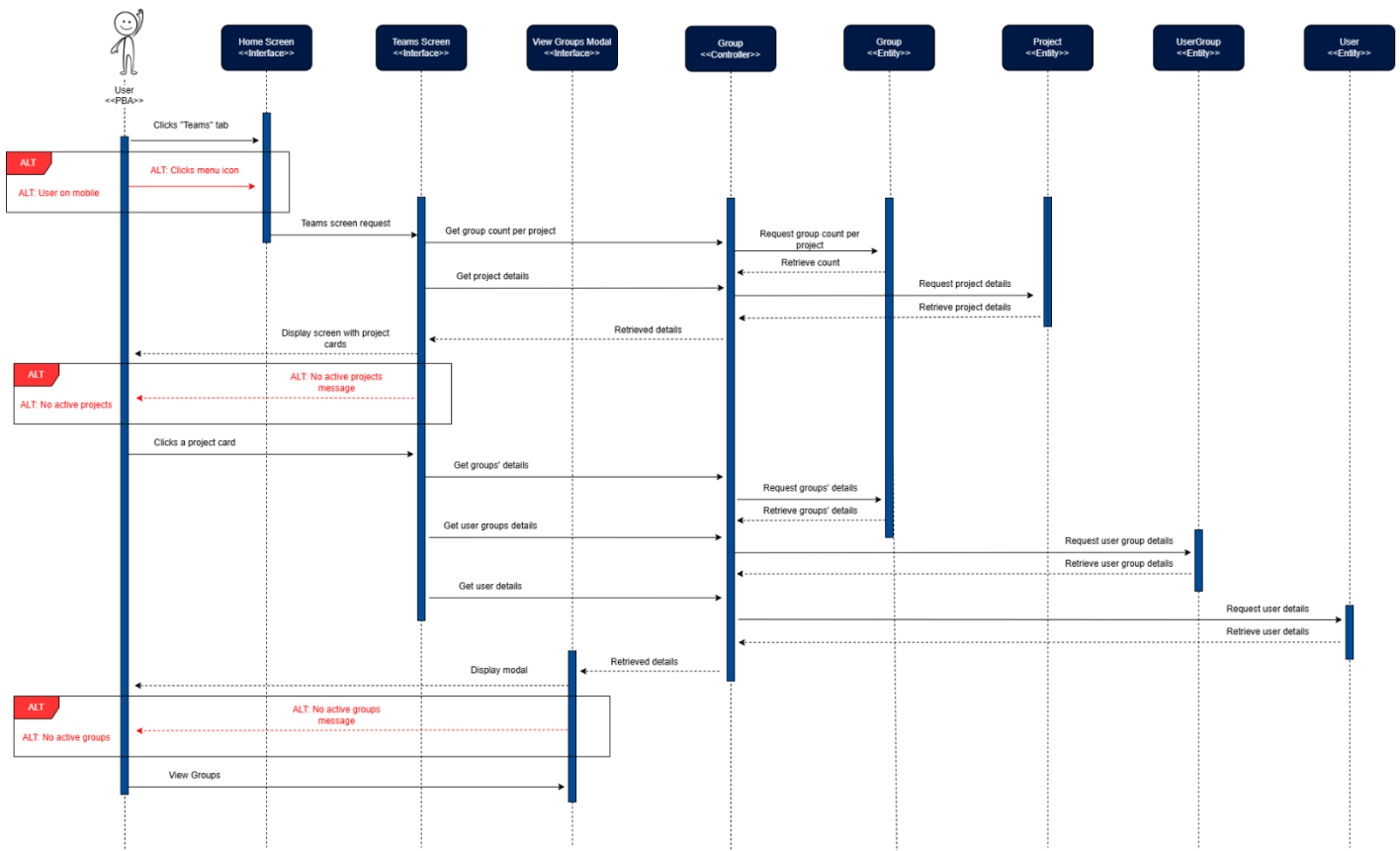
Figure 31: View Groups Sequence Diagram
