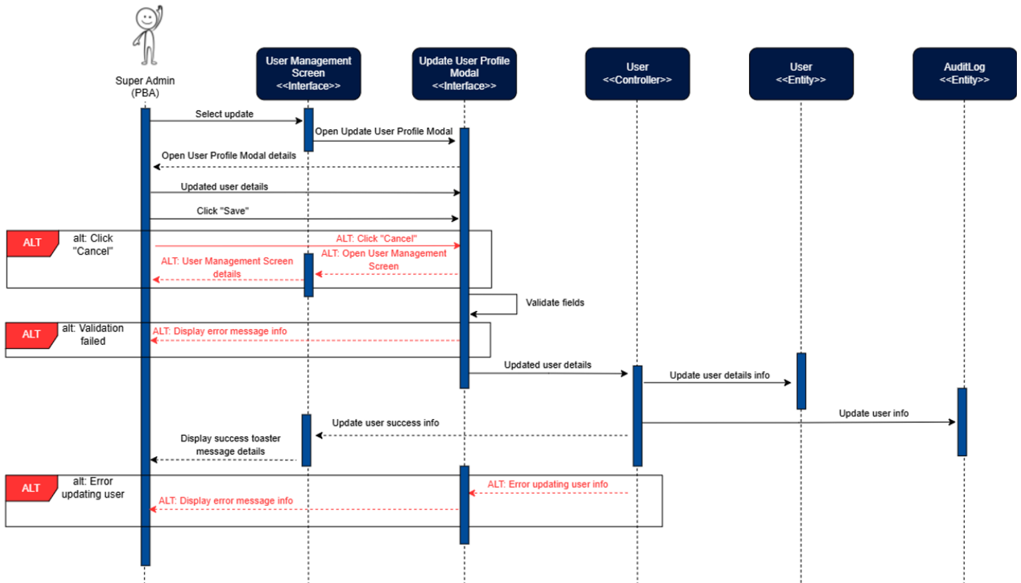
Figure 11: Update User Profile Sequence Diagram
