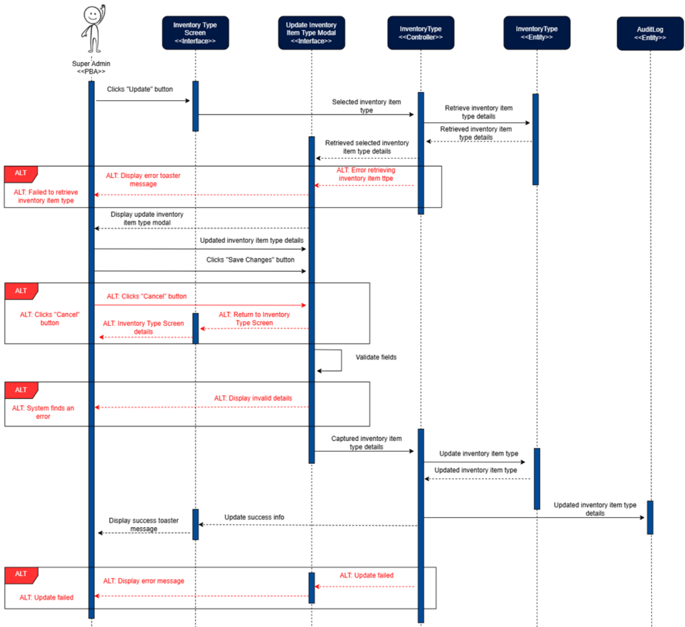
Figure 27: Update Inventory Item Type Sequence Diagram
