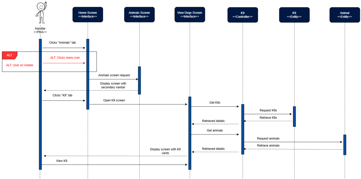
Figure 86: View Dogs Sequence Diagram
