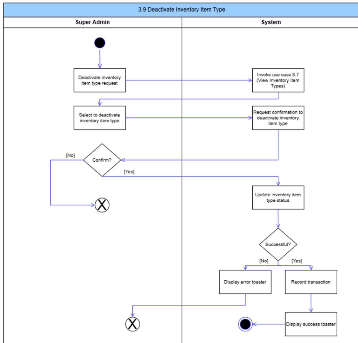
Figure 36: Deactivate Inventory Item Type
