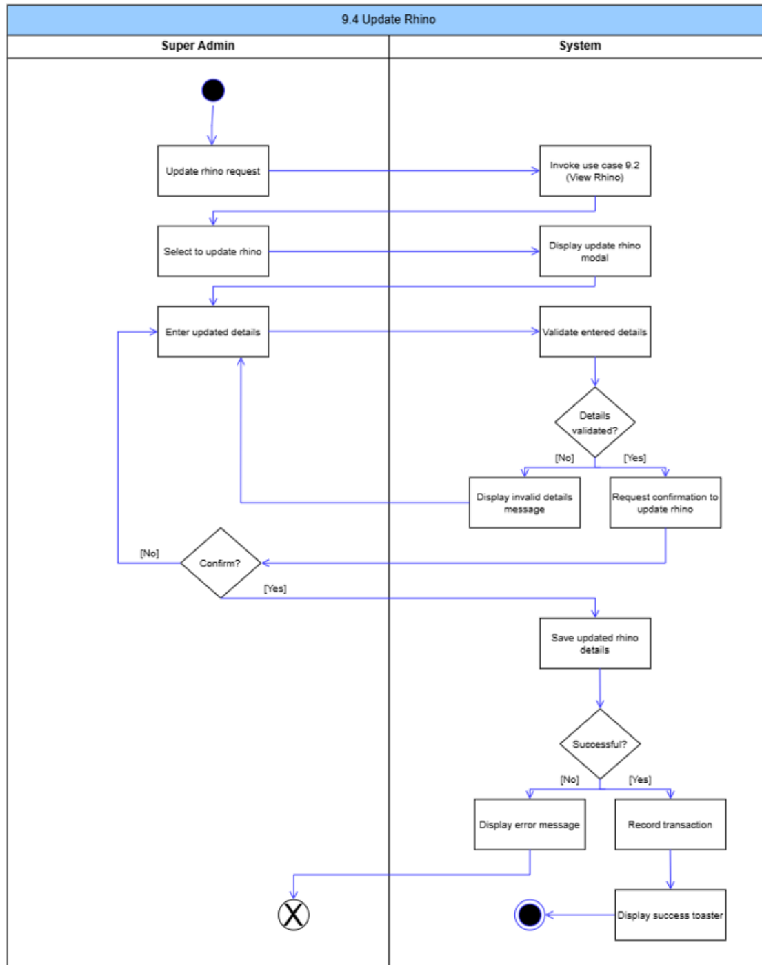
Figure 112: Update Rhino Activity Diagram
