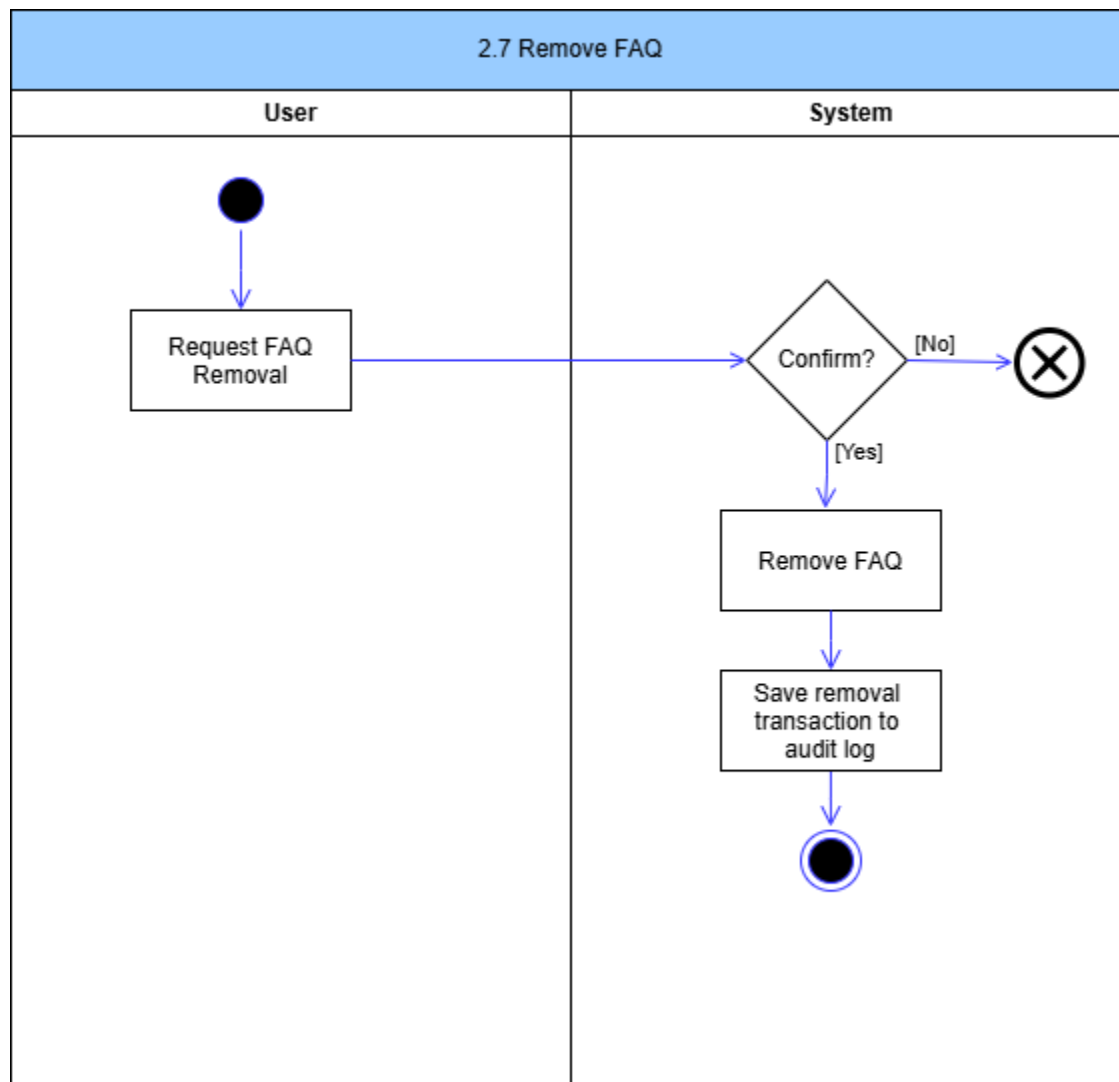
Figure 17: Remove FAQ Activity Diagram
