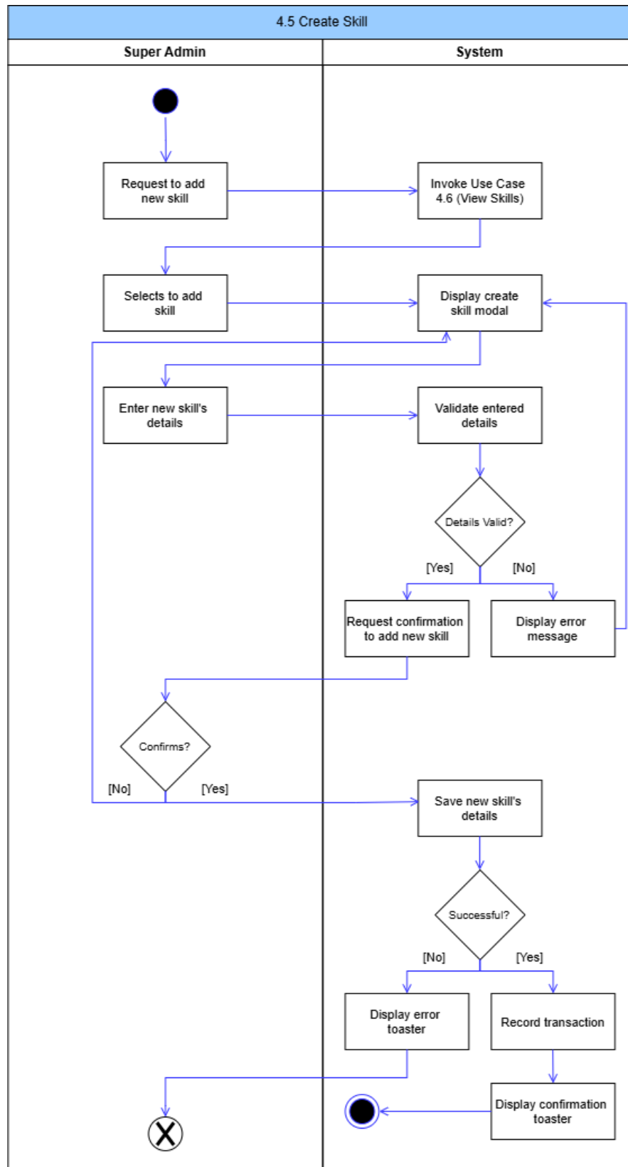
Figure 42: Create Skill Activity Diagram
