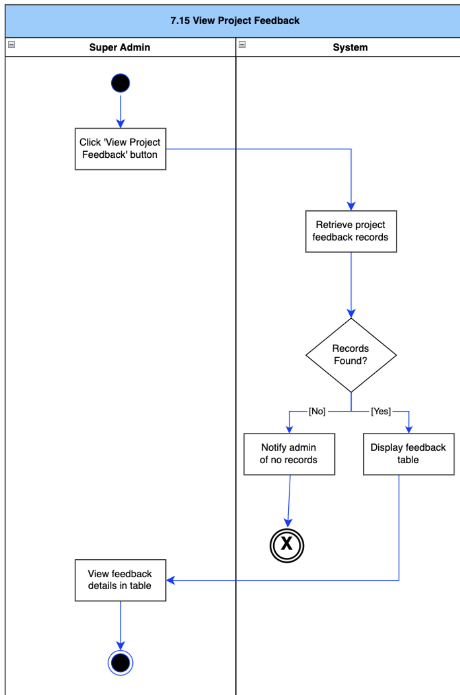
Figure 78: View Project Feedback Activity Diagram
