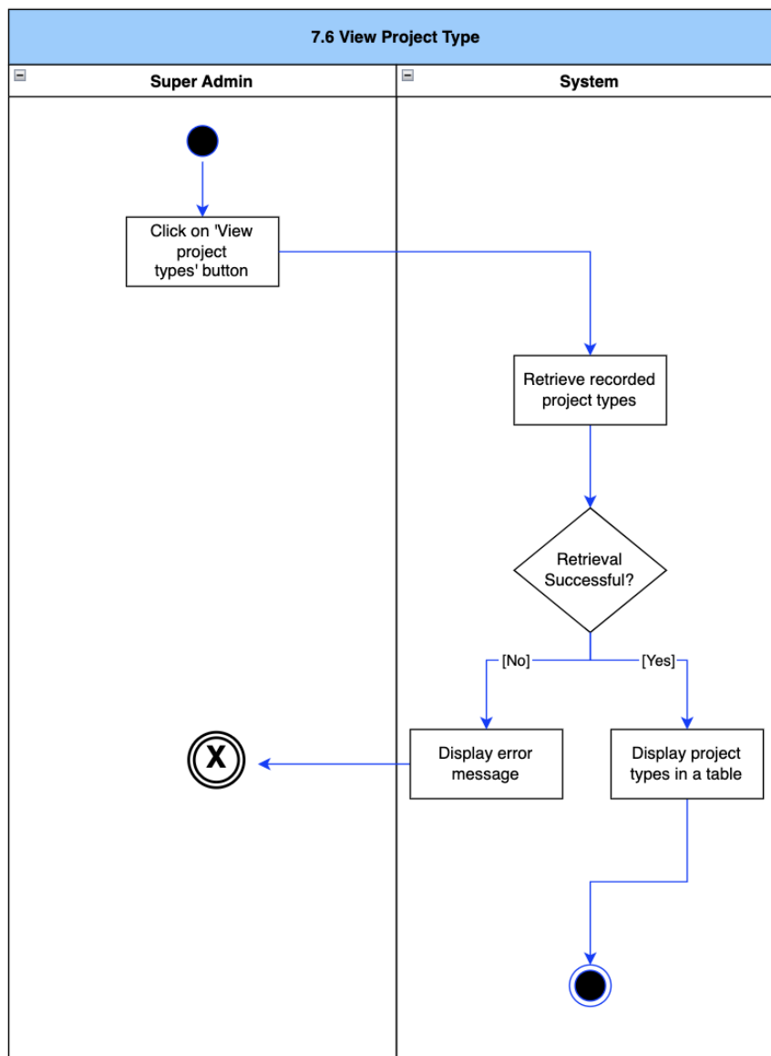
Figure 69: View Project Type Activity Diagram
