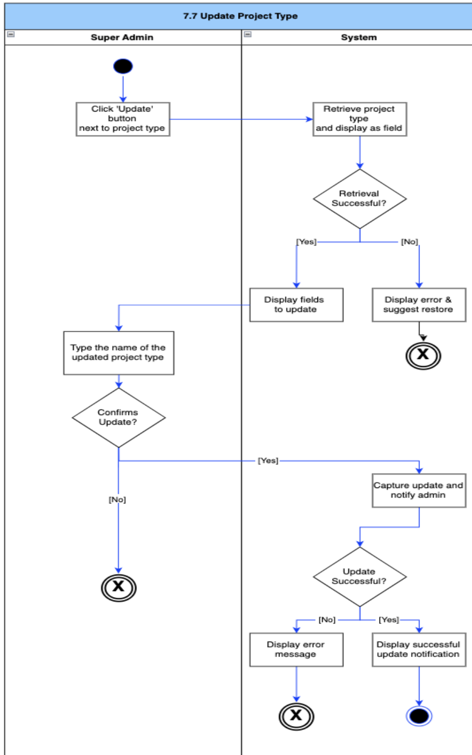
Figure 70: Update Project Type Activity Diagram
