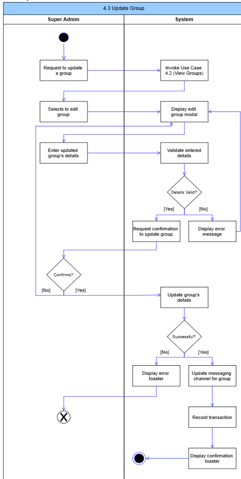
Figure 40: Update Group Activity Diagram
