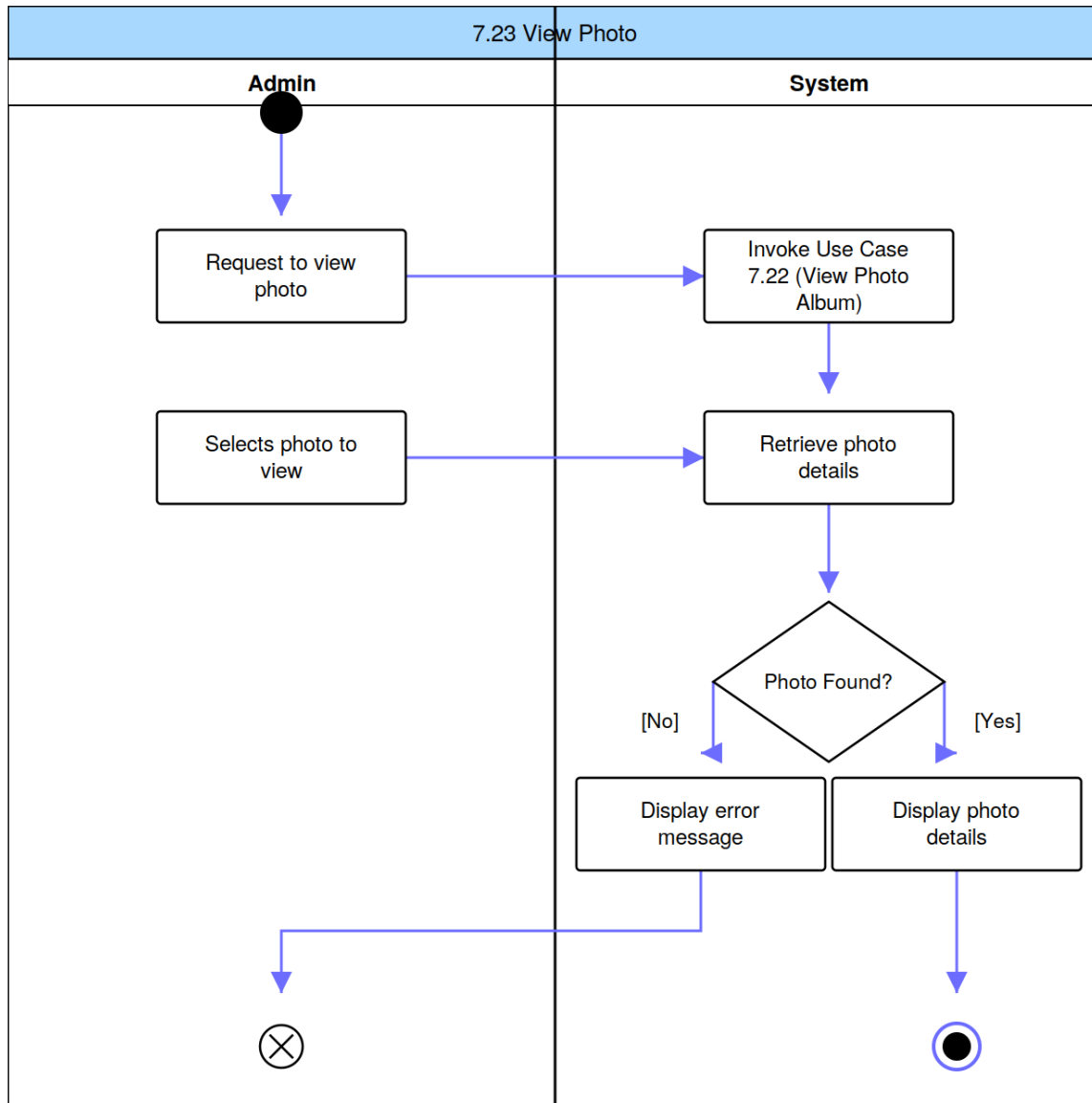
Figure 86: View Photo Activity Diagram
