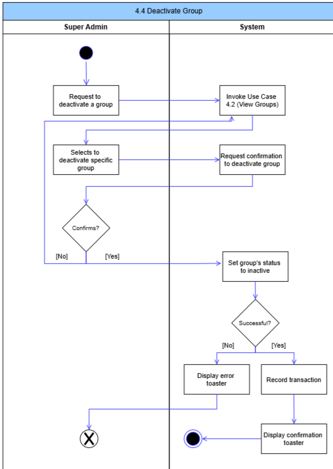
Figure 41: Deactivate Group Activity Diagram
