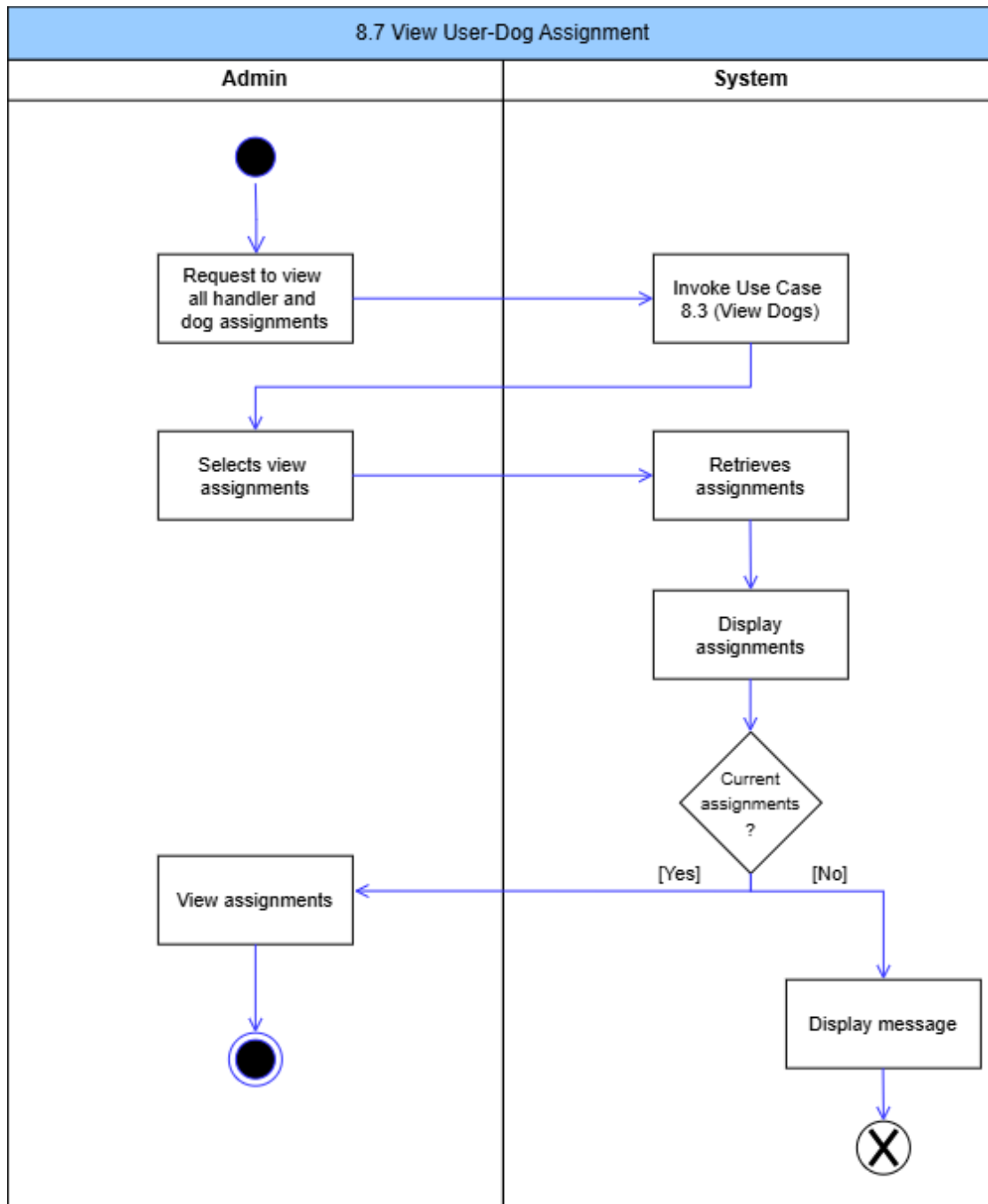
Figure 99: View User-Dog Assignment Activity Diagram
