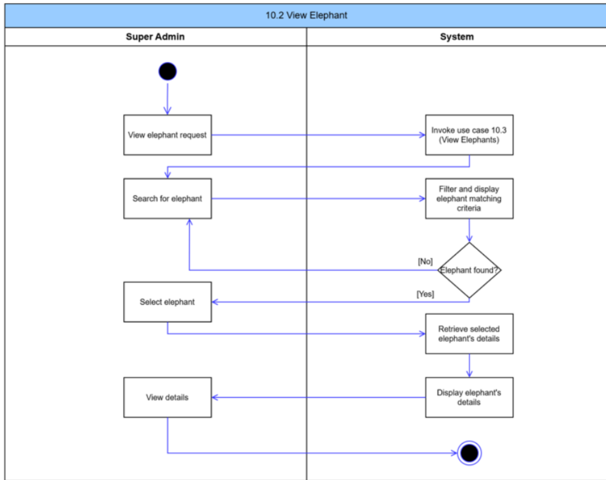
Figure 115: View Elephant Activity Diagram
