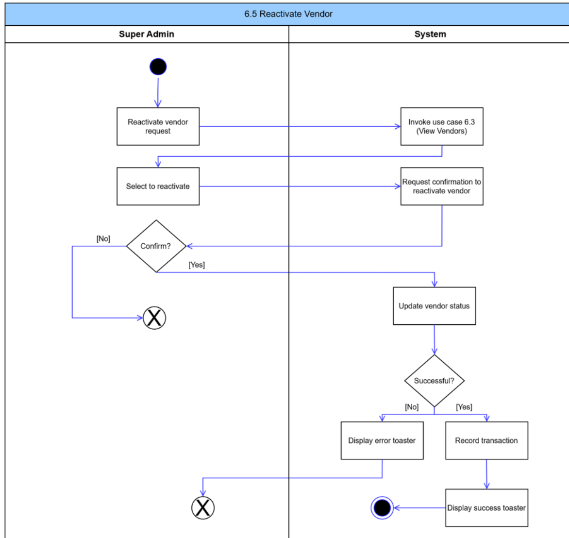
Figure 57: Reactivate Vendor Activity Diagram
