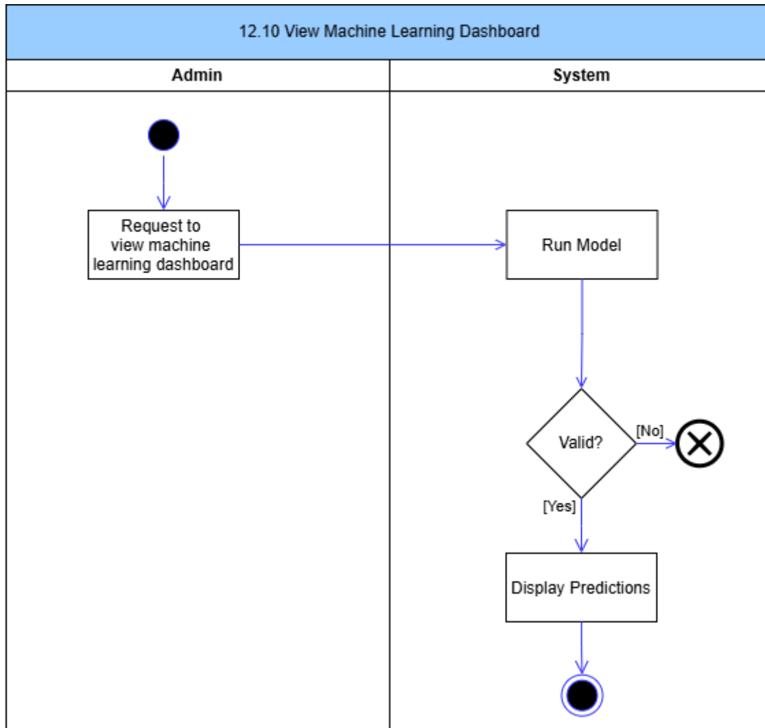
Figure 130: View Machine Learning Dashboard Activity Diagram
