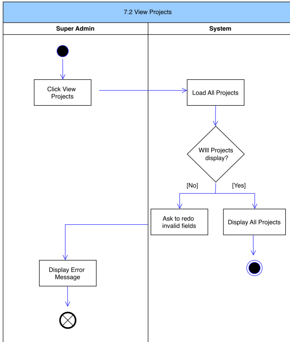
Figure 65: View Project Activity Diagram
