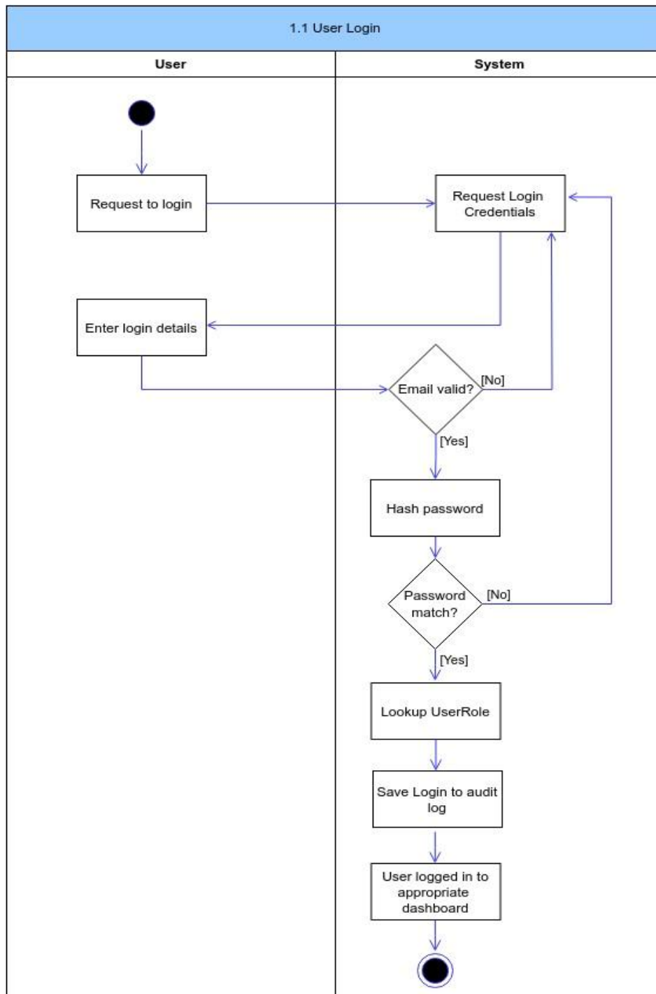
Figure 1: User Login Activity Diagram
