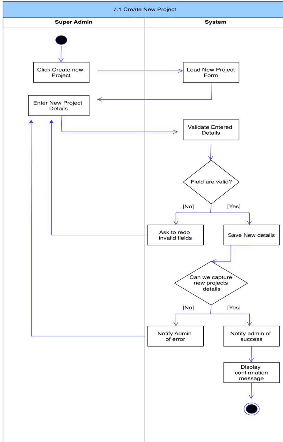
Figure 64: Create Project Activity Diagram
