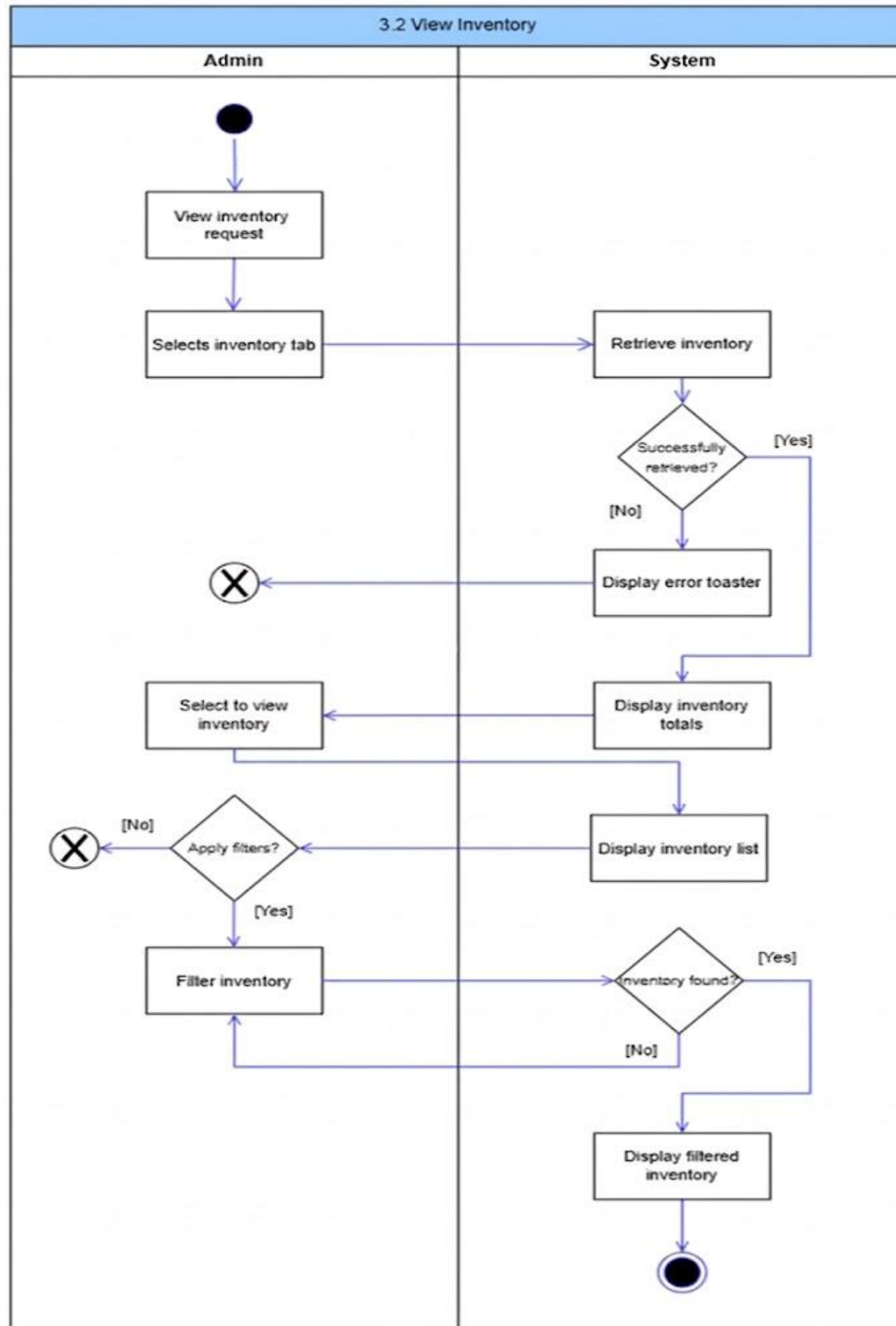
Figure 29: View Inventory Activity Diagram
