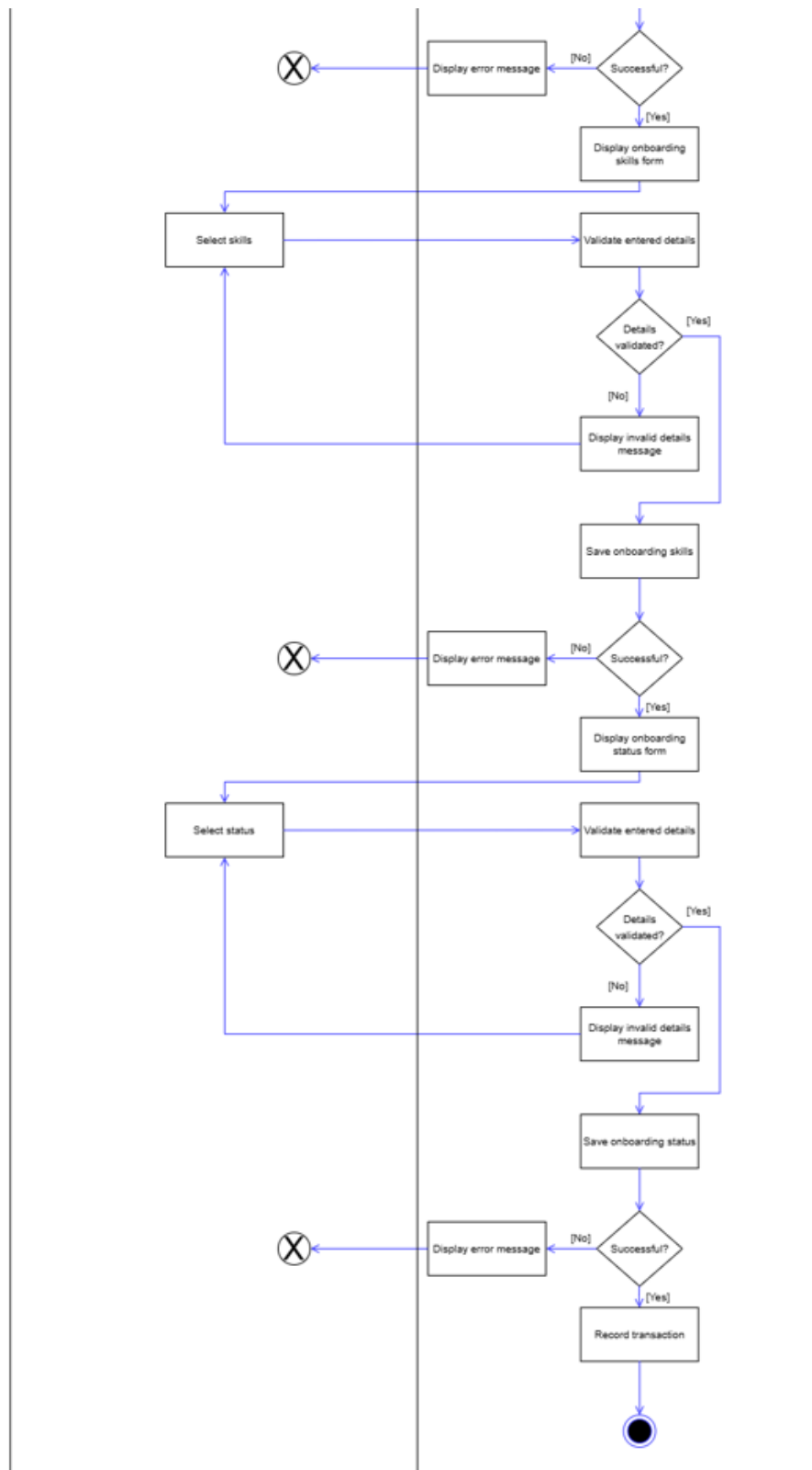
Figure 5: Create User Activity Diagram (Continued)
