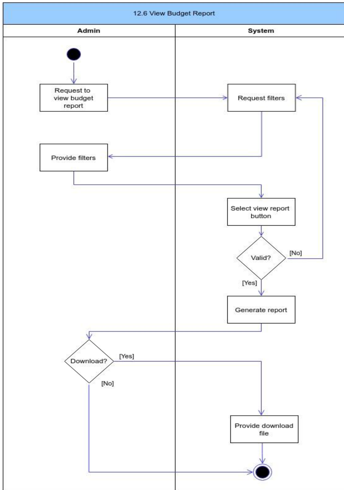
Figure 126: View Budget Report Activity Diagram
