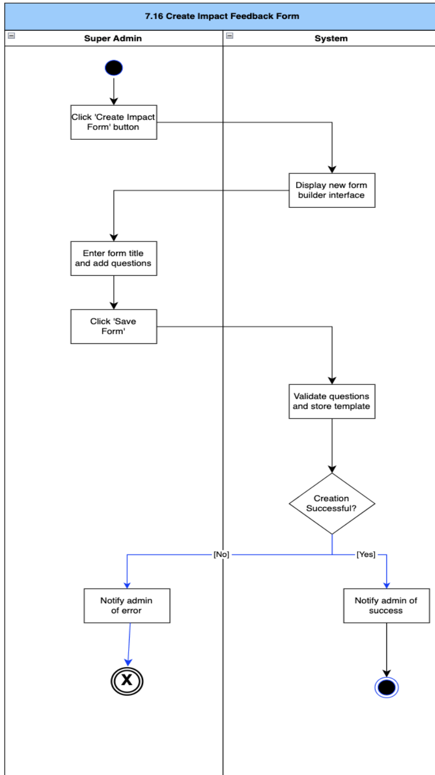
Figure 79: Create Impact Feedback Form Activity Diagram
