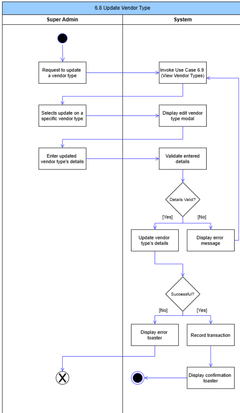
Figure 60: Update Vendor Type Activity Diagram
