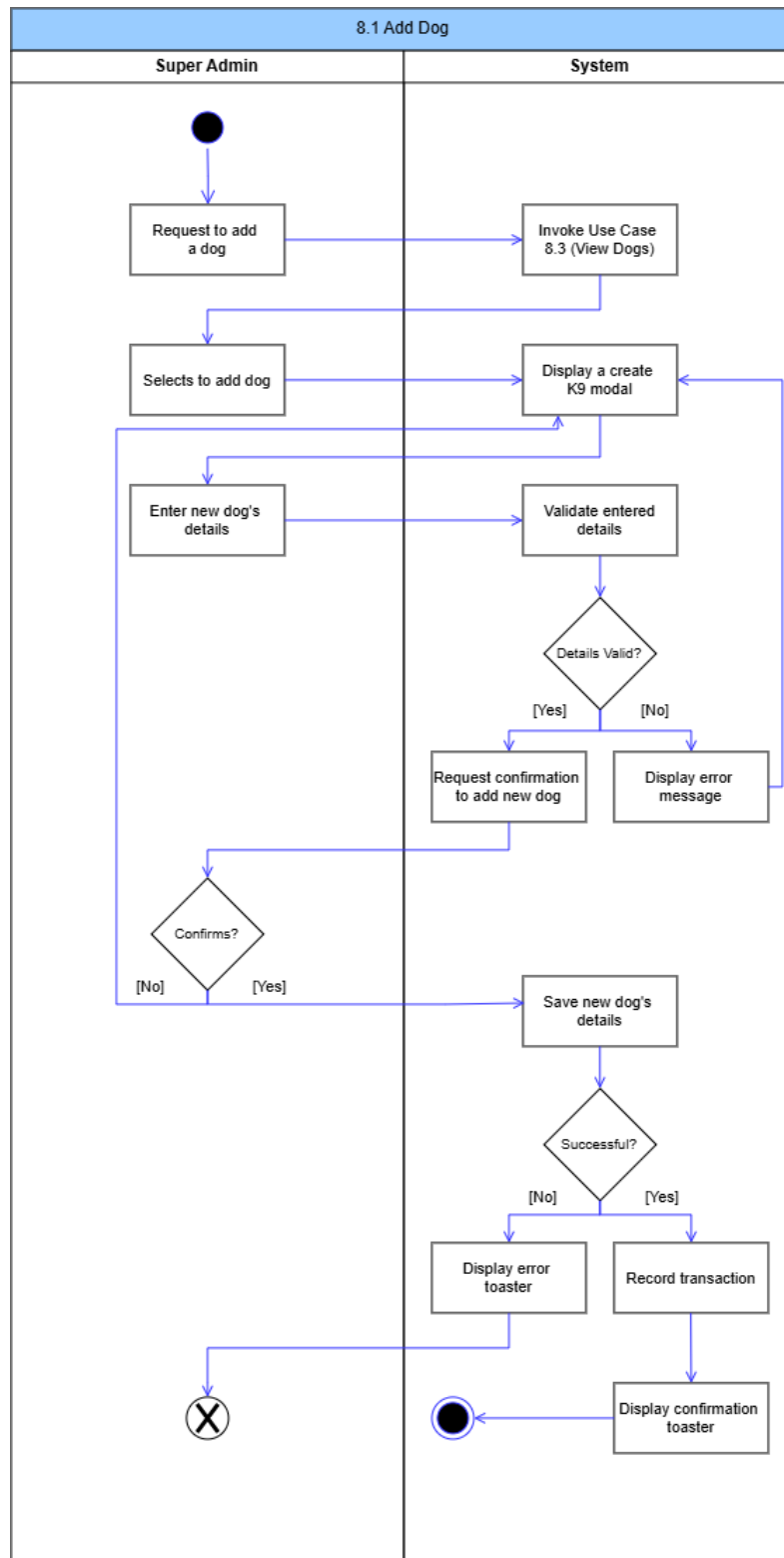
Figure 92: Add Dog Activity Diagram
