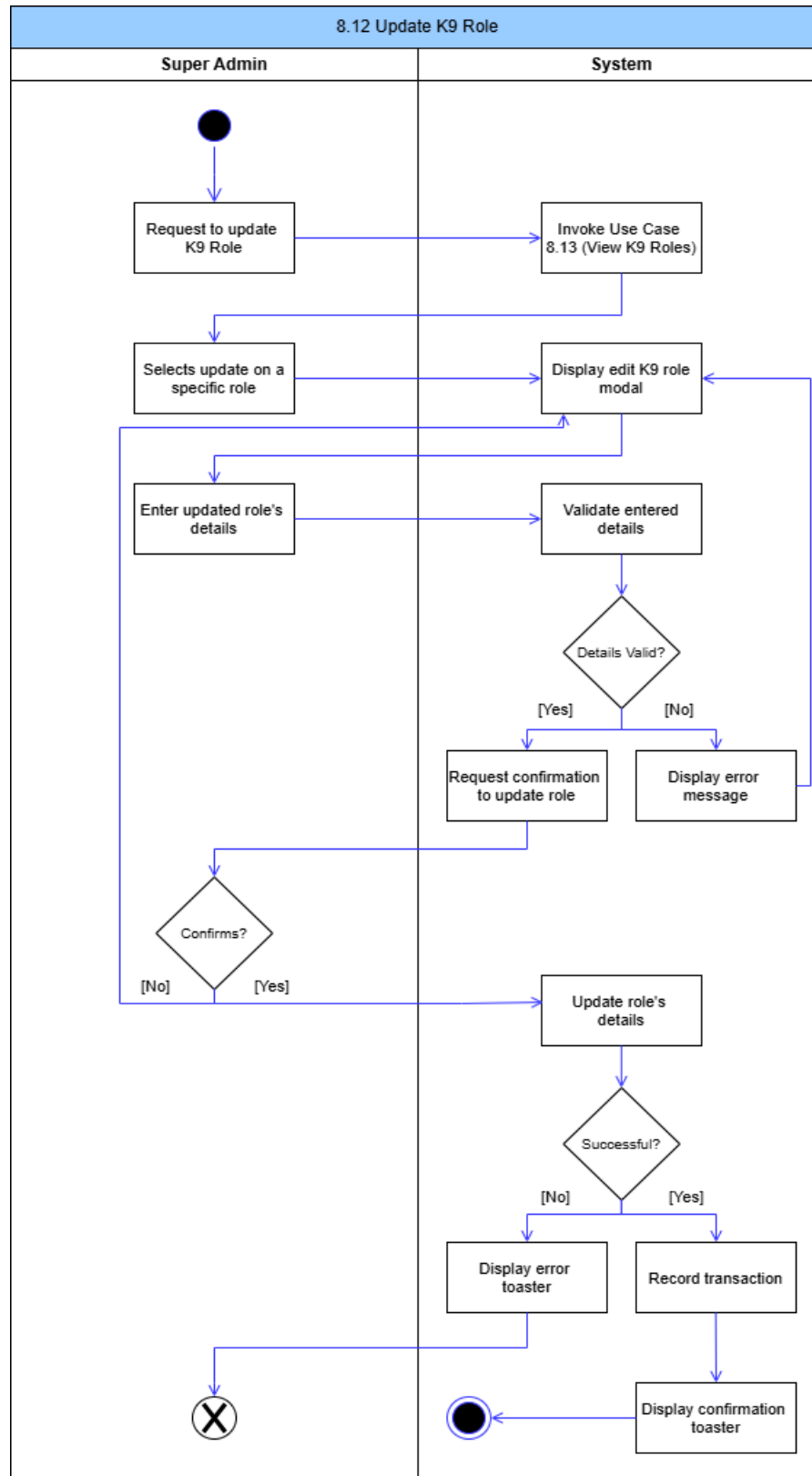
Figure 104: Update K9 Role Activity Diagram
