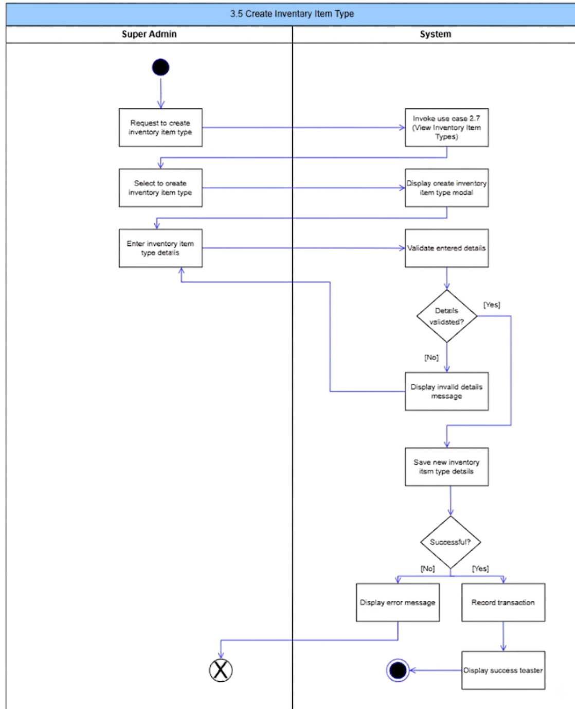
Figure 32: Create Inventory Item Type Activity Diagram
