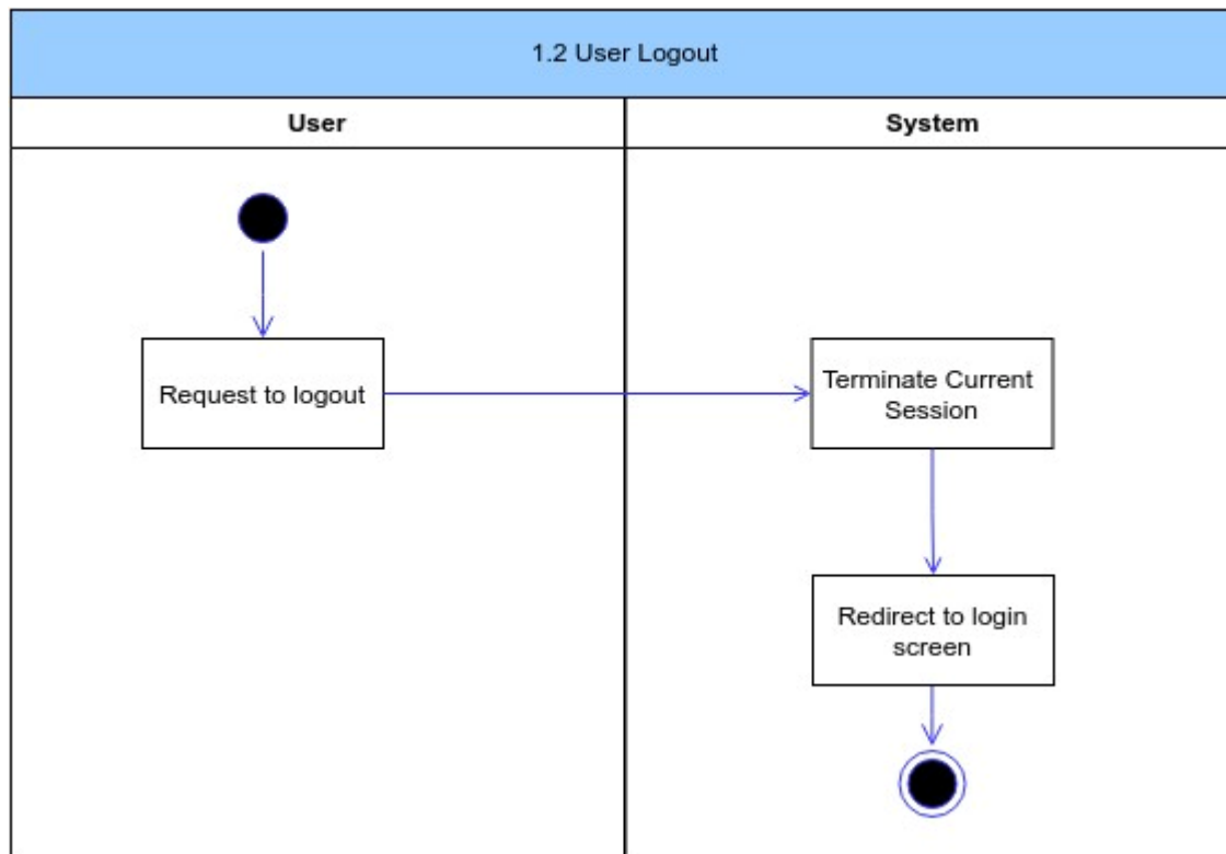
Figure 2: User Logout Activity Diagram
