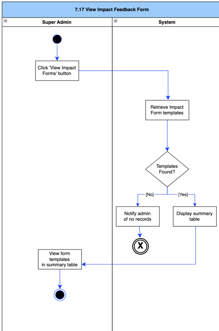
Figure 80: View Impact Feedback Form Activity Diagram
