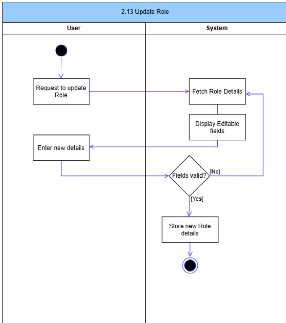
Figure 23: Update Role Activity Diagram
