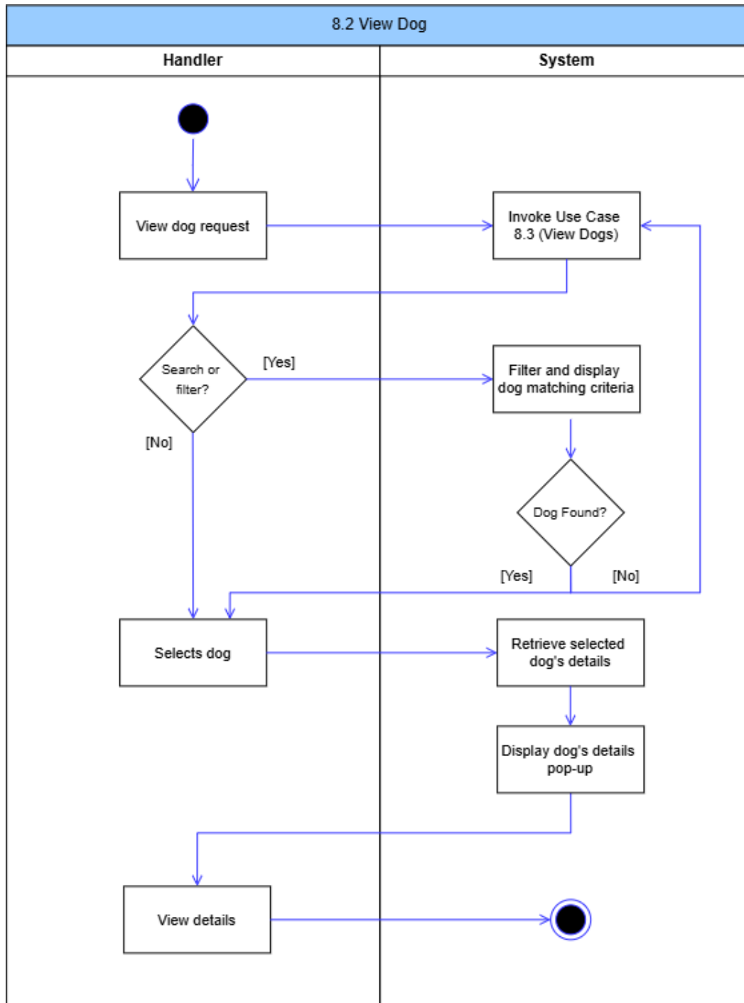
Figure 93: View Dog Activity Diagram
