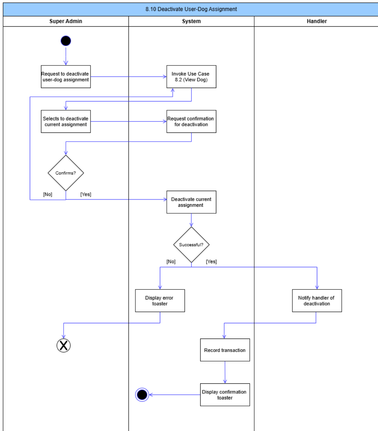
Figure 102: Deactivate User-Dog Assignment Activity Diagram
