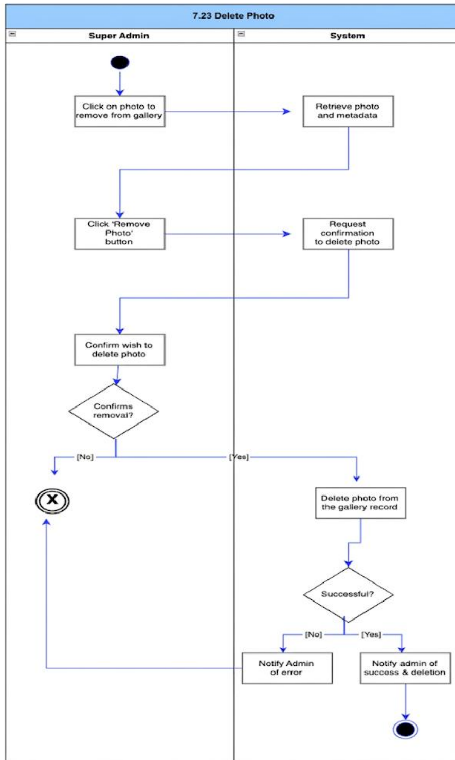
Figure 87: Delete Photo Activity Diagram
