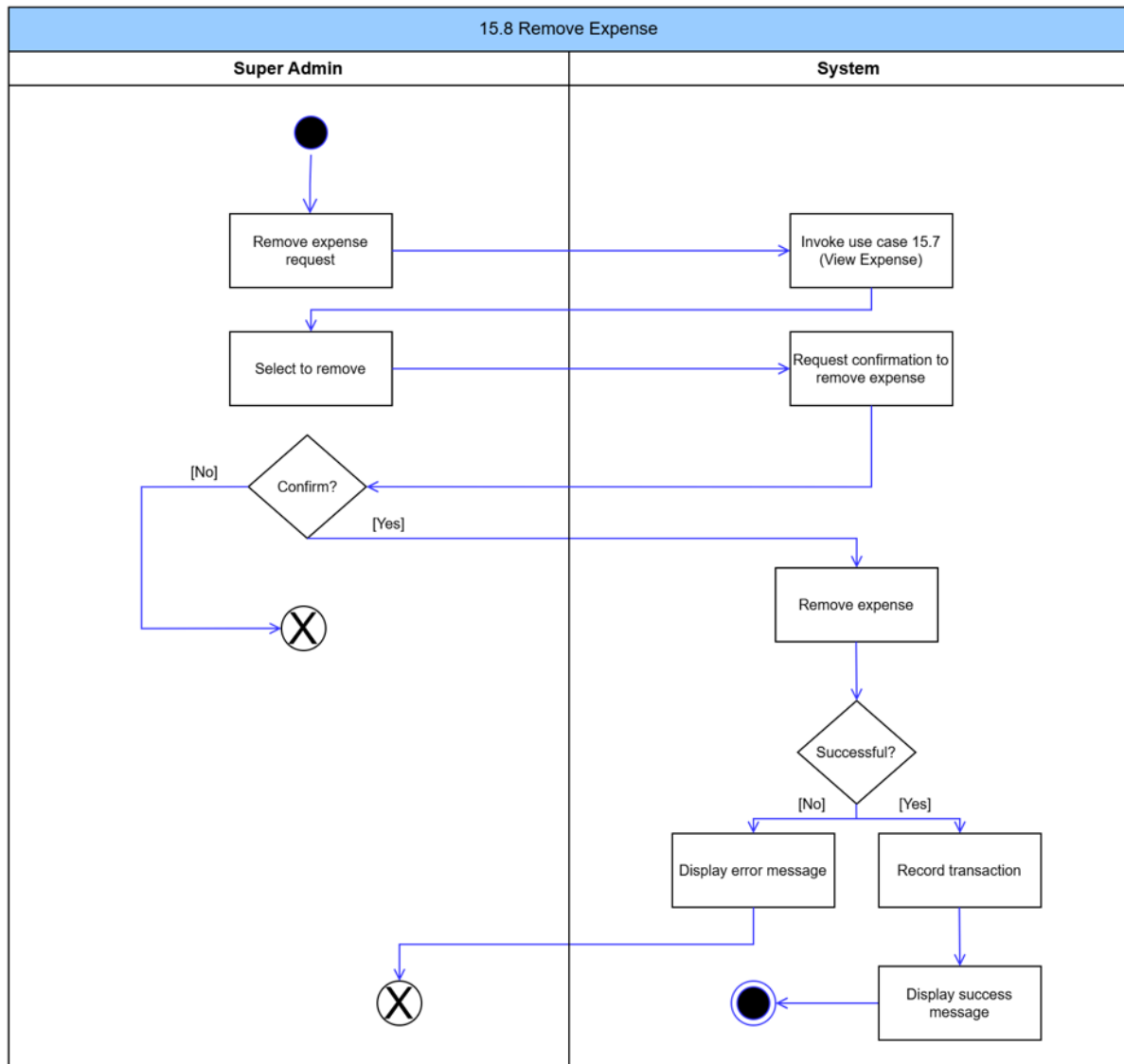
Figure 139: Remove Expense Activity Diagram
