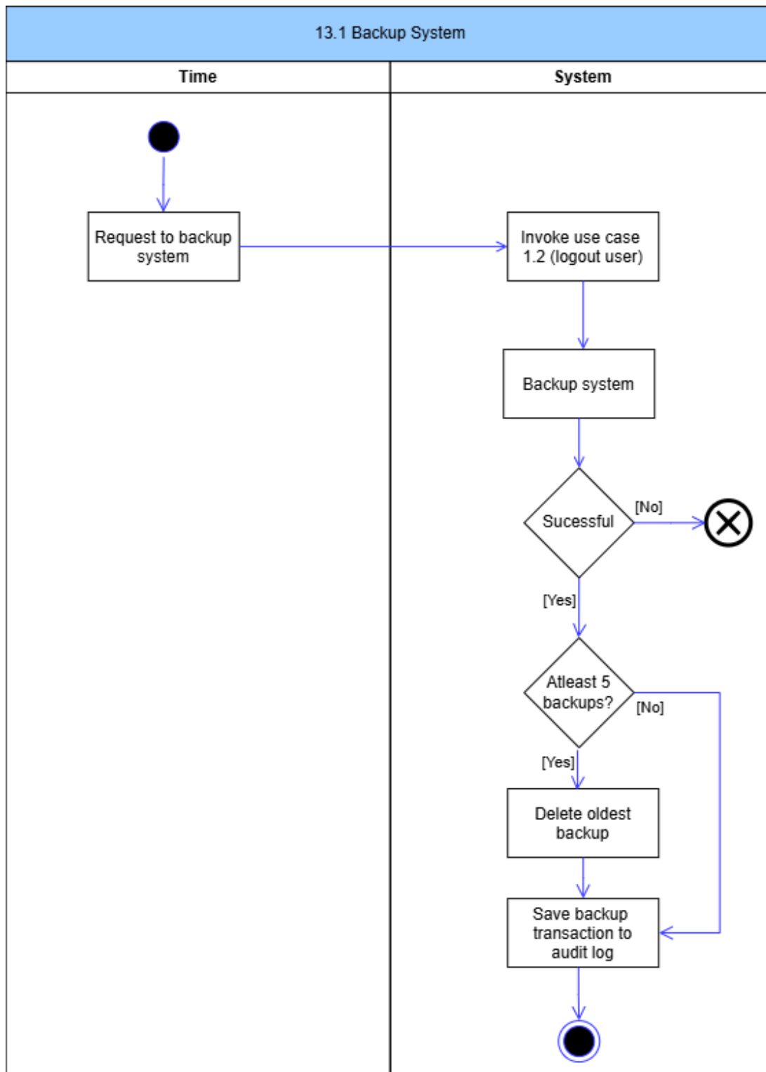
Figure 131: Backup System Activity Diagram
