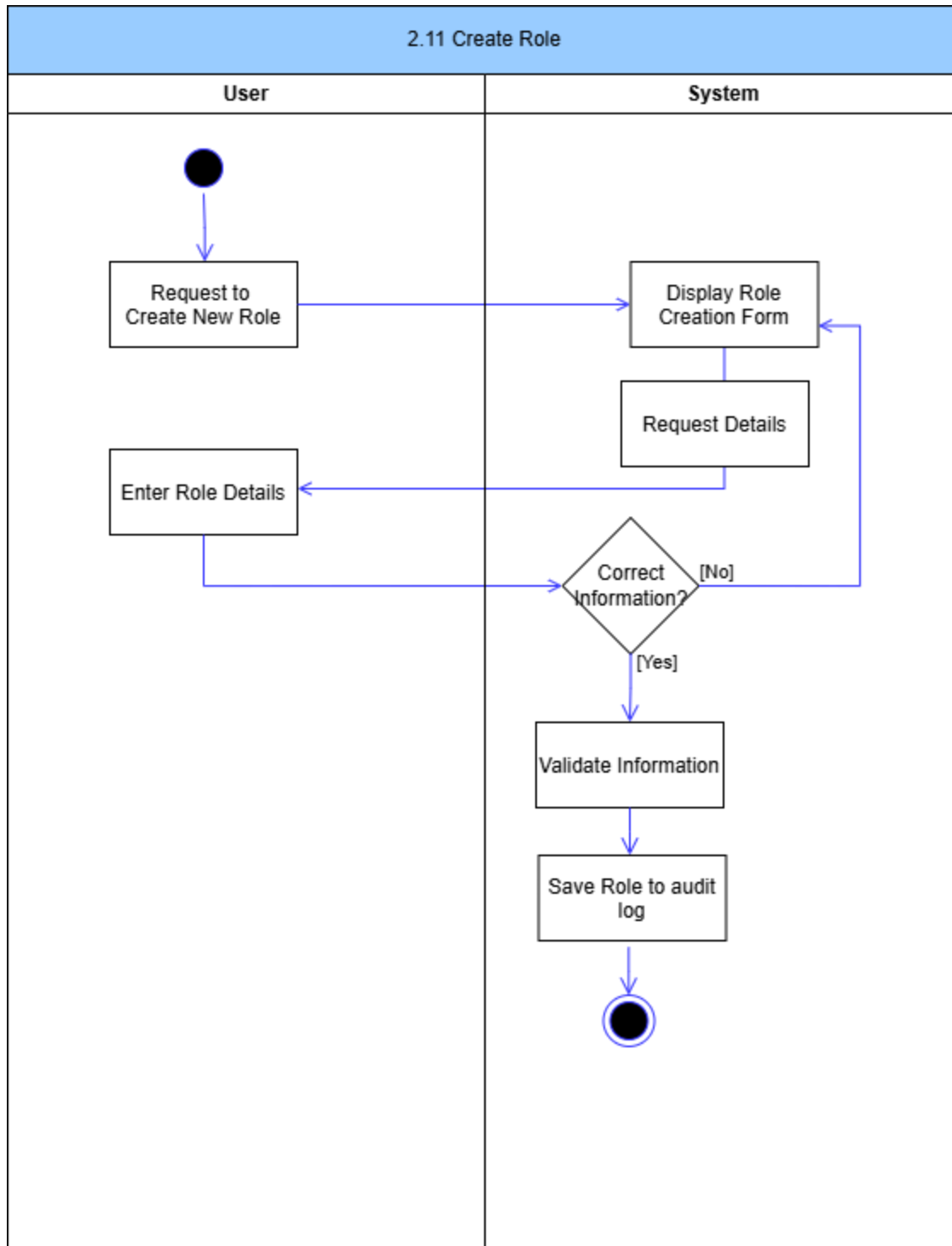
Figure 21: Create Role Activity Diagram
