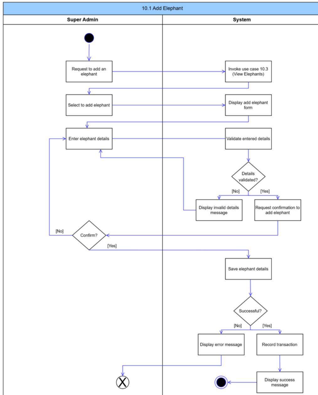
Figure 114: Add Elephant Activity Diagram
