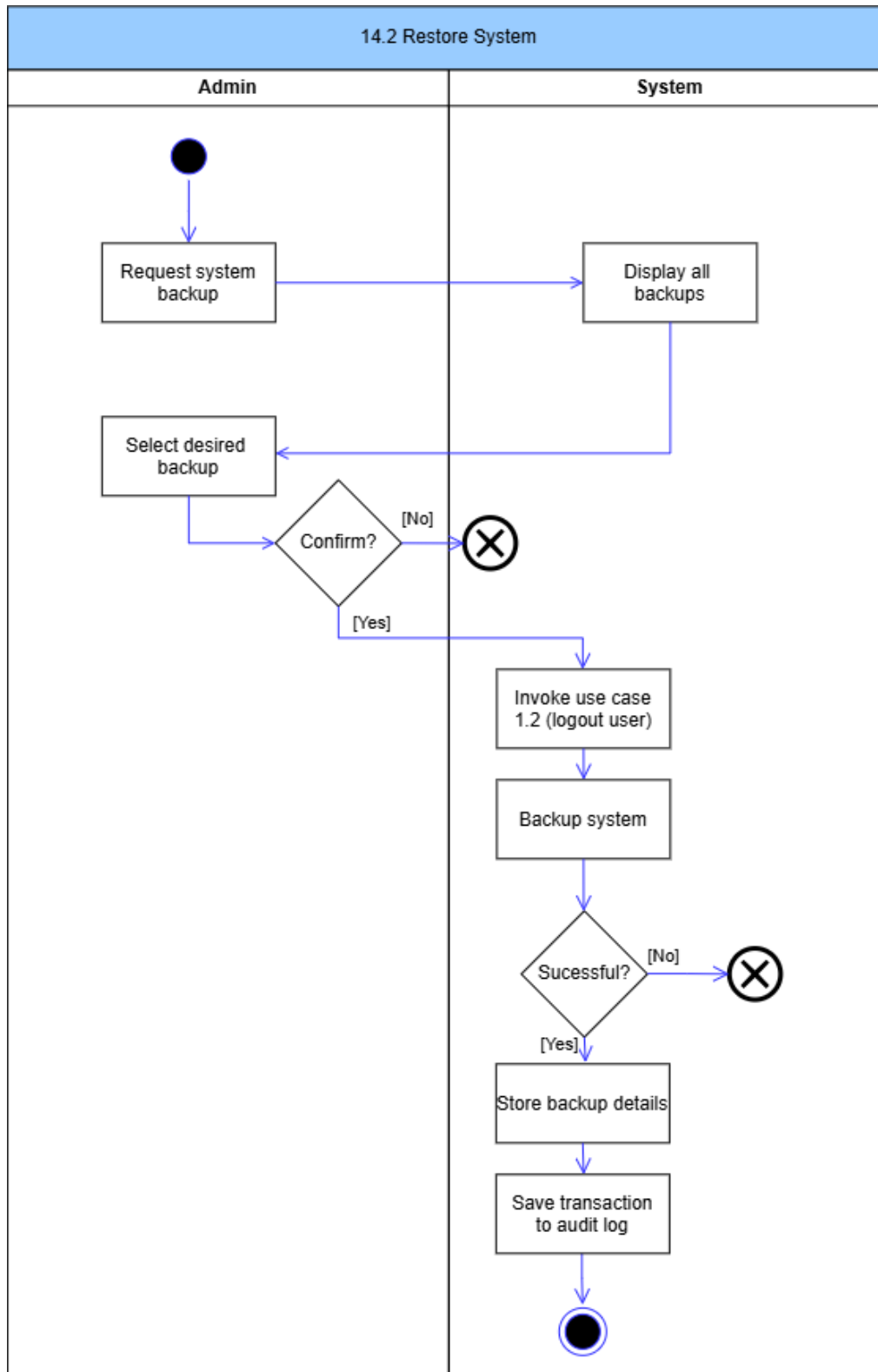
Figure 132: Restore system Activity Diagram
