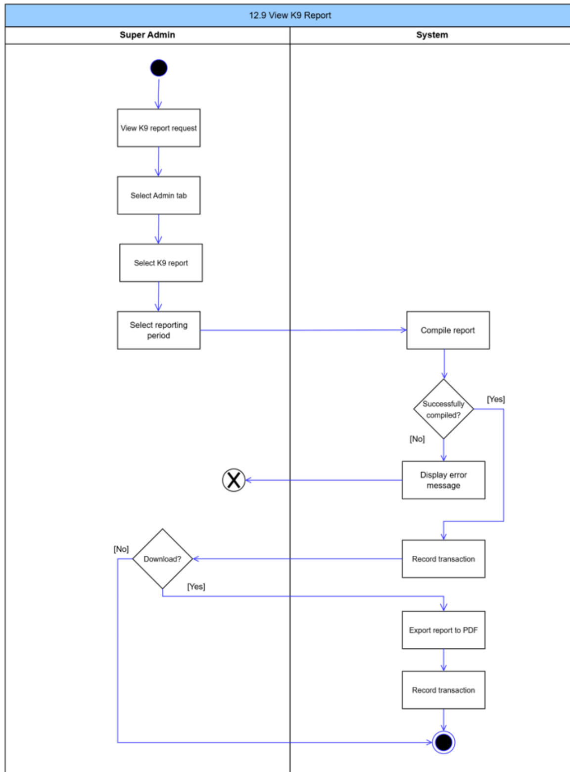
Figure 129: View K9 Report Activity Diagram
