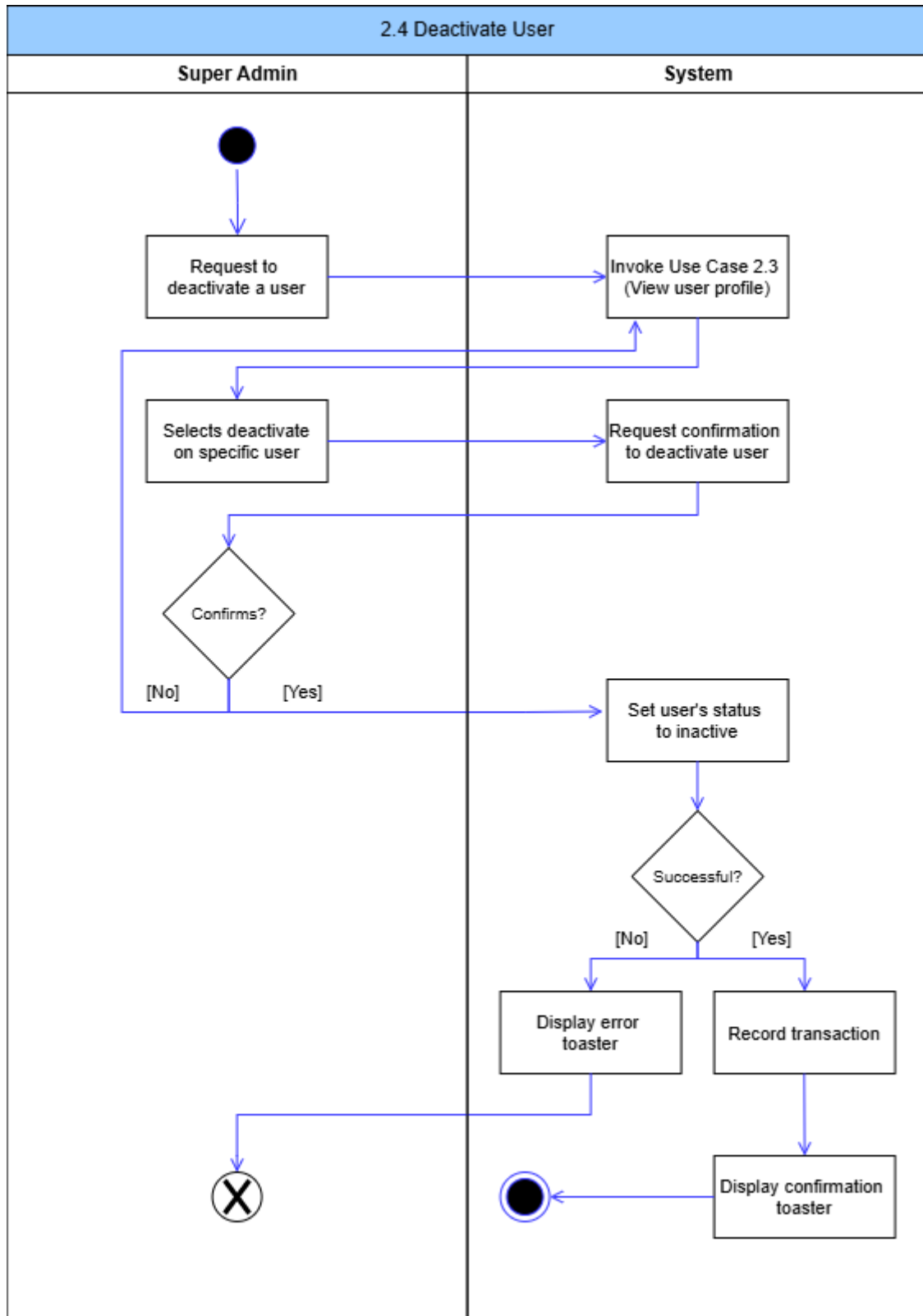
Figure 14: Deactivate User Activity Diagram
