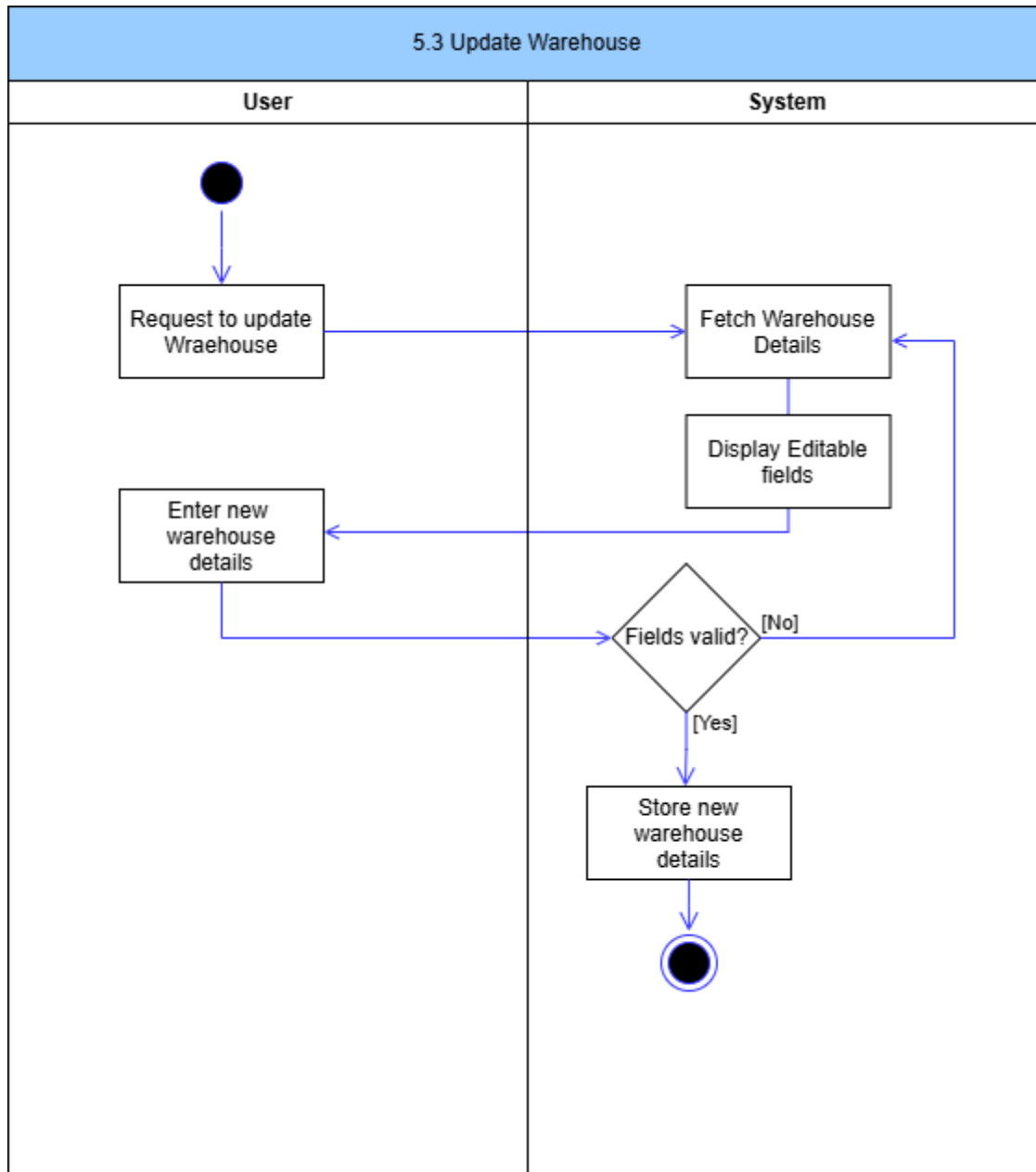
Figure 49: Update Warehouse Activity Diagram
