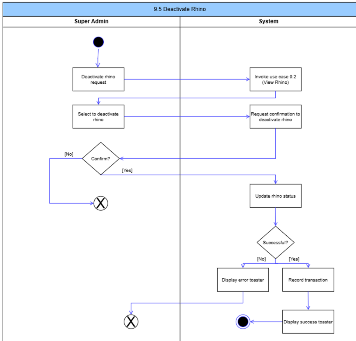
Figure 113: Deactivate Rhino Activity Diagram
