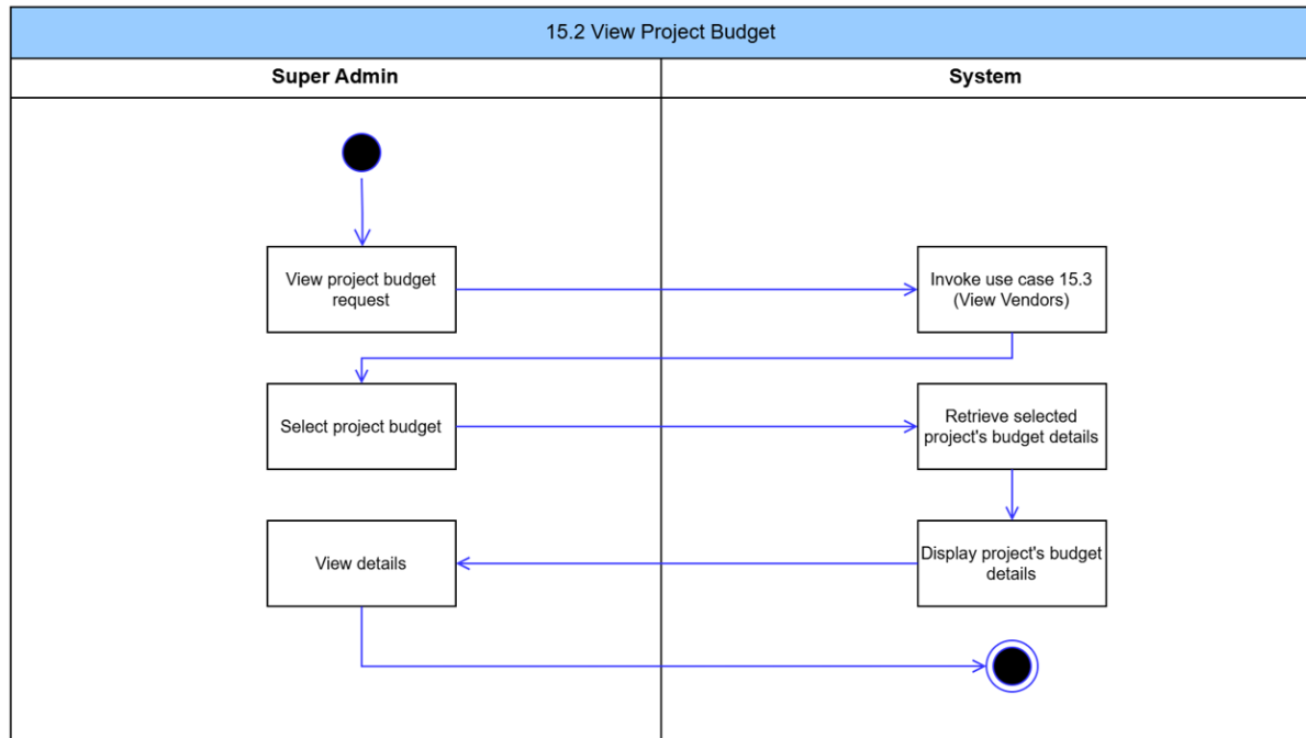
Figure 134: View Project Budget Activity Diagram
