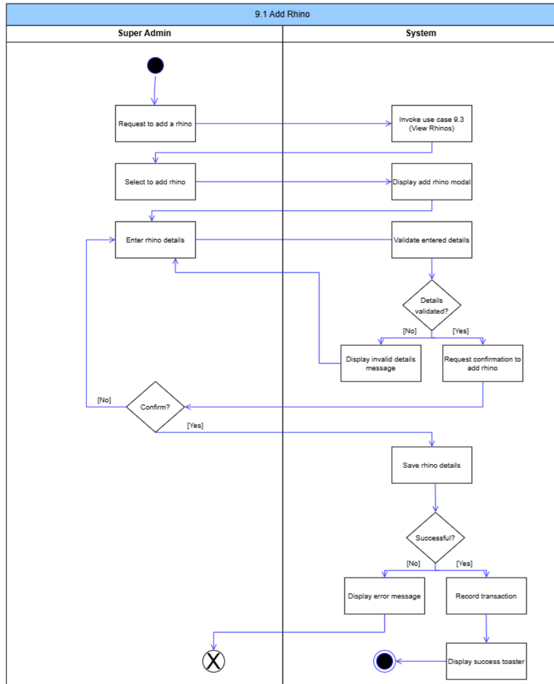
Figure 109: Add Rhino Activity Diagram
