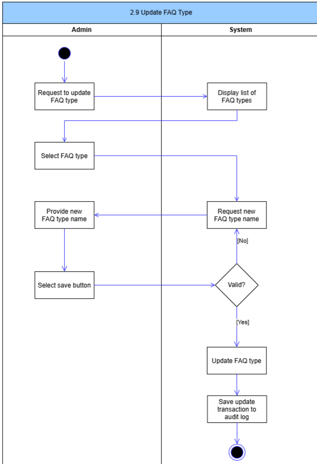
Figure 19: Update FAQ Type Activity Diagram
