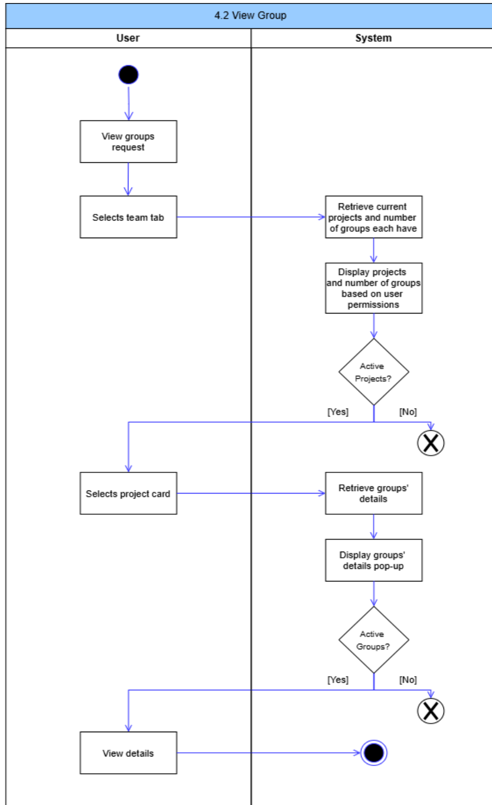
Figure 39: View Group Activity Diagram
