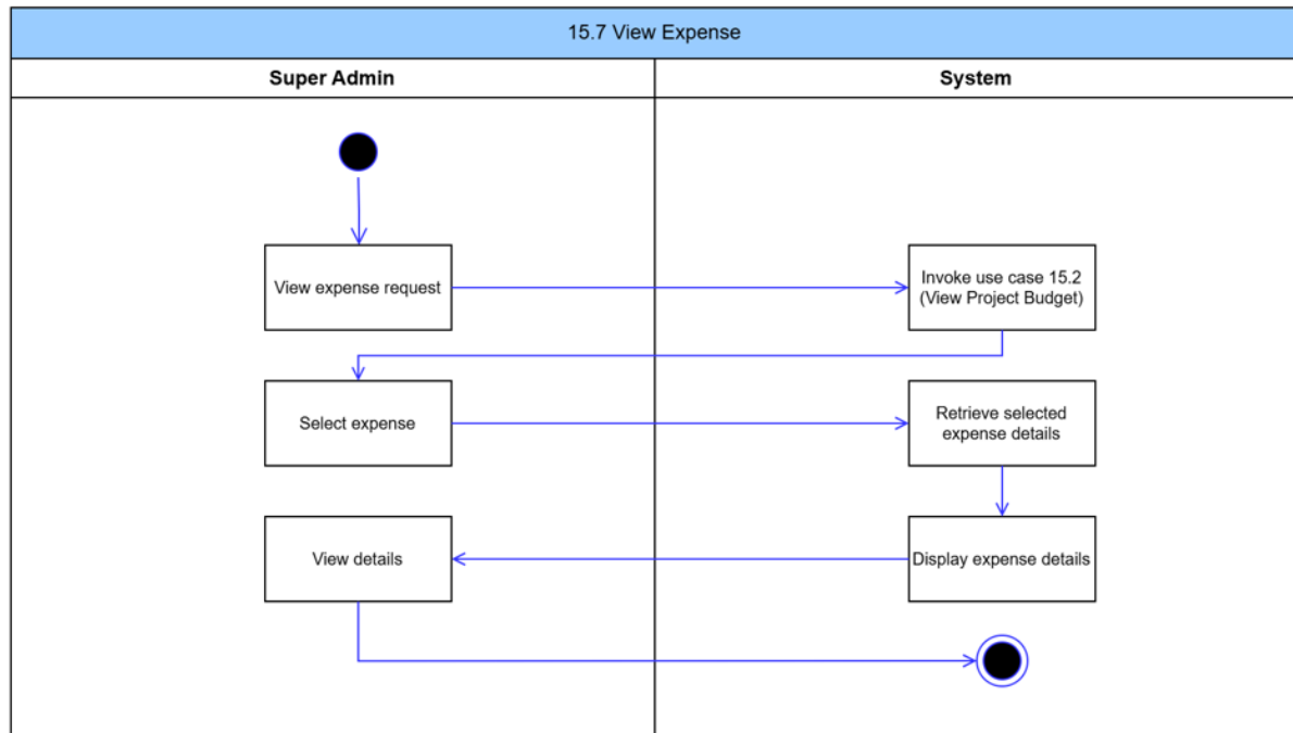
Figure 138: View Expense Activity Diagram
