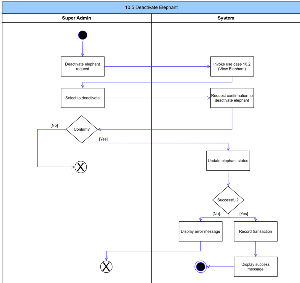
Figure 118: Deactivate Elephant Activity Diagram
