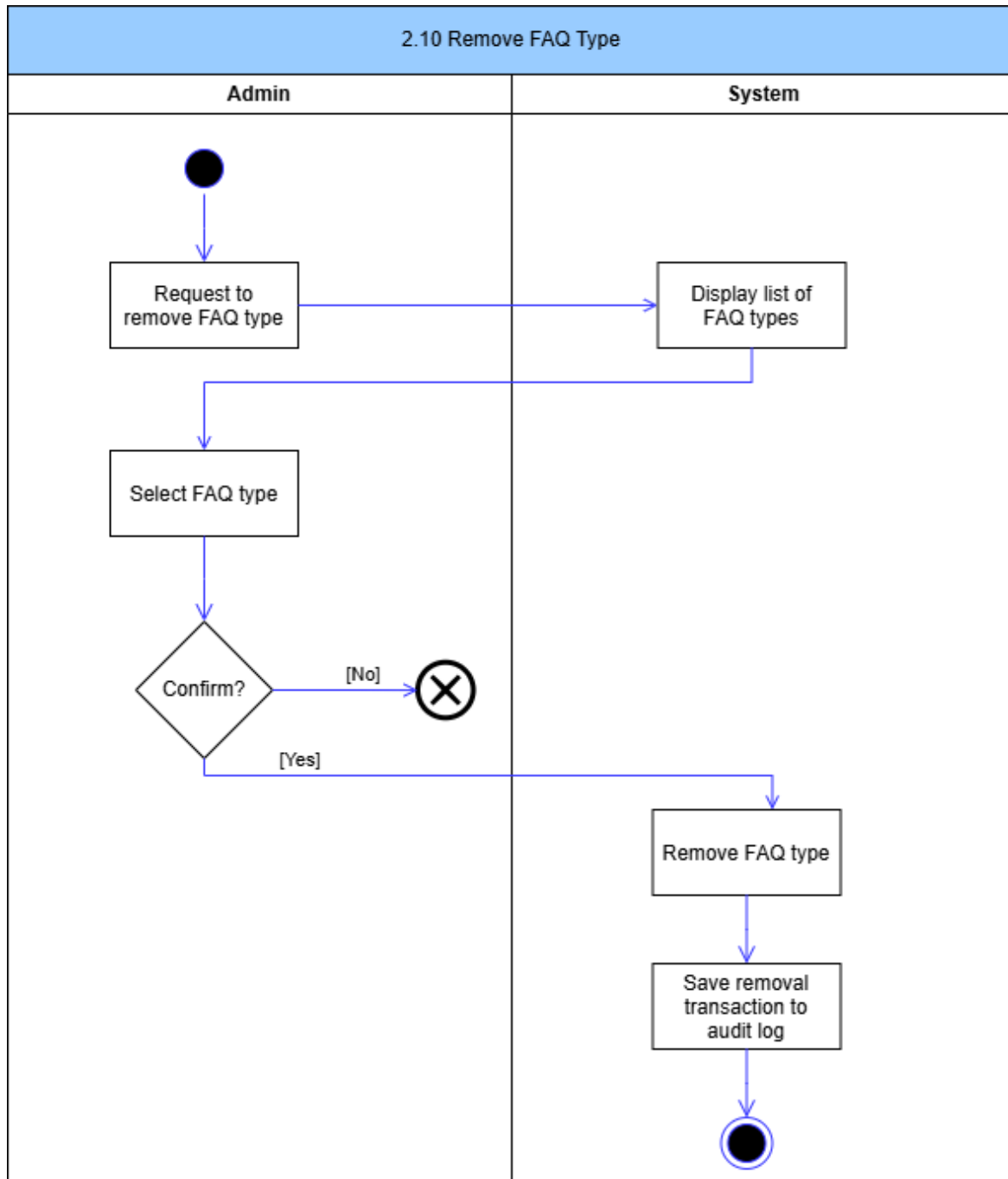
Figure 20: Remove FAQ Type Activity Diagram
