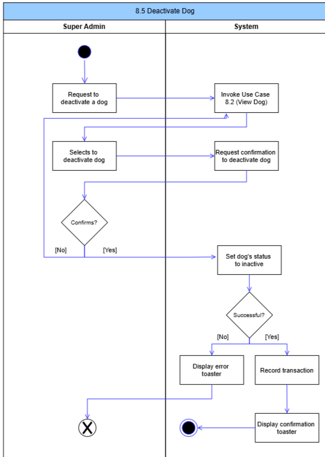
Figure 97: Deactivate Dog Activity Diagram
