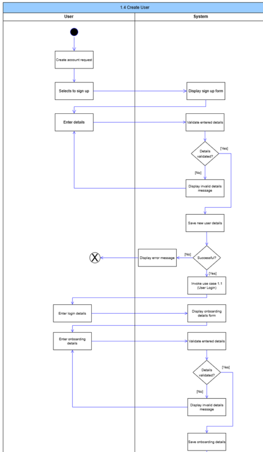
Figure 4: Create User Activity Diagram
