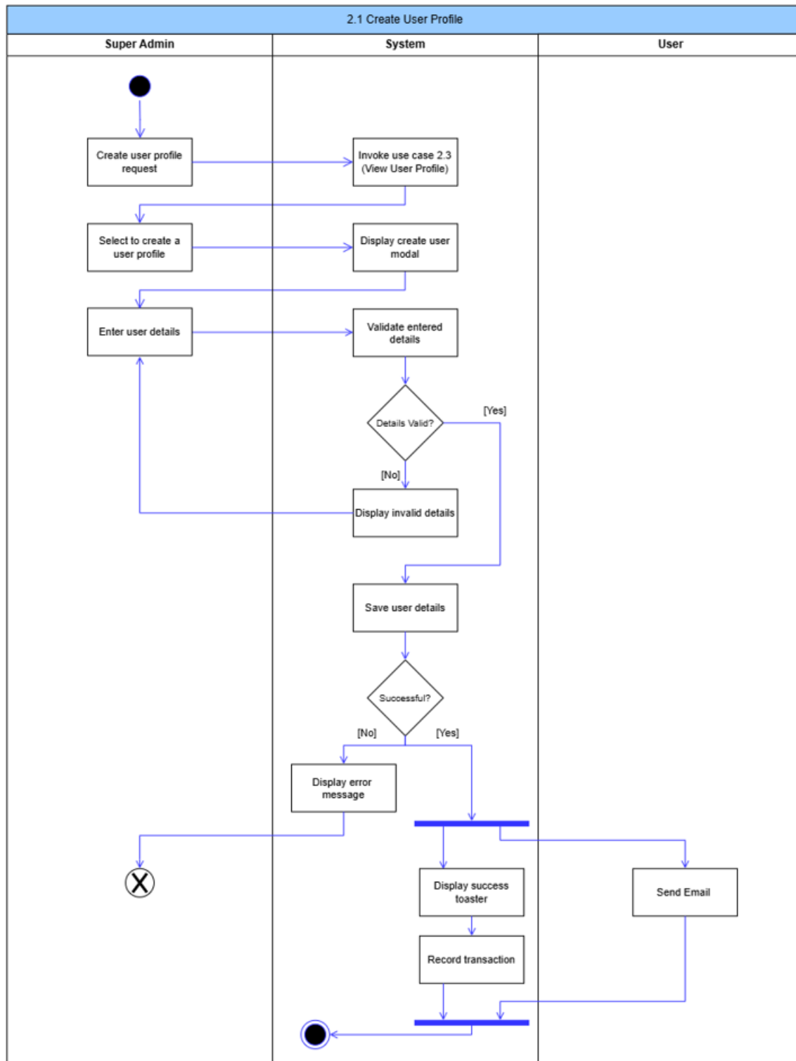
Figure 11: Create User Profile Activity Diagram
