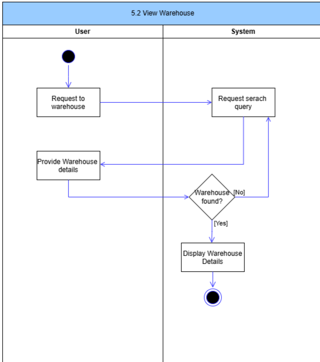
Figure 48: View Warehouse Activity Diagram
