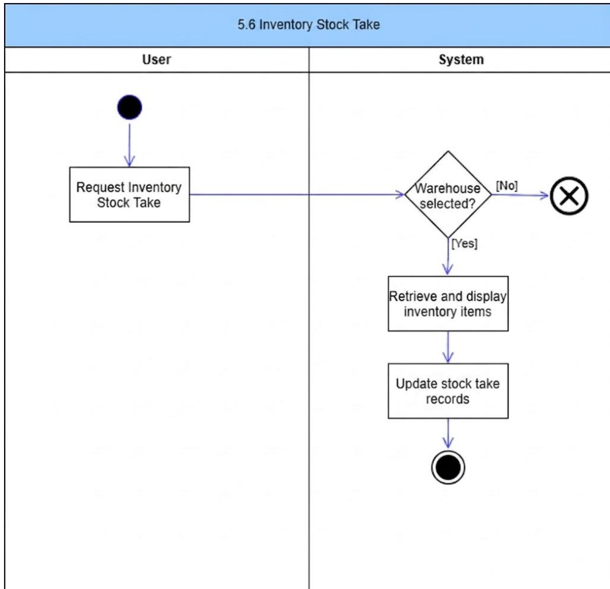
Figure 52: Inventory Stock Take Activity Diagram
