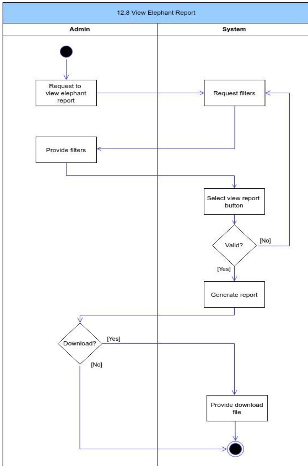
Figure 128: View Elephant Report Activity Diagram
