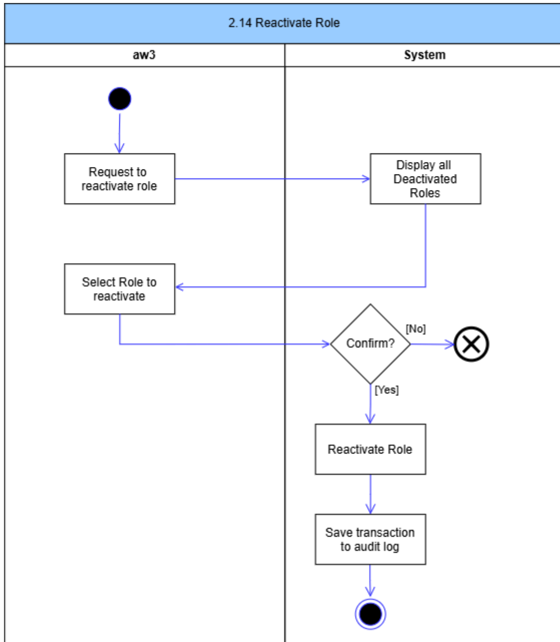
Figure 24: Reactivate Role Activity Diagram
