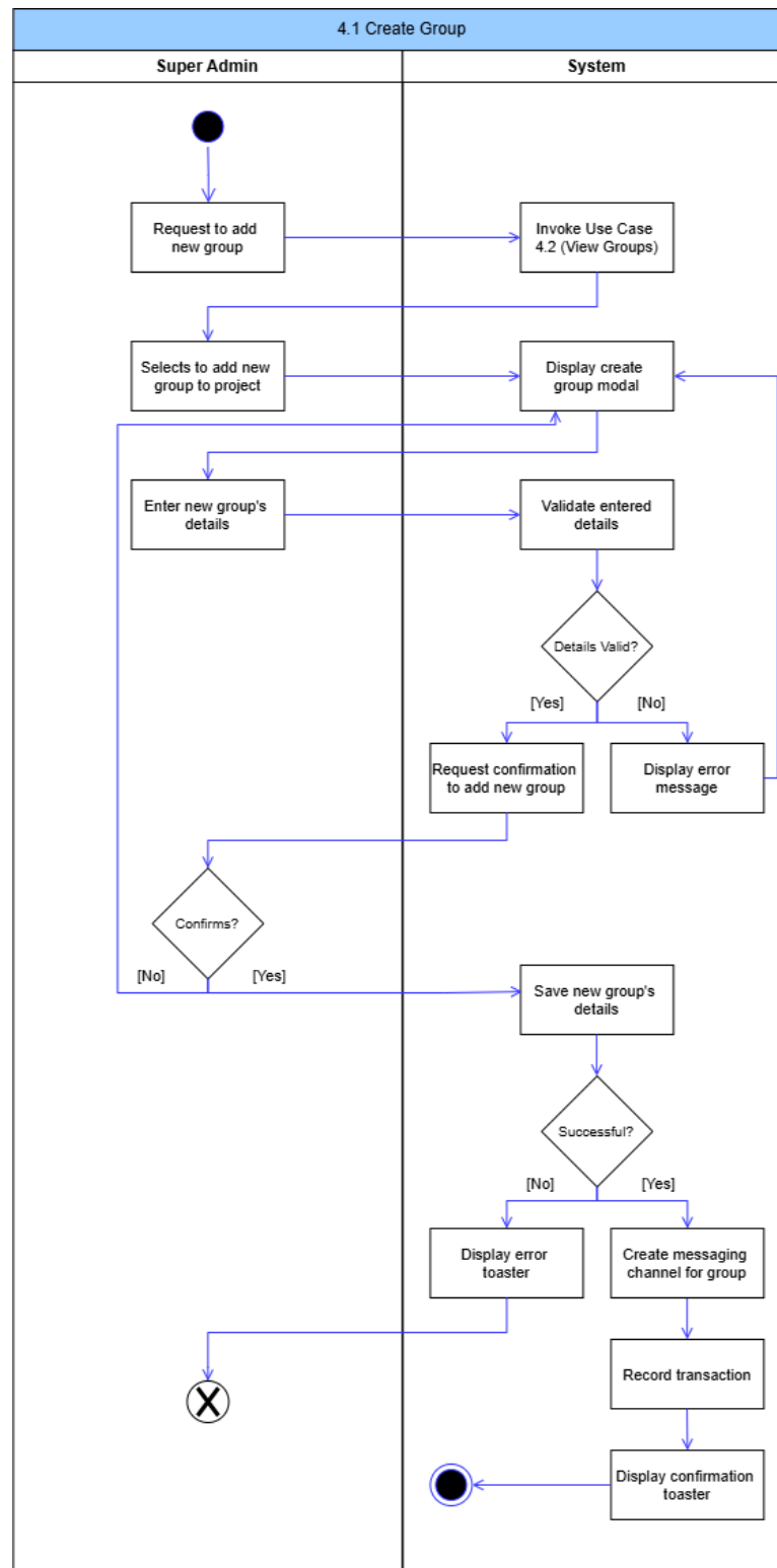
Figure 38: Create Group Activity Diagram
