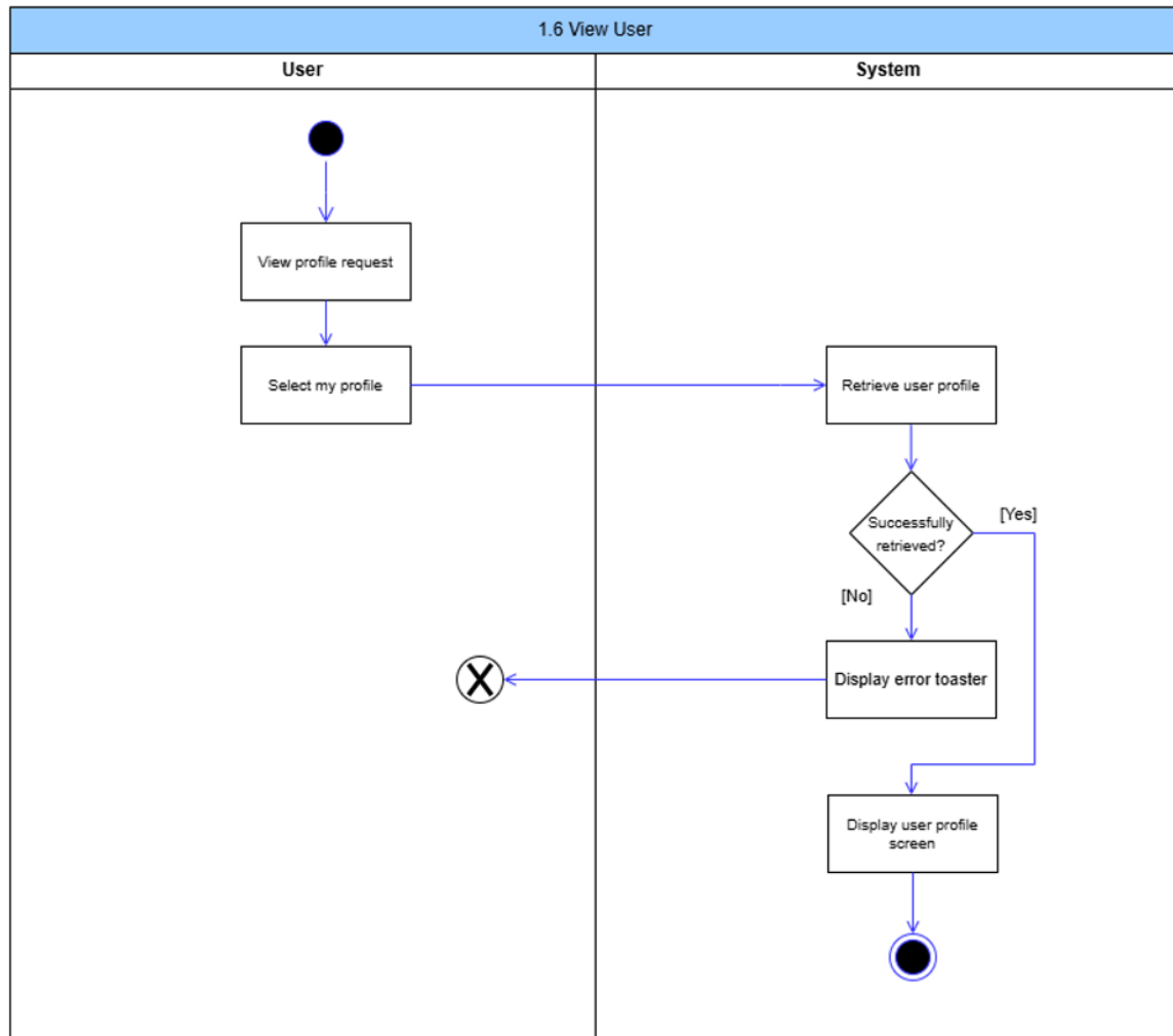
Figure 7: View User Activity Diagram
