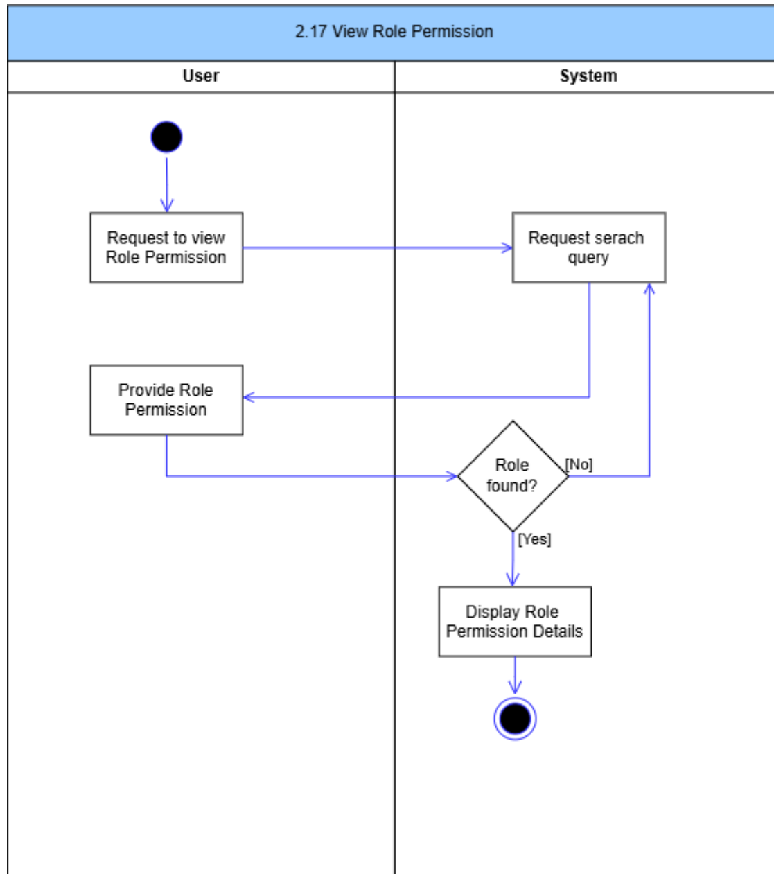
Figure 27: View Role Permission Activity Diagram
