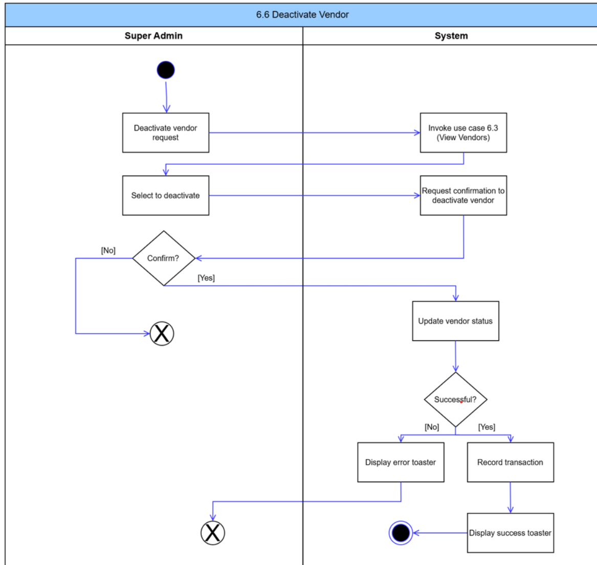
Figure 58: Deactivate Vendor Activity Diagram
