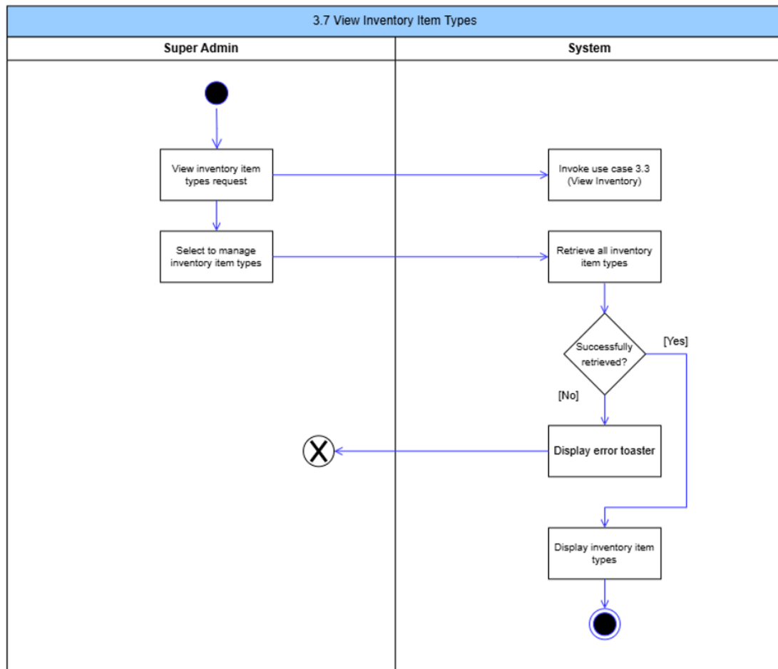
Figure 34: View Inventory Item Types Activity Diagram
