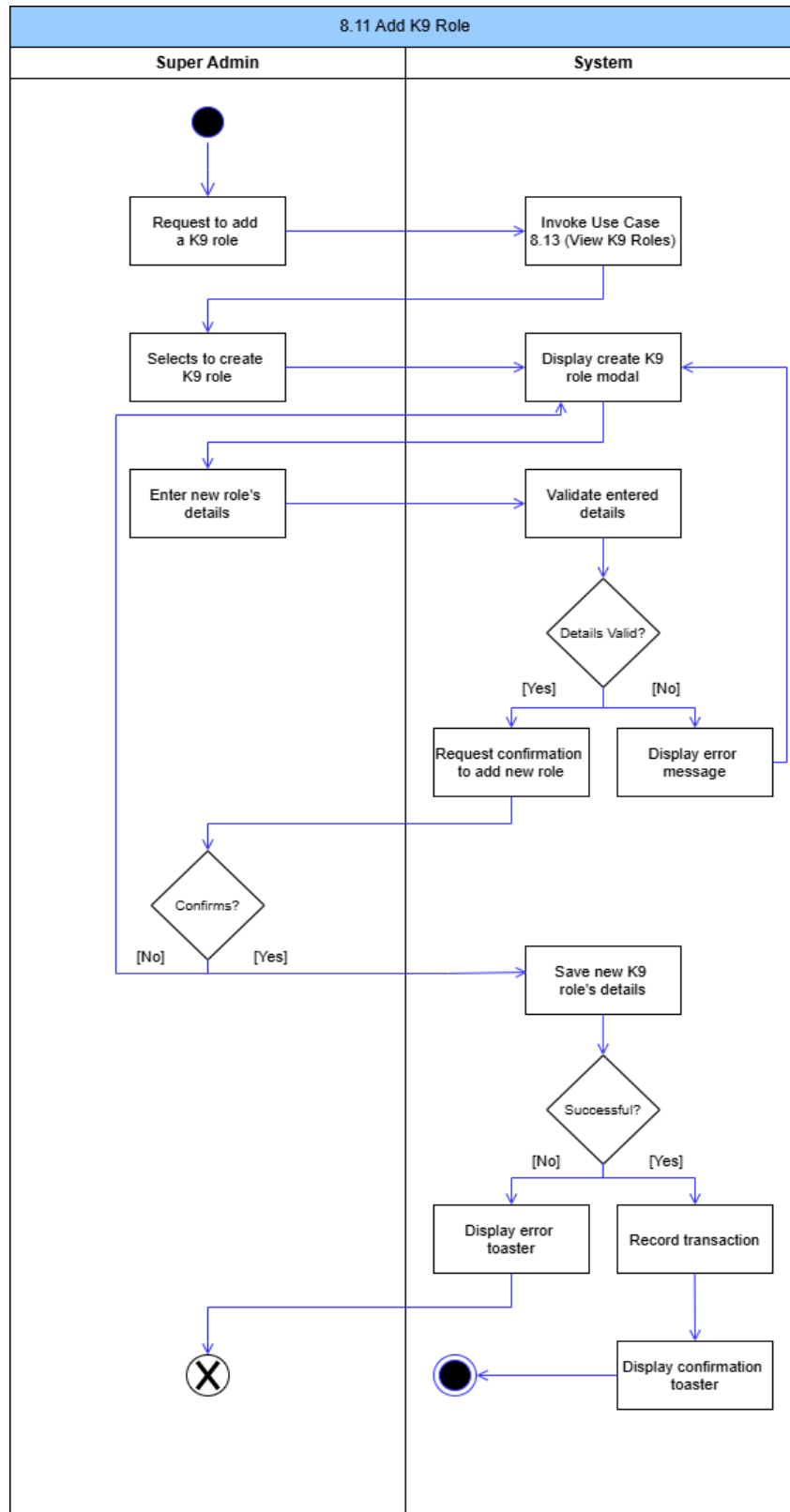
Figure 103: Add K9 Role Activity Diagram
