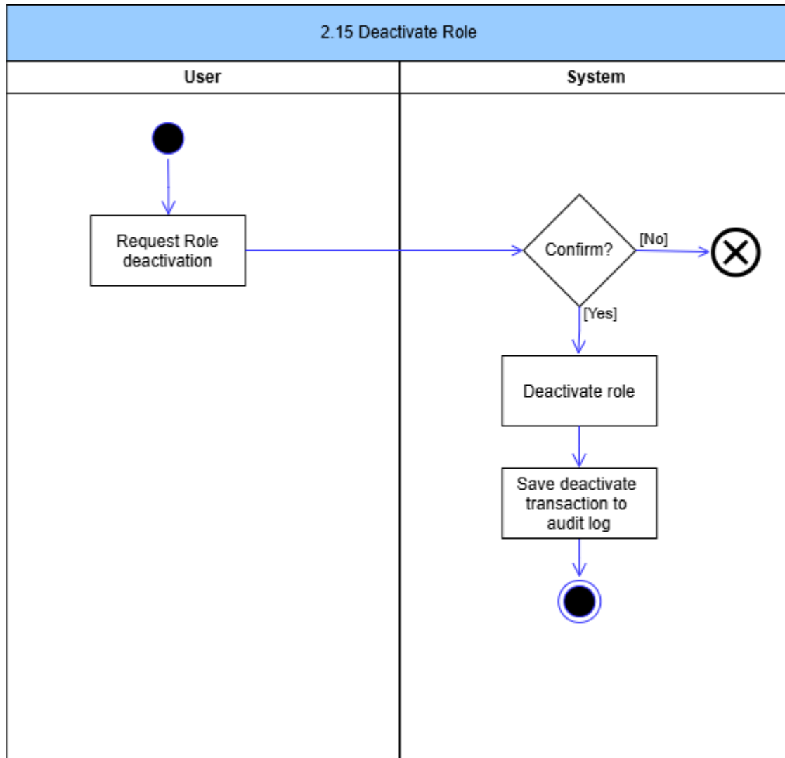
Figure 25: Deactivate Role Activity Diagram
