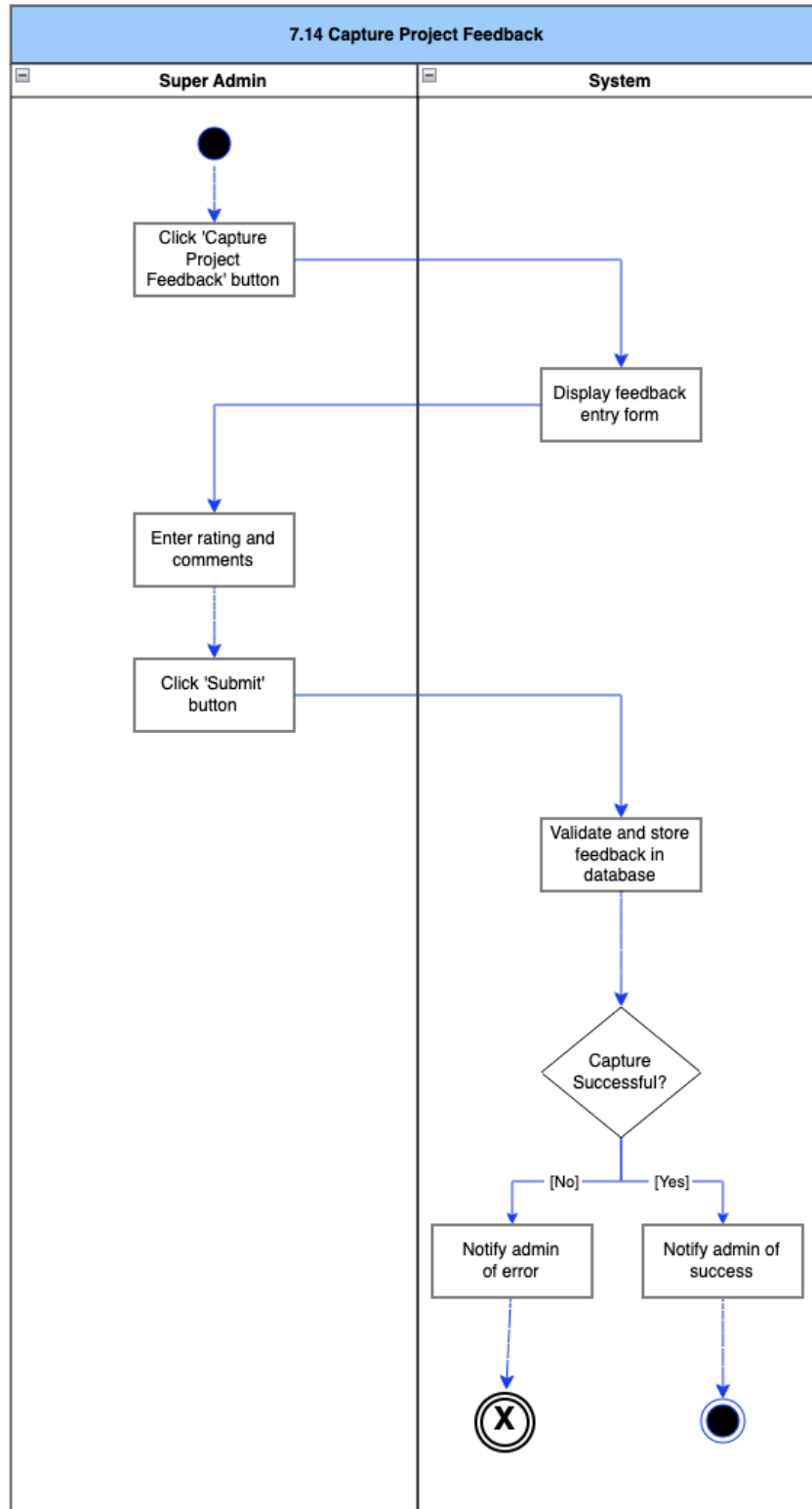
Figure 77: Capture Project Feedback Activity Diagram
