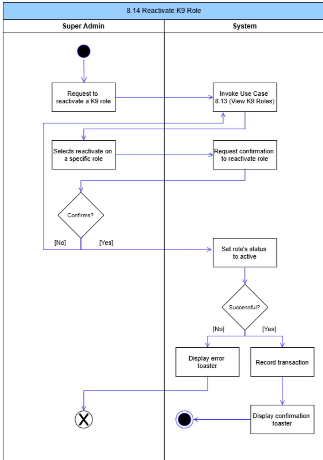
Figure 106: Reactivate K9 Role Activity Diagram
