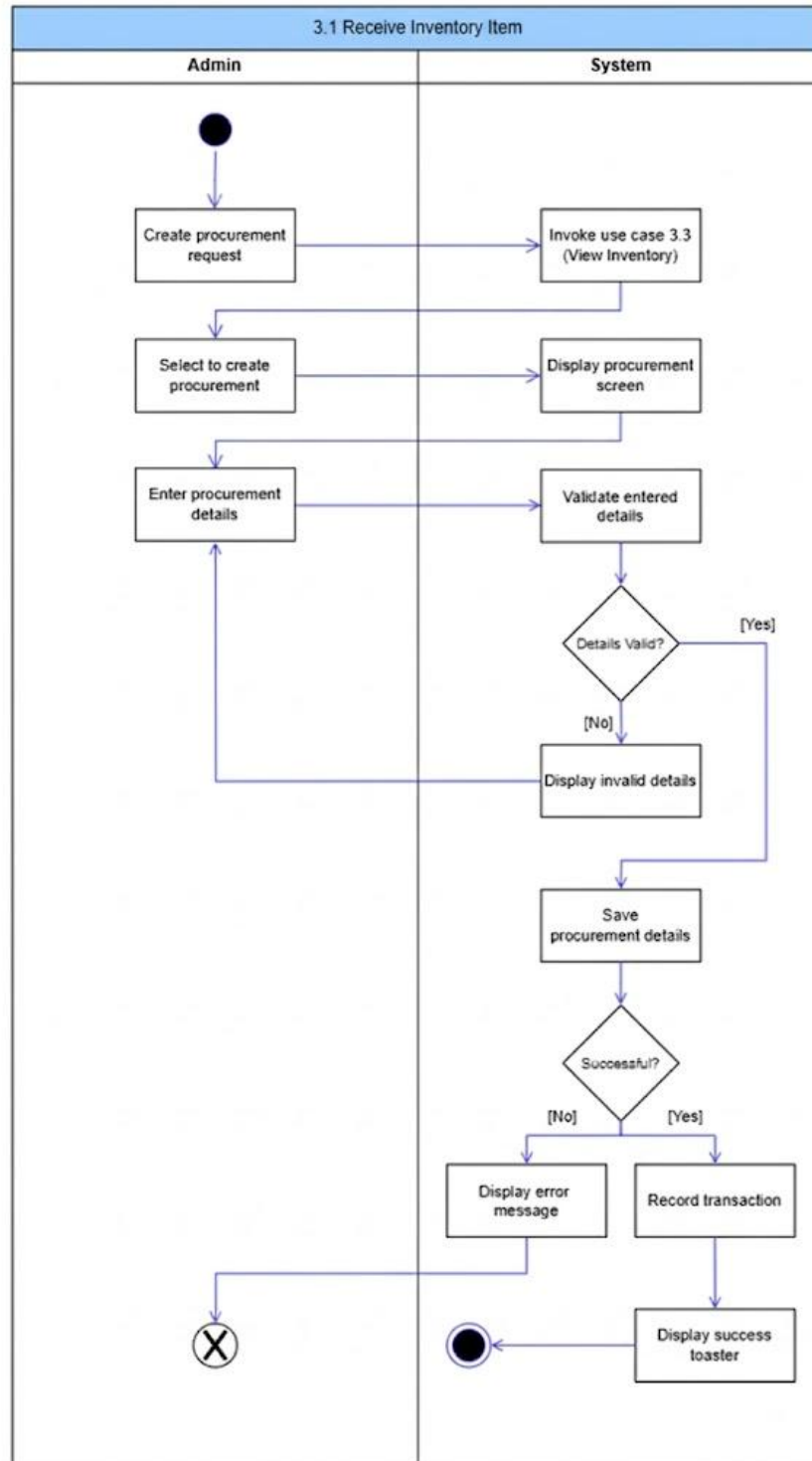
Figure 28: Receive Inventory Item Activity Diagram
