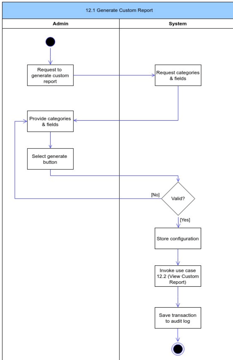
Figure 121: Generate Custom Report Activity Diagram
