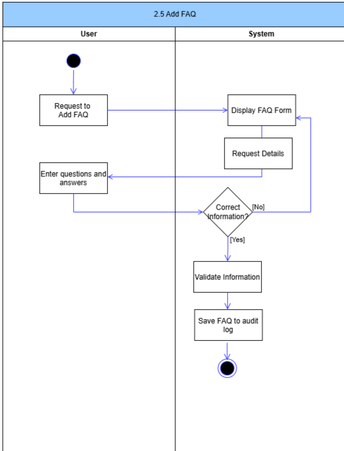
Figure 15: Add FAQ Activity Diagram
