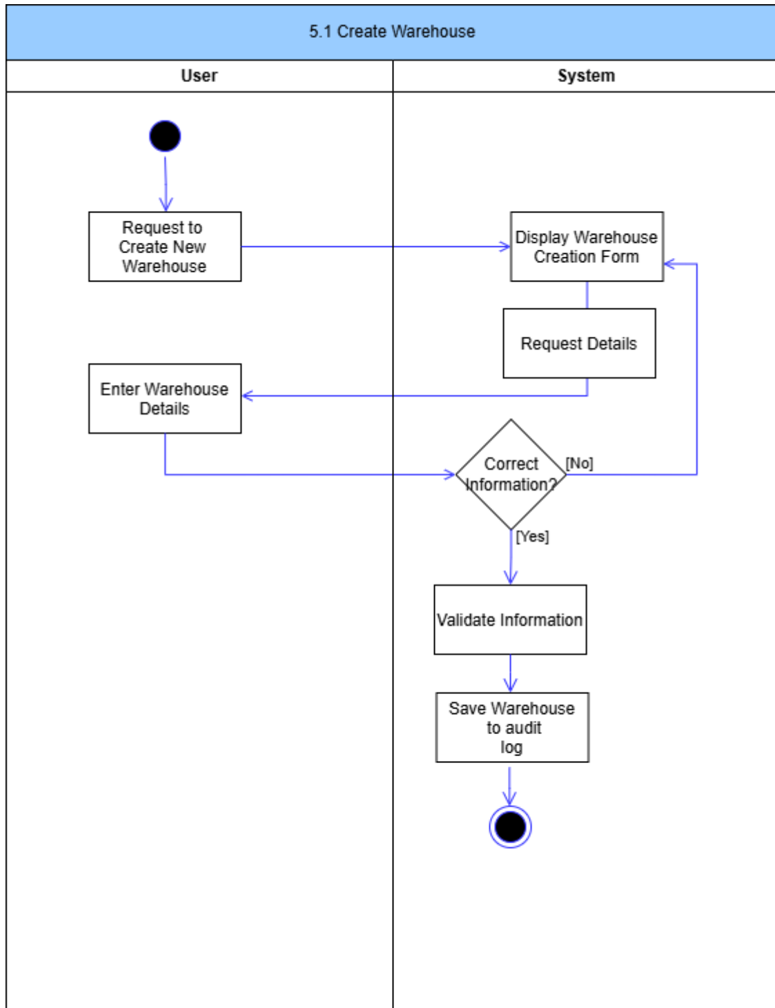
Figure 47: Create Warehouse Activity Diagram
