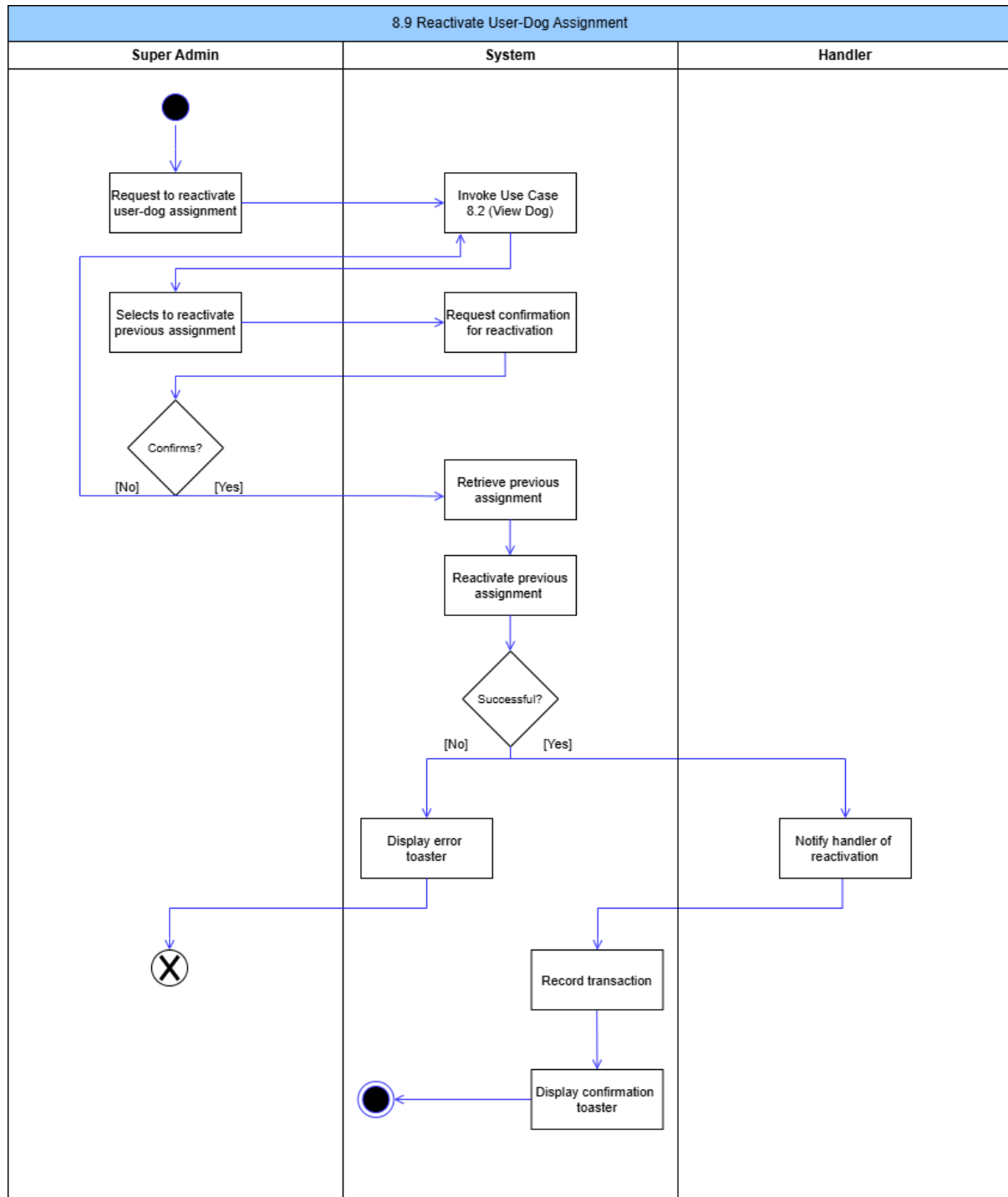
Figure 101: Reactivate User-Dog Assignment Activity Diagram
