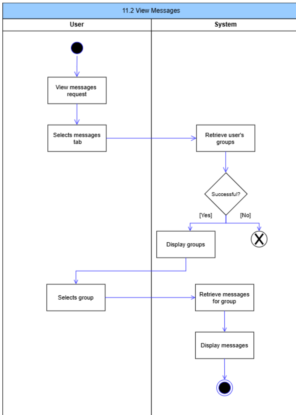
Figure 120: View Messages Activity Diagram
