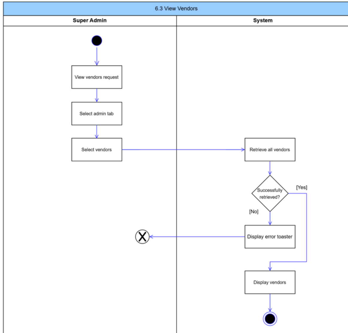
Figure 55: View Vendors Activity Diagram
