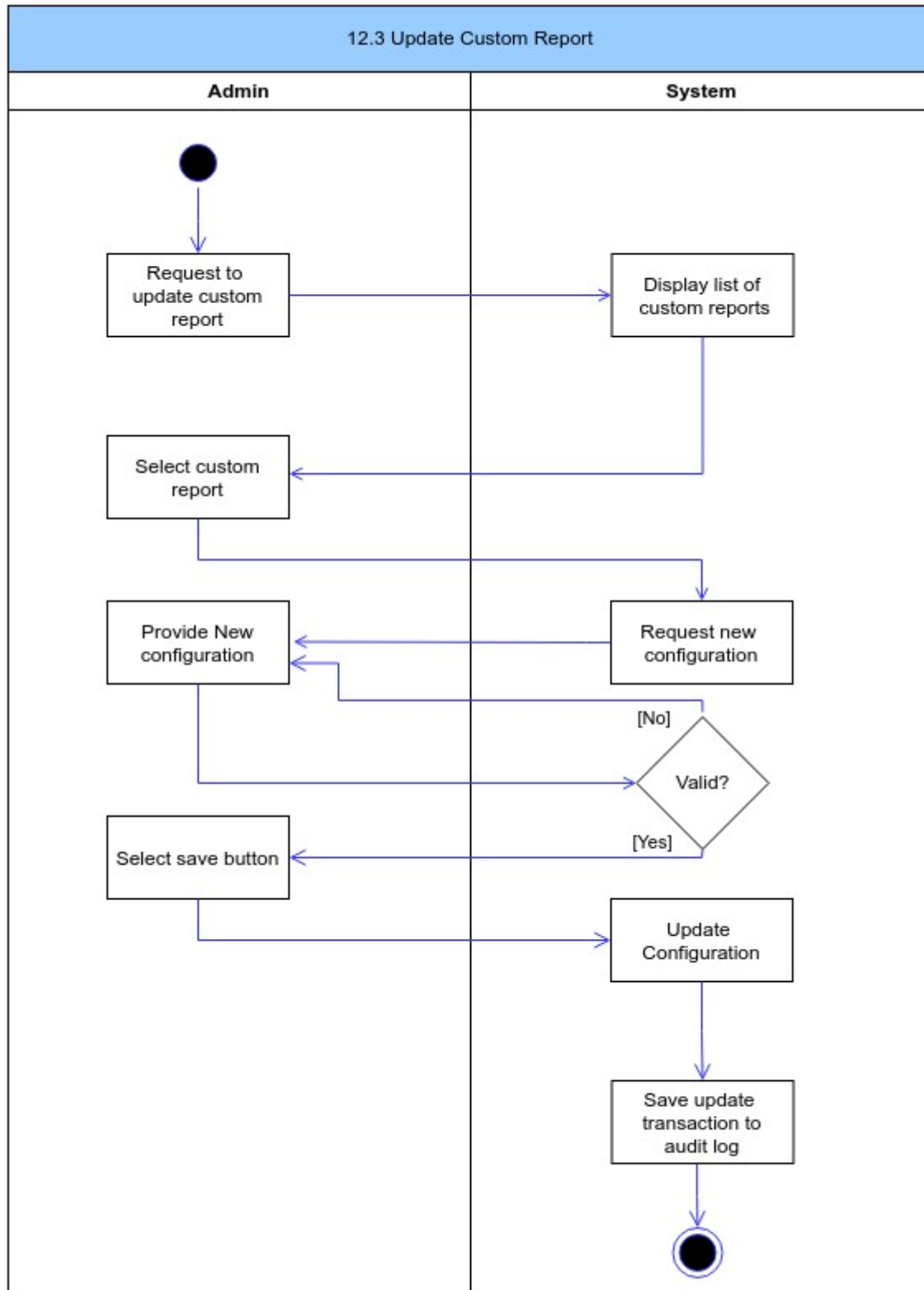
Figure 123: Update Custom Report Activity Diagram
