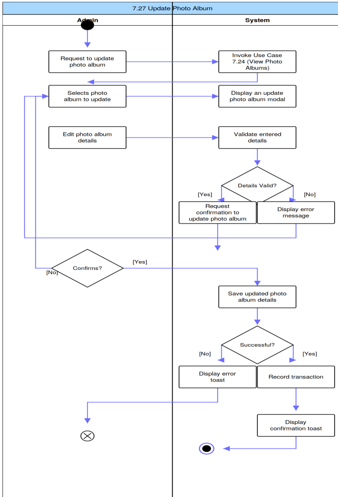
Figure 90: Update Photo Album Activity Diagram
