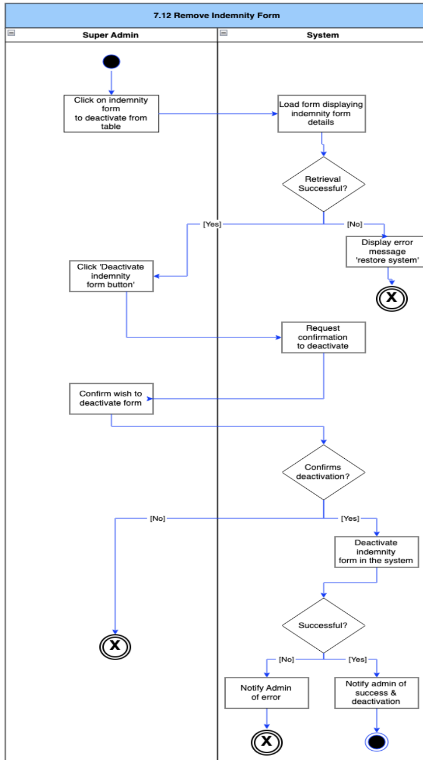
Figure 75: Remove Indemnity Form Activity Diagram
