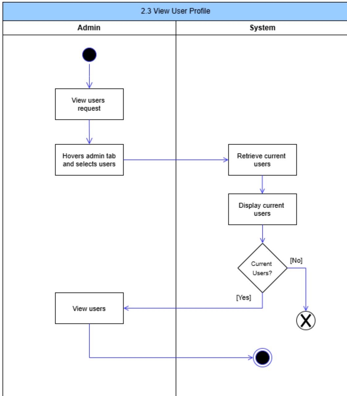
Figure 13: View User Profile Activity Diagram
