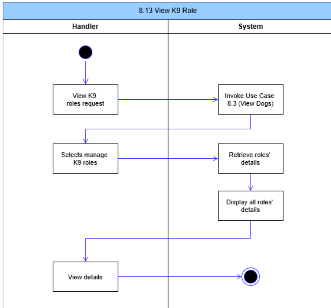
Figure 105: View K9 Role Activity Diagram
