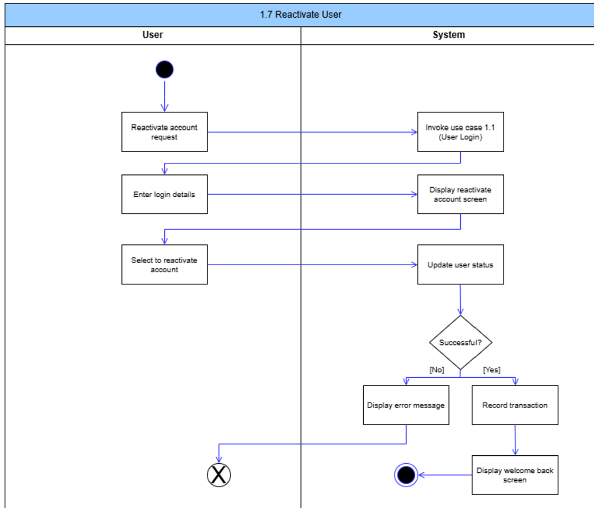
Figure 8: Reactivate User Activity Diagram
