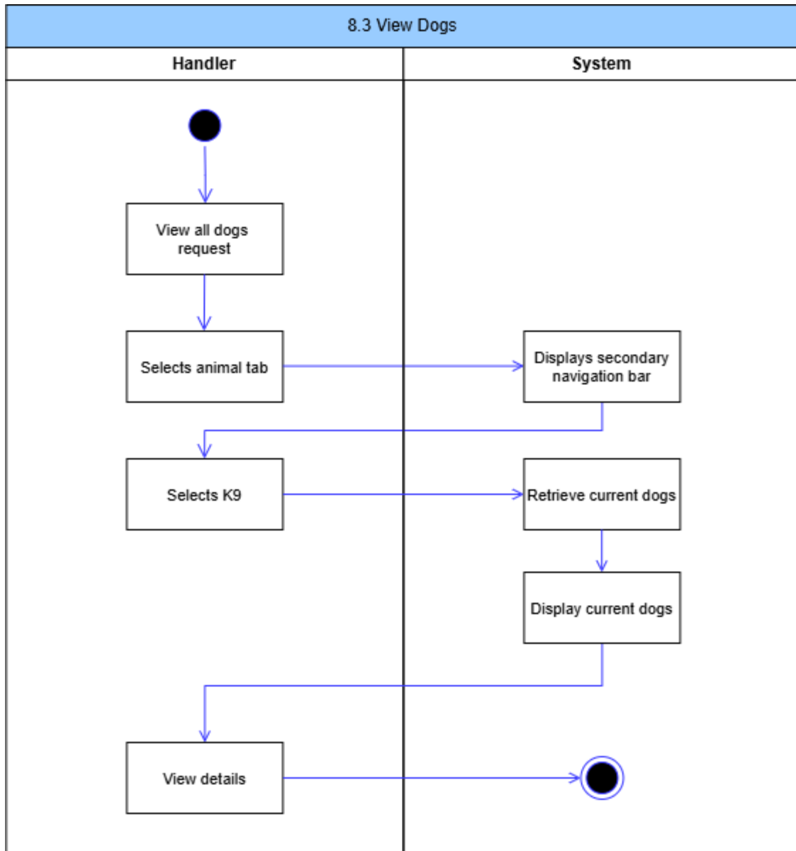
Figure 94: View Dogs Activity Diagram
