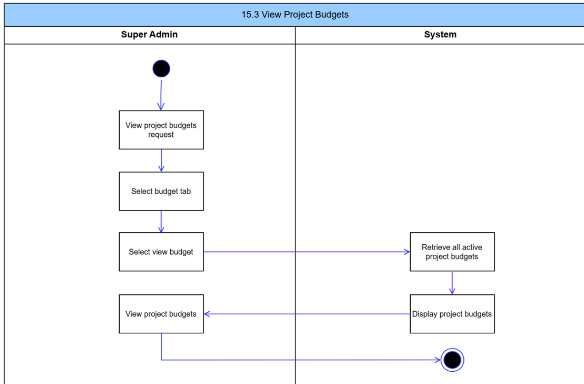
Figure 135: View Project Budgets Activity Diagram
