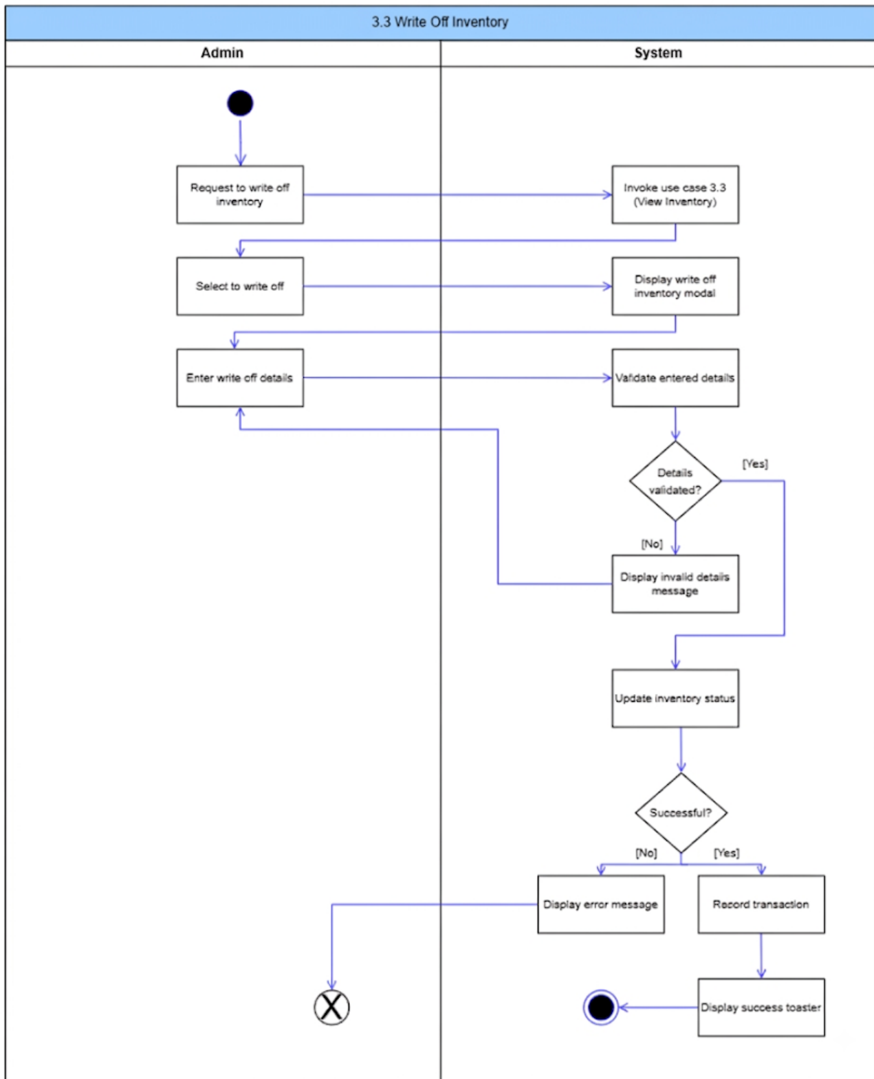
Figure 30: Write Off Inventory Activity Diagram
