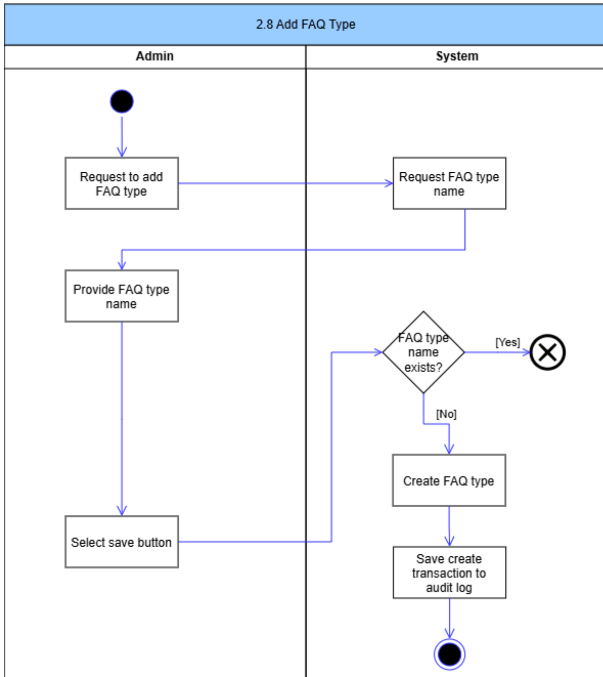
Figure 18: Add FAQ Type Activity Diagram
