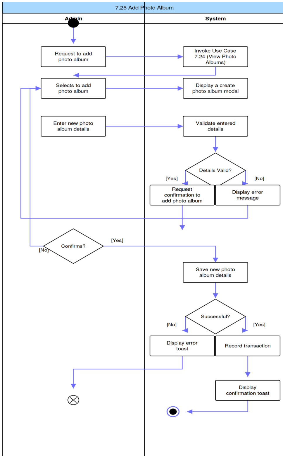
Figure 88: Add Photo Album Activity Diagram
