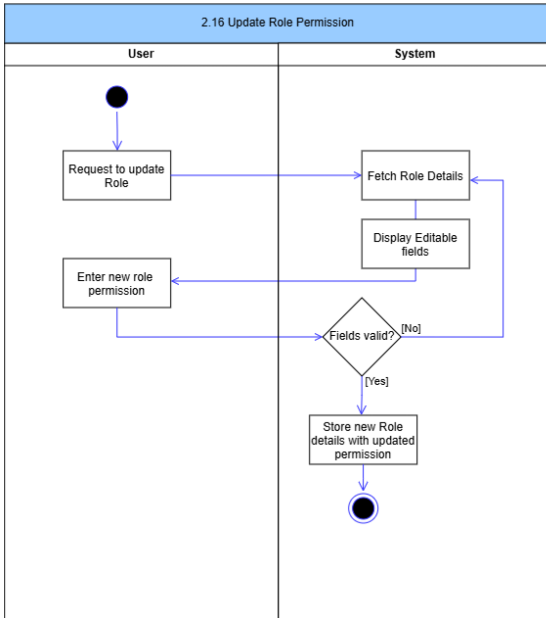
Figure 26: Update Role Permission Activity Diagram
