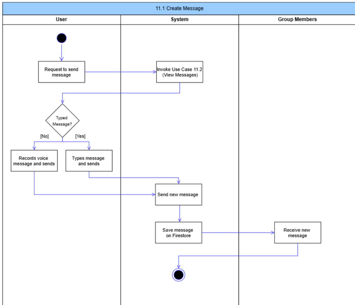
Figure 119: Create Message Activity Diagram
