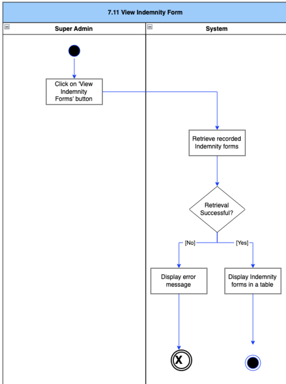
Figure 74: View Indemnity Form Activity Diagram
