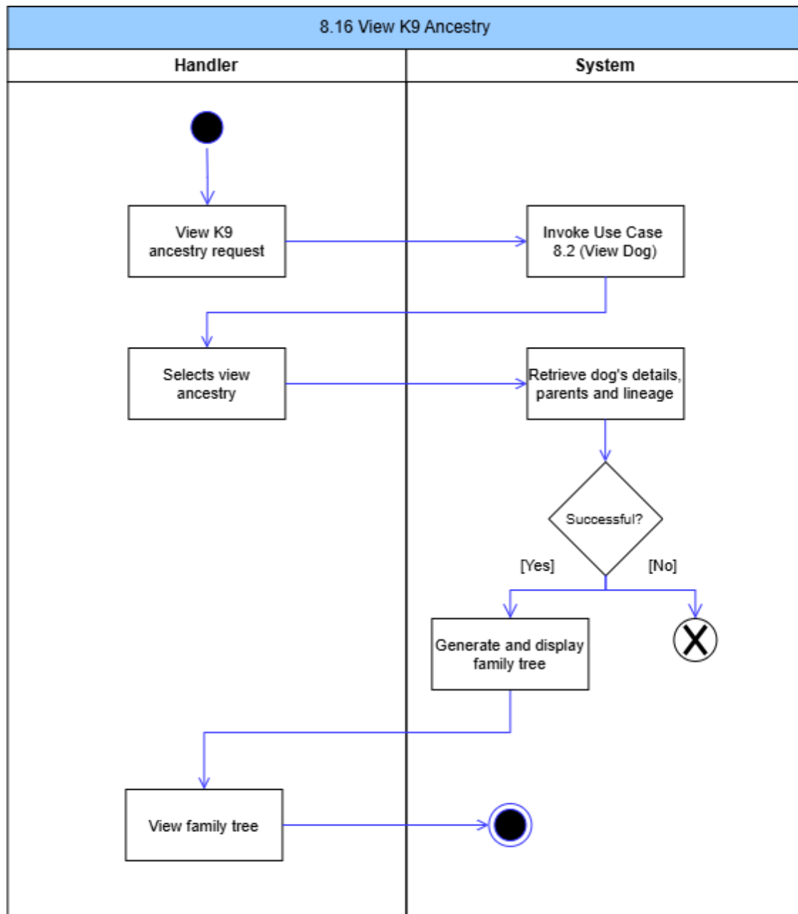
Figure 108: View K9 Ancestry Activity Diagram
