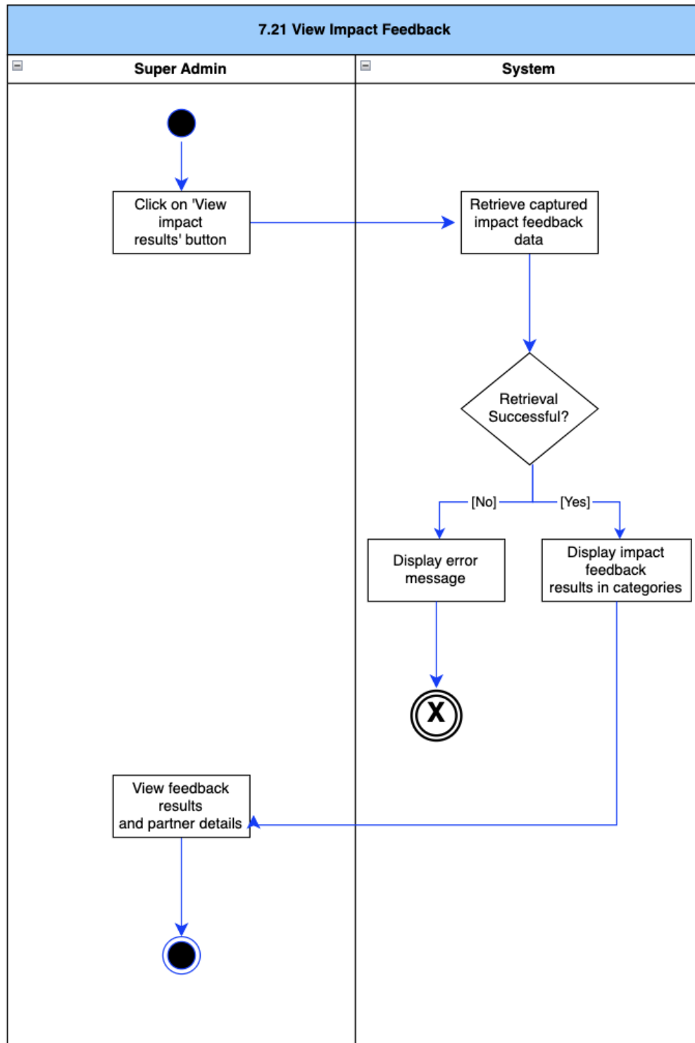
Figure 84: View Impact Feedback Activity Diagram
