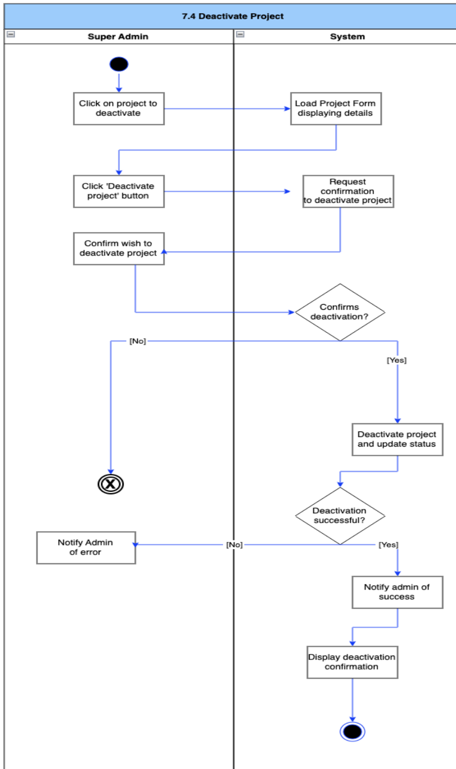
Figure 67: Deactivate Project Activity Diagram
