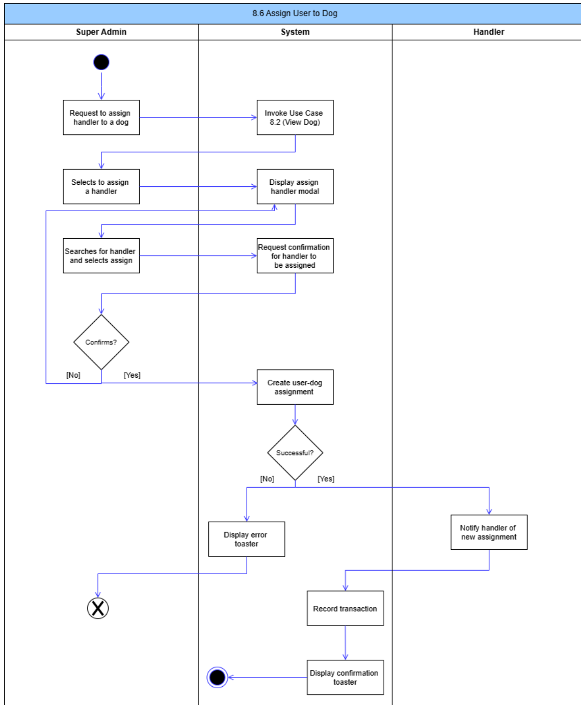
Figure 98: Assign User to Dog Activity Diagram
