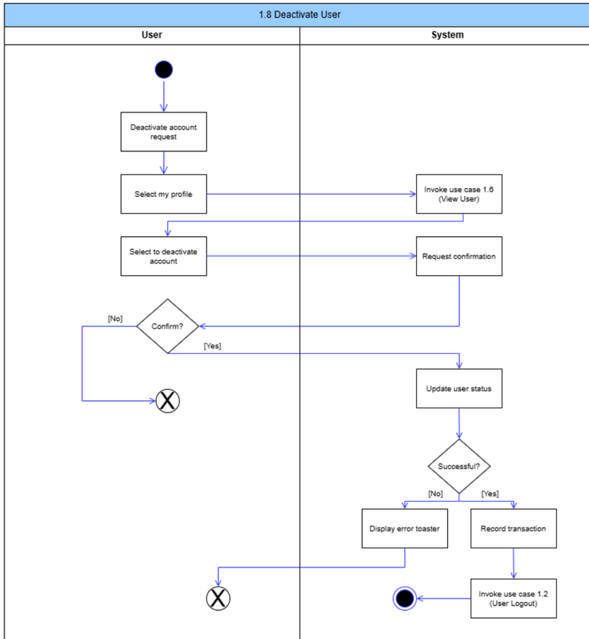
Figure 9: Deactivate User Activity Diagram
