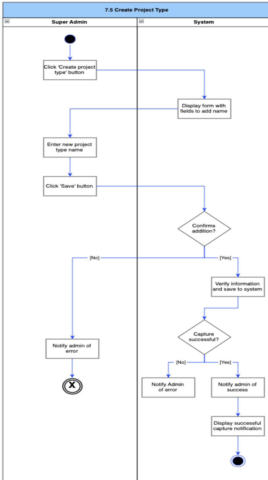
Figure 68: Create Project Type Activity Diagram
