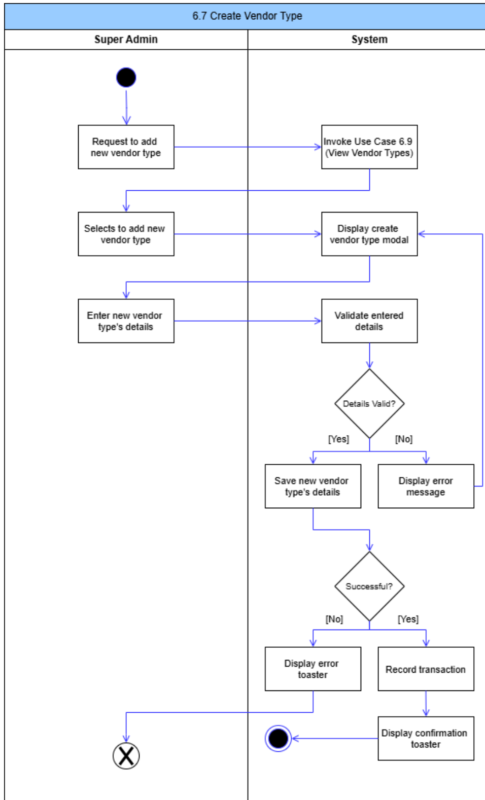
Figure 59: Create Vendor Type Activity Diagram
