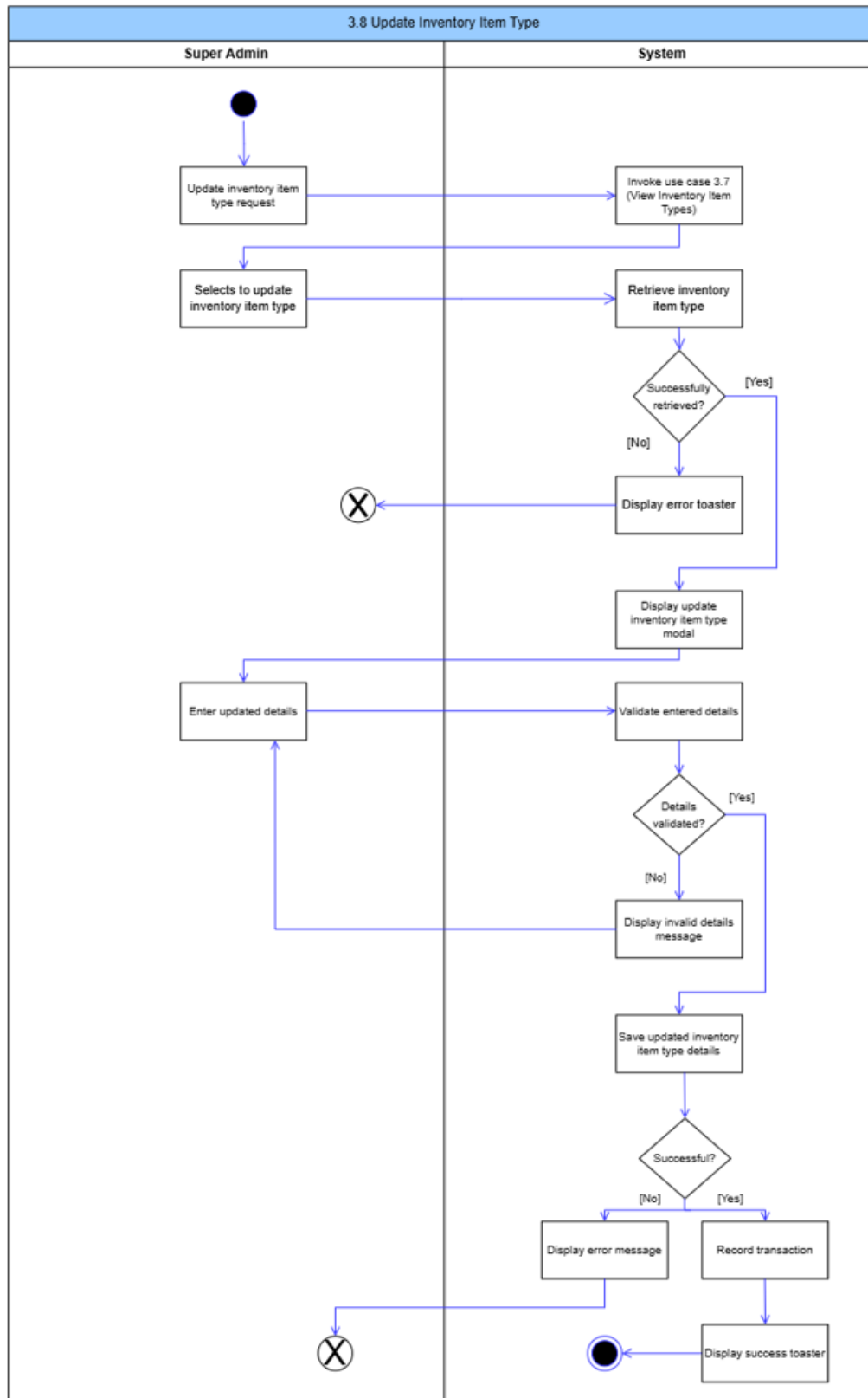
Figure 35: Update Inventory Item Type Activity Diagram
