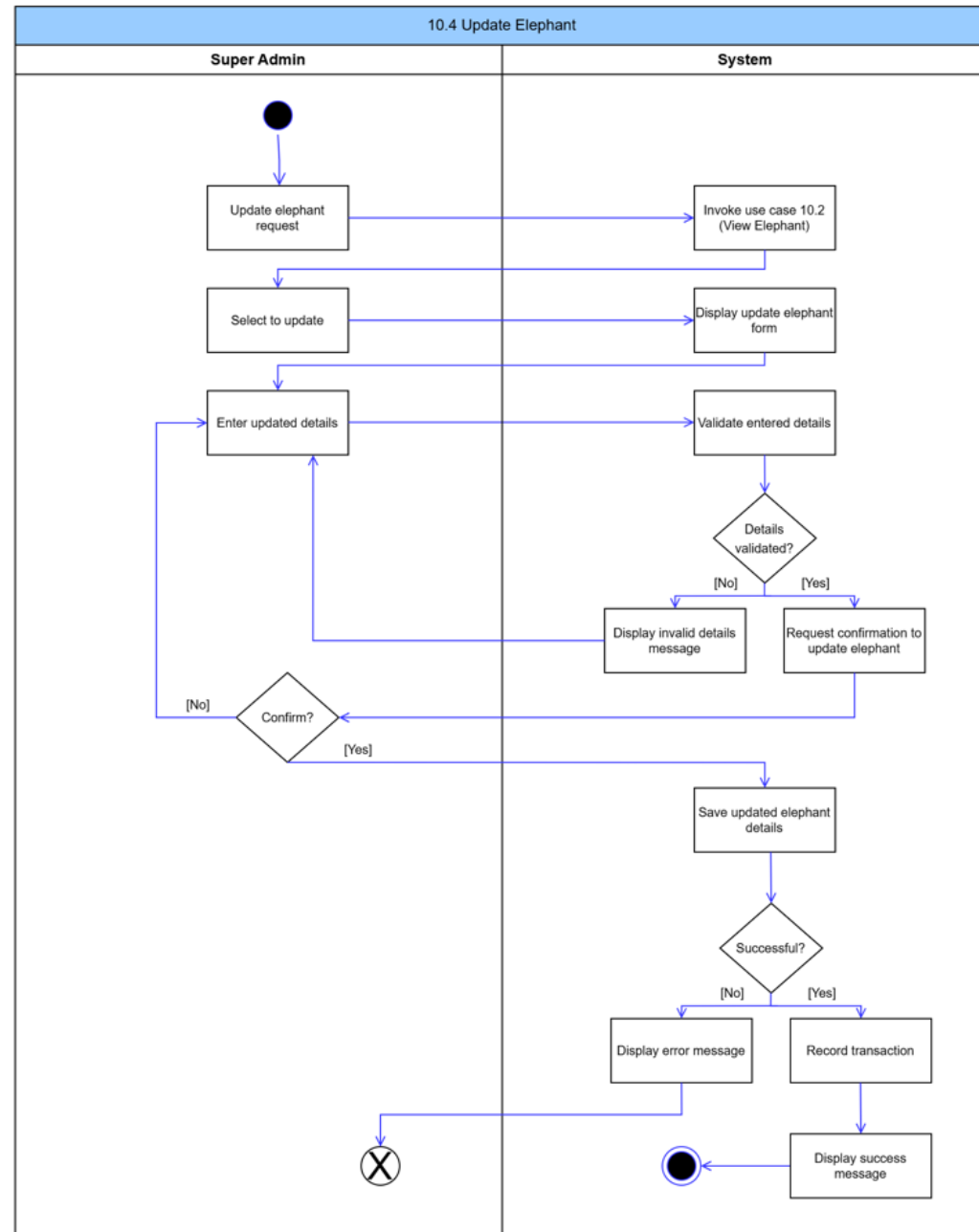
Figure 117: Update Elephant Activity Diagram
