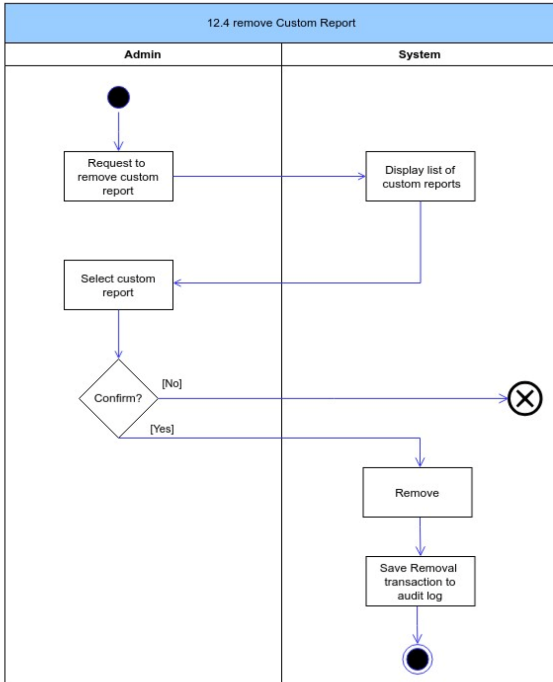
Figure 124: Remove Custom Report Activity Diagram
