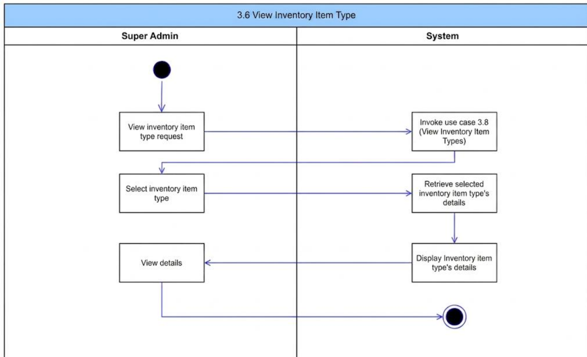
Figure 33: View Inventory Item Type Activity Diagram
