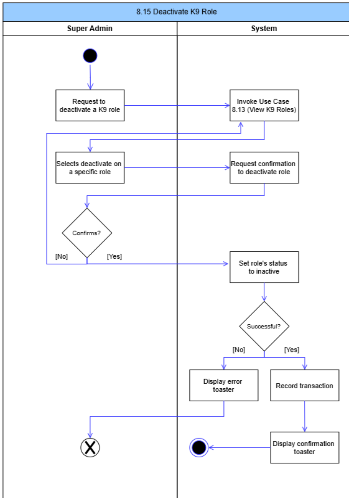
Figure 107: Deactivate K9 Role Activity Diagram
