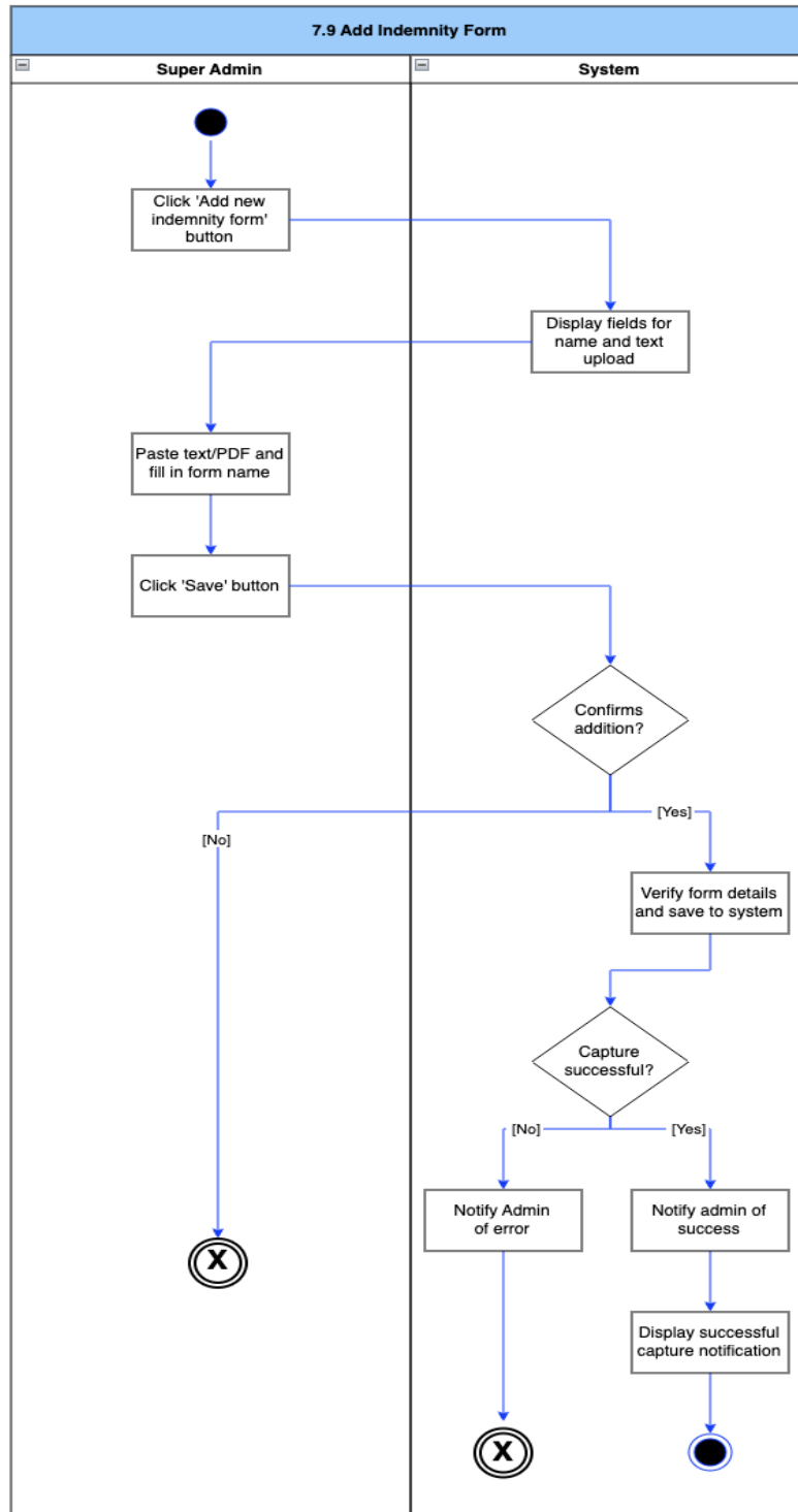
Figure 72: Add Indemnity Form Activity Diagram
