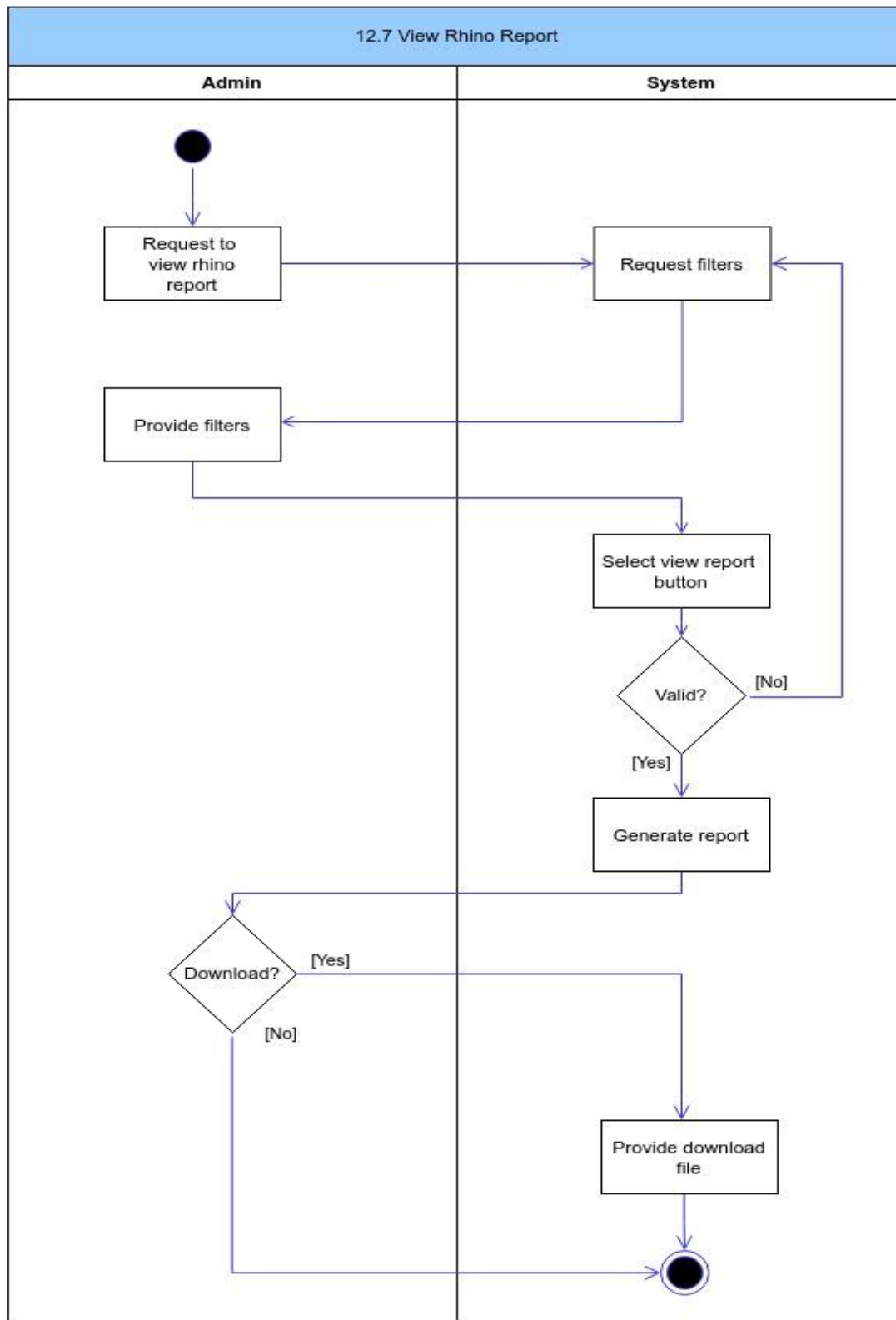
Figure 127: View Rhino Report Activity Diagram
