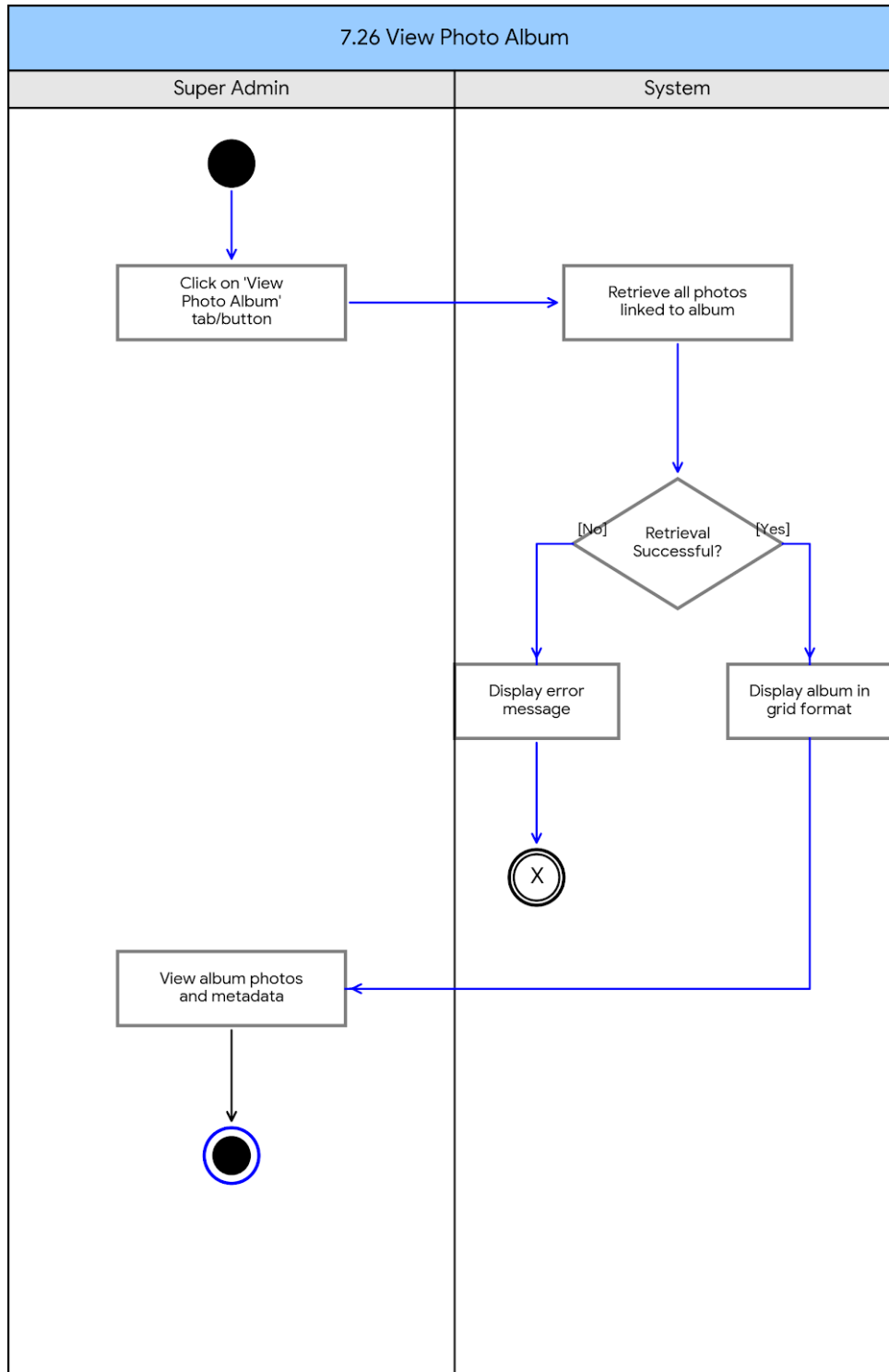
Figure 89: View Photo Album Activity Diagram
