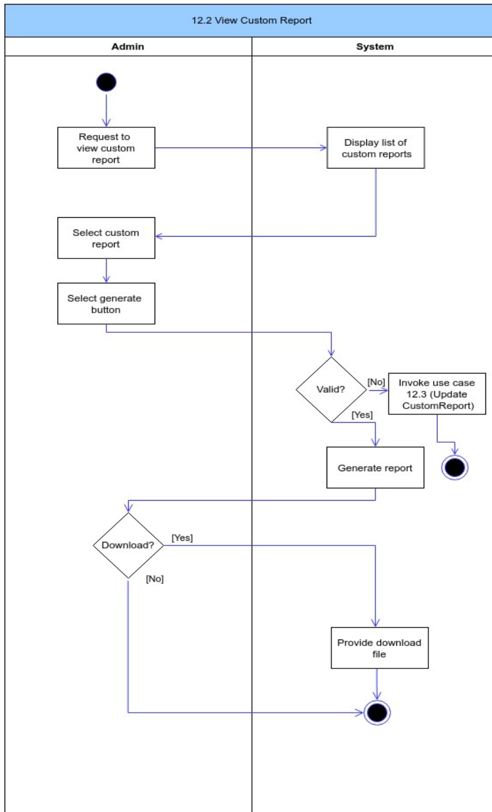
Figure 122: View Custom Report Activity Diagram
