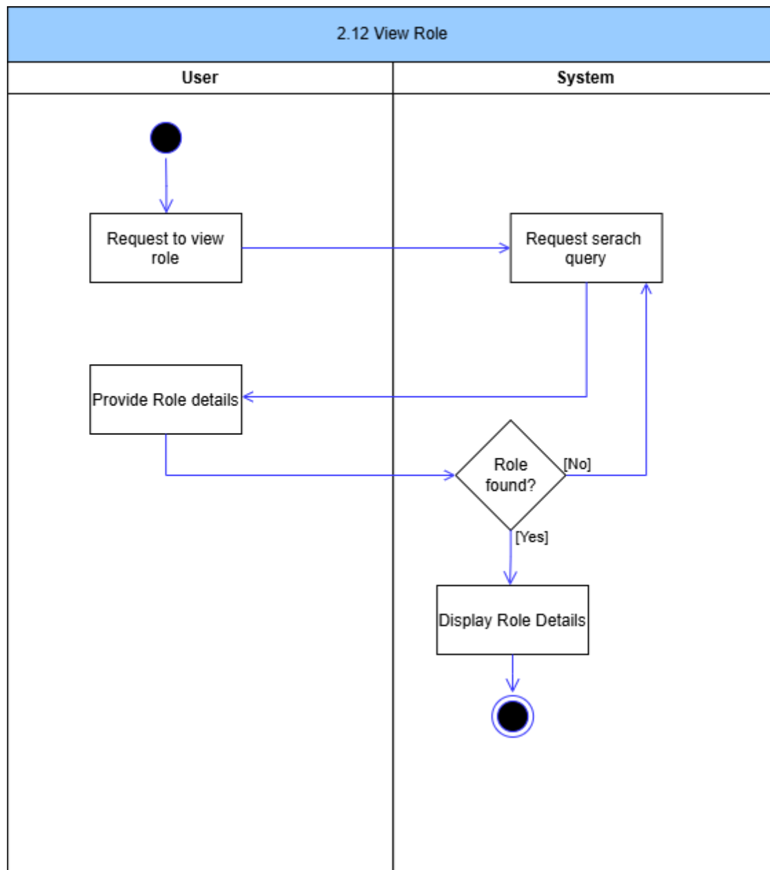
Figure 22: View Role Activity Diagram
