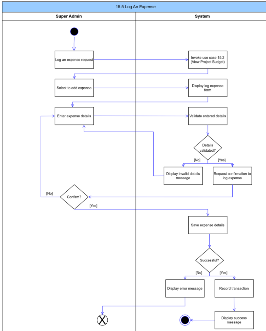
Figure 136: Log An Expense Activity Diagram
