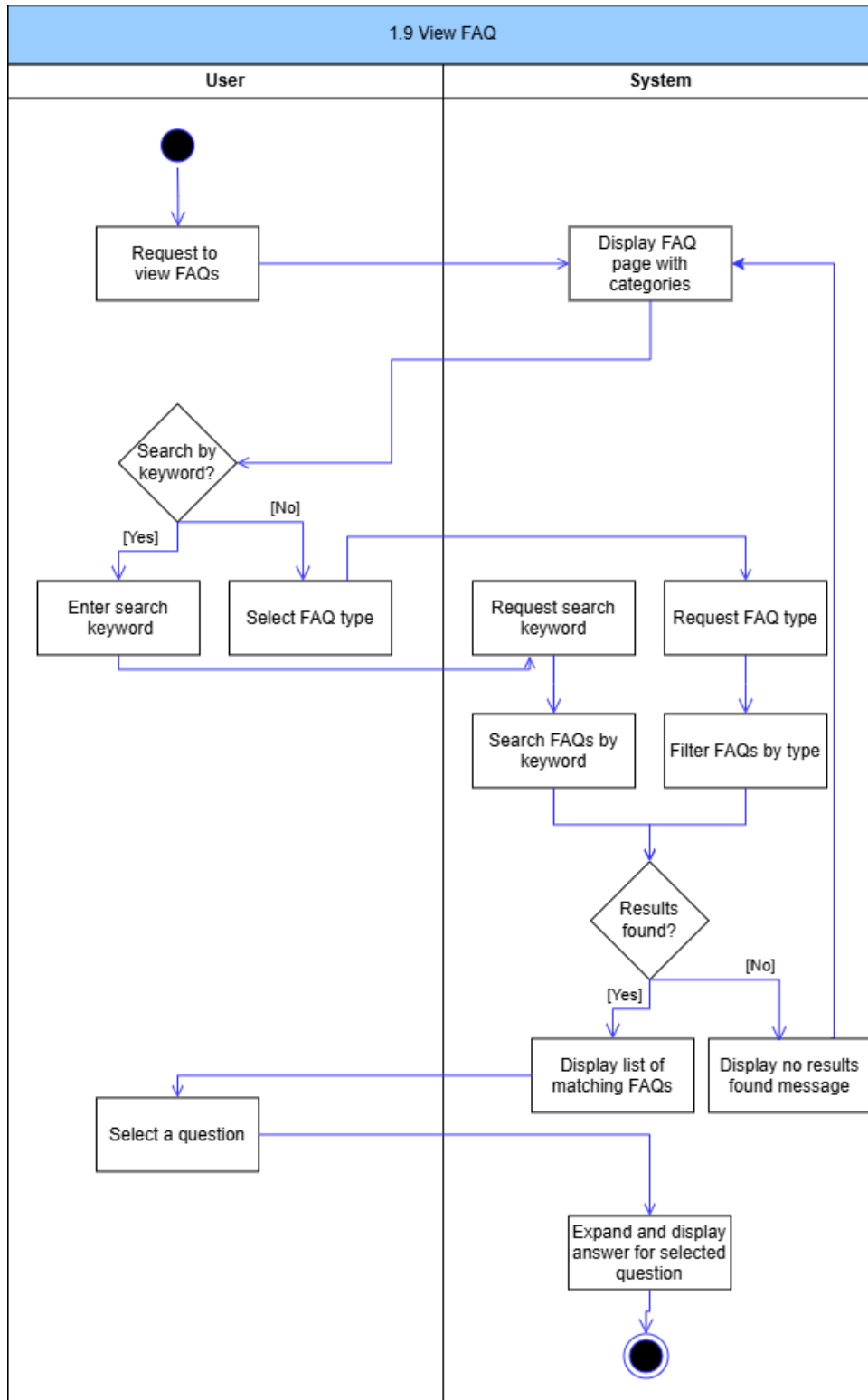
Figure 10: View FAQ Activity Diagram
