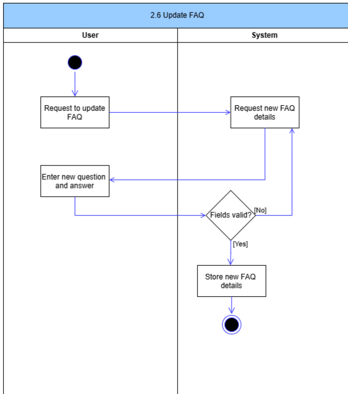
Figure 16: Update FAQ Activity Diagram
