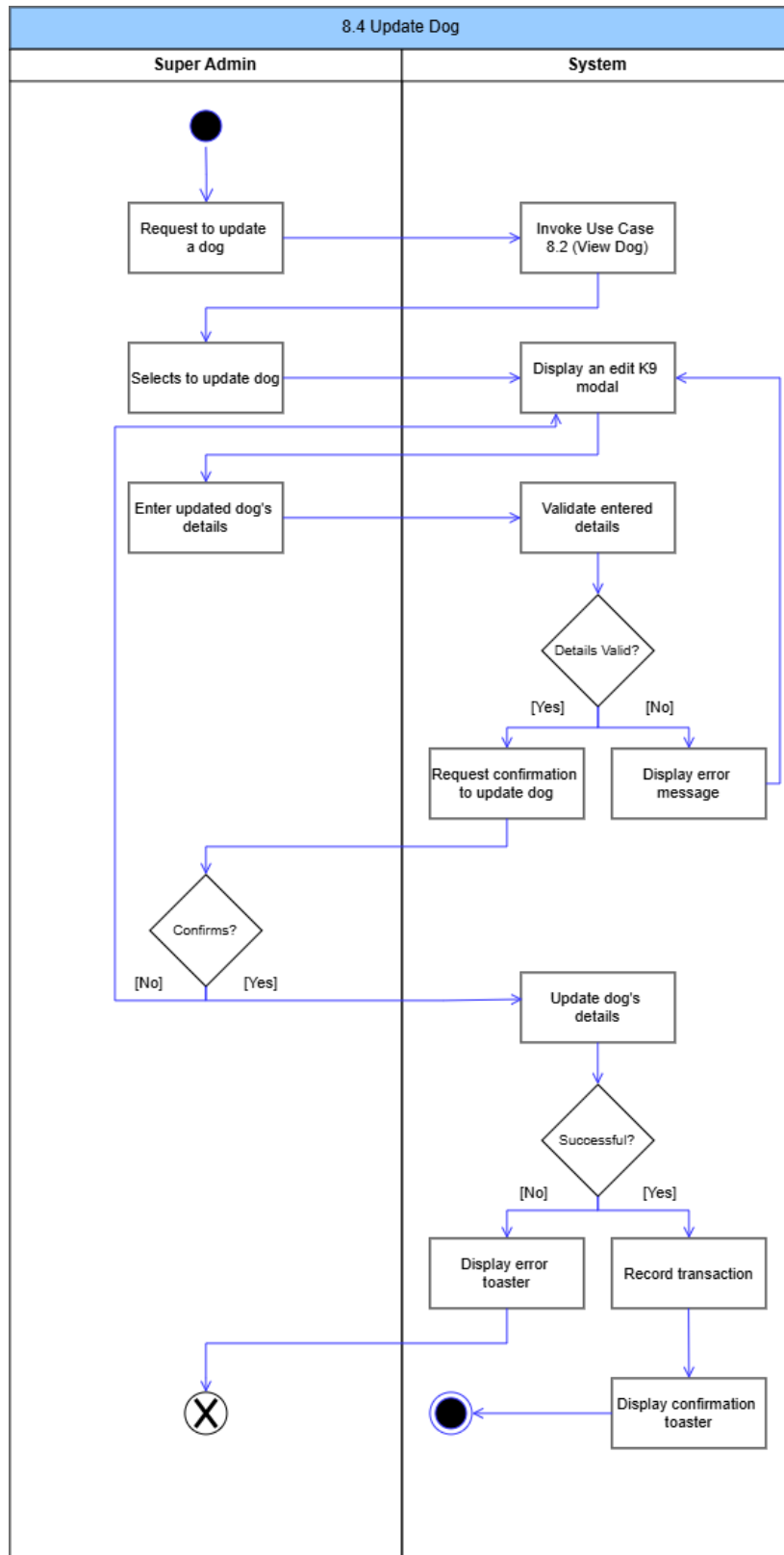
Figure 95: Update Dog Activity Diagram
