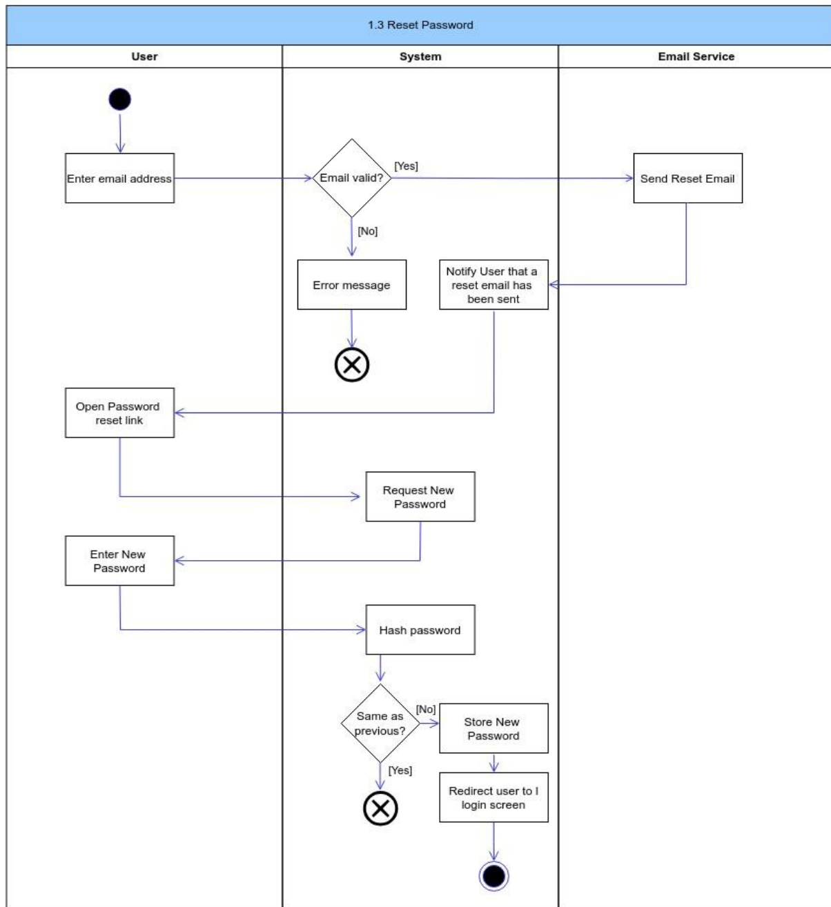
Figure 3: Reset Password Activity Diagram
