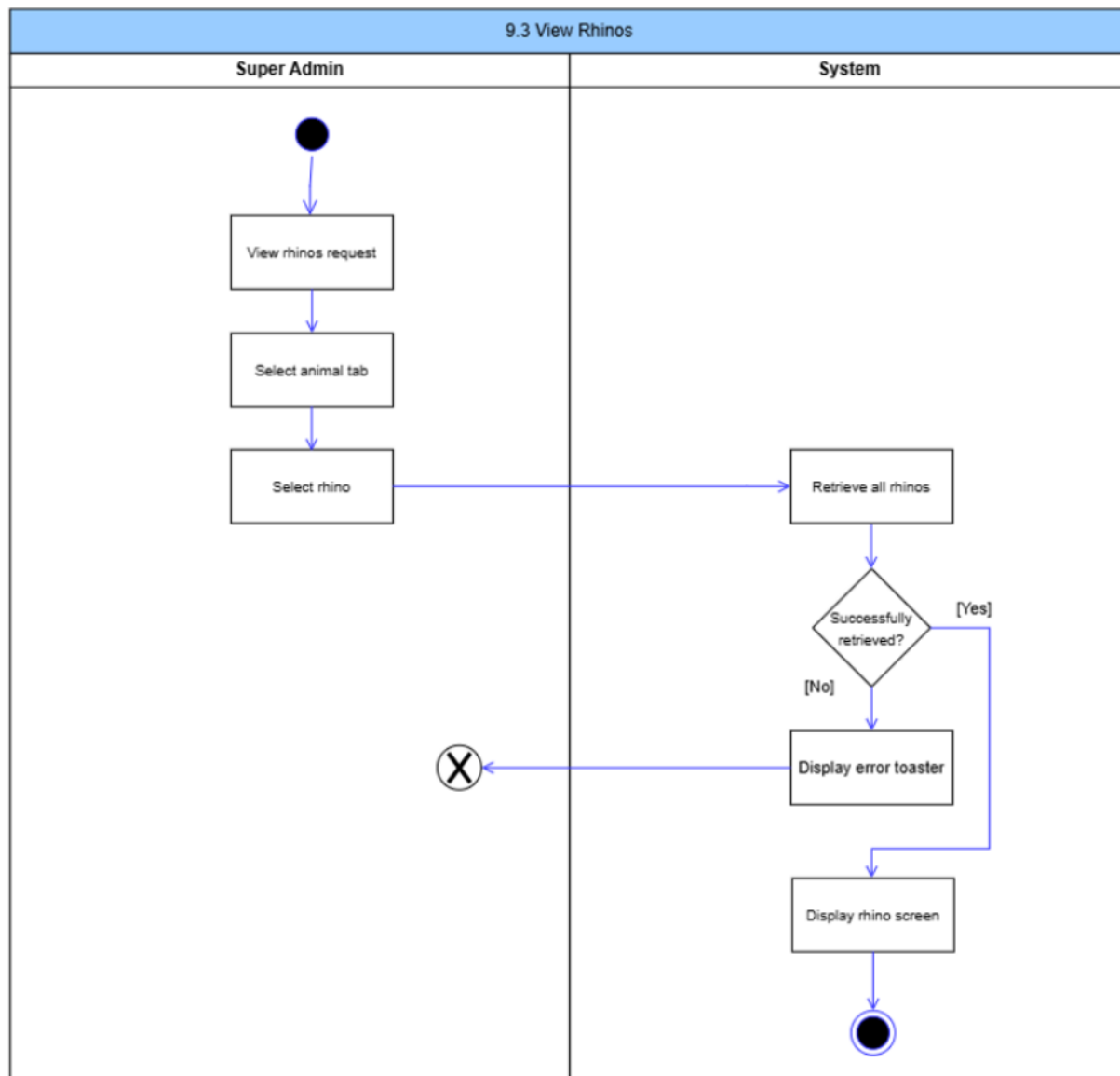
Figure 111: View Rhinos Activity Diagram
