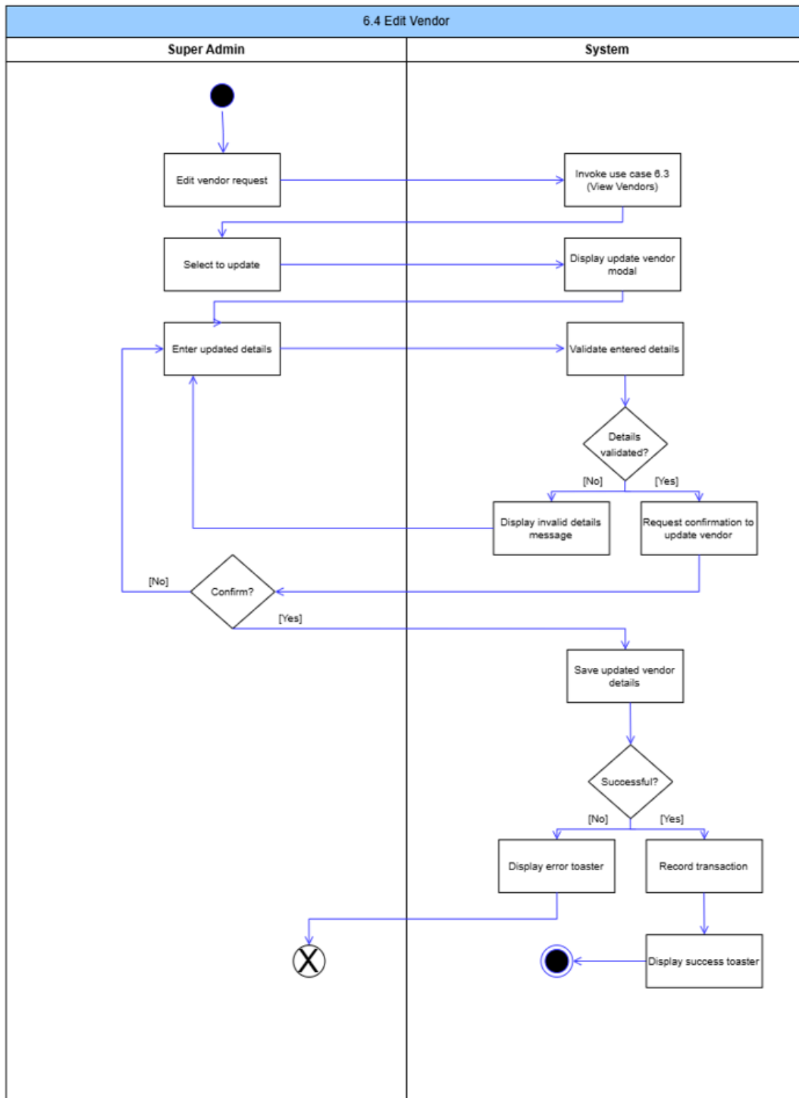
Figure 56: Edit Vendor Activity Diagram
