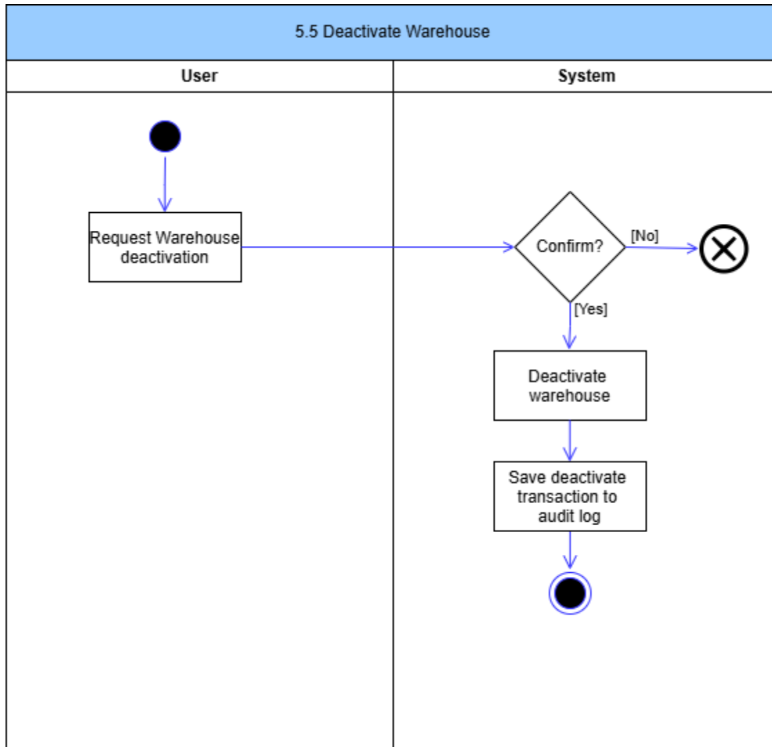
Figure 51: Deactivate Warehouse Activity Diagram
