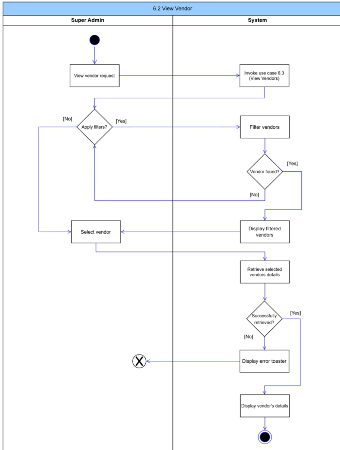
Figure 54: View Vendor Activity Diagram
