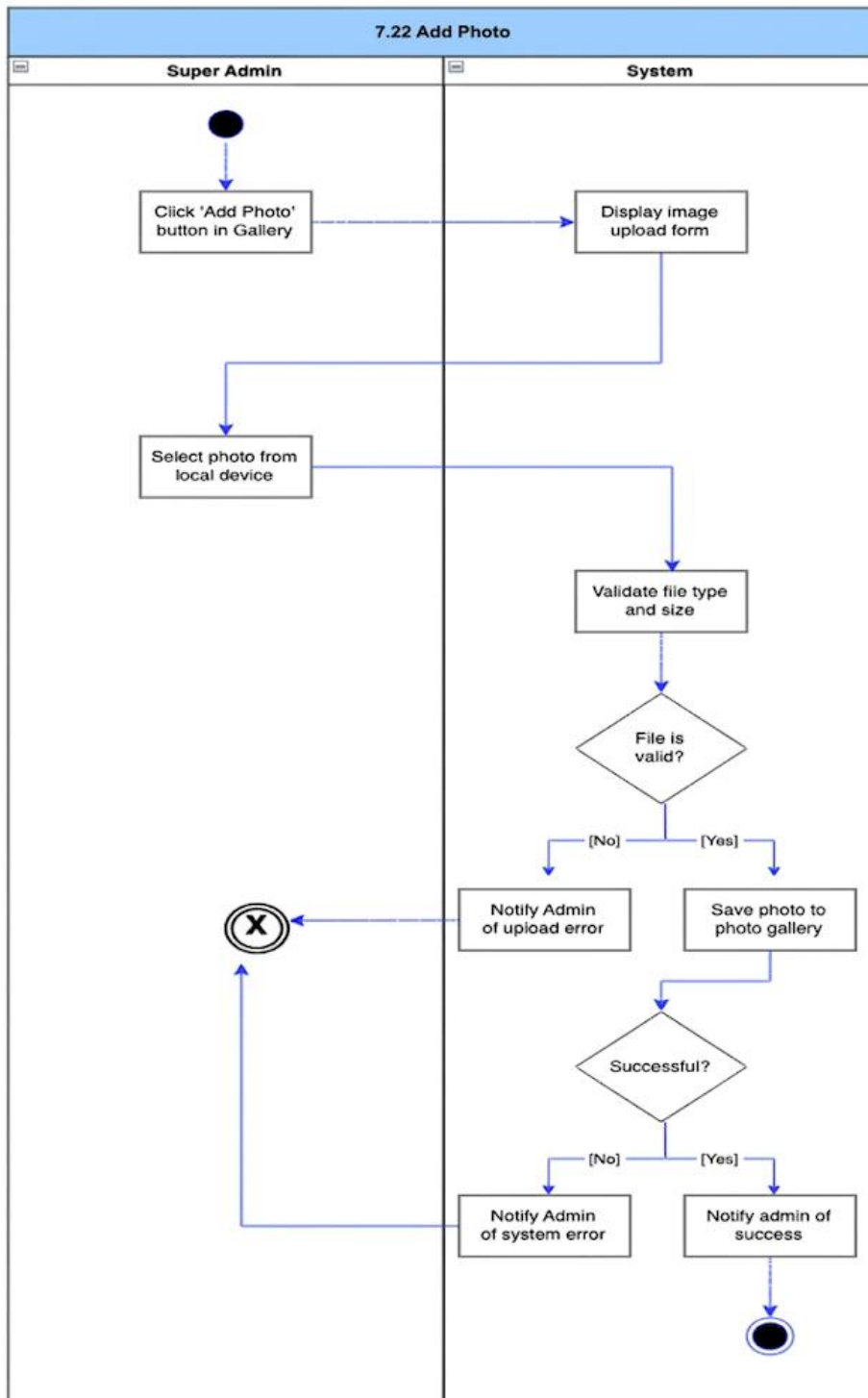
Figure 85: Add Photo Activity Diagram
