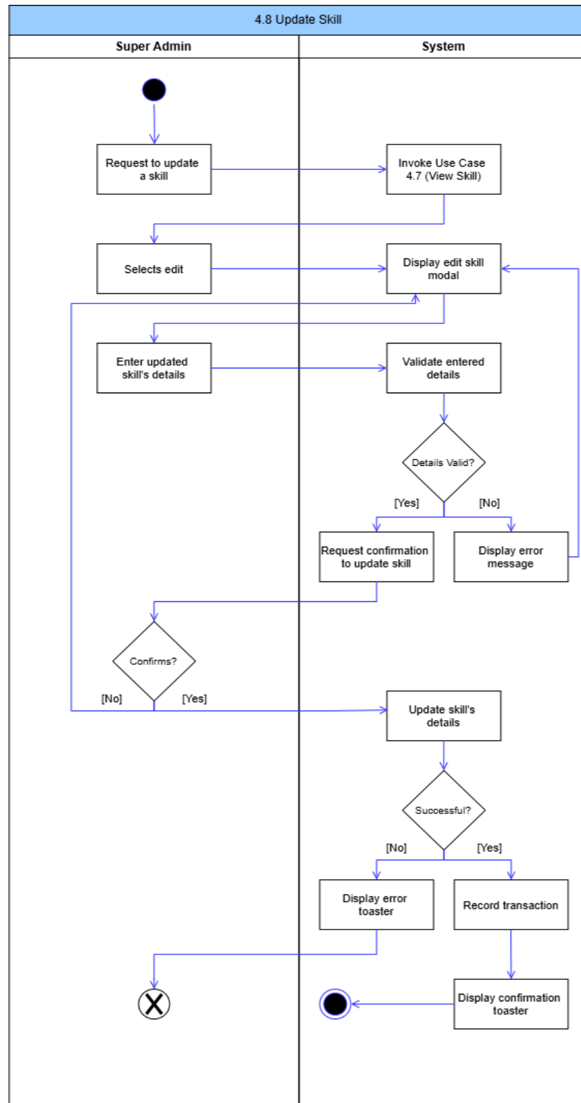
Figure 45: Update Skill Activity Diagram
