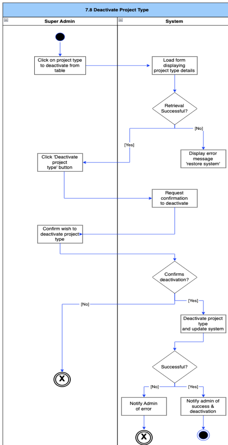
Figure 71: Deactivate Project Type Activity Diagram
