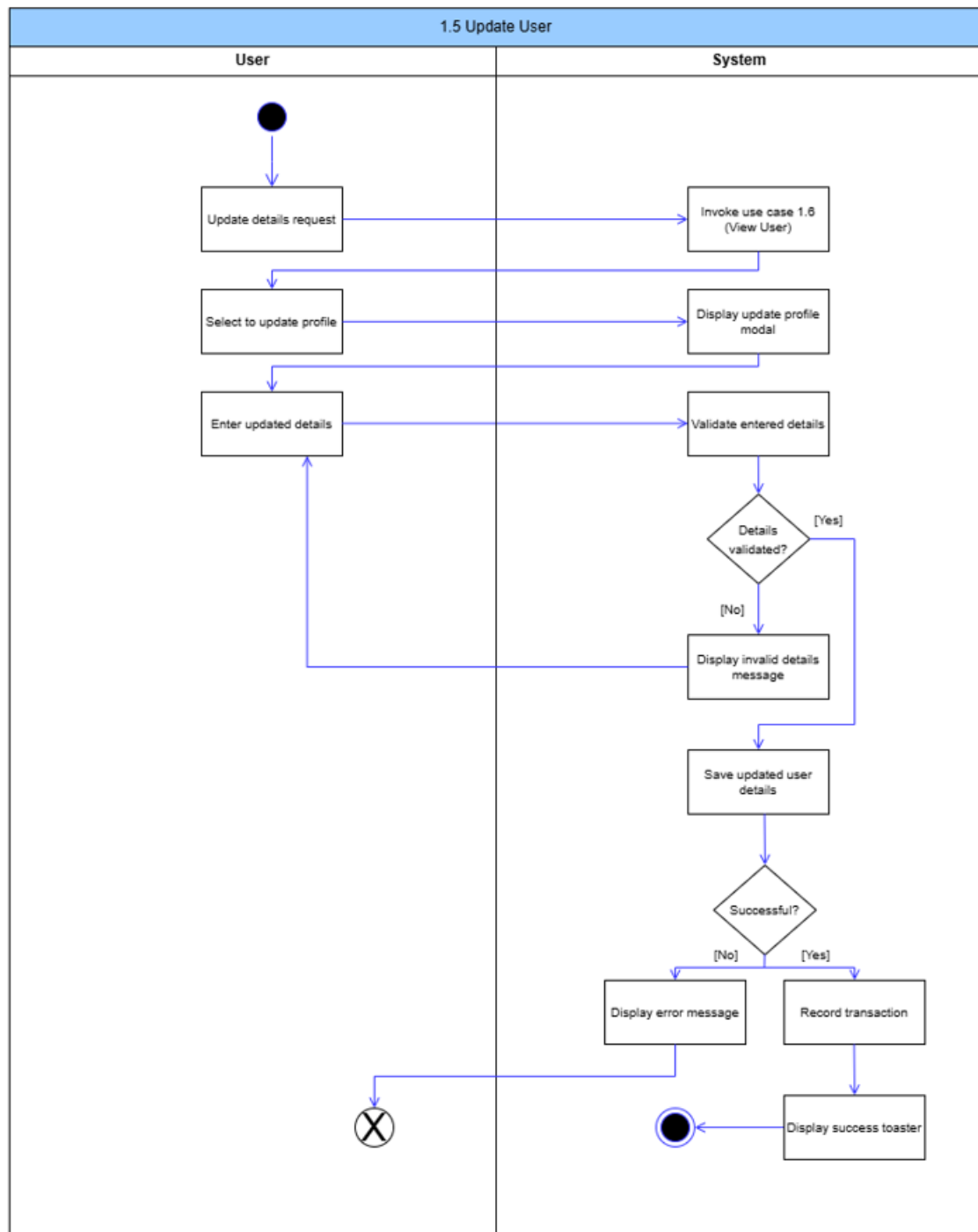
Figure 6: Update User Activity Diagram
