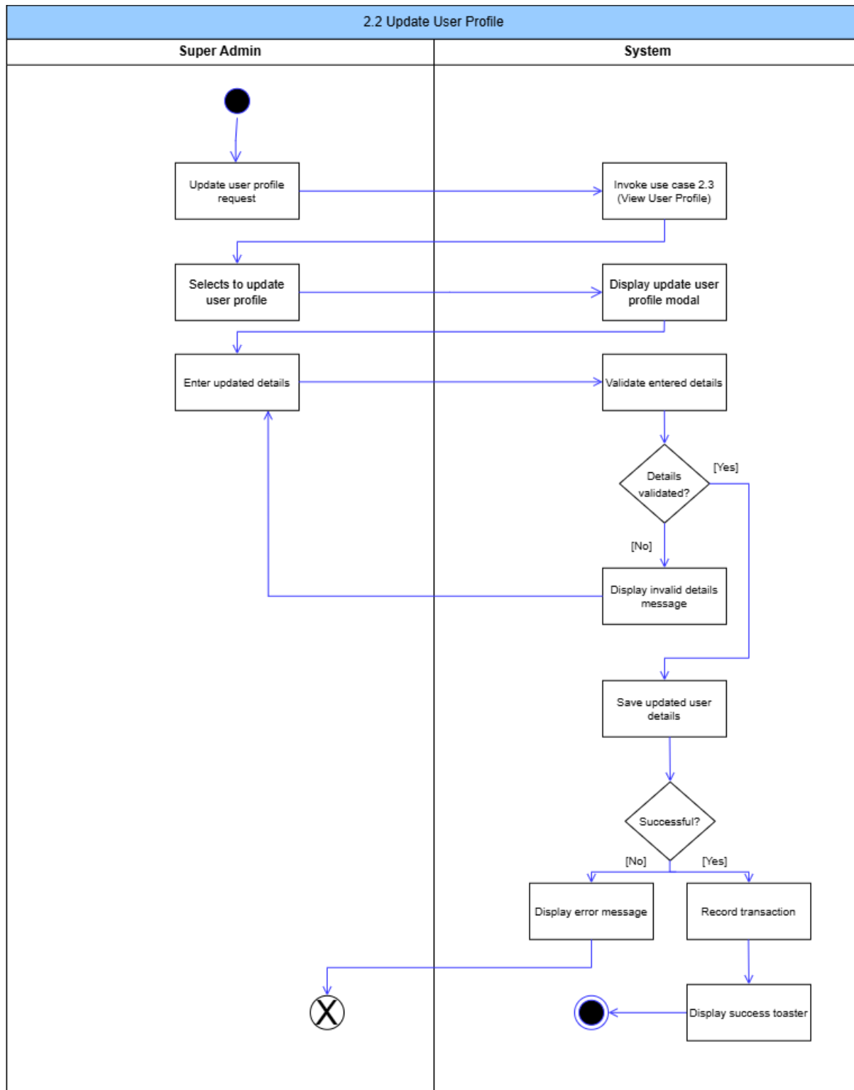
Figure 12: Update User Profile Activity Diagram
