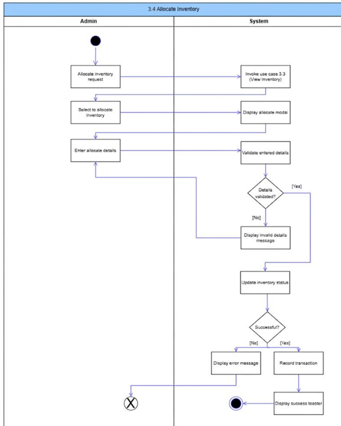
Figure 31: Allocate Inventory Activity Diagram
