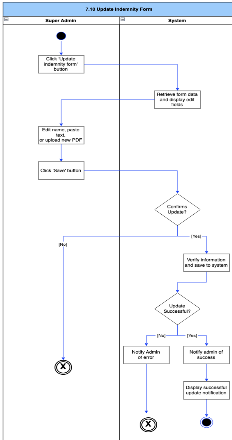
Figure 73: Update Indemnity Form Activity Diagram
