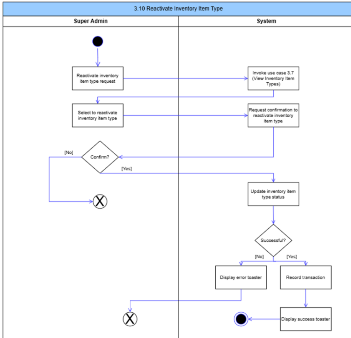
Figure 37: Reactivate Inventory Item Type Activity Diagram
