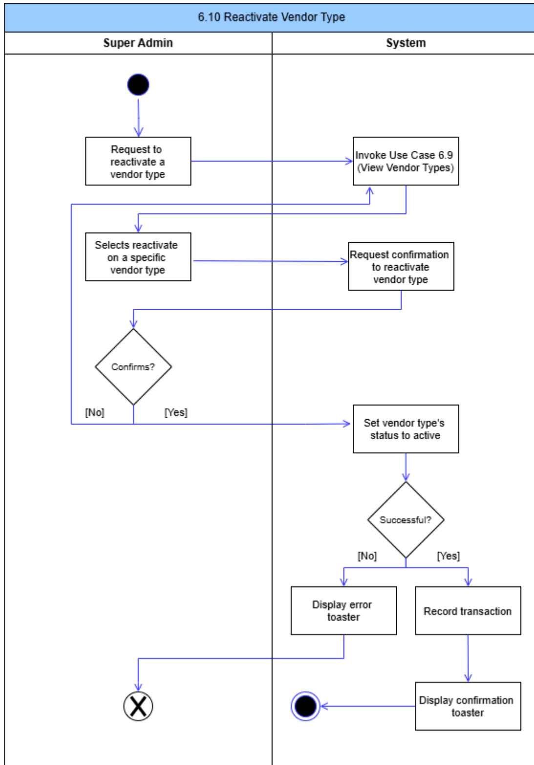
Figure 62: Reactivate Vendor Type Activity Diagram
