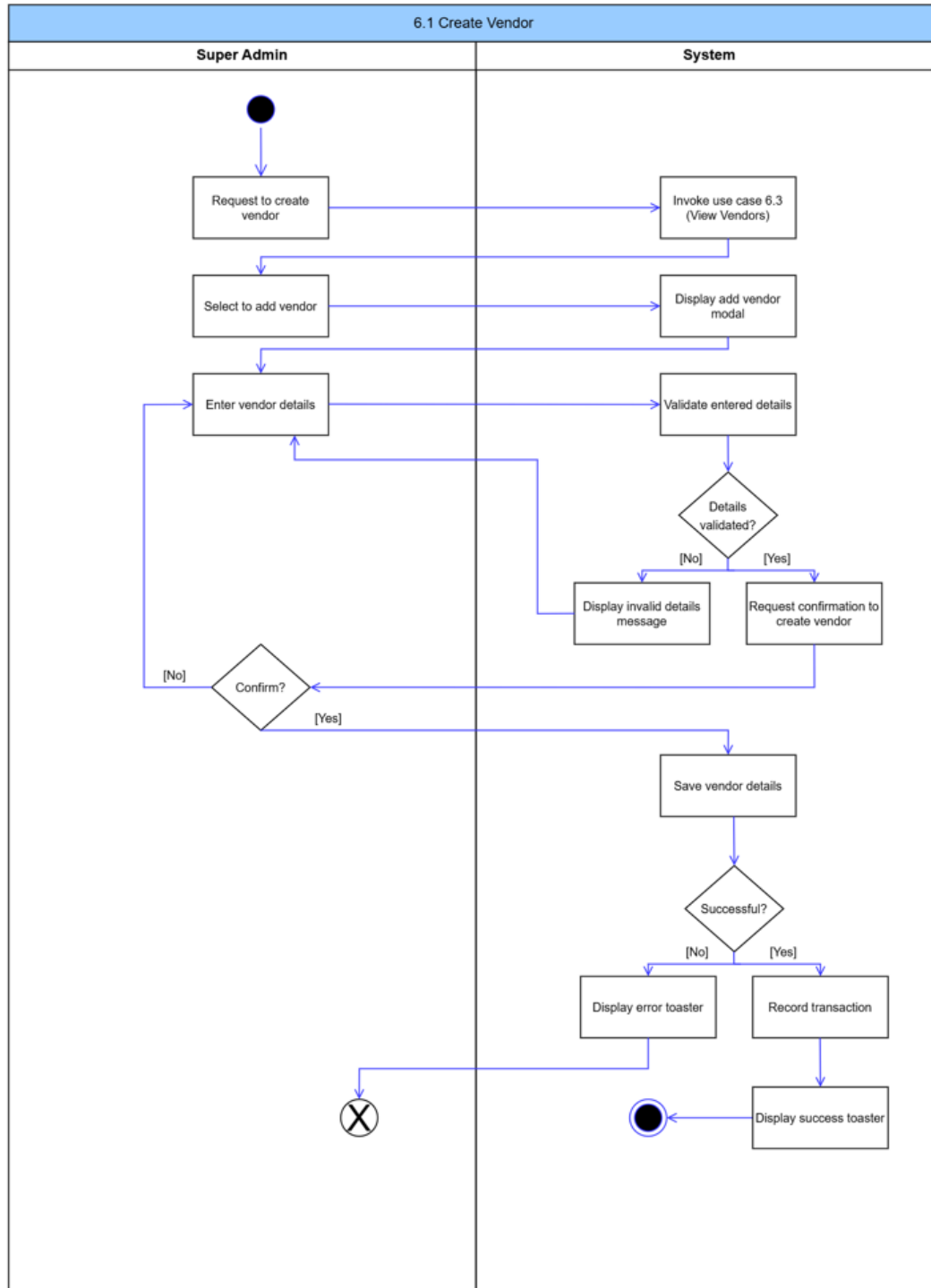
Figure 53: Create Vendor Activity Diagram
