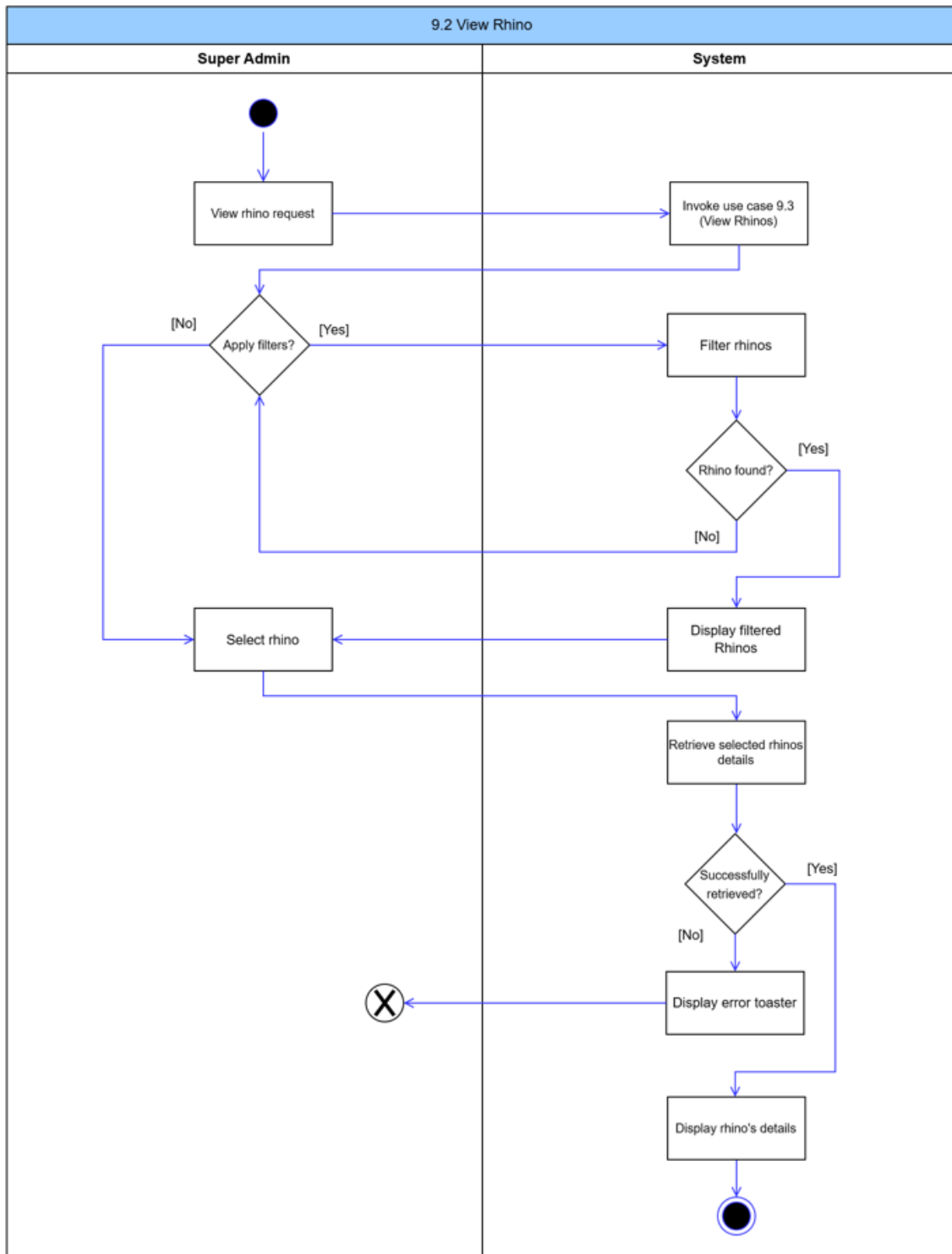
Figure 110: View Rhino Activity Diagram
