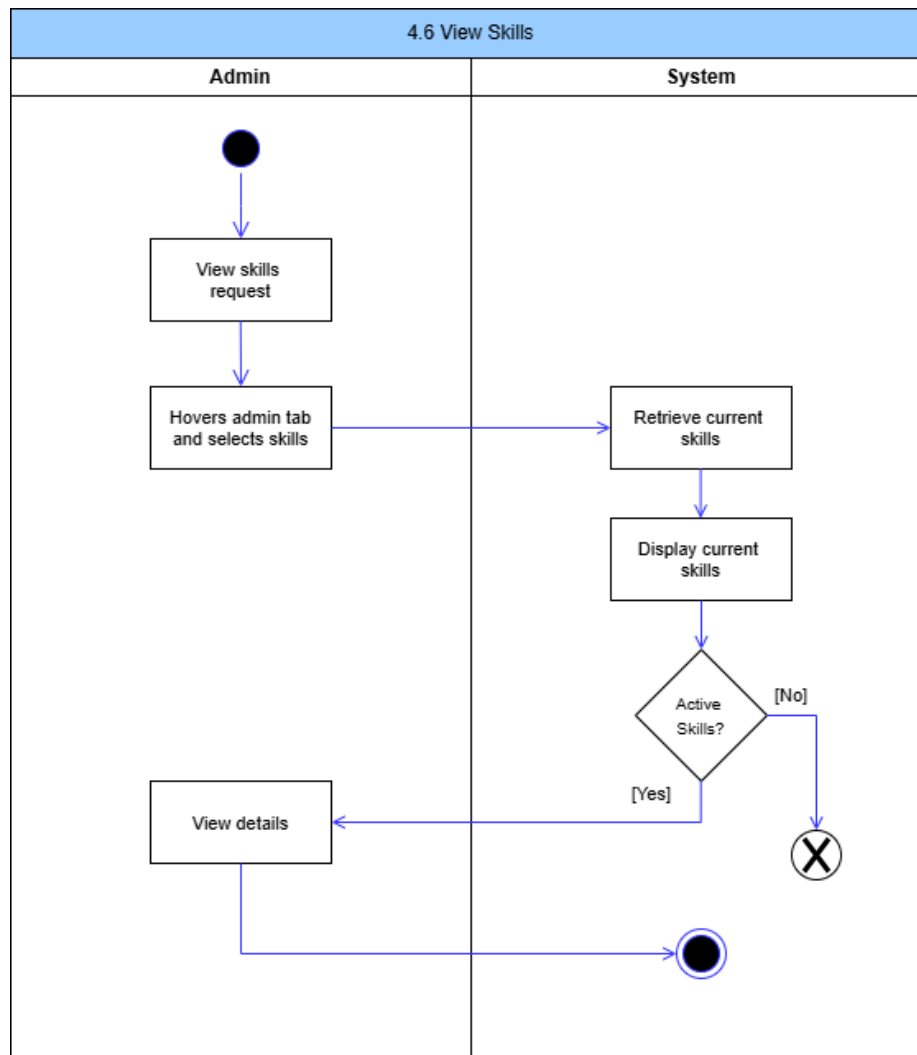
Figure 43: View Skills Activity Diagram
