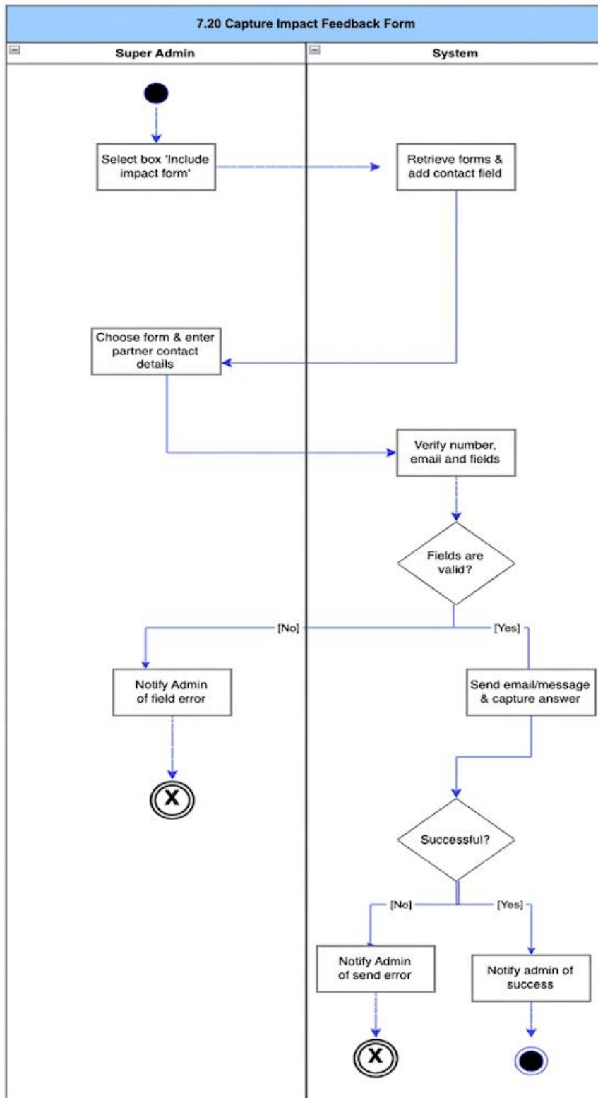
Figure 83: Capture Impact Feedback Activity Diagram
