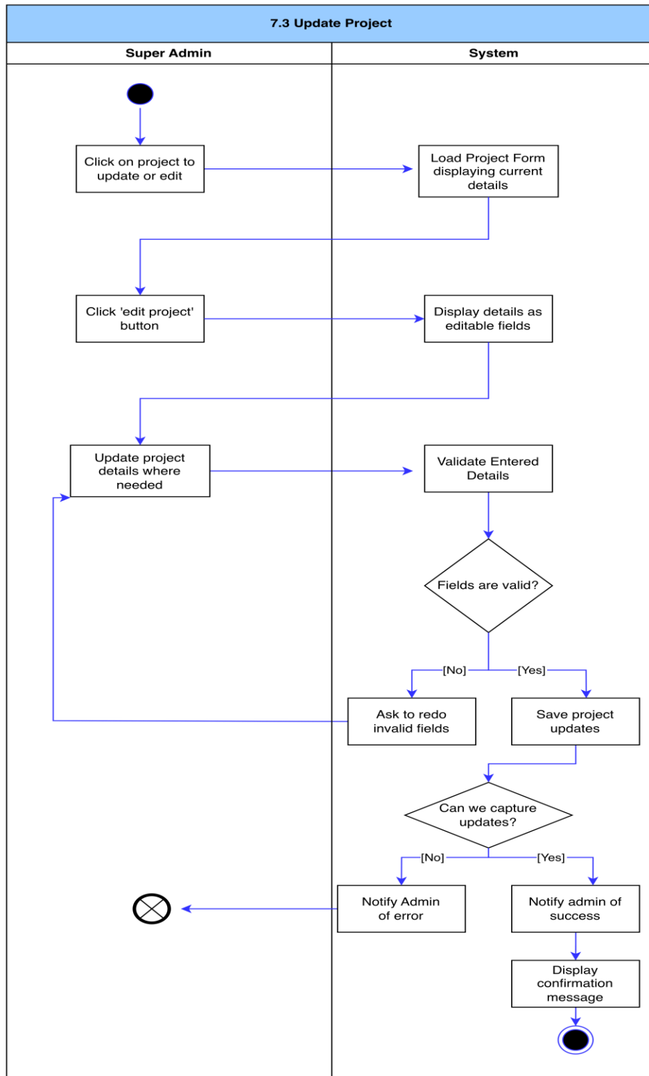
Figure 66: Update Project Activity Diagram
