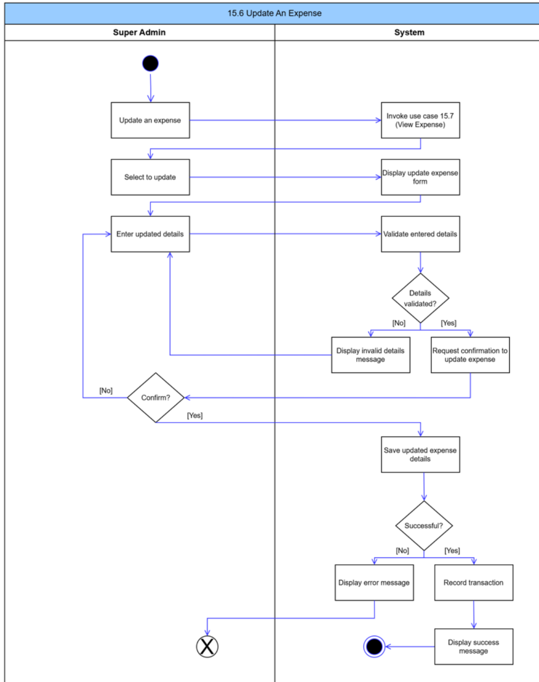
Figure 137: Update Expense Activity Diagram
