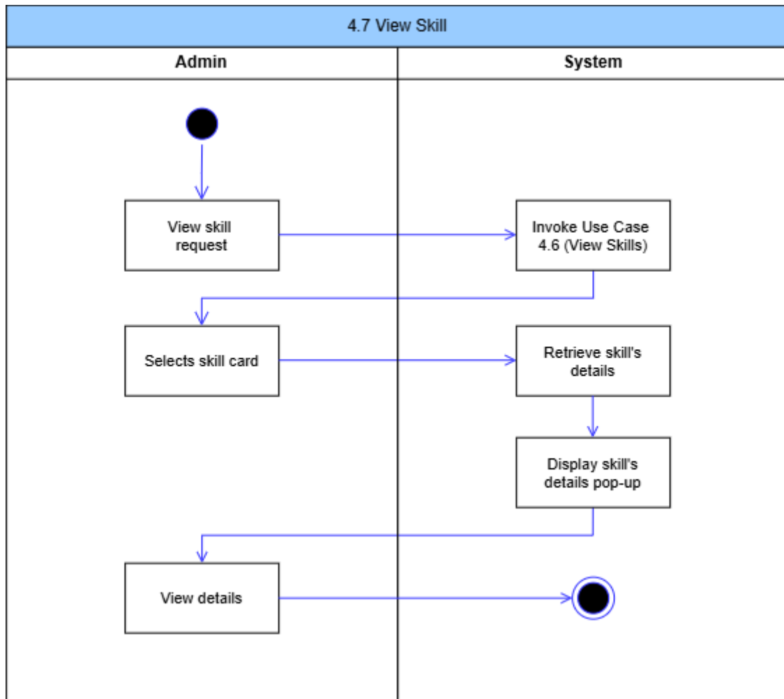
Figure 44: View Skill Activity Diagram
