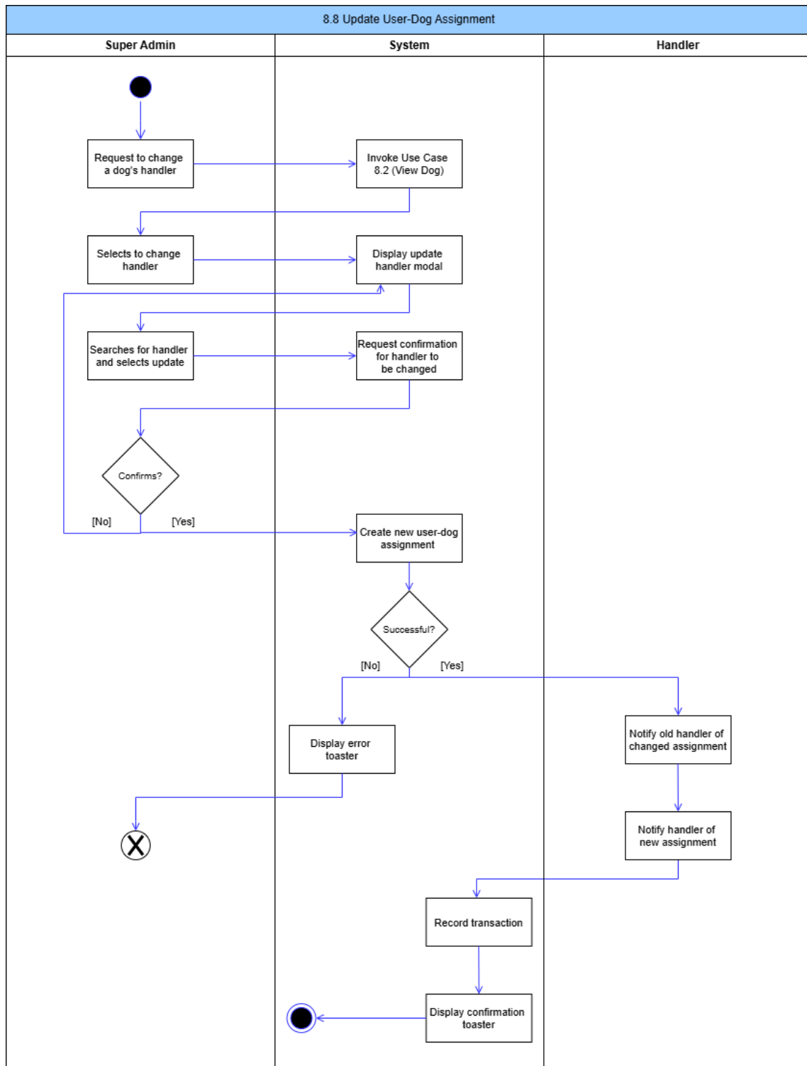
Figure 100: Update User-Dog Assignment Activity Diagram
