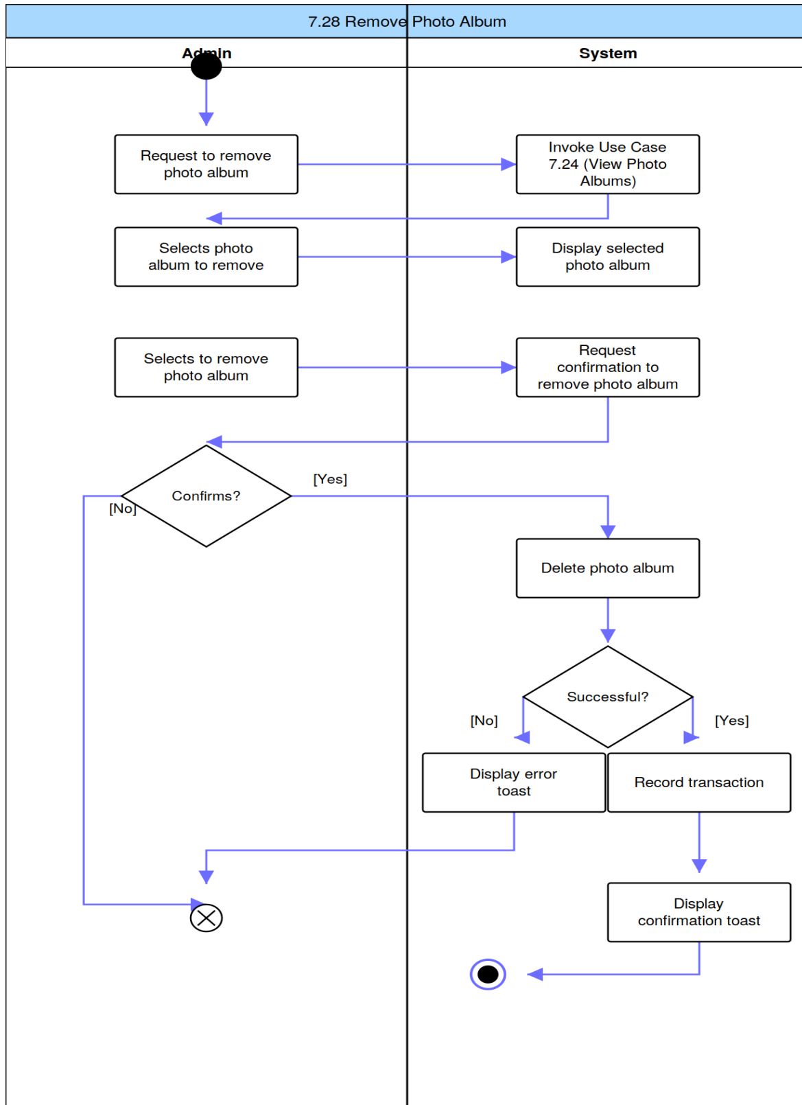
Figure 91: Remove Photo Album Activity Diagram
