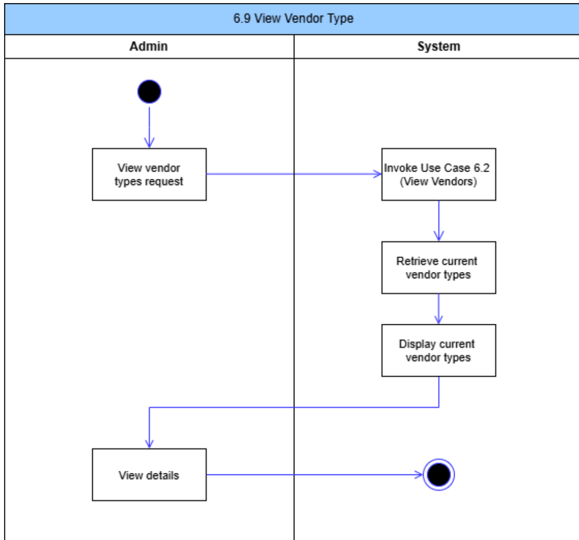
Figure 61: View Vendor Types Activity Diagram
