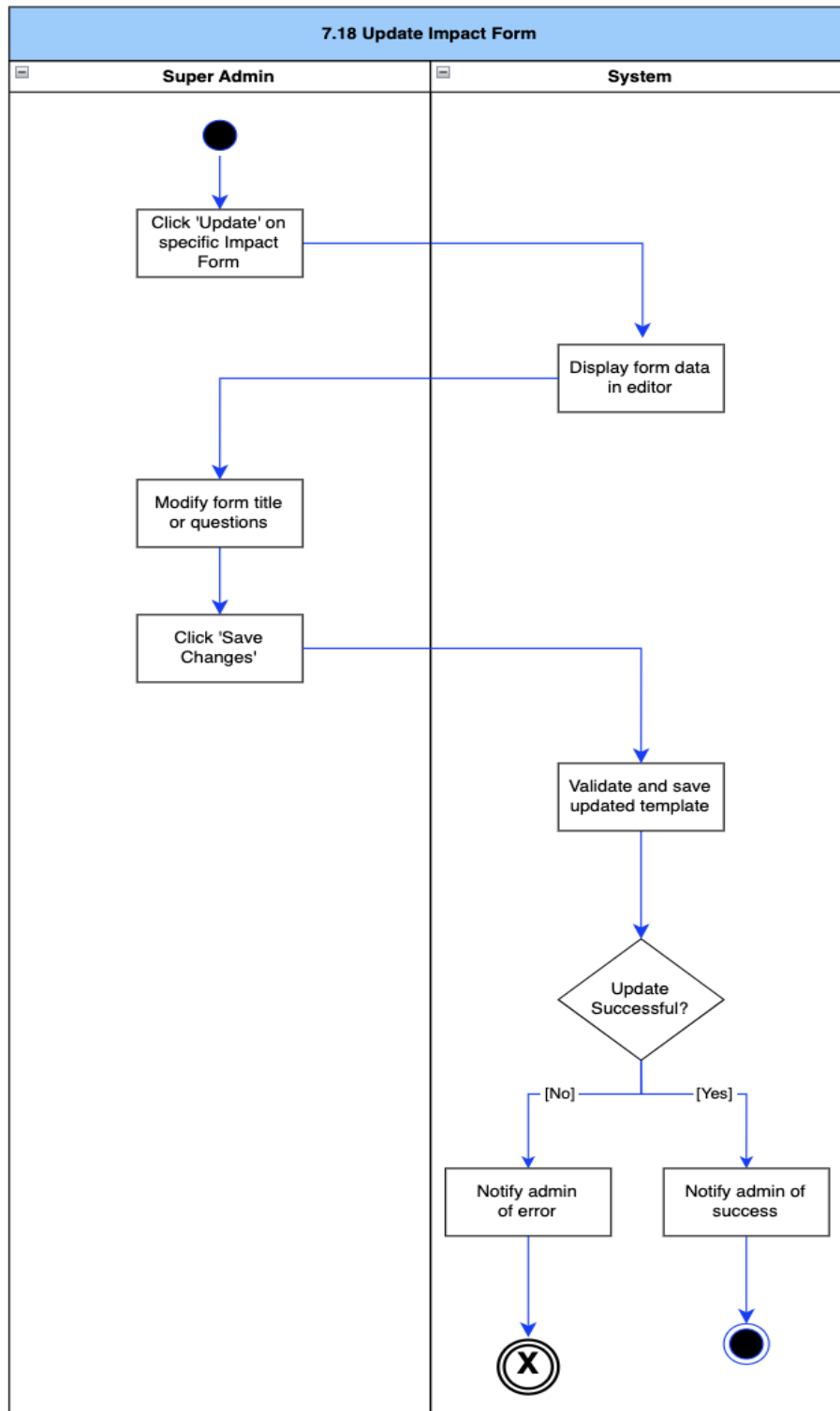
Figure 81: Update Impact Feedback Form Activity Diagram
