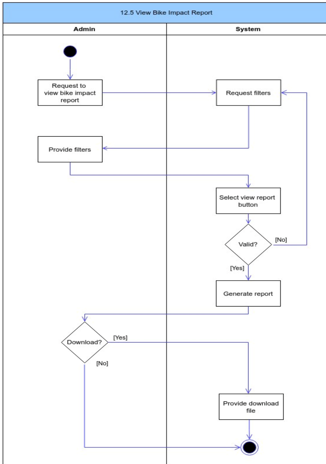
Figure 125: View Bike Impact Report Activity Diagram
