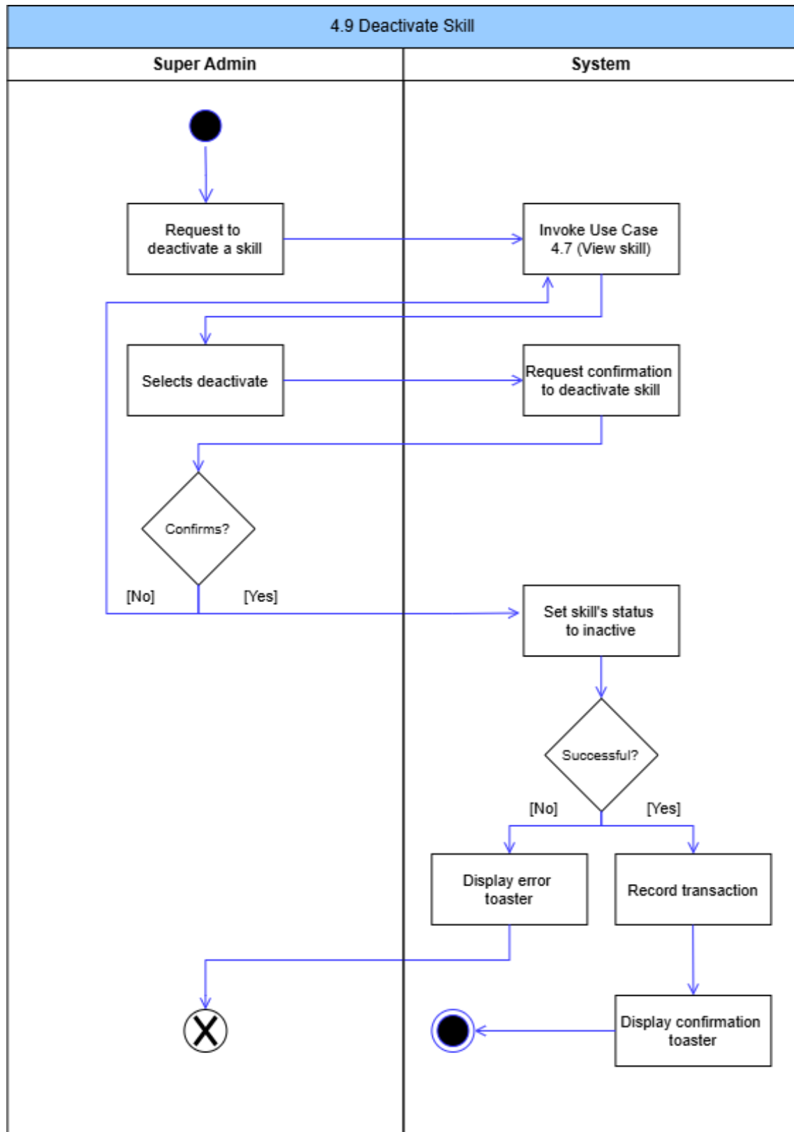
Figure 46: Deactivate Skill Activity Diagram
