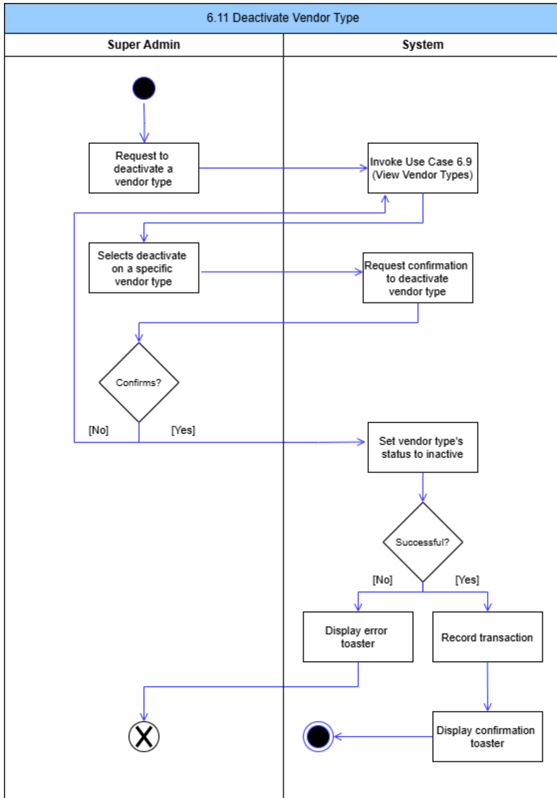
Figure 63: Deactivate Vendor Type Activity Diagram
